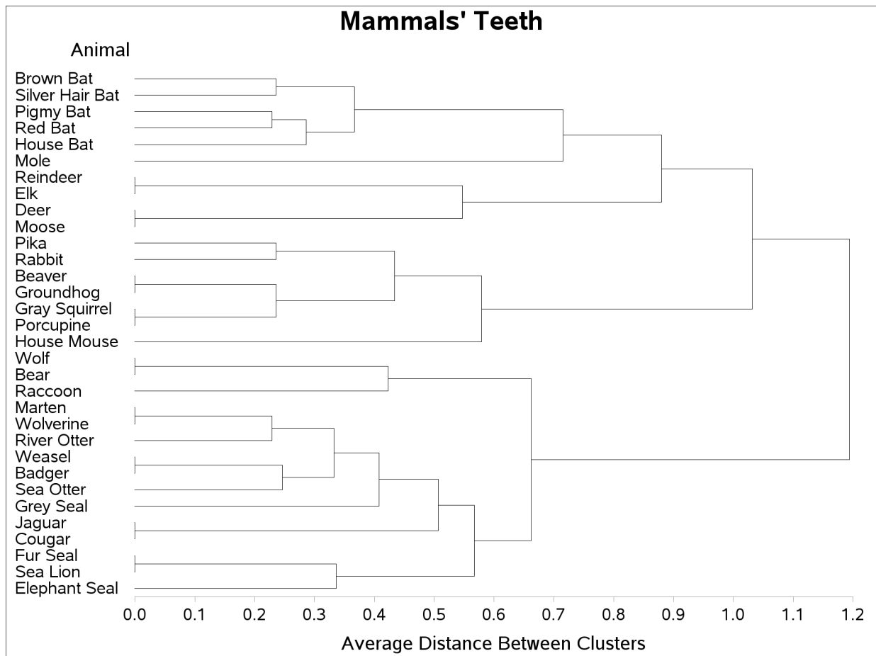
Output 126.1.3 Tree Diagram of Mammal Teeth Clusters
