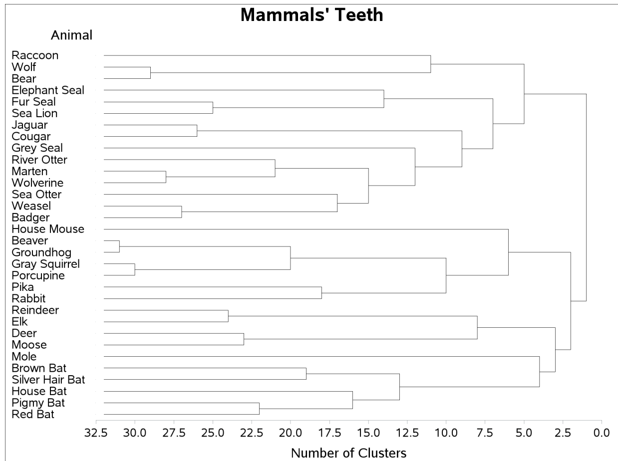
Output 126.1.4 PROC TREE with SORT and HEIGHT= Options
