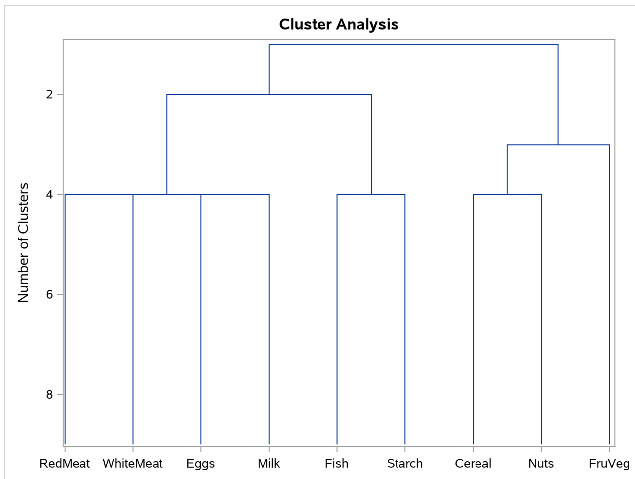
Figure 126.1 Dendrogram from PROC VARCLUS and ODS Graphics
