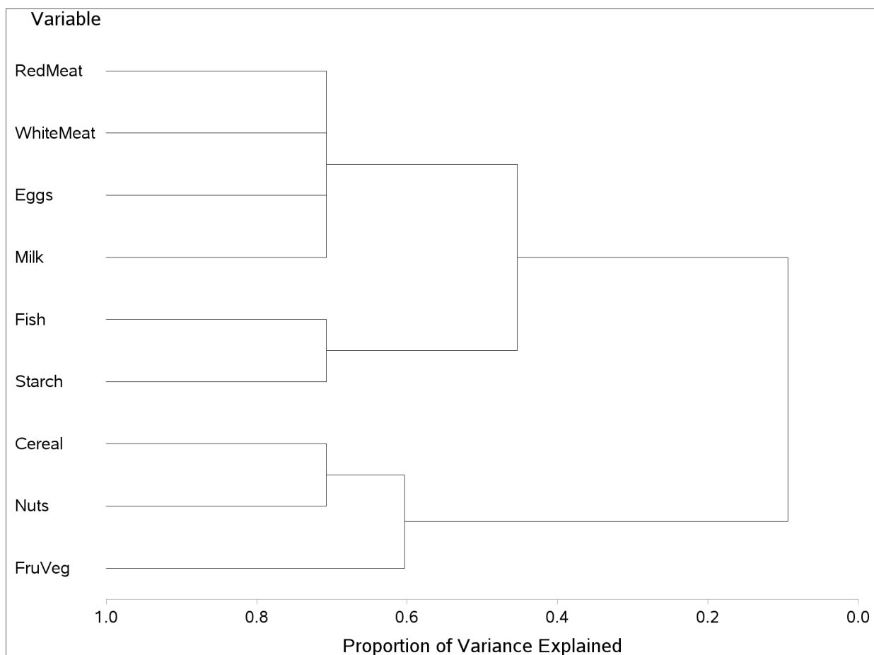
Figure 126.3 Horizontal Tree Diagram with _PROPOR_ as the HEIGHT Variable
