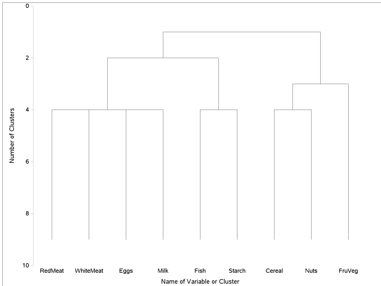
Figure 126.2 Graphical Tree Diagram from PROC TREE
