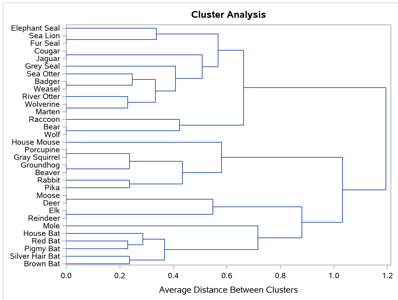
Output 126.1.2 Dendrogram from PROC CLUSTER
