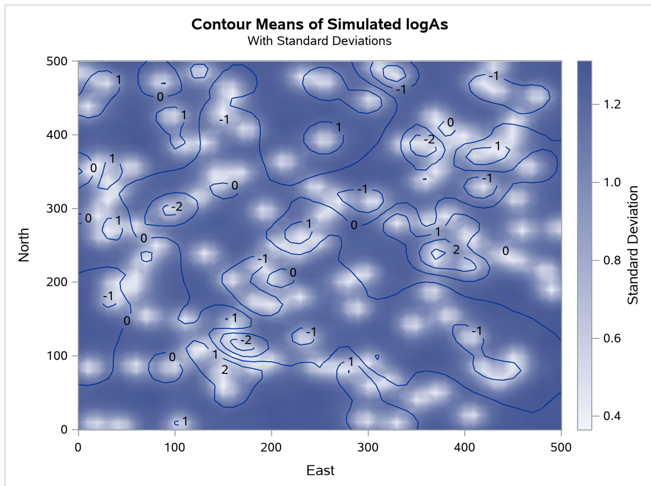
Output 111.3.7 Simulated Arsenic Logarithm Values with Gaussian-Gaussian Covariance
