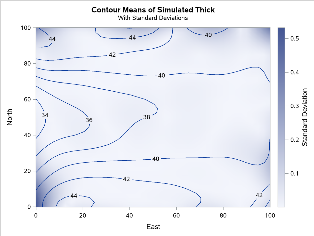
Figure 111.5 Contour Plot of Conditionally Simulated Coal Seam Thickness
