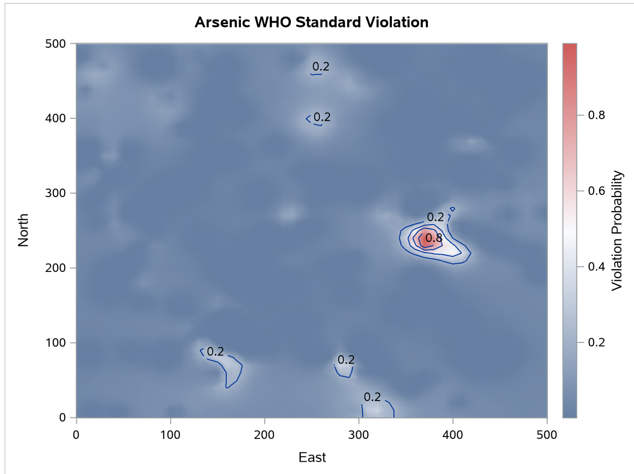
Output 111.3.9 Map of Violation of the Arsenic WHO Standard Probability
