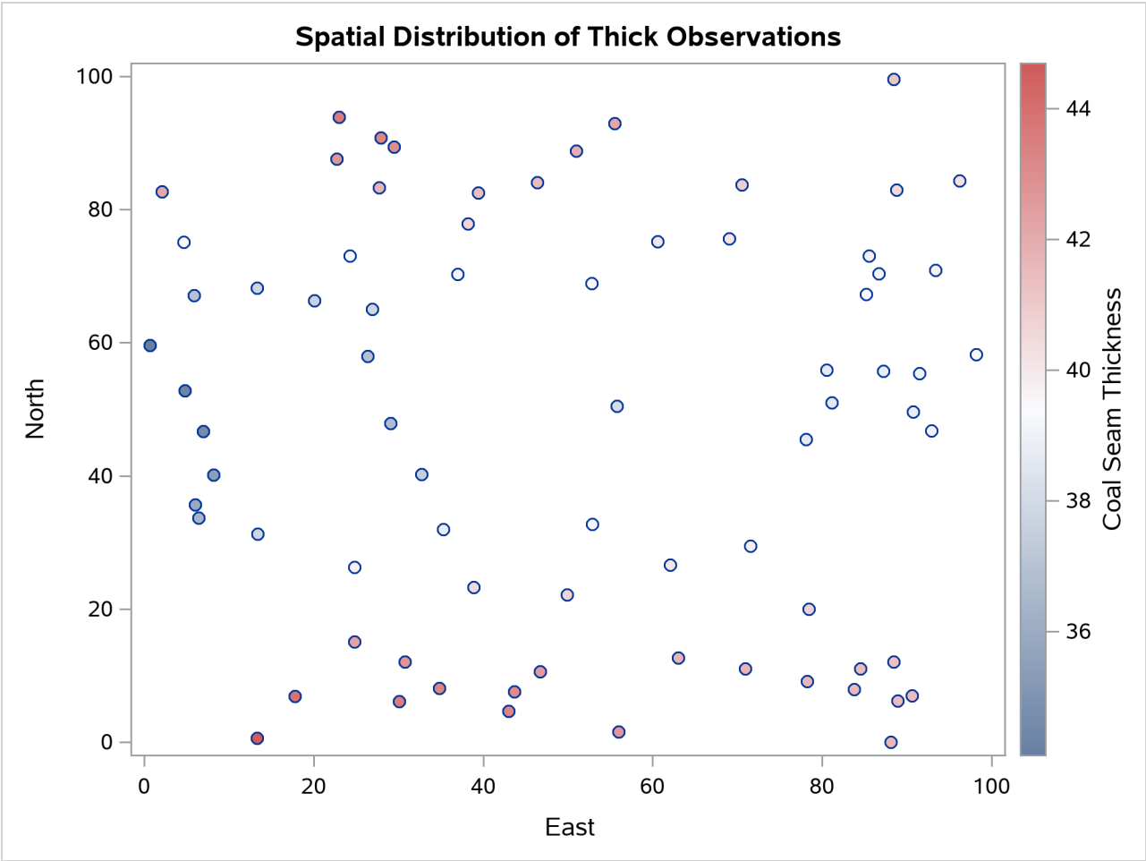
Figure 111.2 Scatter Plot of the Observations Spatial Distribution
