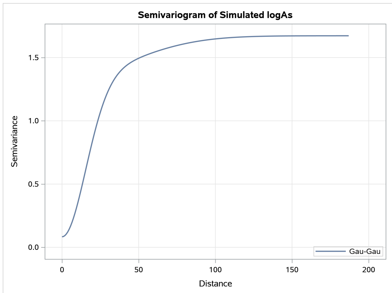
Output 111.3.6 Gaussian-Gaussian Semivariogram Model Used in Simulation
