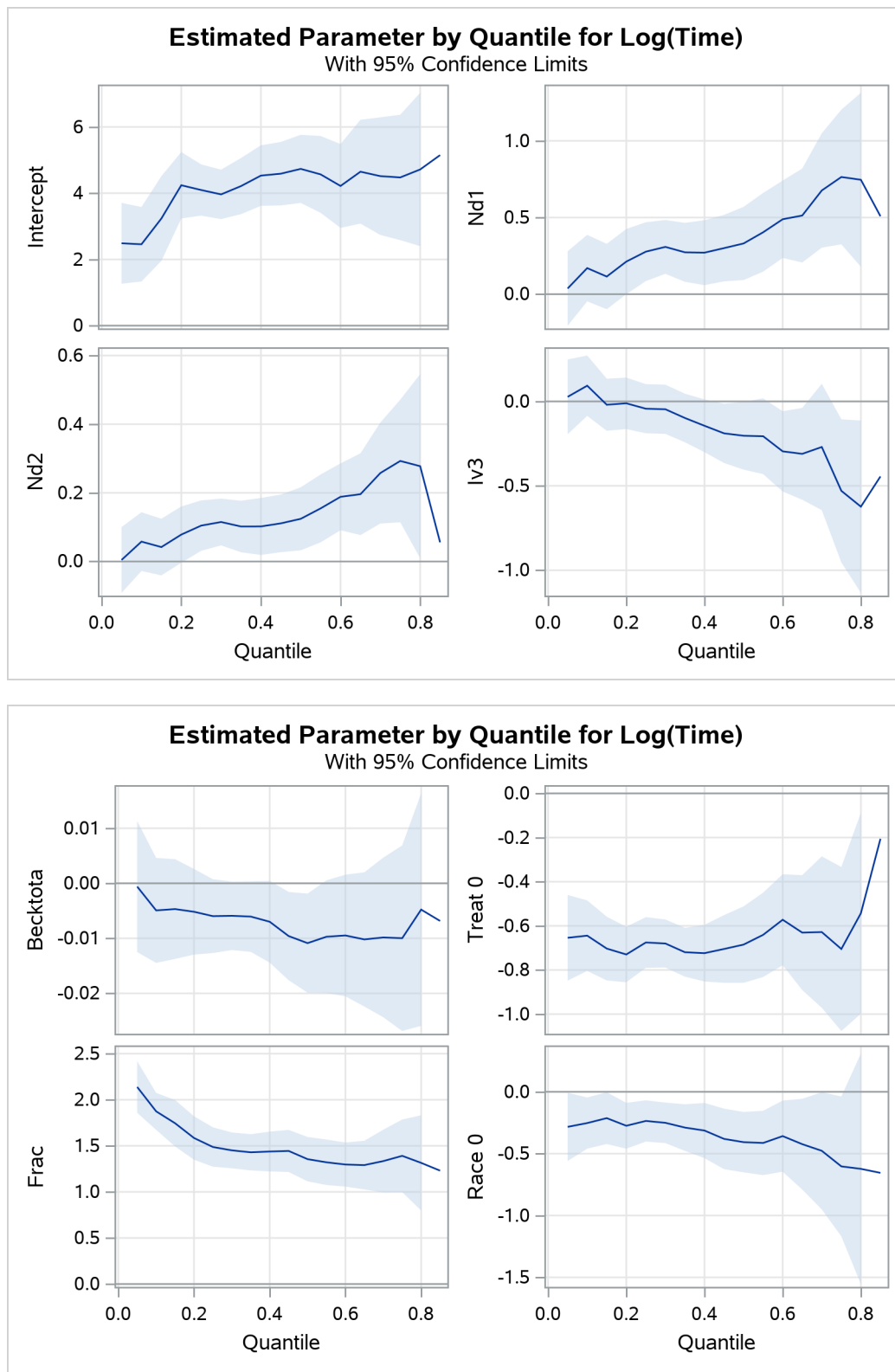
Output 101.2.2 Quantile Processes with 95% Confidence Bands
