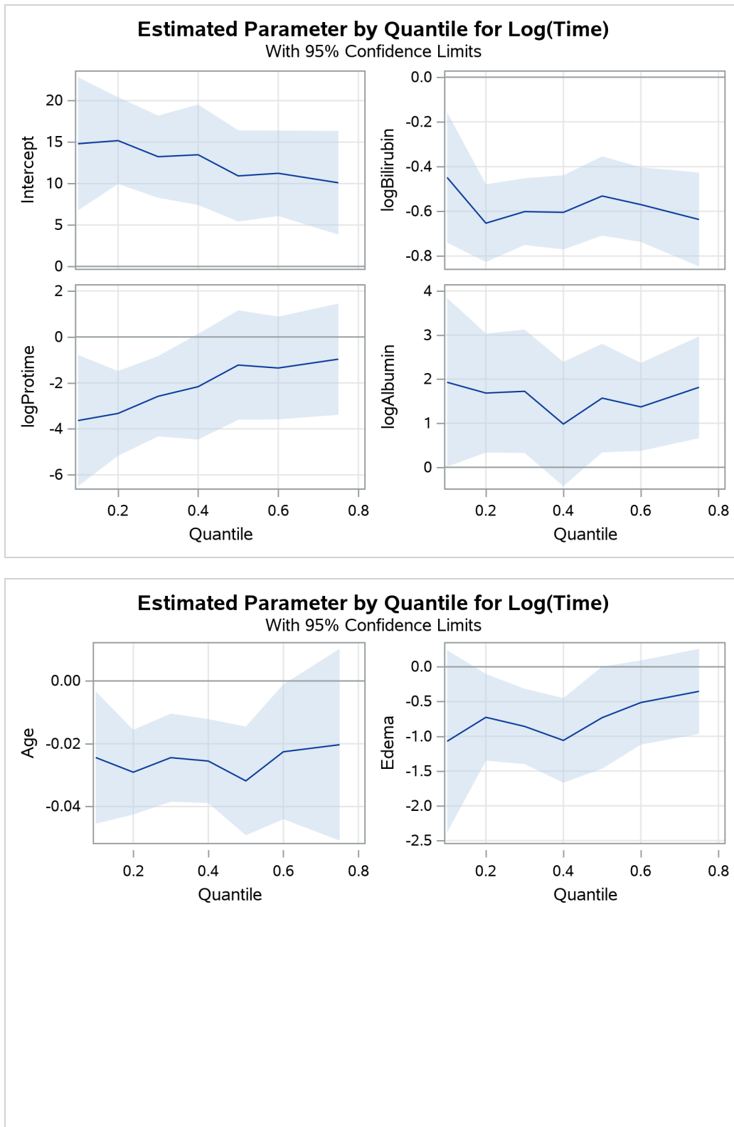
Output 101.1.4 Quantile Processes with 95% Confidence Bands
