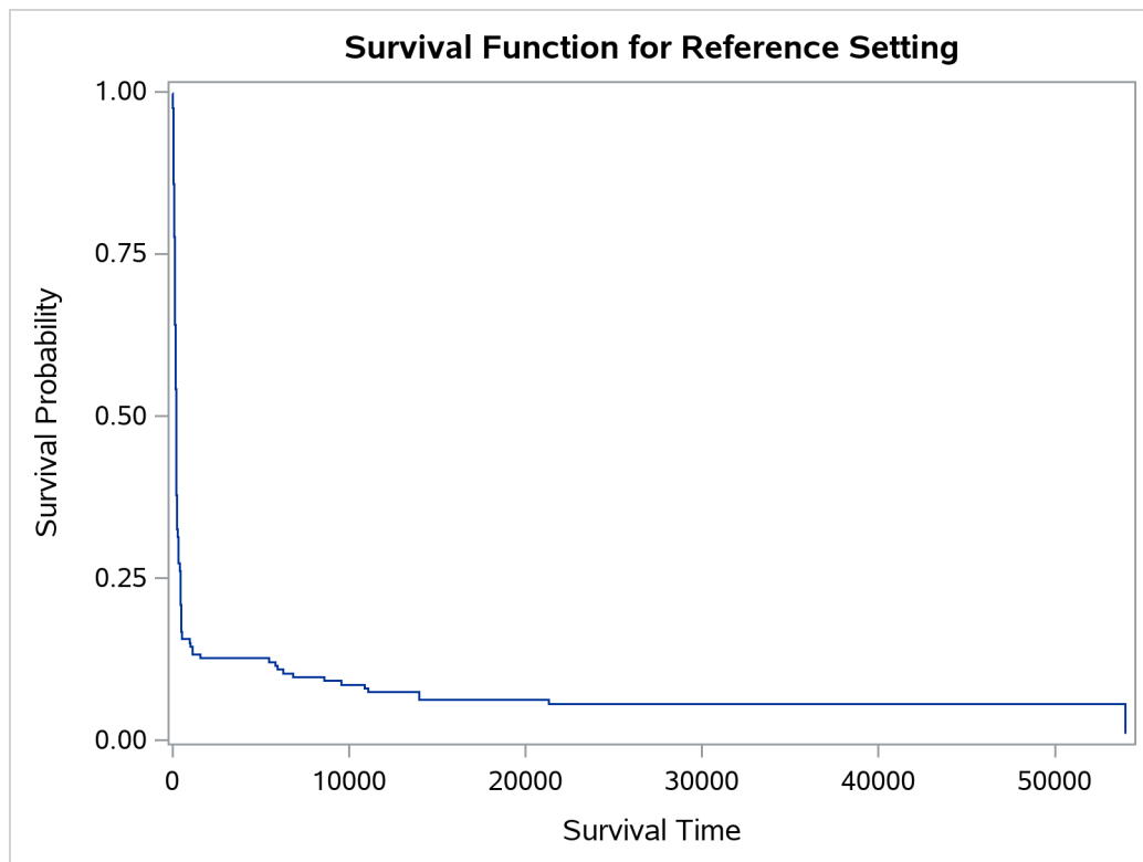
Output 101.2.3 Survival Function
