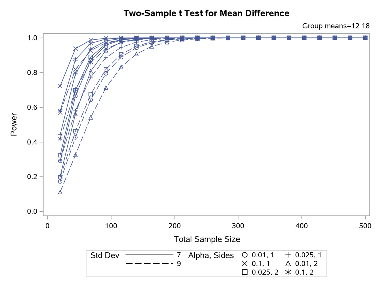
Output 95.8.16 Plot with Features Explicitly Linked to Parameters
