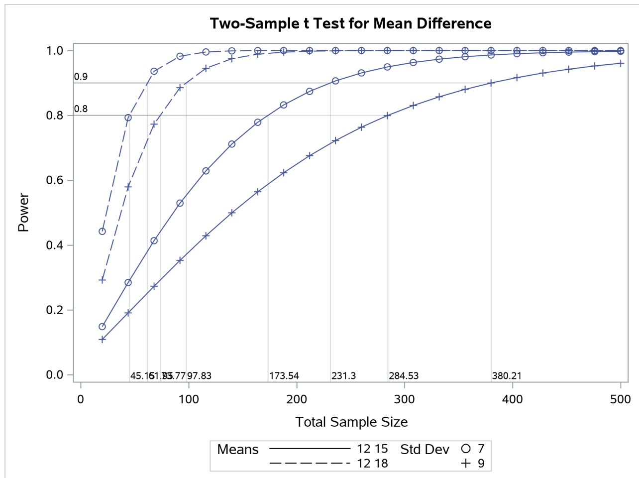
Output 95.8.12 Plot with CROSSREF=YES Style Reference Lines from Y Axis
