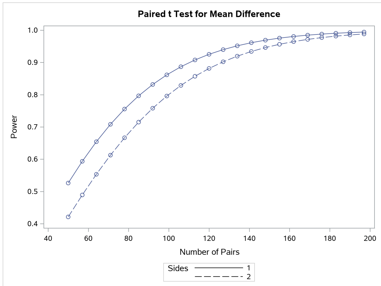
Output 95.3.2 Plot of Power versus Sample Size for Paired t Analysis of Crossover Design
