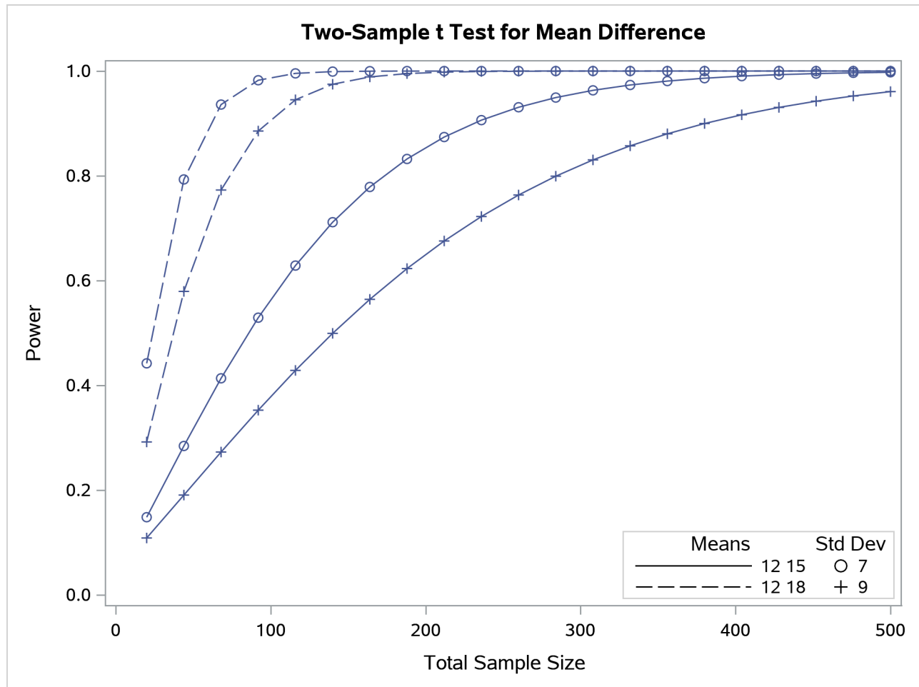
Output 95.8.19 Plot with a Nonnumbered By-Curve Key
