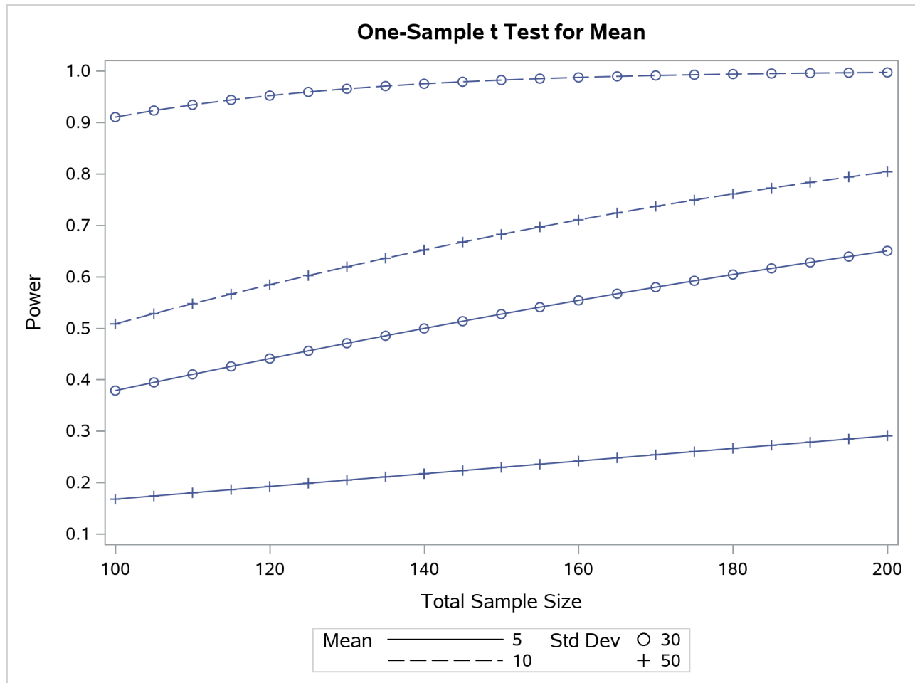
Figure 95.3 Plot of Power versus Sample Size for One-Sample t Test with Input Ranges
