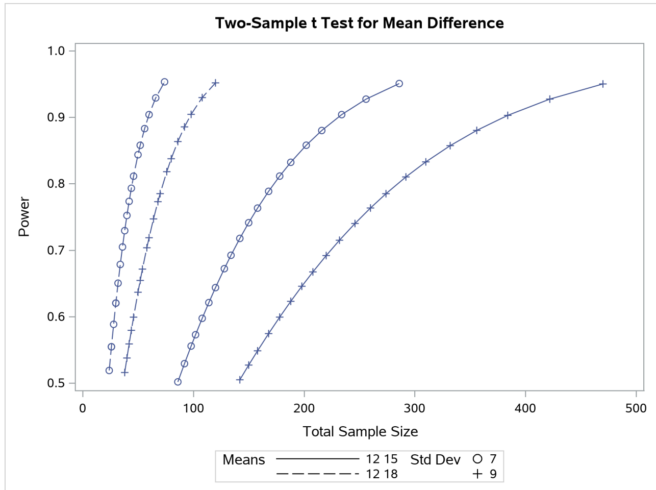
Output 95.8.3 Plot of Power versus Sample Size using First Strategy
