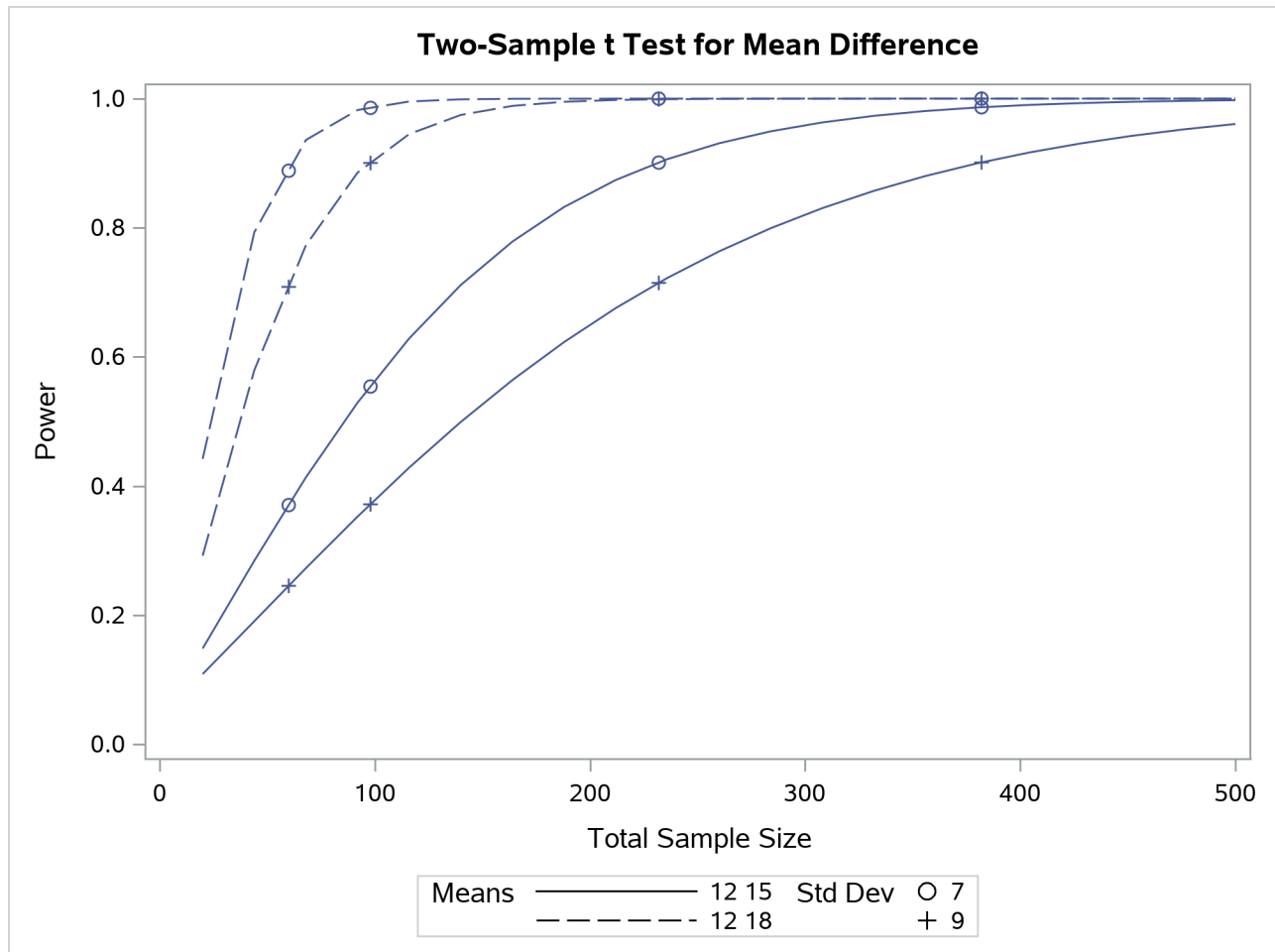
Output 95.8.21 Plot with MARKERS=ANALYSIS
