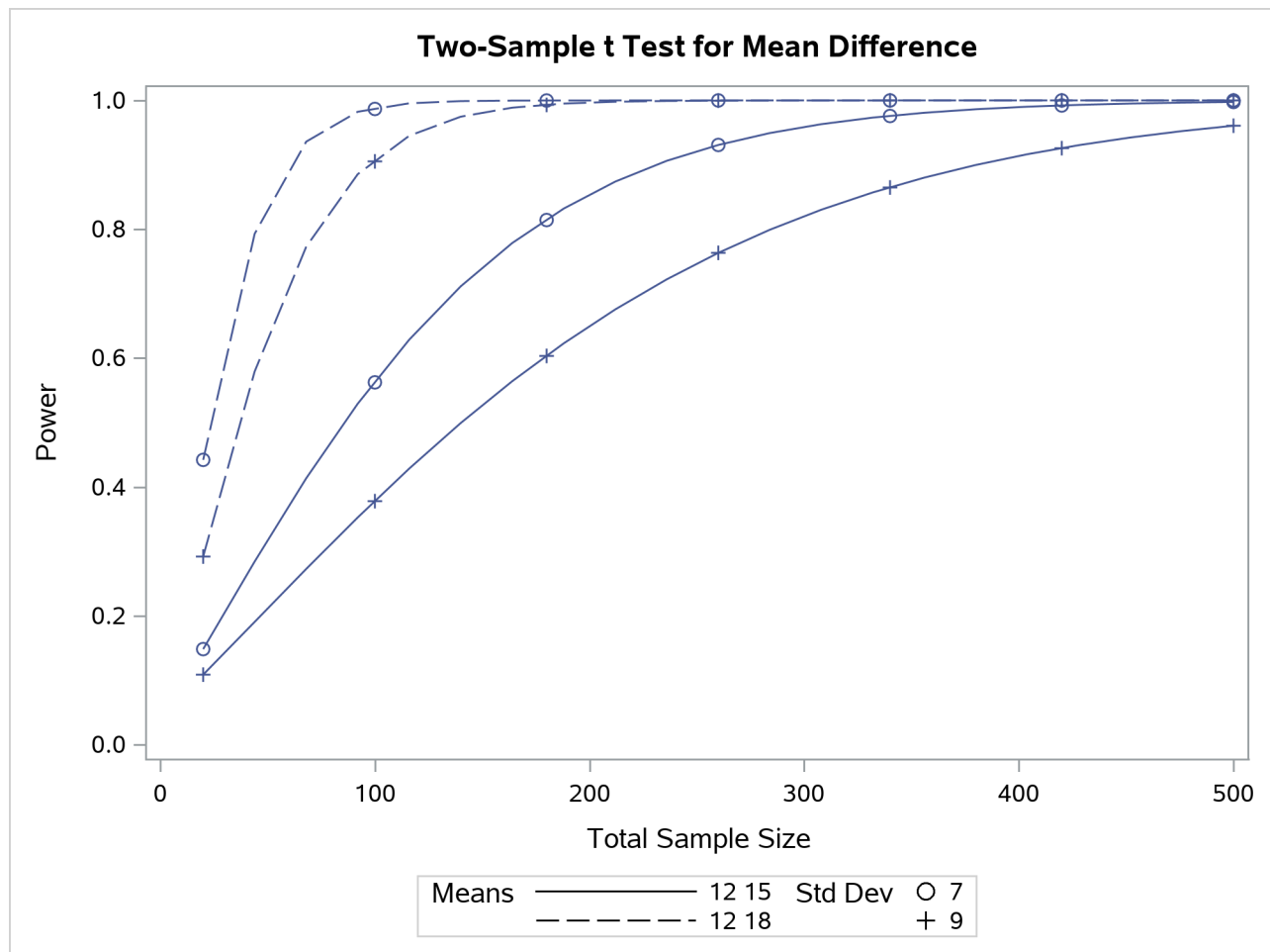
Output 95.8.22 Plot with MARKERS=NICE
