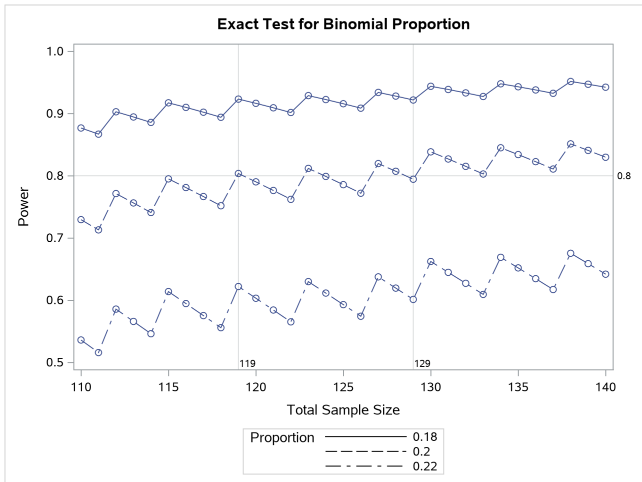
Output 95.2.4 Plot for Assessing Sensitivity to True Proportion Value
