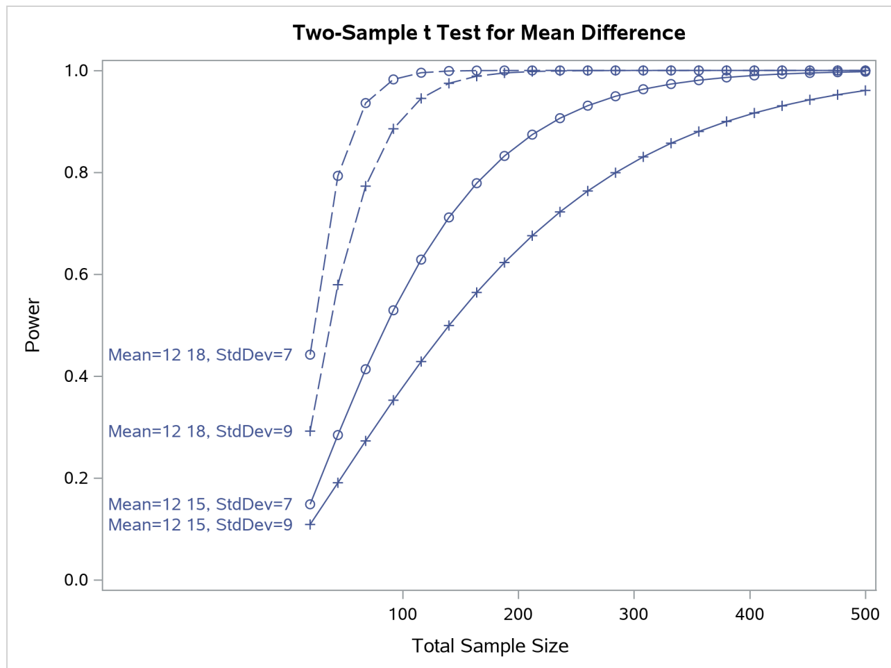
Output 95.8.20 Plot with Directly Labeled Curves
