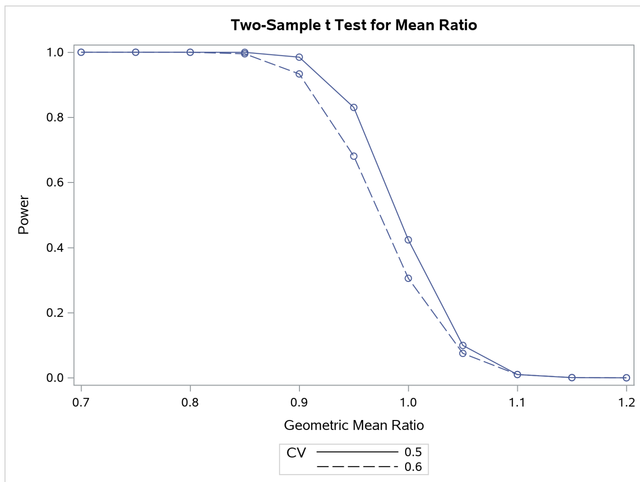
Output 95.4.2 Plot of Power versus Mean Ratio for Noninferiority Test
