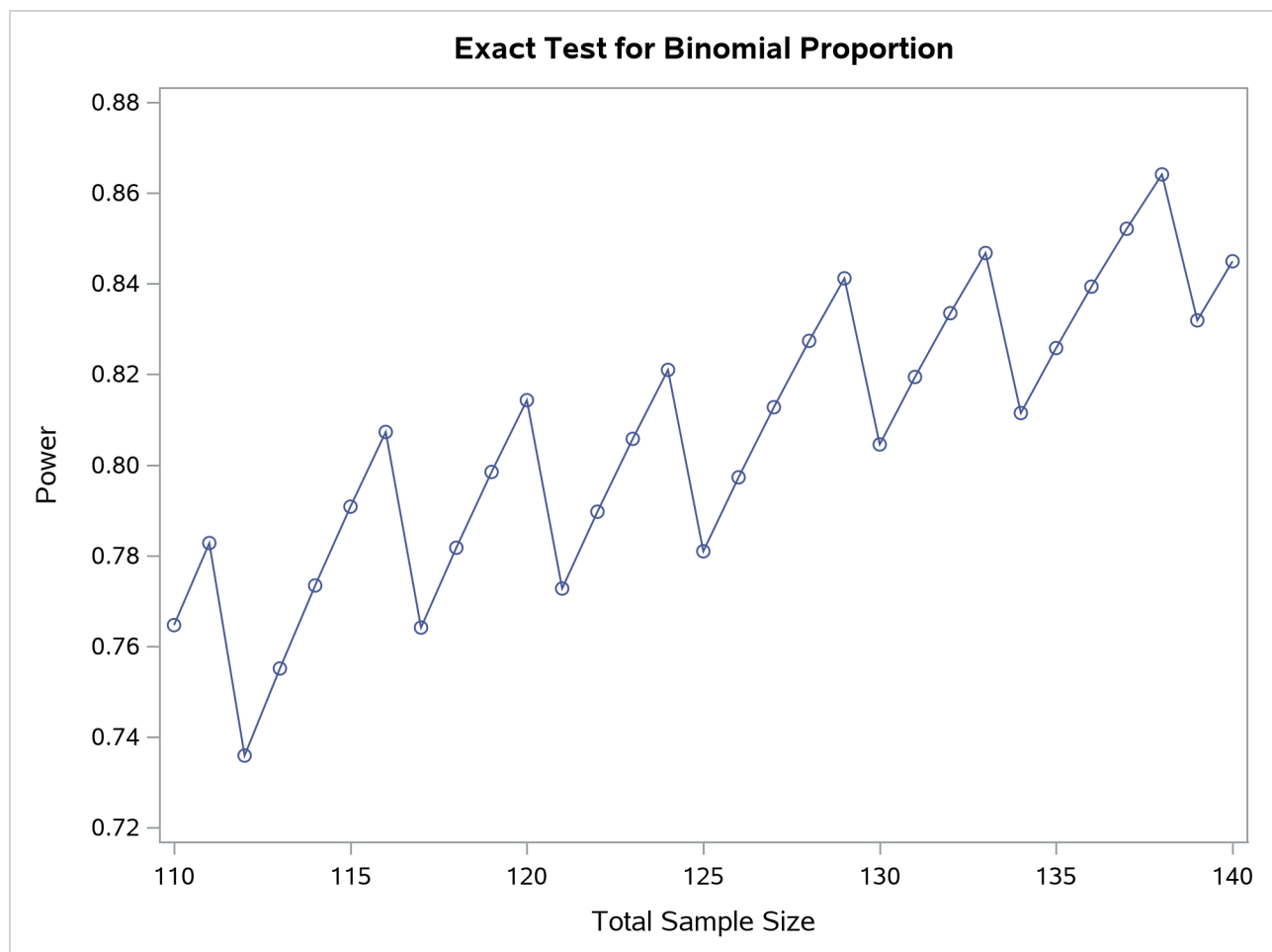
Output 95.2.6 Plot of Power versus Sample Size for Another One-sided Test
