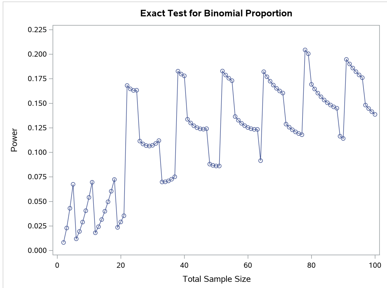
Output 95.2.7 Plot of Power versus Sample Size for a Two-Sided Test
