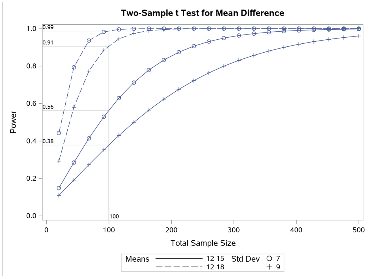
Output 95.8.13 Plot with CROSSREF=YES Style Reference Lines from X Axis
