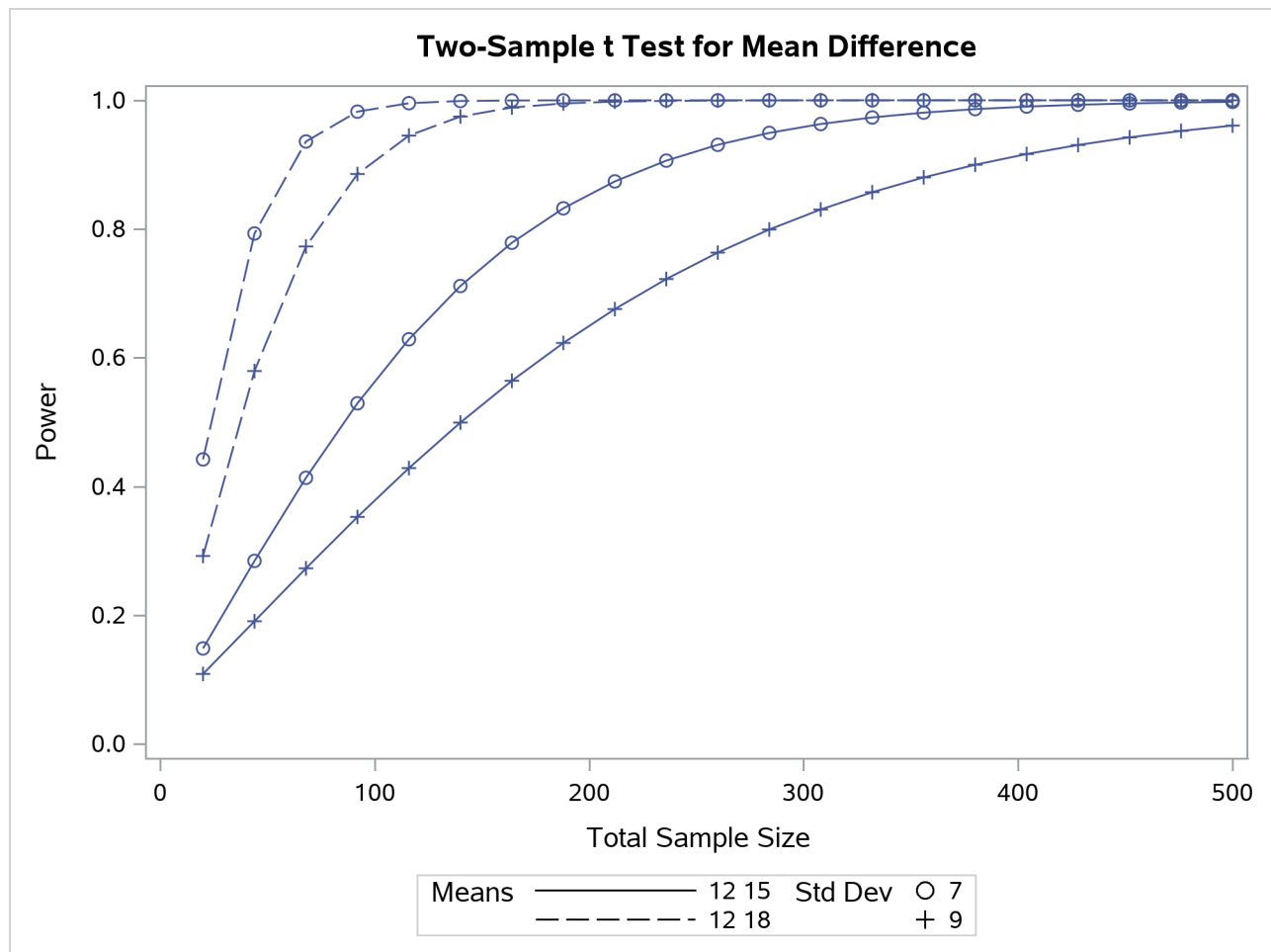
Output 95.8.5 Plot of Power versus Sample Size Using Second Strategy
