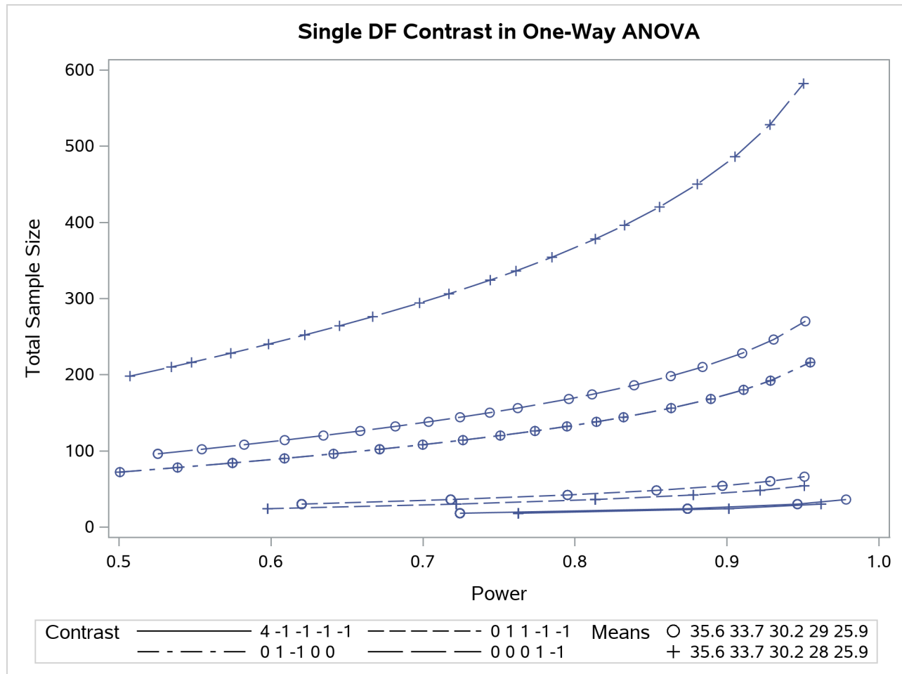
Output 95.1.2 Plot of Sample Size versus Power for One-Way ANOVA Contrasts
