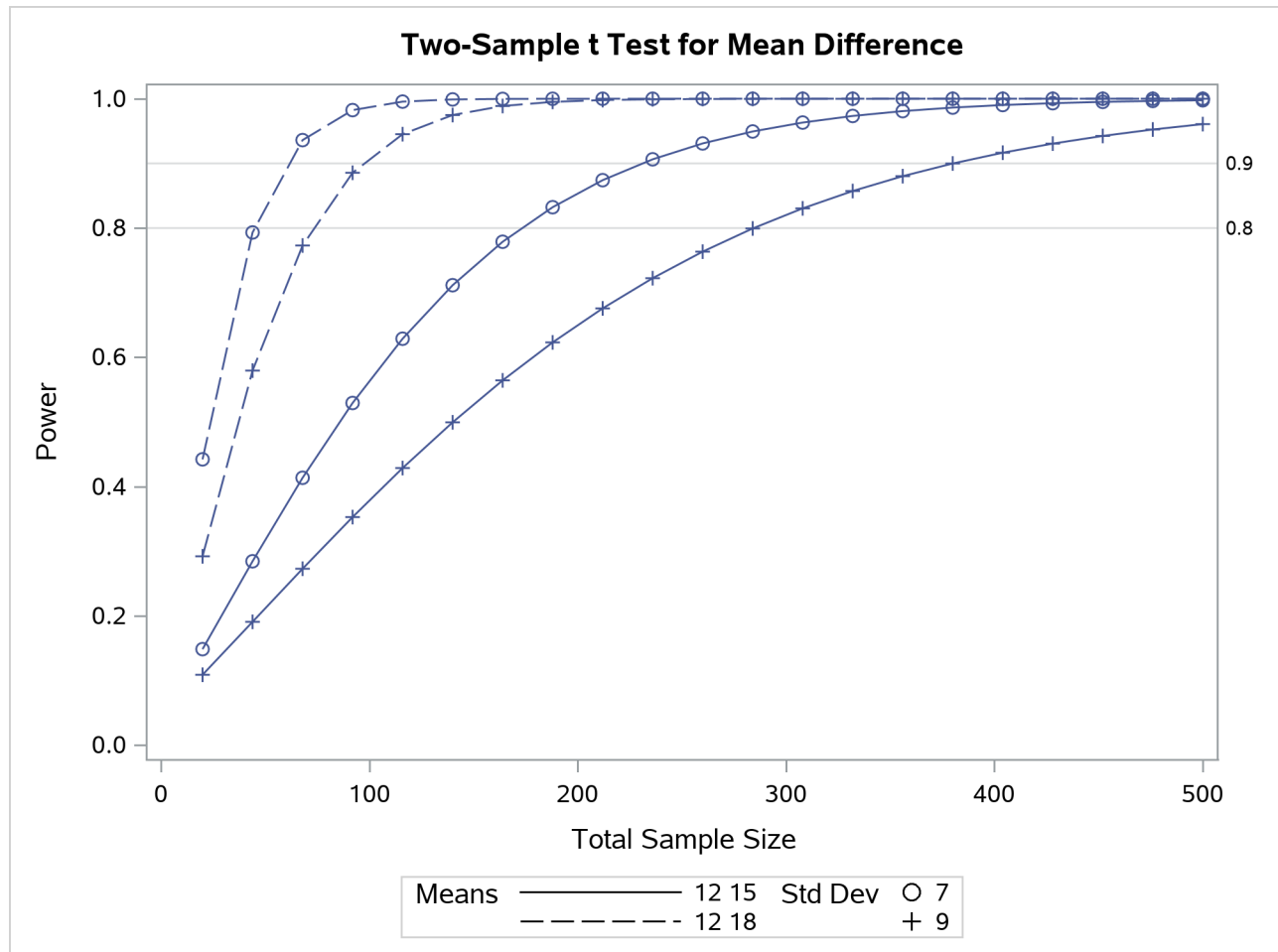
Output 95.8.11 Plot with Simple Reference Lines on Y Axis
