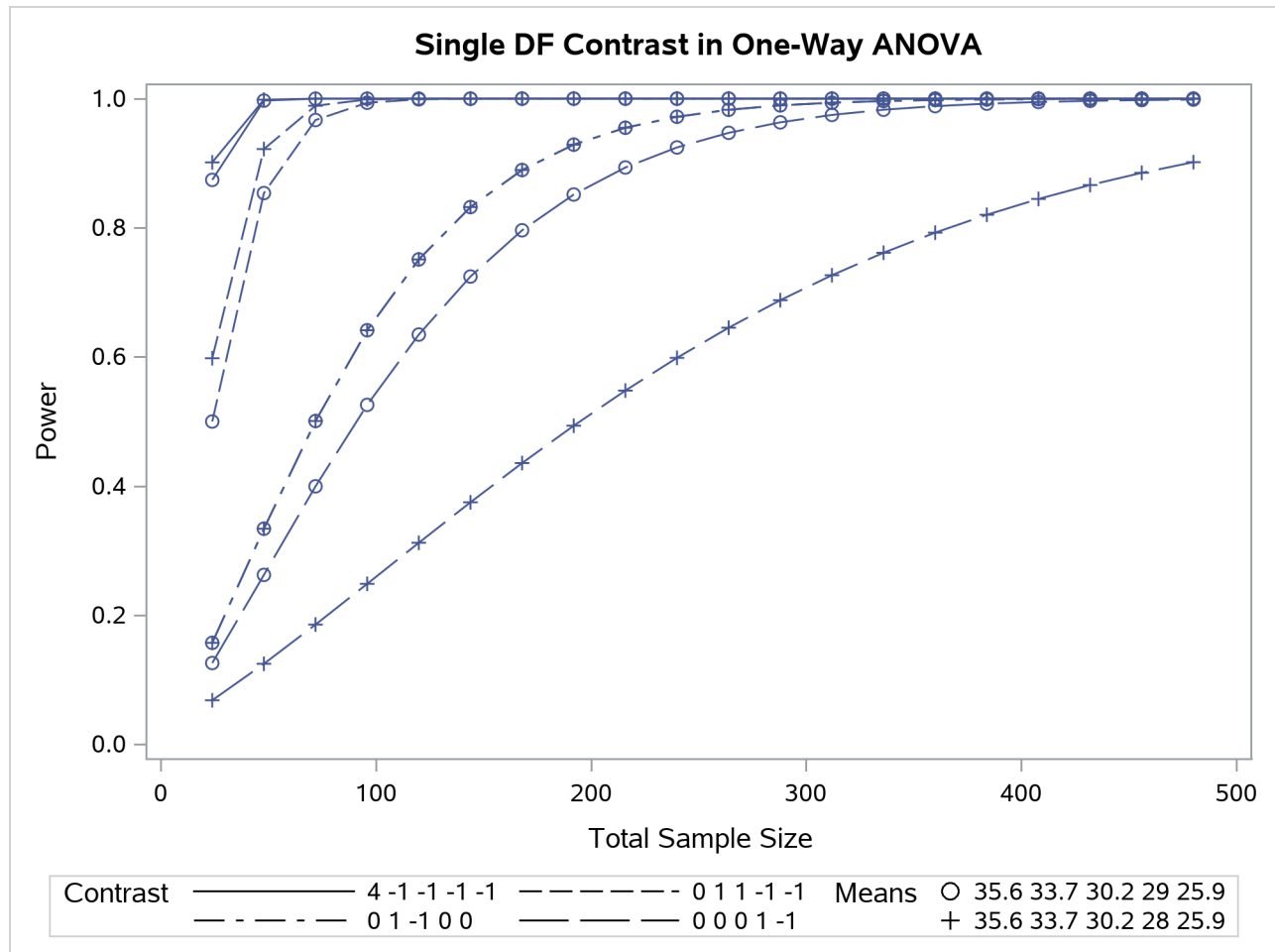
Output 95.1.3 Plot of Power versus Sample Size for One-Way ANOVA Contrasts
