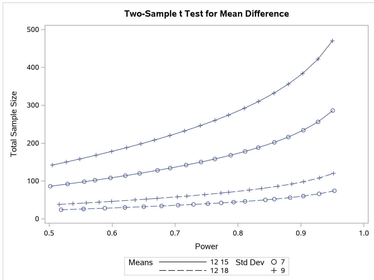
Output 95.8.2 Plot of Sample Size versus Power
