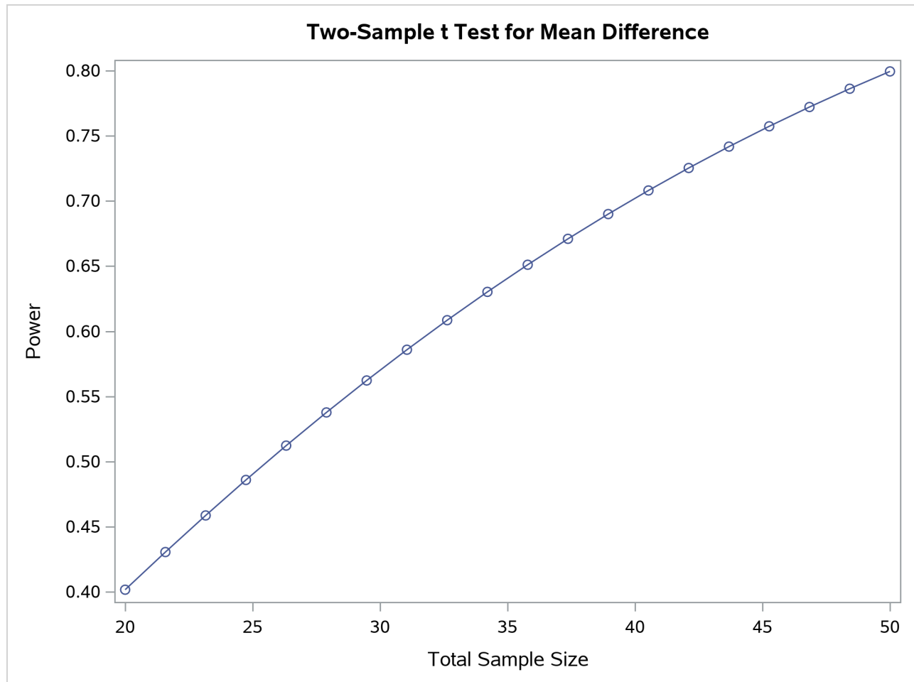
Output 95.8.10 Plot with Fractional Sample Sizes
