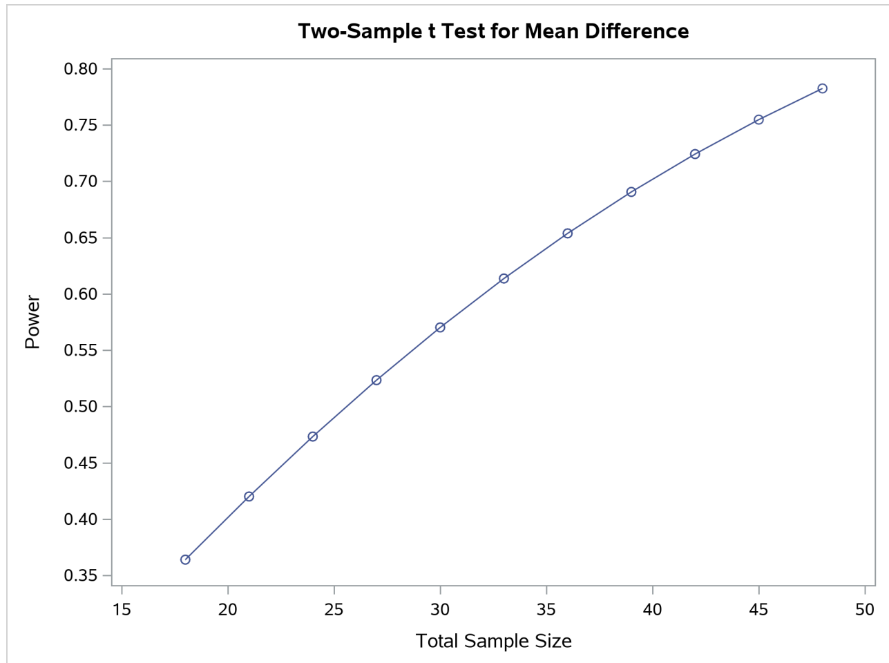
Output 95.8.7 Plot with Overlapping Points
