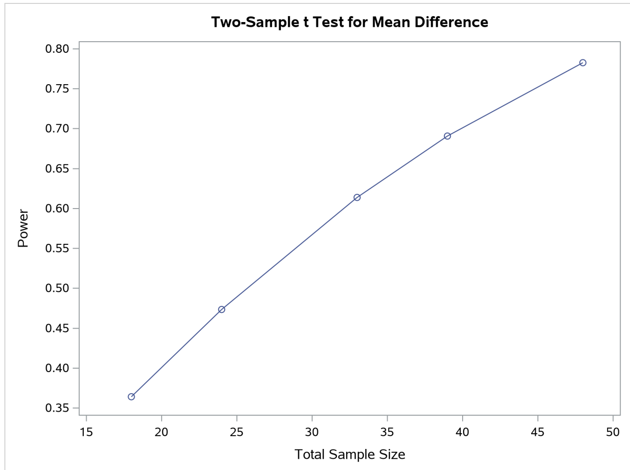
Output 95.8.9 Plot with Unequally Spaced Points
