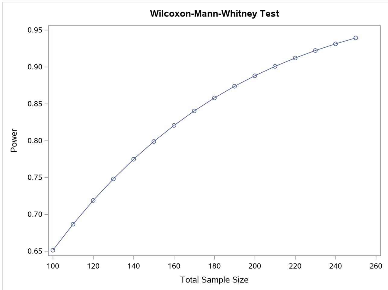
Output 95.10.2 Plot of Power versus Sample Size for Wilcoxon Power Analysis
