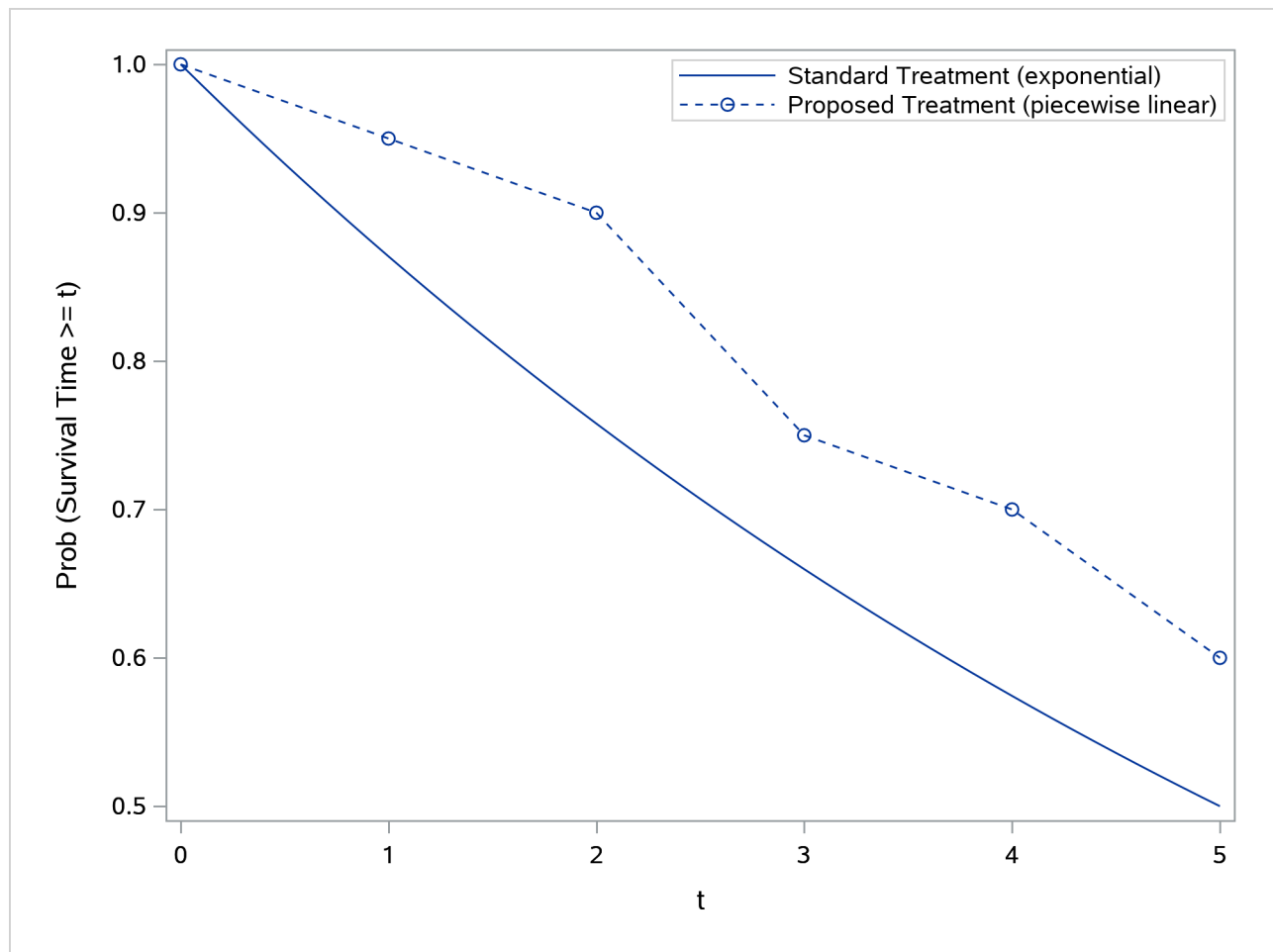
Output 95.6.1 Survival Curves
