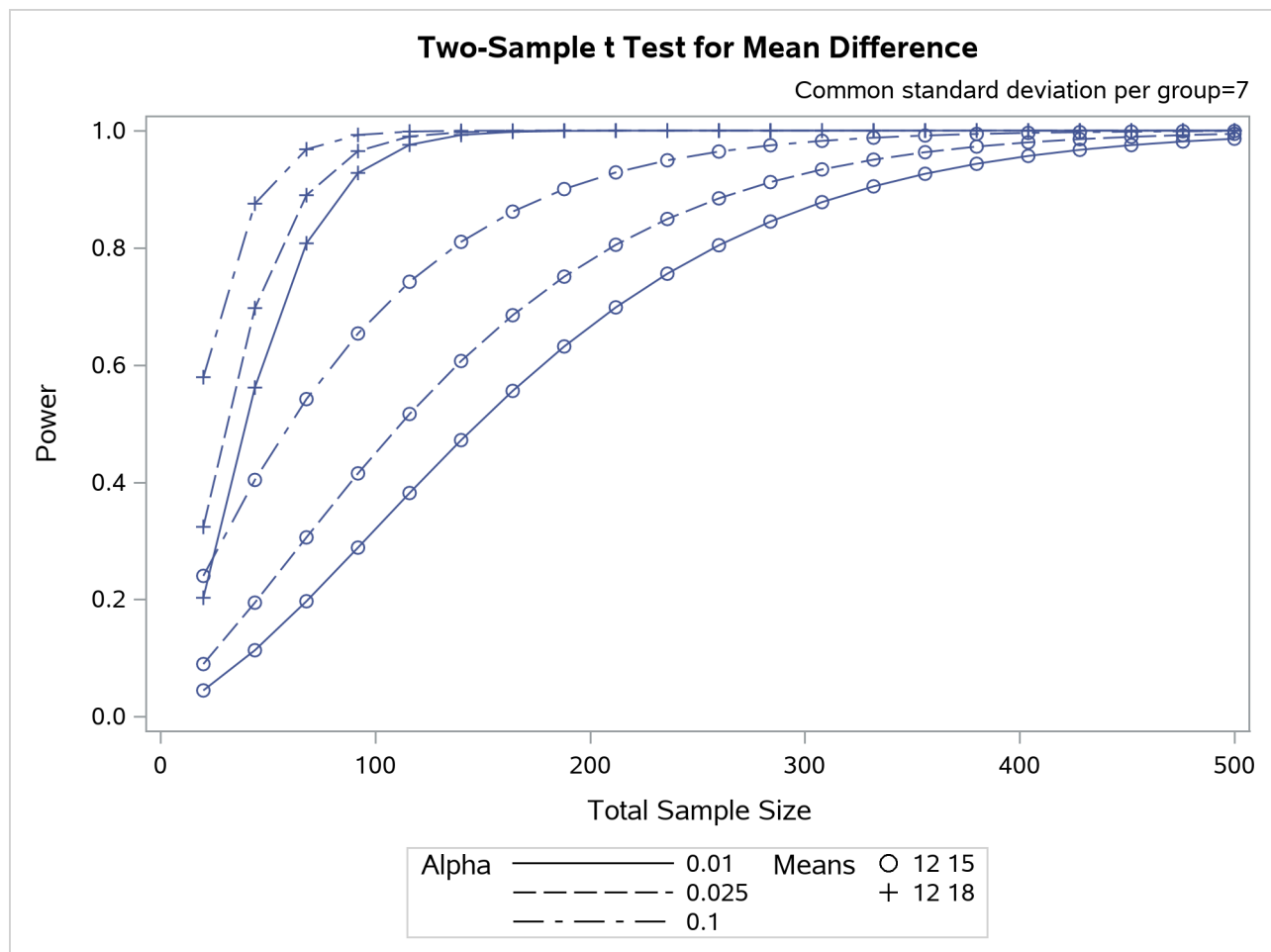
Output 95.8.14 Plot with Default VARY Settings
