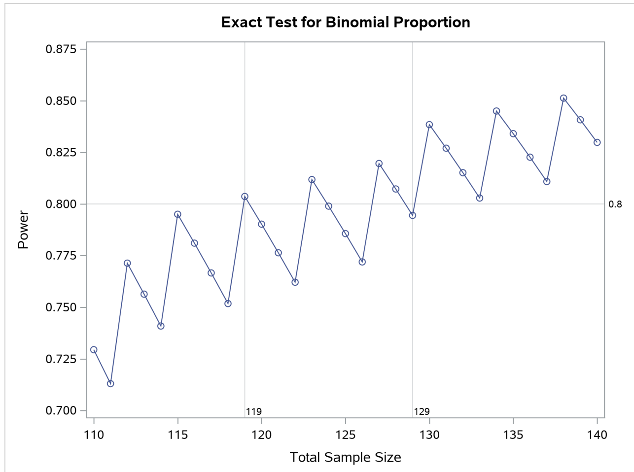
Output 95.2.3 Plot of Power versus Sample Size for Exact Binomial Test
