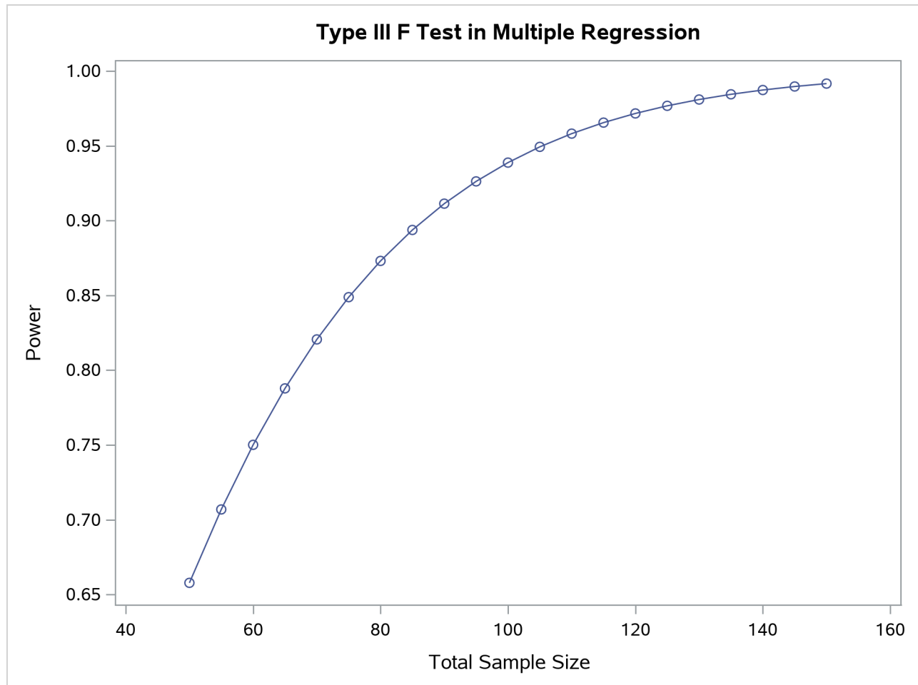
Output 95.5.2 Plot of Power versus Sample Size for Multiple Regression
