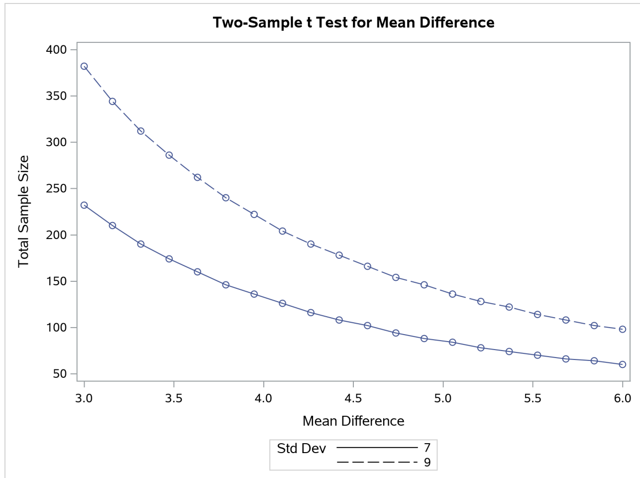
Output 95.8.6 Plot of Sample Size versus Mean Difference
