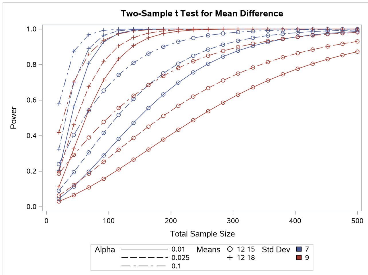
Output 95.8.15 Plot with Varying Color Instead of Panel
