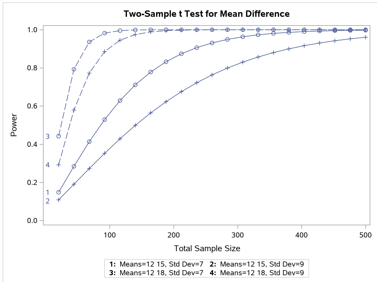
Output 95.8.18 Plot with a Numbered By-Curve Key
