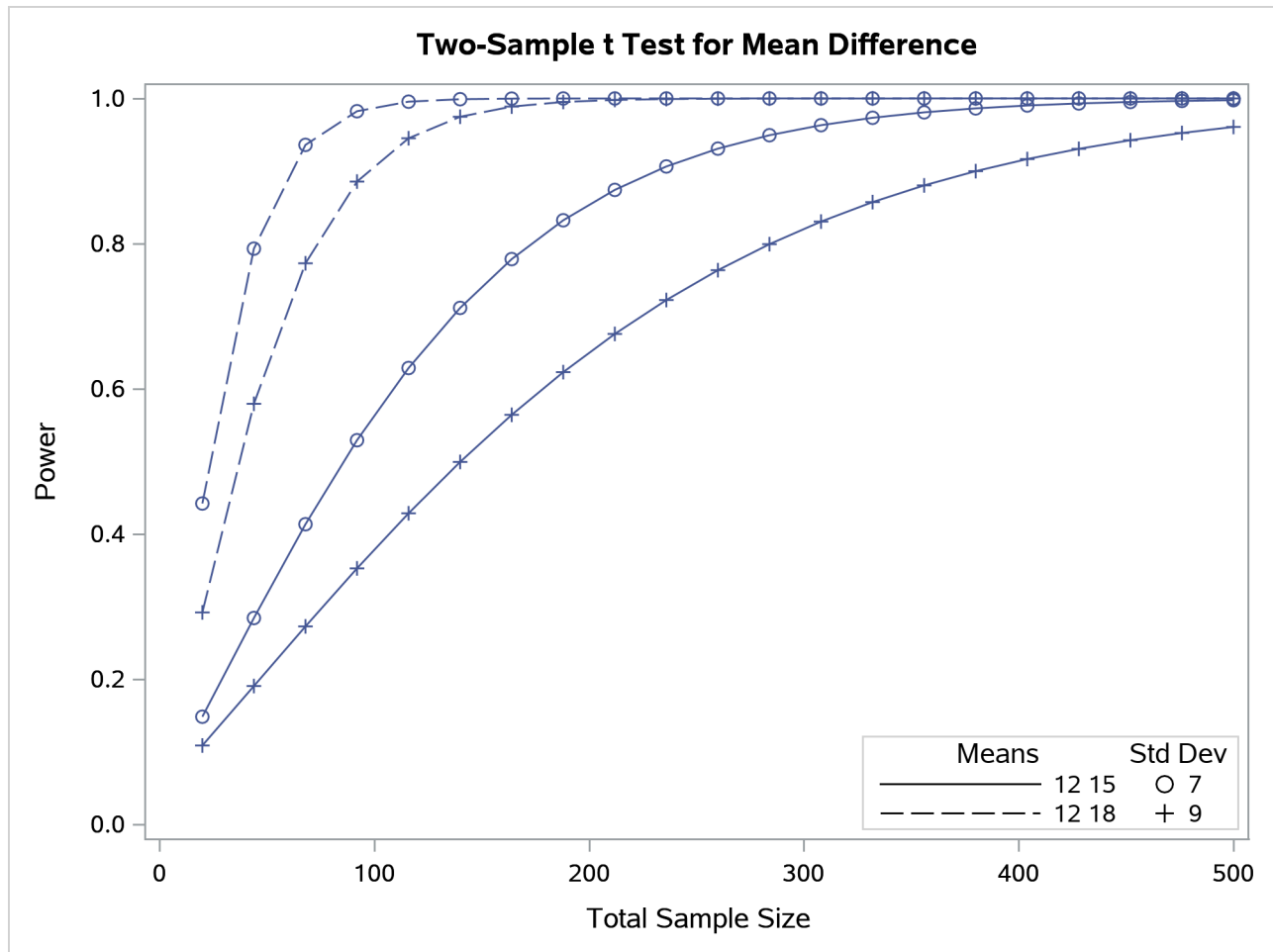
Output 95.8.17 Plot with a By-Feature Key inside the Plotting Region
