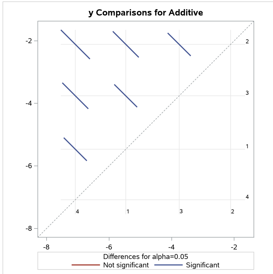
Output 93.3.2 LS-Means Plot of Pairwise Differences
