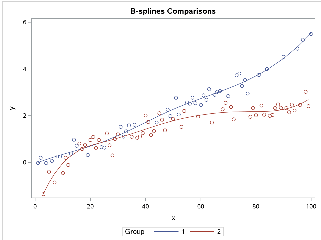
Output 93.6.2 Observed Data and Predicted Values by Group
