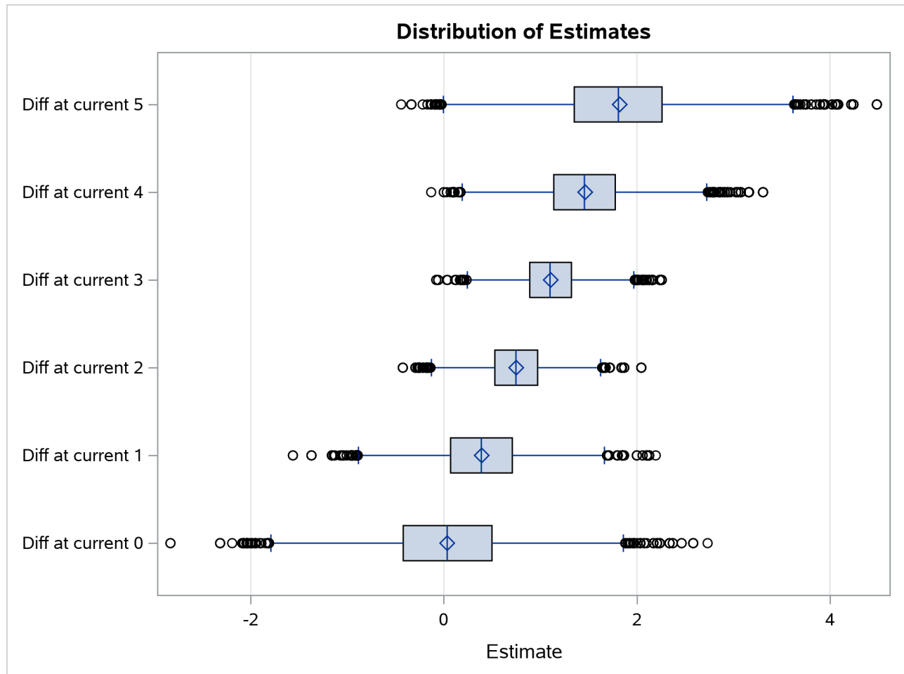
Output 93.4.3 Box Plot of Difference between Two Experiments
