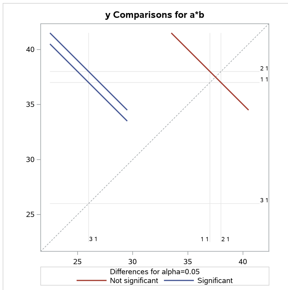
Figure 93.6 LS-Means Difference Diffogram
