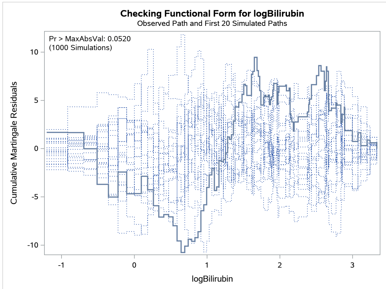
Output 91.12.6 Cumulative Martingale Residuals versus log(Bilirubin)
