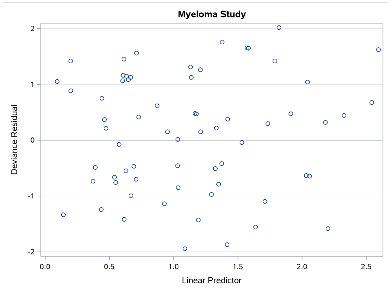
Output 91.9.2 Deviance Residual Plot
