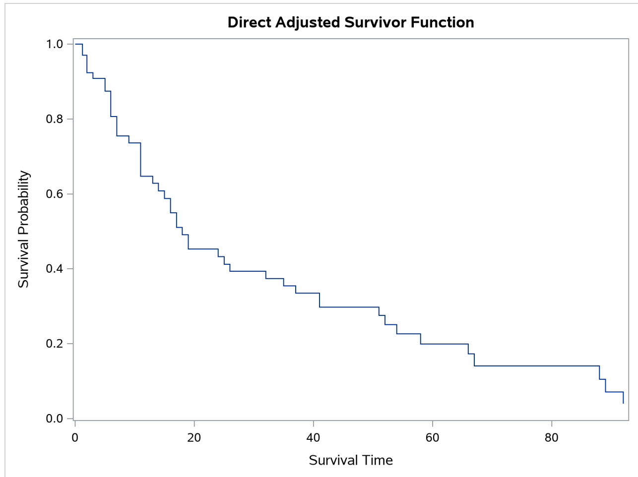
Output 91.8.3 Average Survival Function for the Myeloma Data
