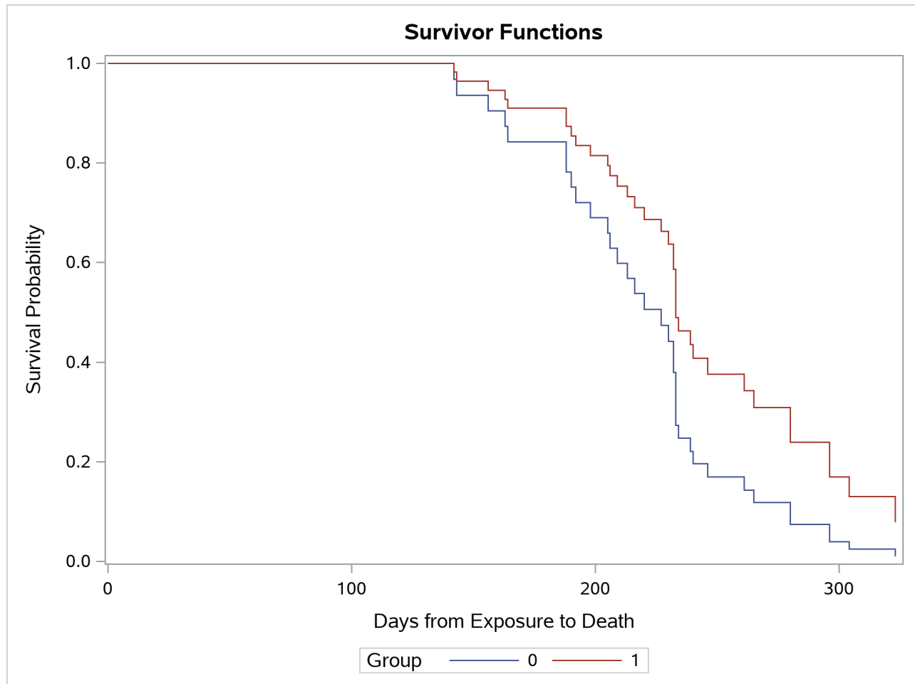
Figure 91.2 Survivorship for the Two Pretreatment Regimes
