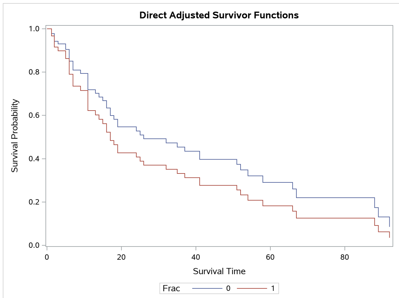
Output 91.8.4 Average Survival by Fracture Status
