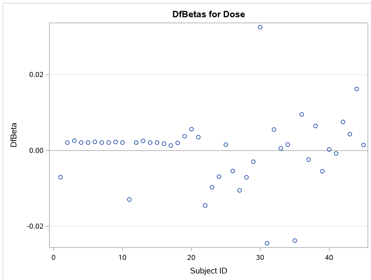
Output 91.7.2 Plot of DFBETA Statistic for DOSE versus Subject Number
