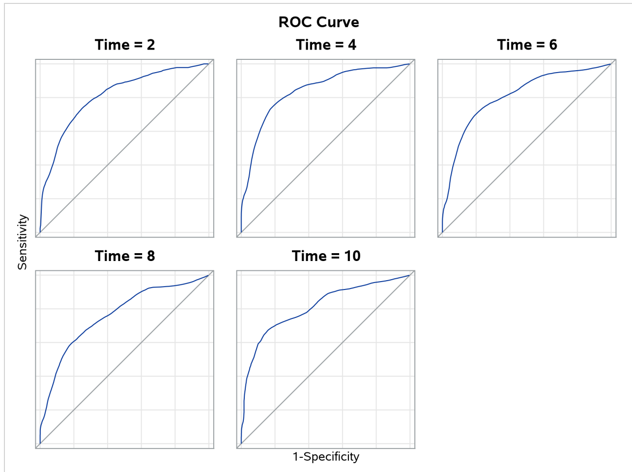
Output 91.16.2 ROC Plot at Selected Time Points
