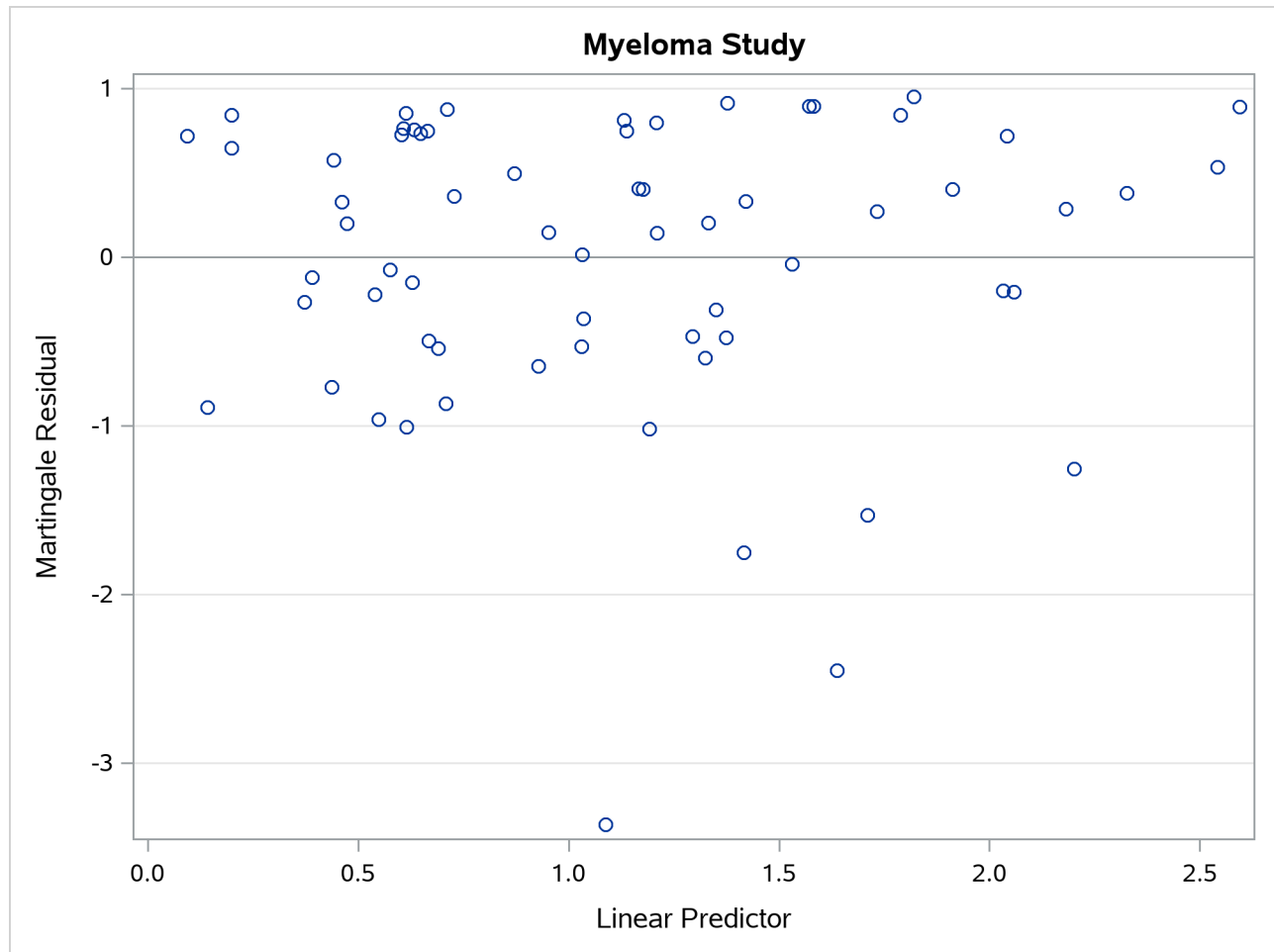
Output 91.9.1 Martingale Residual Plot
