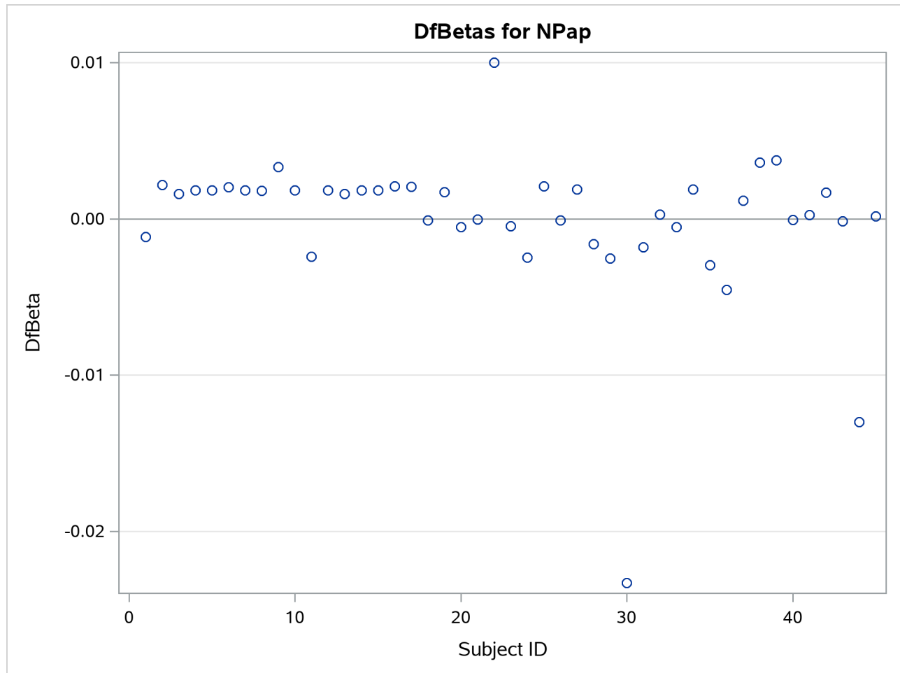
Output 91.7.3 Plot of DFBETA Statistic for NPAP versus Subject Number
