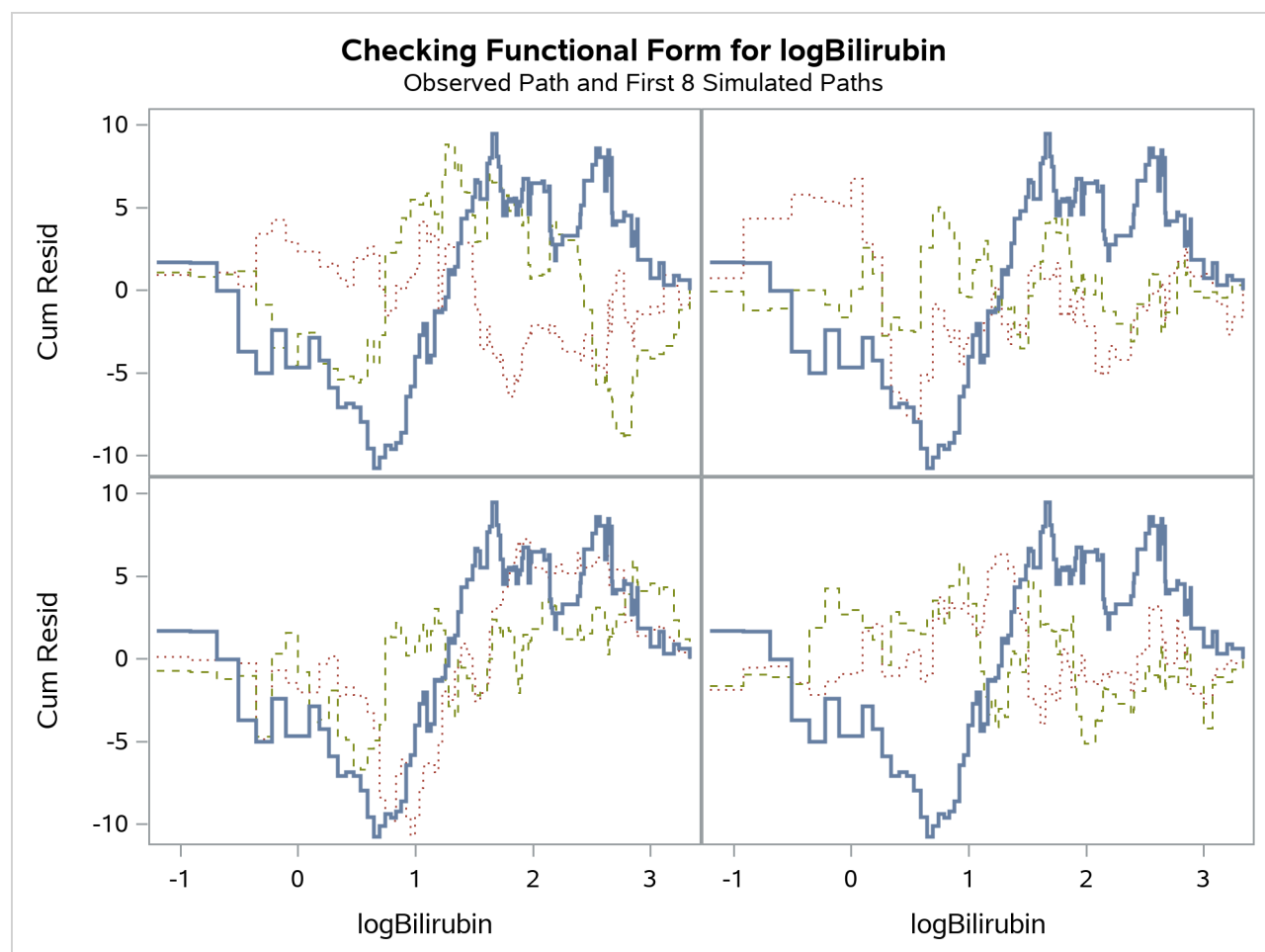
Output 91.12.5 Panel Plot of Cumulative Martingale Residuals versus log(Bilirubin)
