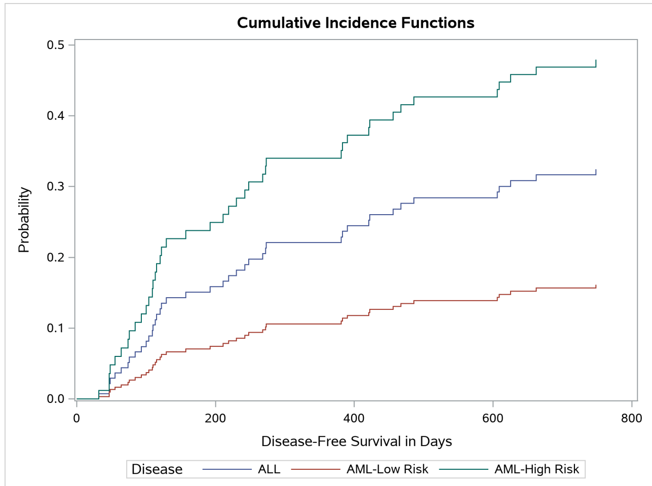
Output 91.15.5 CIFs of the Three Disease Groups
