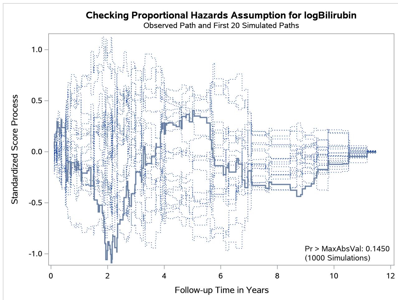
Output 91.12.7 Standardized Score Process for log(Bilirubin)
