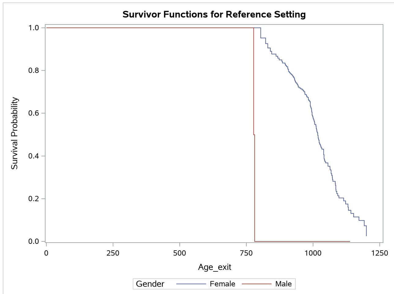
Figure 91.18 Product-Limit Estimates for Women and Men
