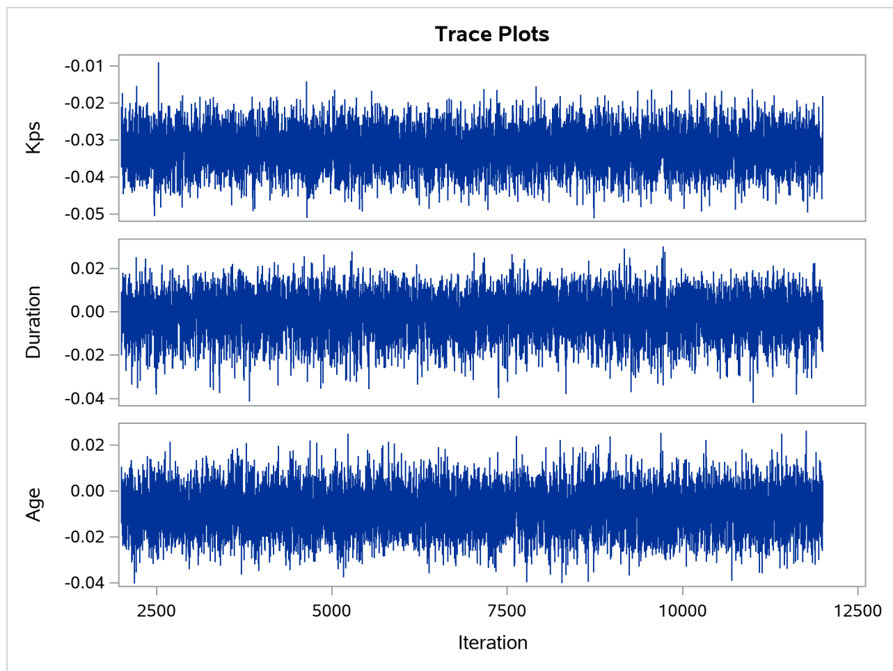
Output 91.13.10 Trace Plots
