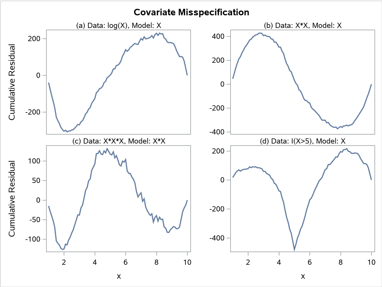
Output 91.12.3 Typical Cumulative Residual Plot Patterns
