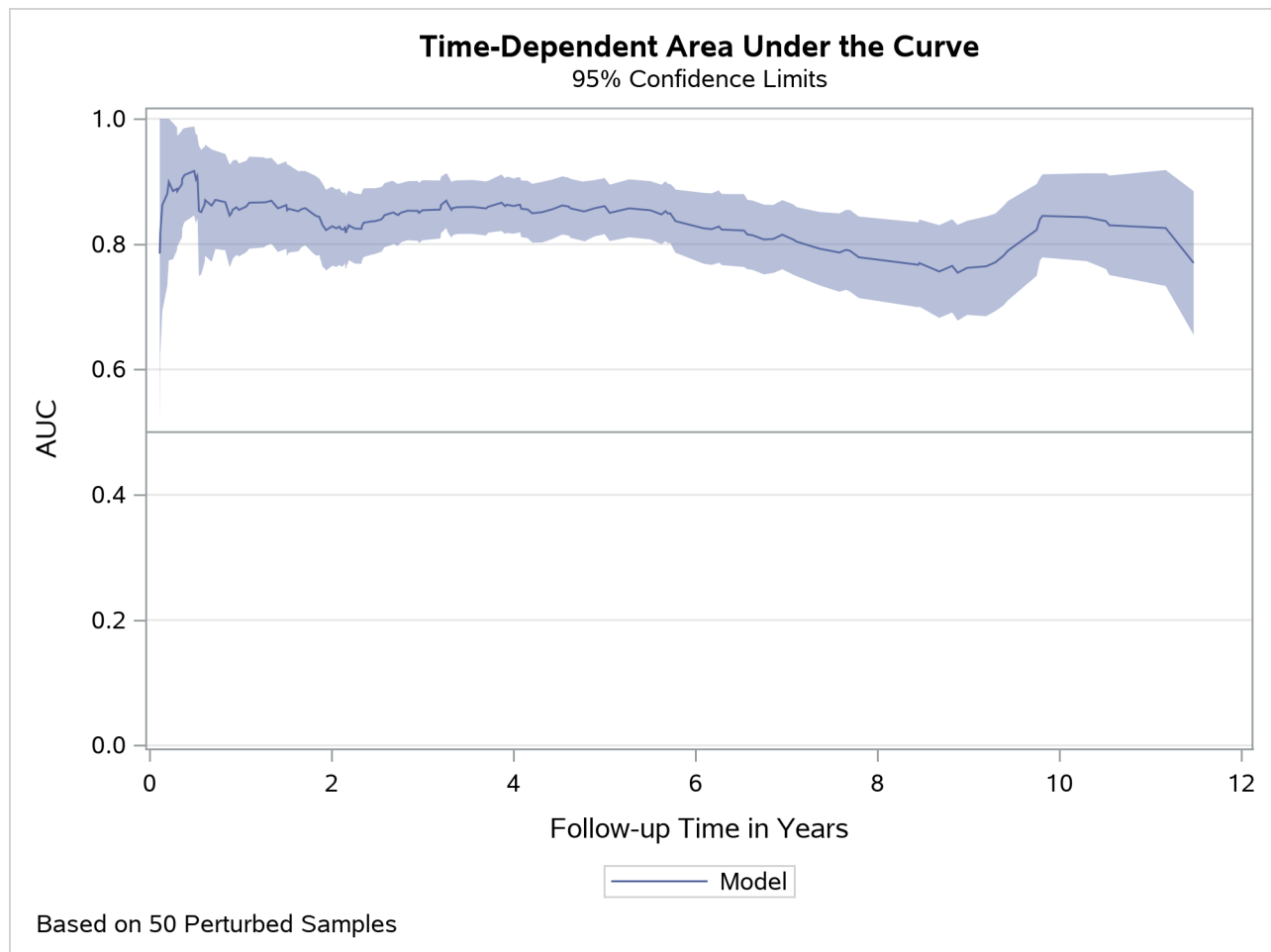
Output 91.16.3 AUC Plot with 95% Confidence Limits
