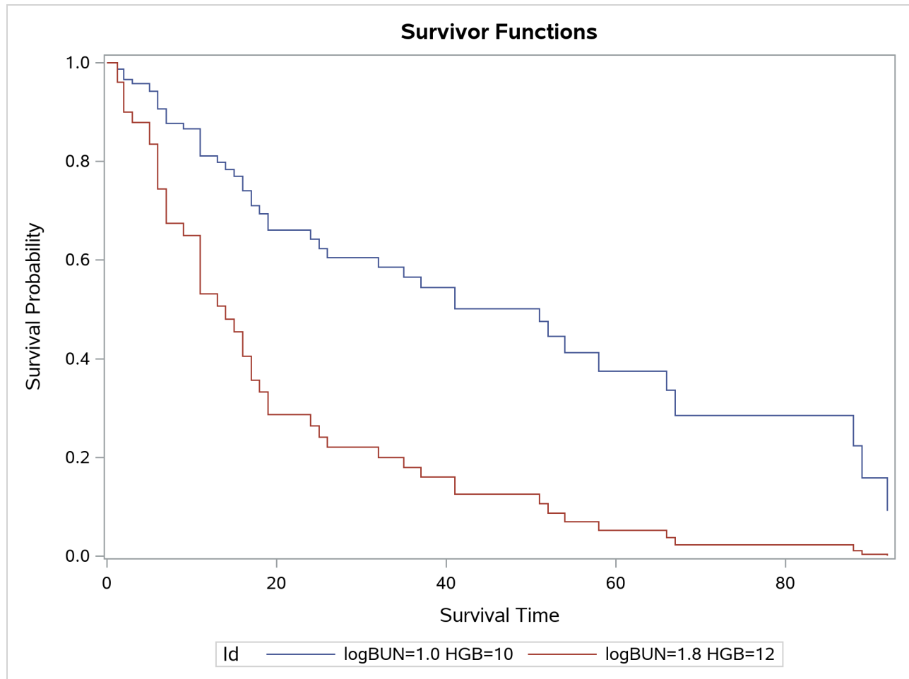
Output 91.8.1 Estimated Survivor Function Plot
