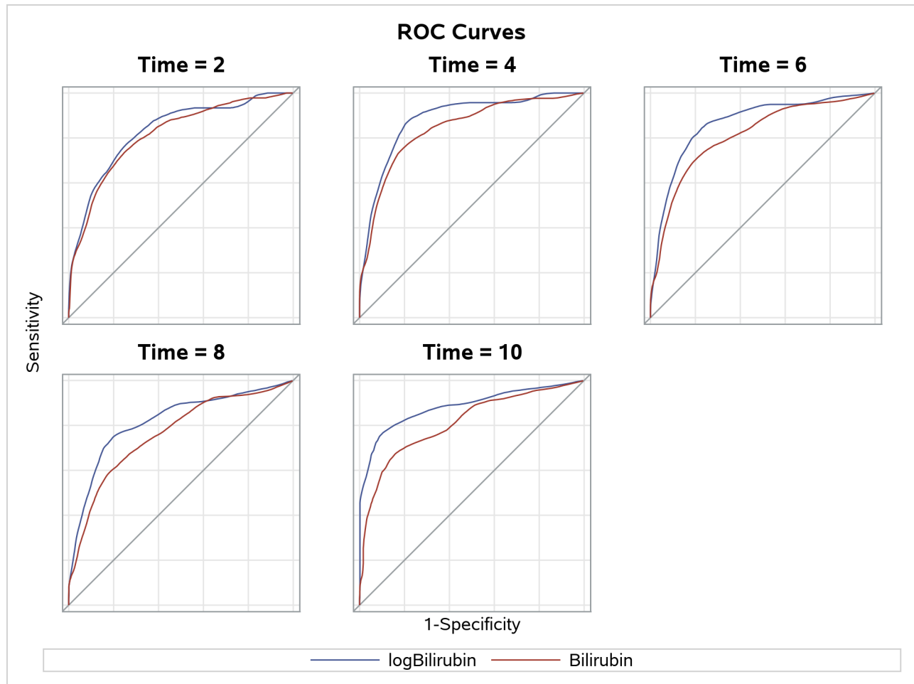
Output 91.16.5 ROC Plots to Evaluate the Log Transform for Bilirubin
