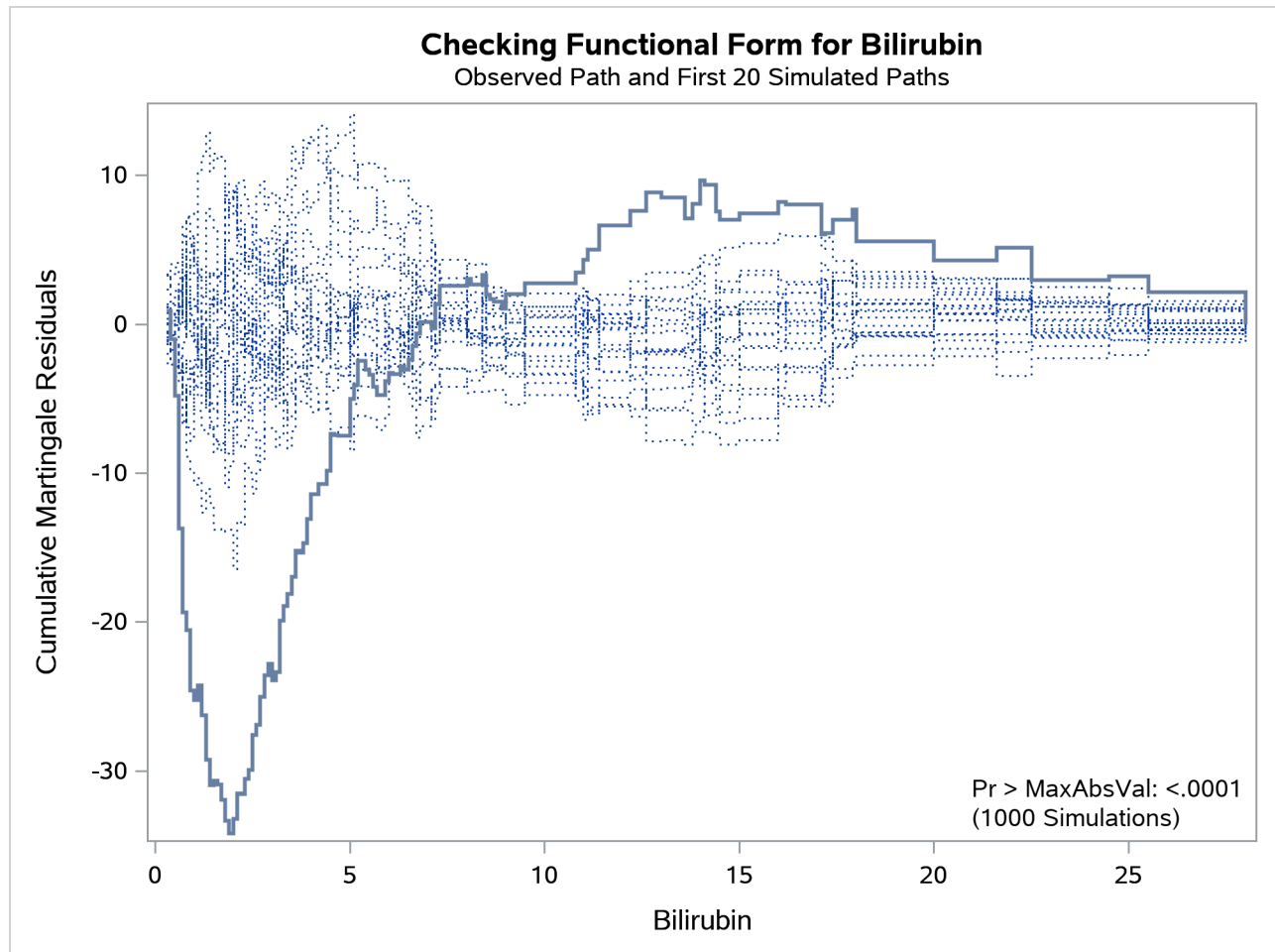
Output 91.12.2 Cumulative Martingale Residuals vs Bilirubin
