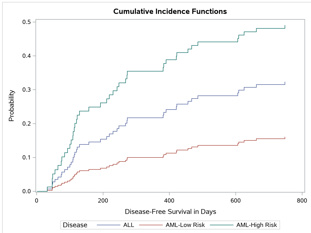
Output 91.15.9 CIFs of the Three Disease Groups (Cause-Specific Analysis) for the All Group
