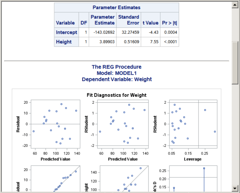
Figure 23.27 Statistical Output with the SAPPHIRE Style and HTML Destination
