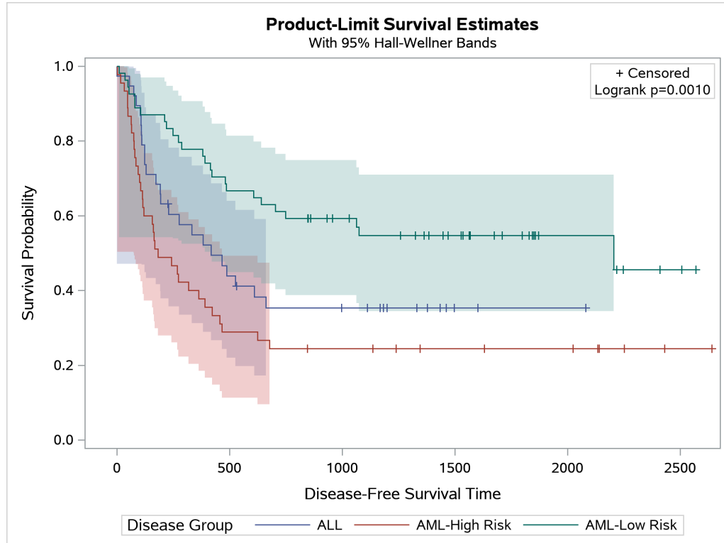
Figure 23.4 Survival Plot
