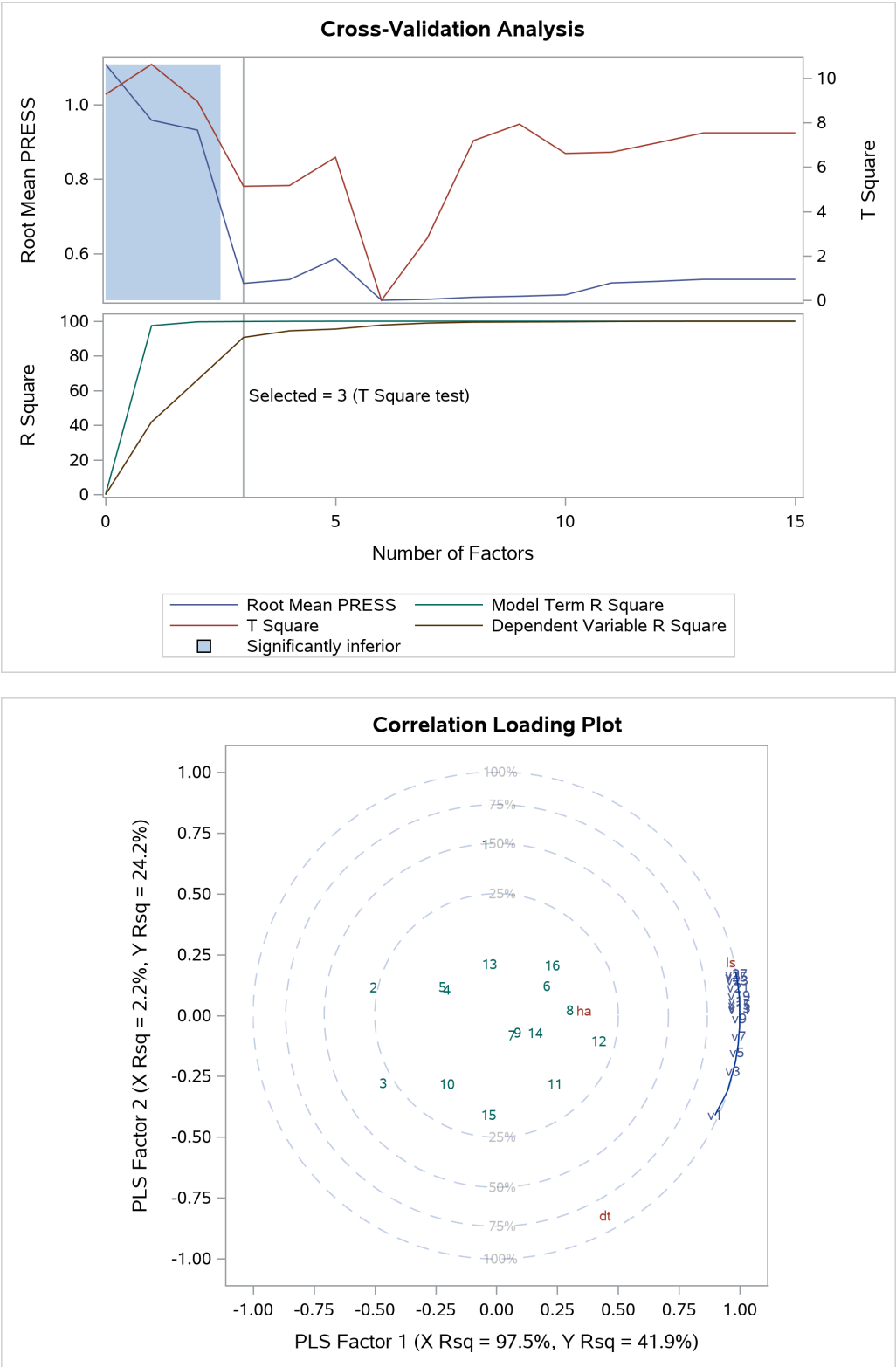
Figure 23.8 Partial Least Squares
