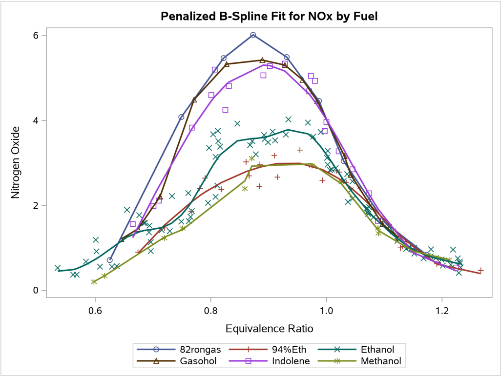
Figure 23.65 Fit Plot with the Modified Style
