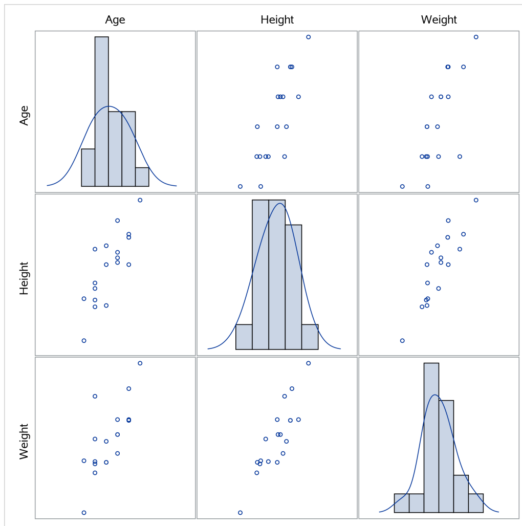
Figure 23.73 Scatter Plot Matrix with PROC SGSCATTER
