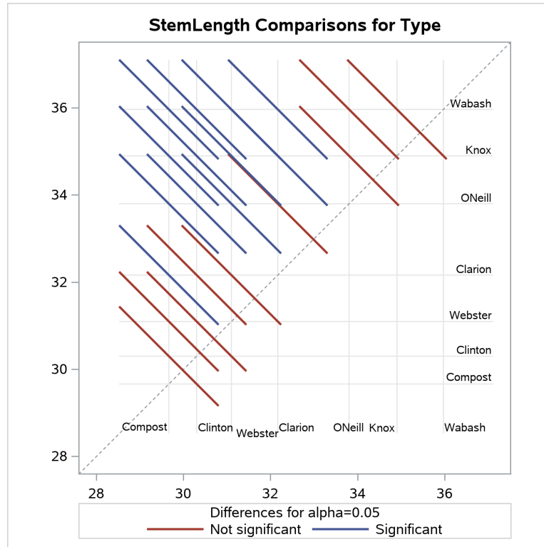
Figure 23.10 LS-Means Diffogram
