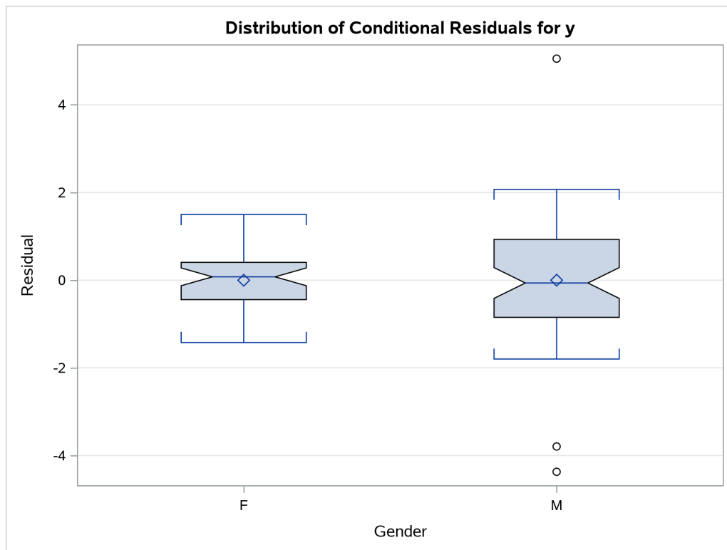
Output 23.5.2 Box Plot with the Richer Style
