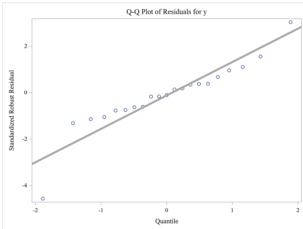
Figure 23.70 Q-Q Plot That Uses the NEWSTYLE Style with a Thicker Line
