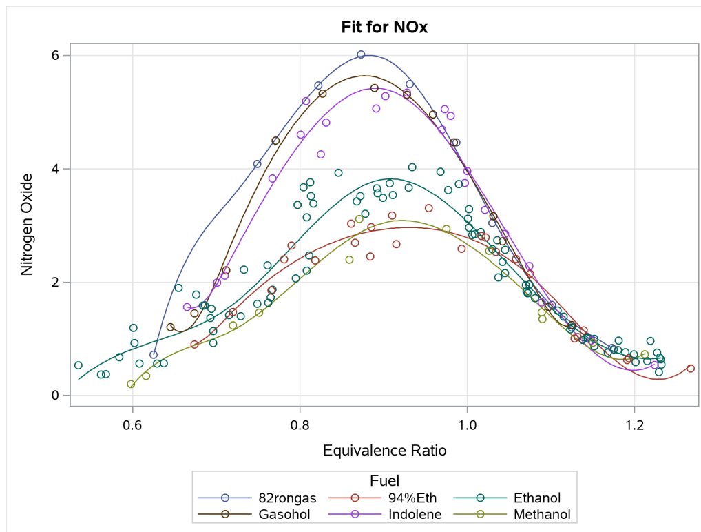
Output 23.6.23 EFFECT and EFFECTPLOT Statements with a CLASS Variable
