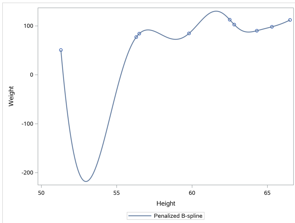
Output 23.6.6 Overfit Sparse Data
