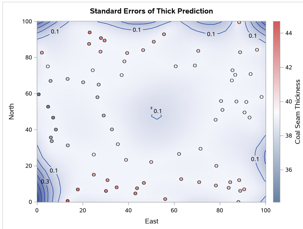
Figure 23.7 continued
