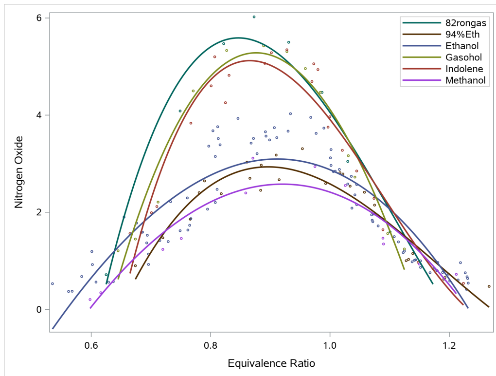
Output 23.6.9 Grouped Cubic Polynomial Fit Plot
