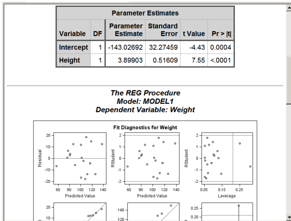
Figure 23.24 Statistical Output with the LISTING Style and HTML Destination
