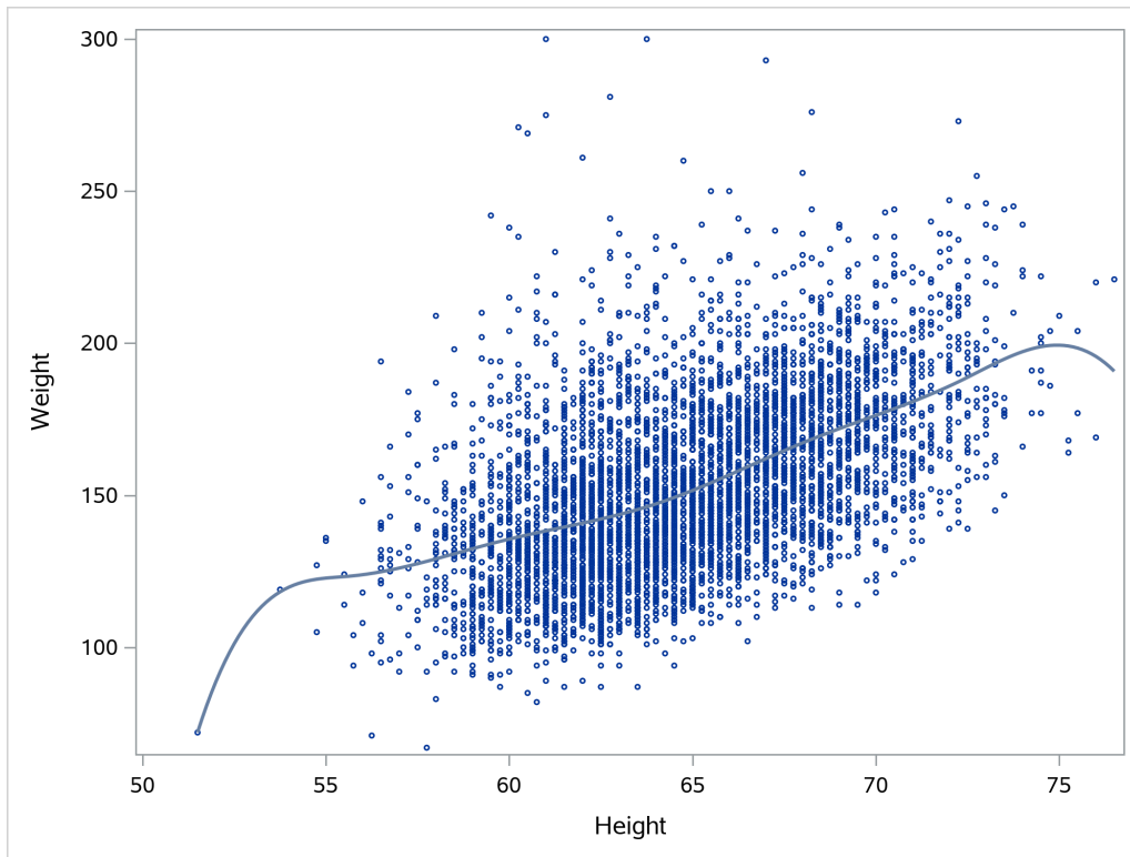
Output 23.6.4 B-Spline Fit Plot
