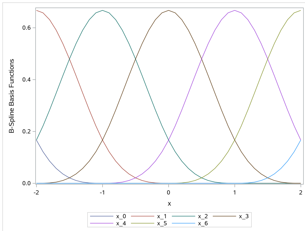
Output 23.6.26 B-Spline Basis
