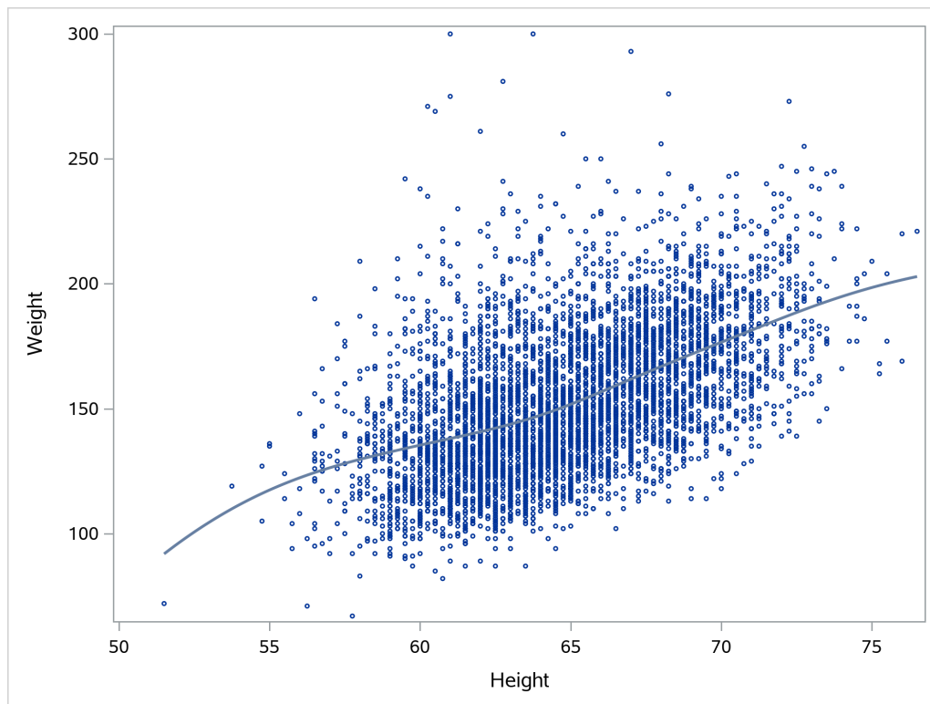
Output 23.6.2 Penalized B-Spline Fit Plot
