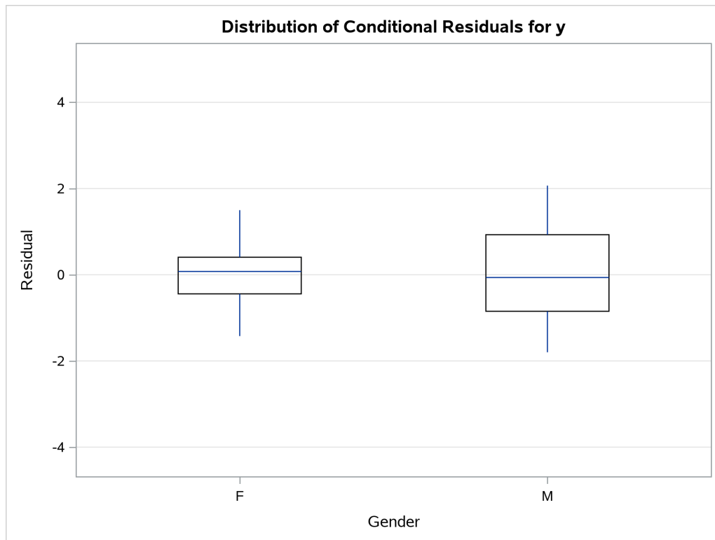
Output 23.5.1 Box Plot with the Sparse Style
