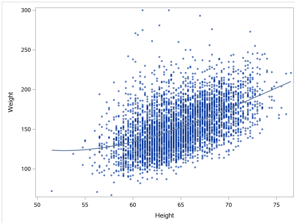
Output 23.6.1 Cubic Polynomial Fit Plot
