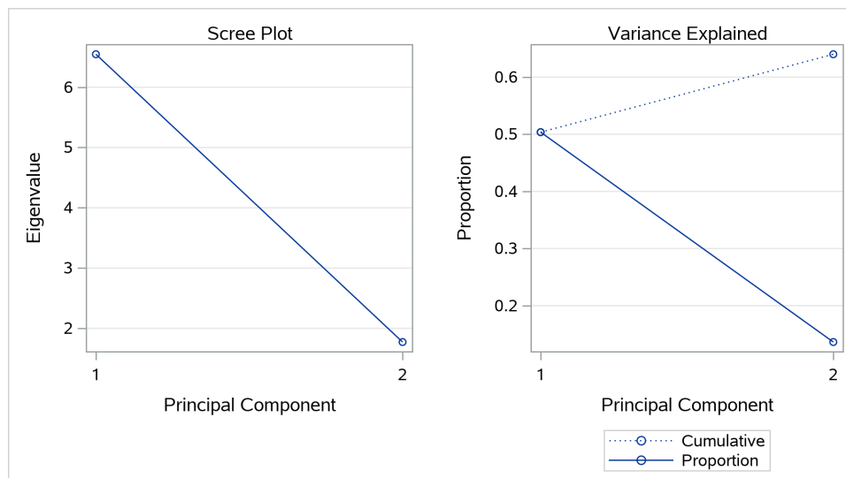
Figure 23.11 Principal Component Analysis
