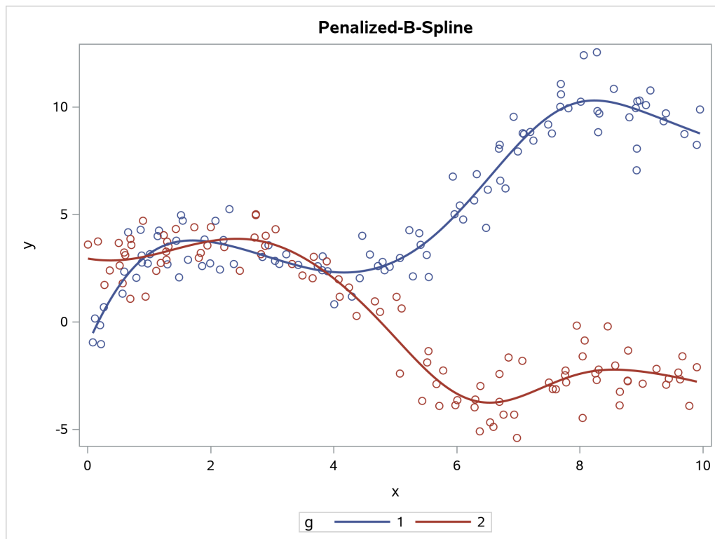
Output 23.6.19 Penalized B-Splines and Monotone Splines
