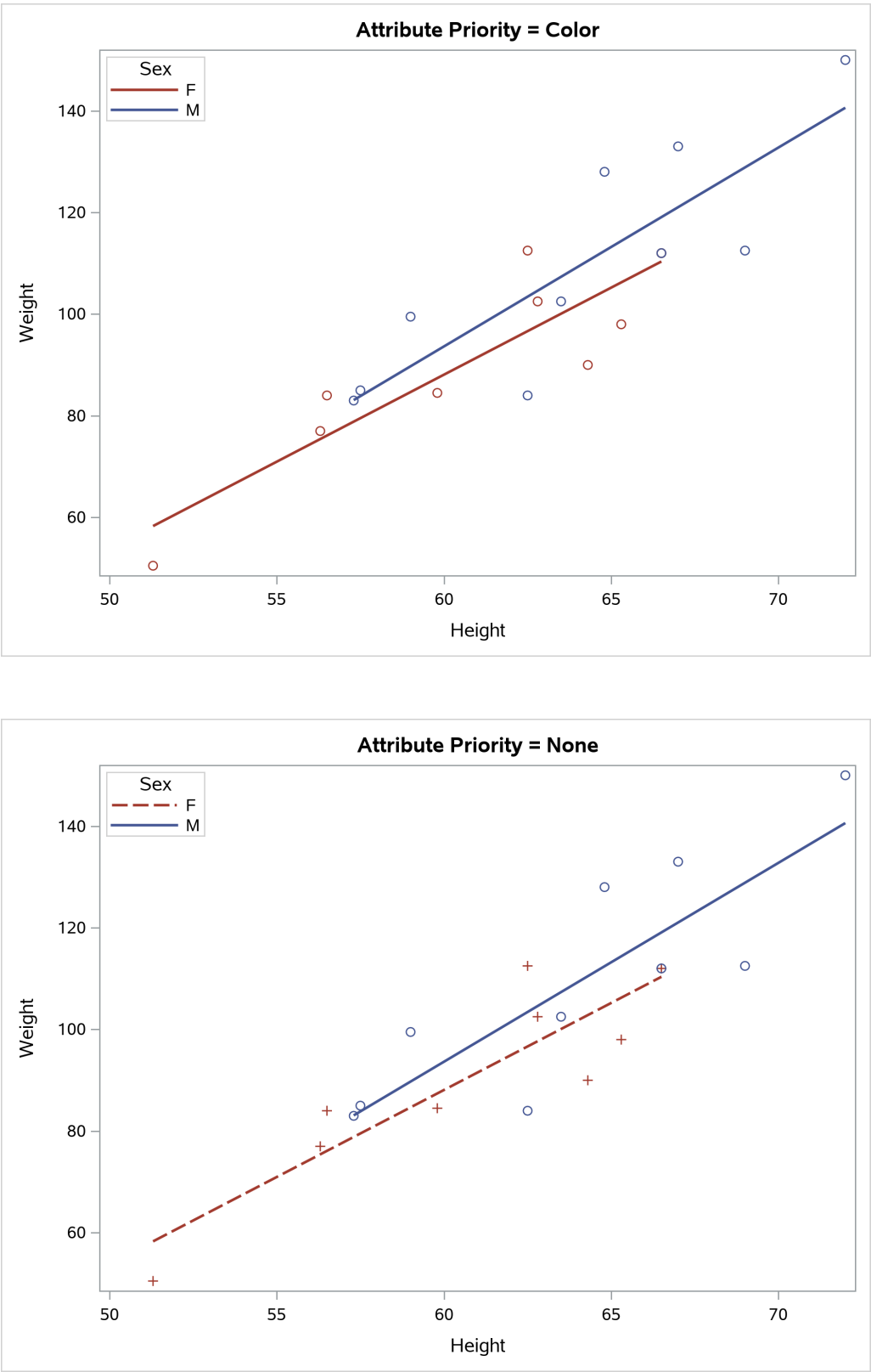
Figure 23.15 Attribute Priority
