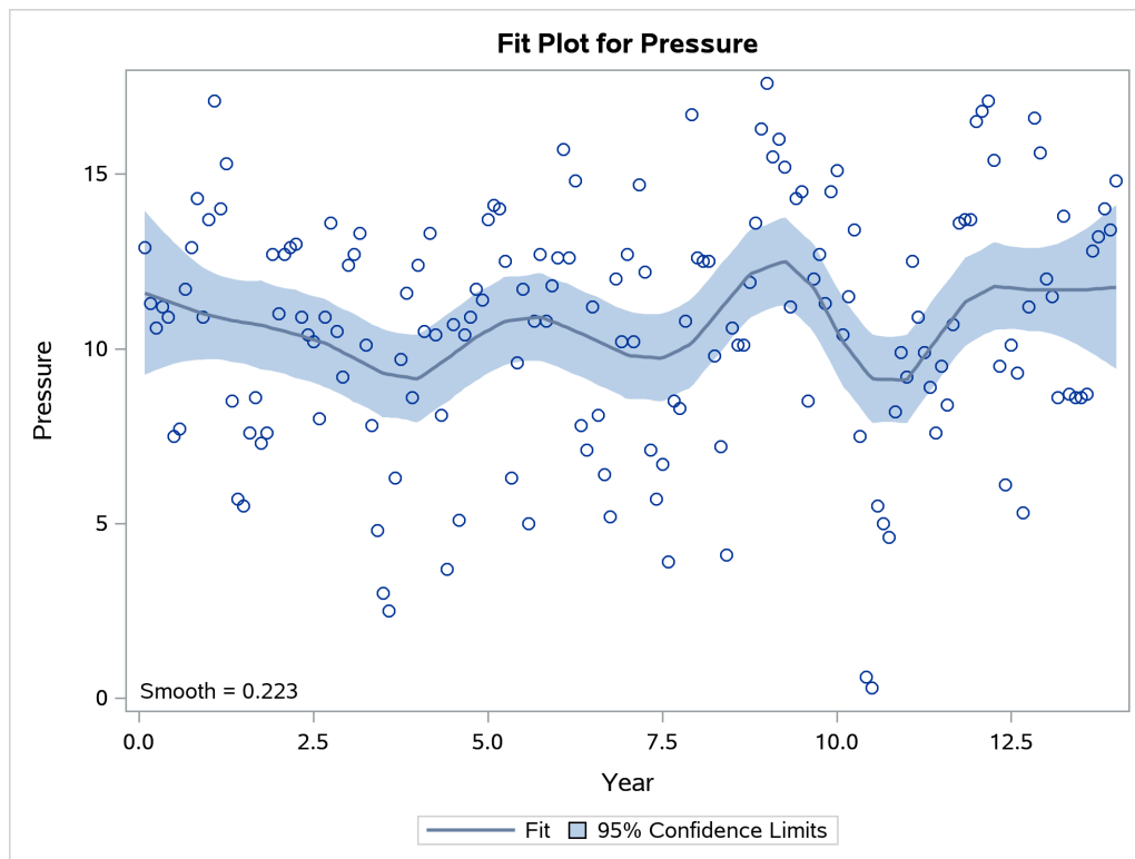
Output 23.2.1 Loess Fit Plot with the HTMLBLUE Style
