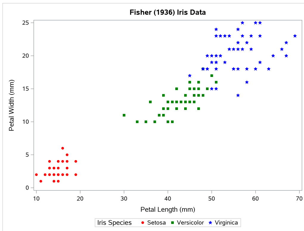
Figure 23.16 Iris Data
