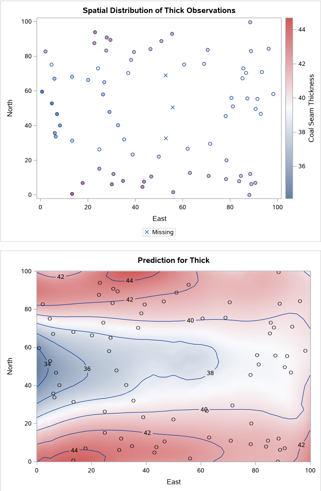
Figure 23.7 Spatial Distribution
