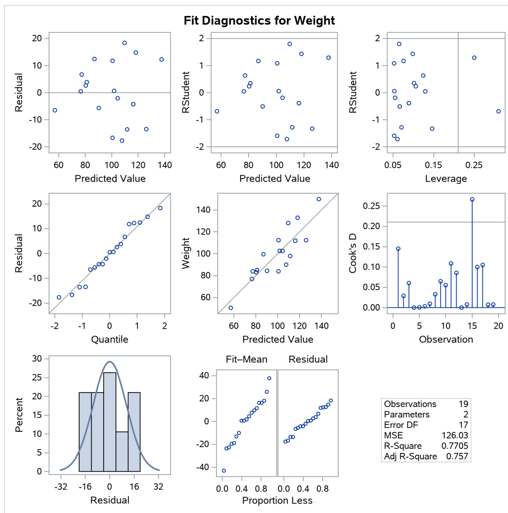
Figure 23.1 Fit Diagnostics Panel
