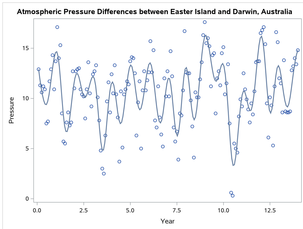
Figure 23.72 Penalized B-Spline Fit with PROC SGPLOT
