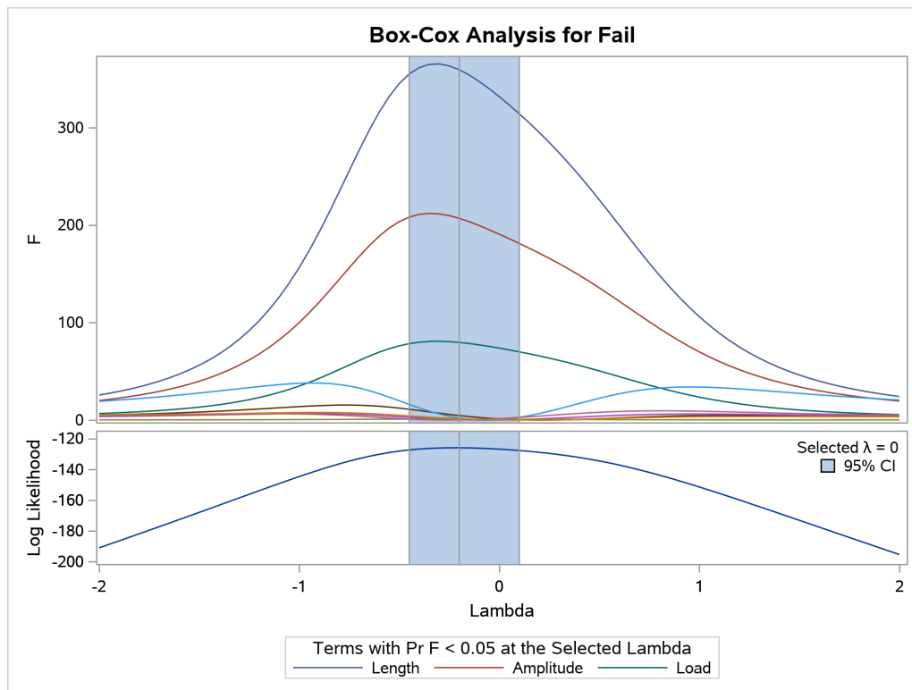
Figure 23.9 Box-Cox “Significant Effects”
