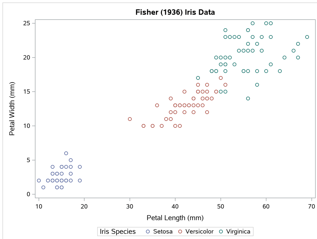
Figure 23.12 Iris Data
