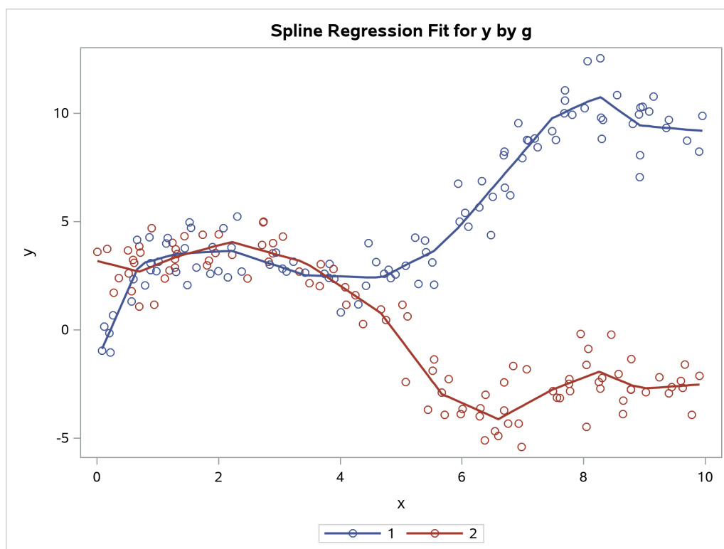
Output 23.6.20 Piecewise-Linear Splines
