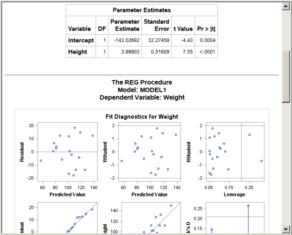
Figure 23.26 Statistical Output with the PEARL Style and HTML Destination
