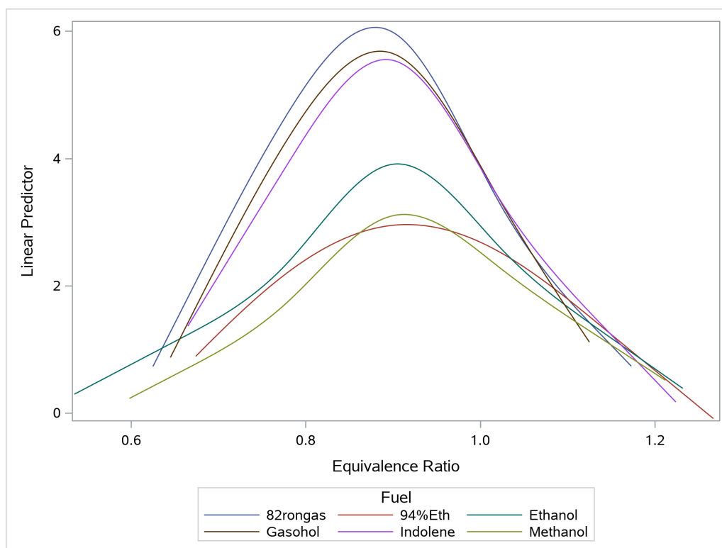
Output 23.6.30 Scored Observations
