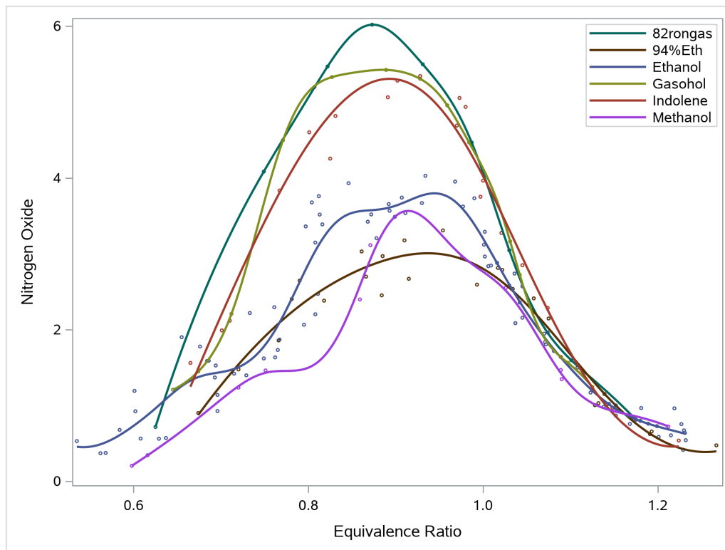
Output 23.6.10 Grouped Penalized B-Spline Fit Plot
