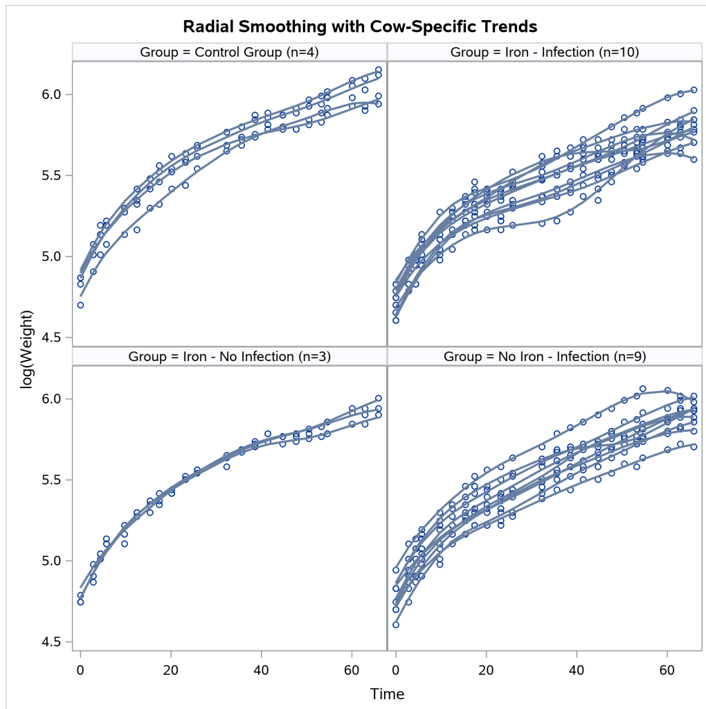
Figure 23.74 Fit Using PROC SGPPANEL
