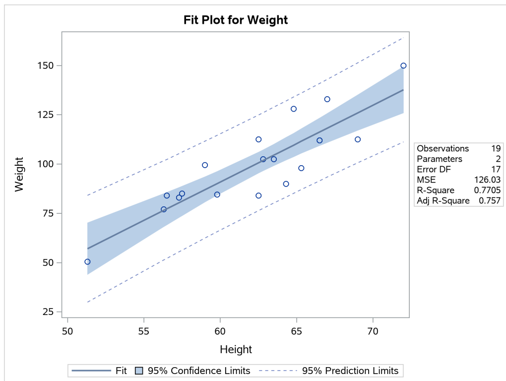
Figure 23.3 Fit Plot
