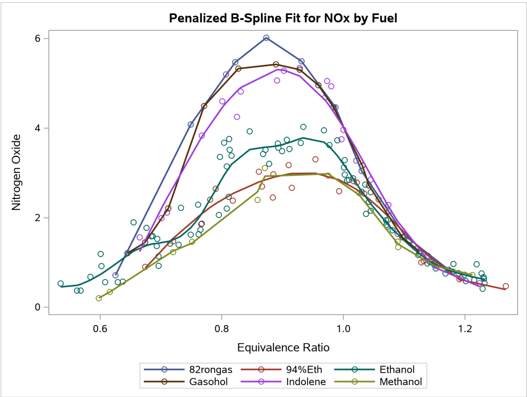
Figure 23.64 Fit Plot with the HTMLBLUE Style
