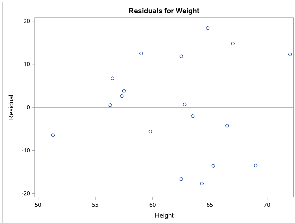
Figure 23.2 Residual Plot
