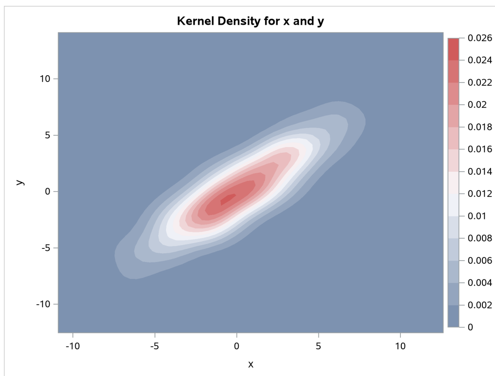
Figure 23.5 Contour Plot of Estimated Density
