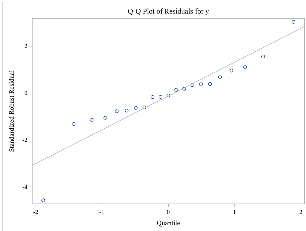
Figure 23.69 Q-Q Plot That Uses the NEWSTYLE Style
