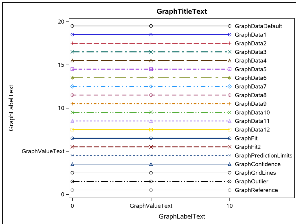
Figure 23.44 Attributes of Style Elements in the LISTING Style
