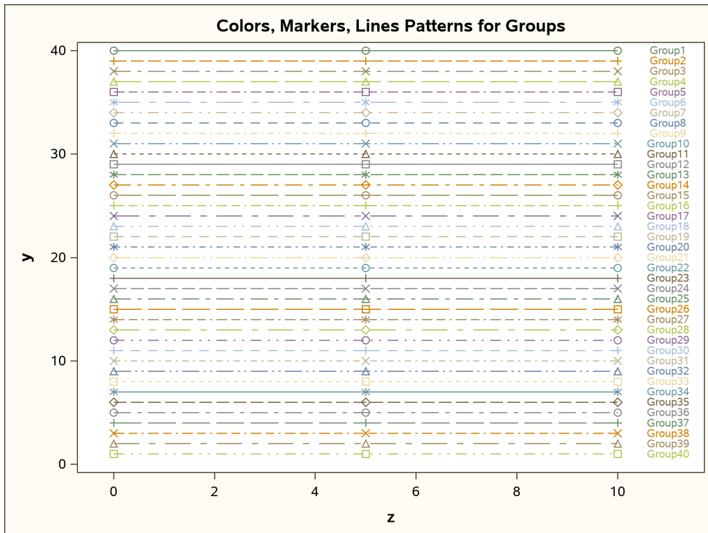
Figure 23.53 Markers, Lines, and Colors with Groups in the ANALYSIS Style
