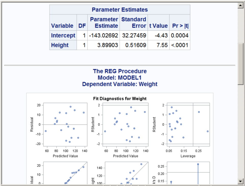
Figure 23.19 Statistical Output with the HTMLBLUE Style and HTML Destination
