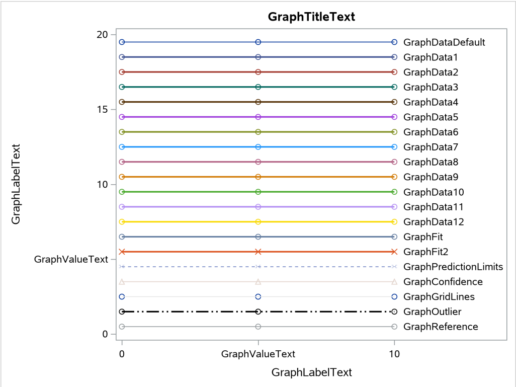
Figure 23.39 Attributes of Style Elements in the HTMLBLUE Style
