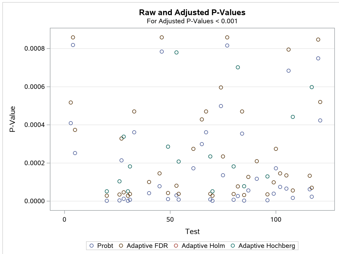
Output 85.6.7 Raw and Adjusted p -Values
