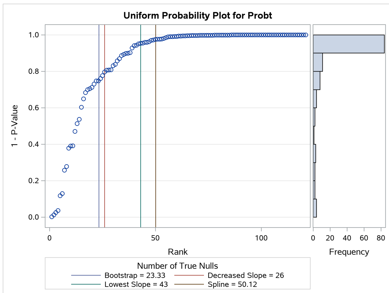
Output 85.6.4 p -Value Distribution
