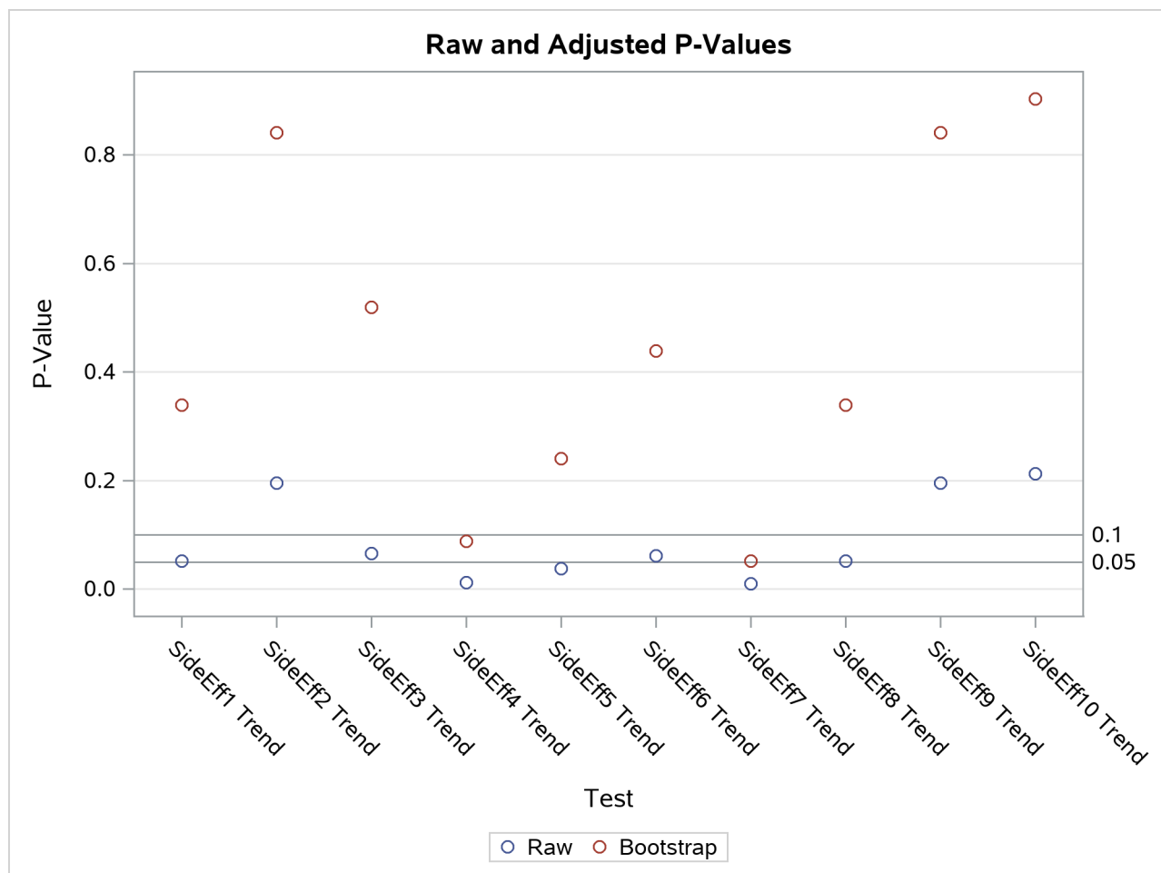
Figure 85.4 Adjusted p -Values
