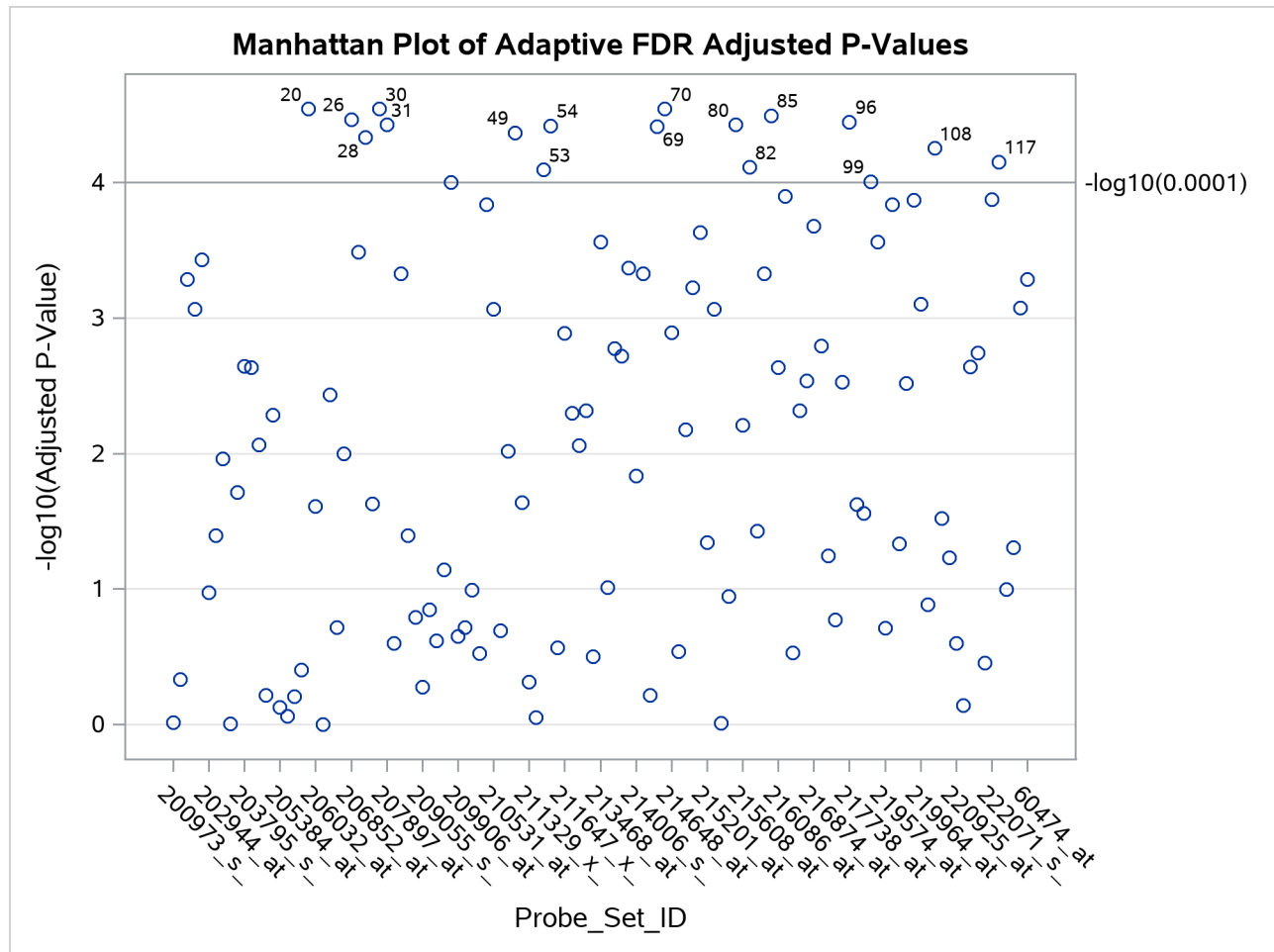
Output 85.6.6 Manhattan Plot
