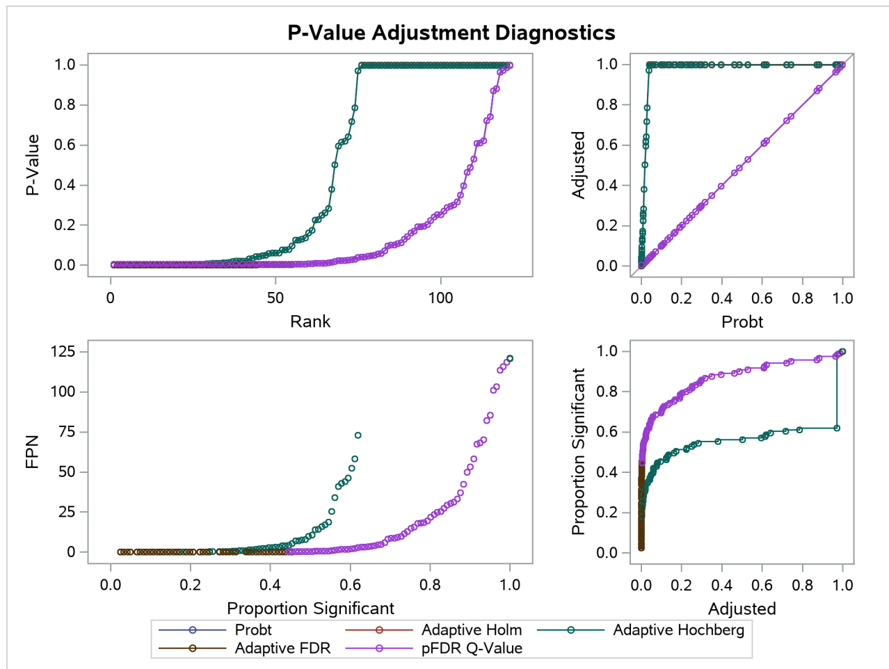
Output 85.6.5 Adjustment Diagnostics
