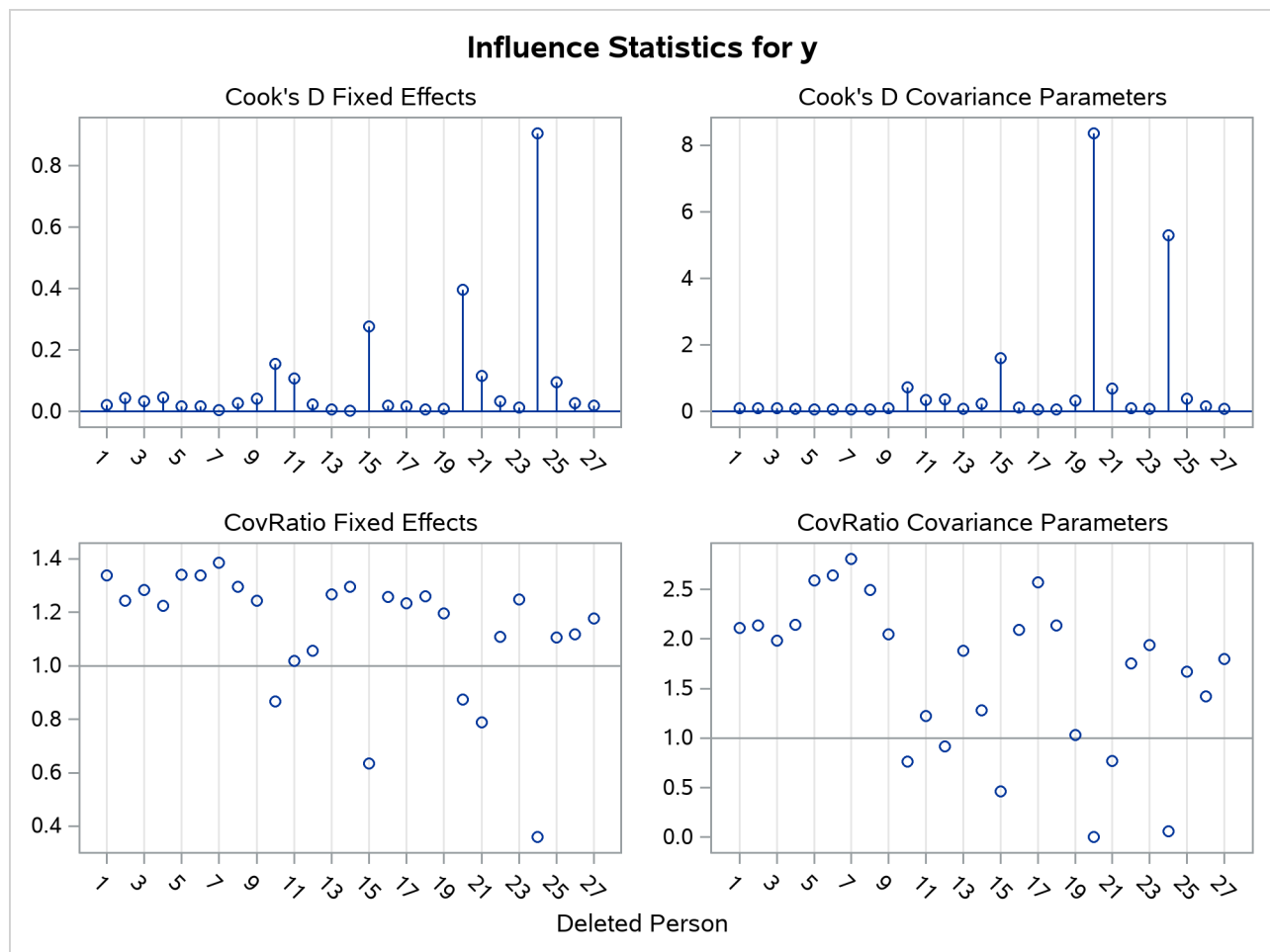
Figure 83.17 Influence Diagnostics
