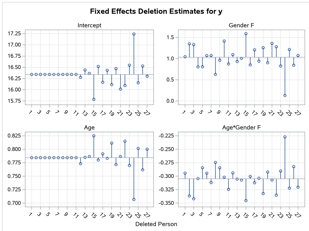
Figure 83.18 Deletion Estimates
