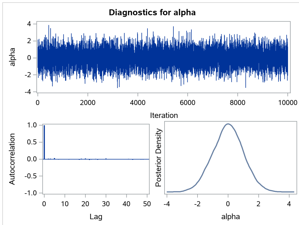
Output 79.1.3 Diagnostics Plots for \alpha
