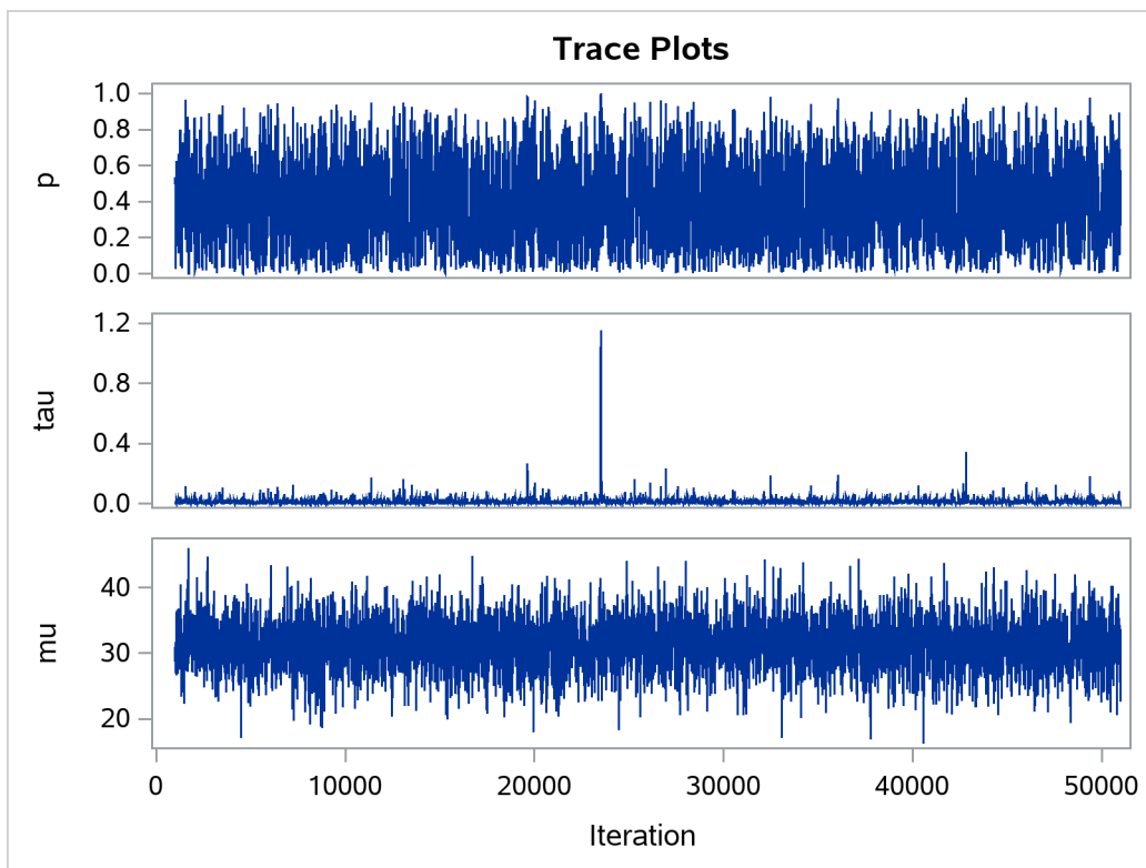
Output 79.20.4 Trace Plots after Transformation
