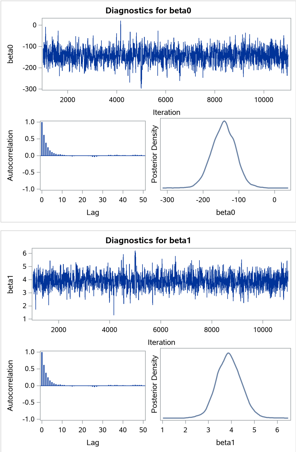
Figure 79.5 Diagnostic Plots for \beta_0 , \beta_1 and \sigma^2
