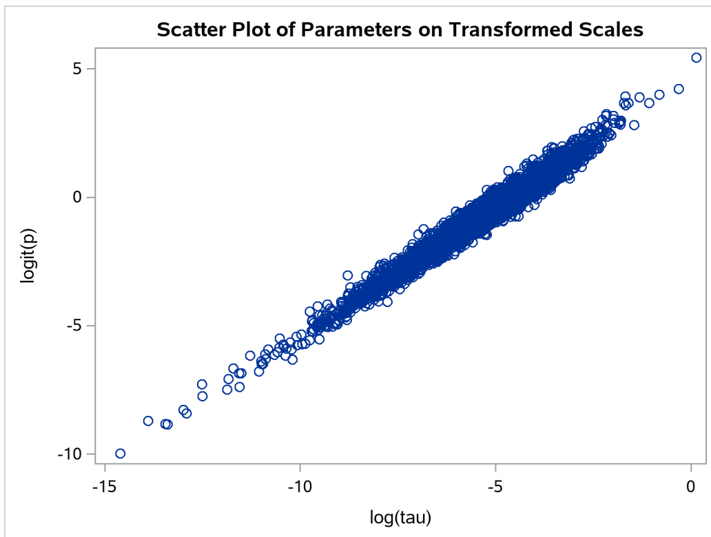
Output 79.20.6 Scatter Plot of \log(\tau) versus \text{logit}(p) , After Transformation
