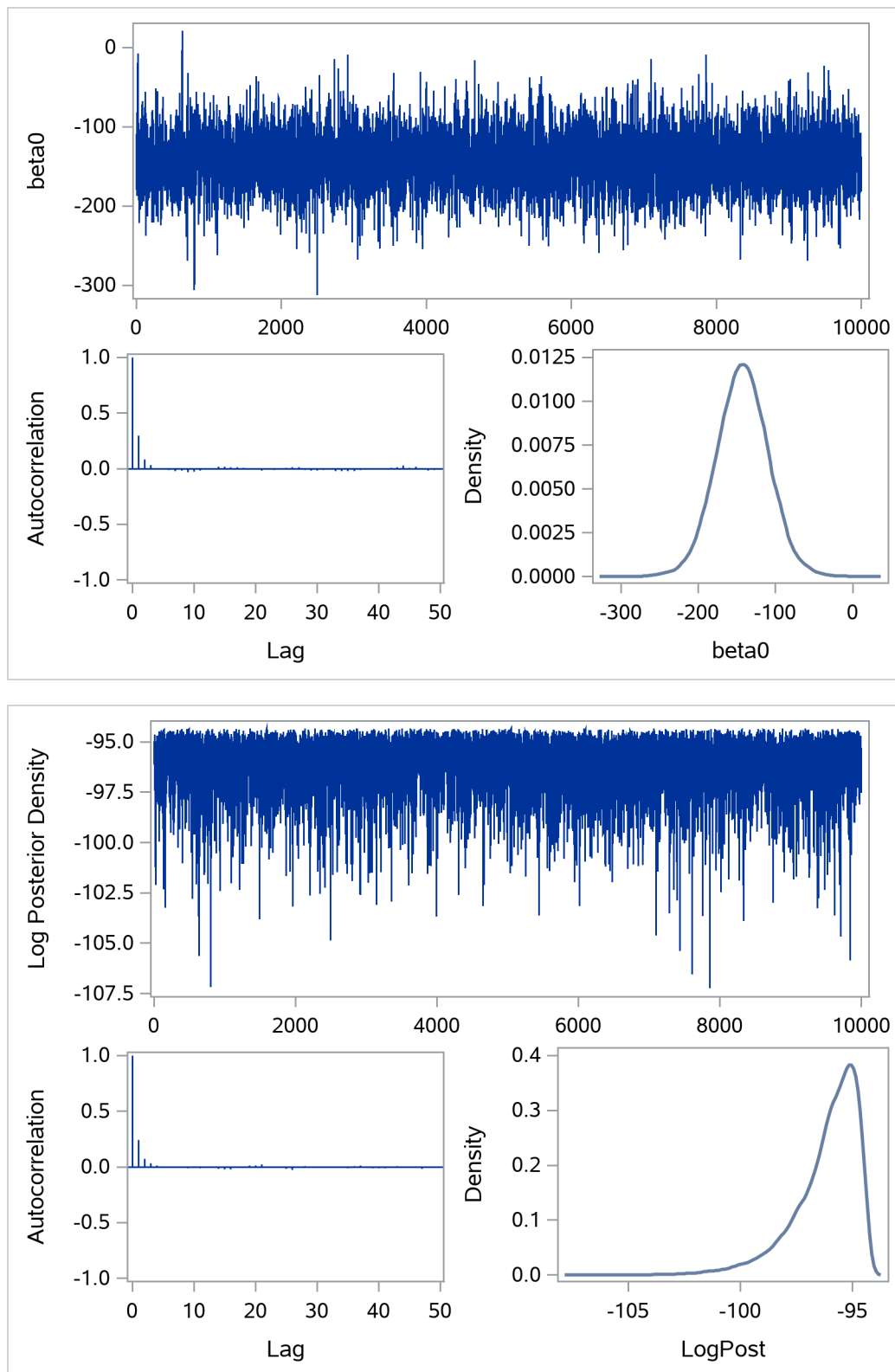
Figure 79.23 Regenerated Diagnostics Plots for beta0 and Logpost
