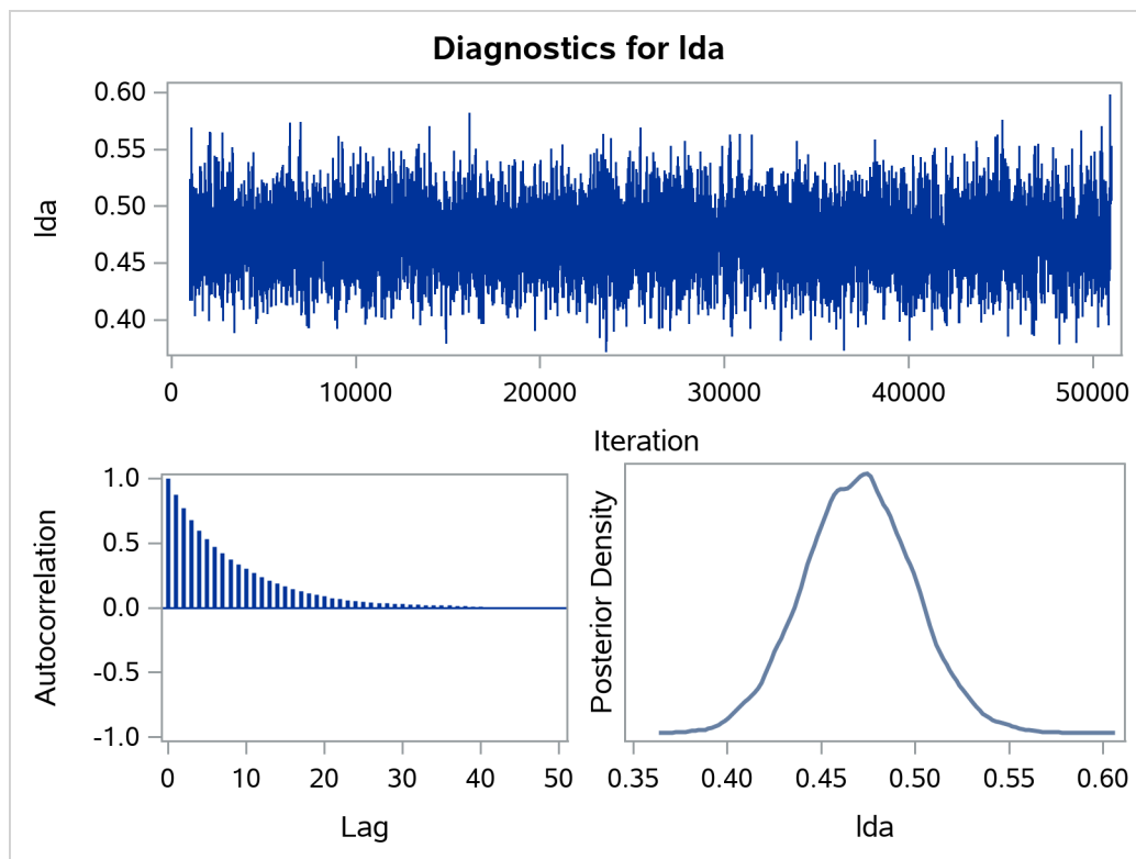
Output 79.2.2 Diagnostic Plots for \lambda
