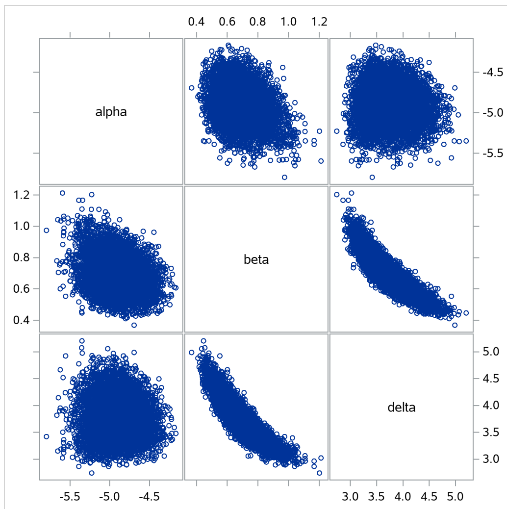
Output 79.6.7 Pairwise Scatter Plots of the Transformed Parameters
