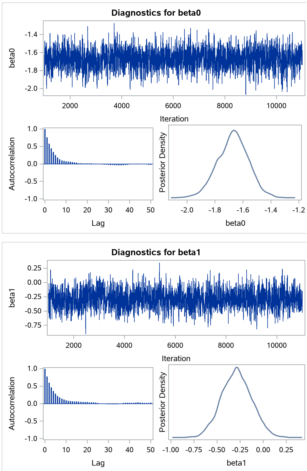
Output 79.13.1 Posterior Plots for \beta_0 and \beta_1 in the Exponential Survival Analysis
