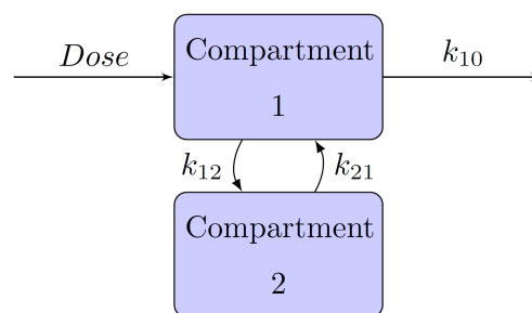
Figure 79.18 Two-Compartment Model
