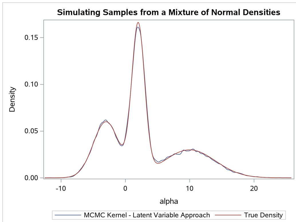
Output 79.1.9 Estimated Density (Latent Variable Approach) versus the True Density
