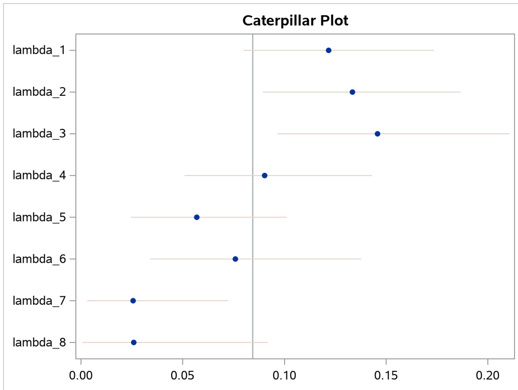
Output 79.16.4 Caterpillar Plot of the Hazards in the Piecewise Exponential Model
