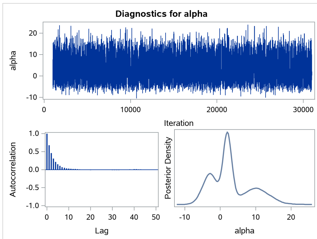
Output 79.1.8 Plots of Posterior Samples from a Mixture Normal Distribution
