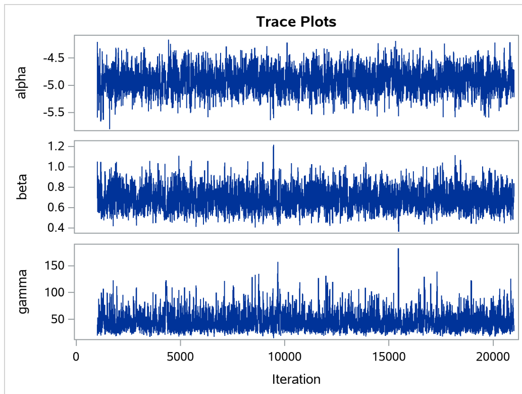
Output 79.6.4 Plots for Parameters, Sampling on the Log Scale of Gamma
