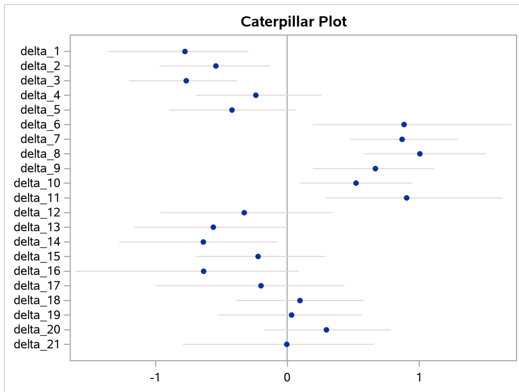
Figure 79.24 Caterpillar Plot of the Random-Effects Parameters
