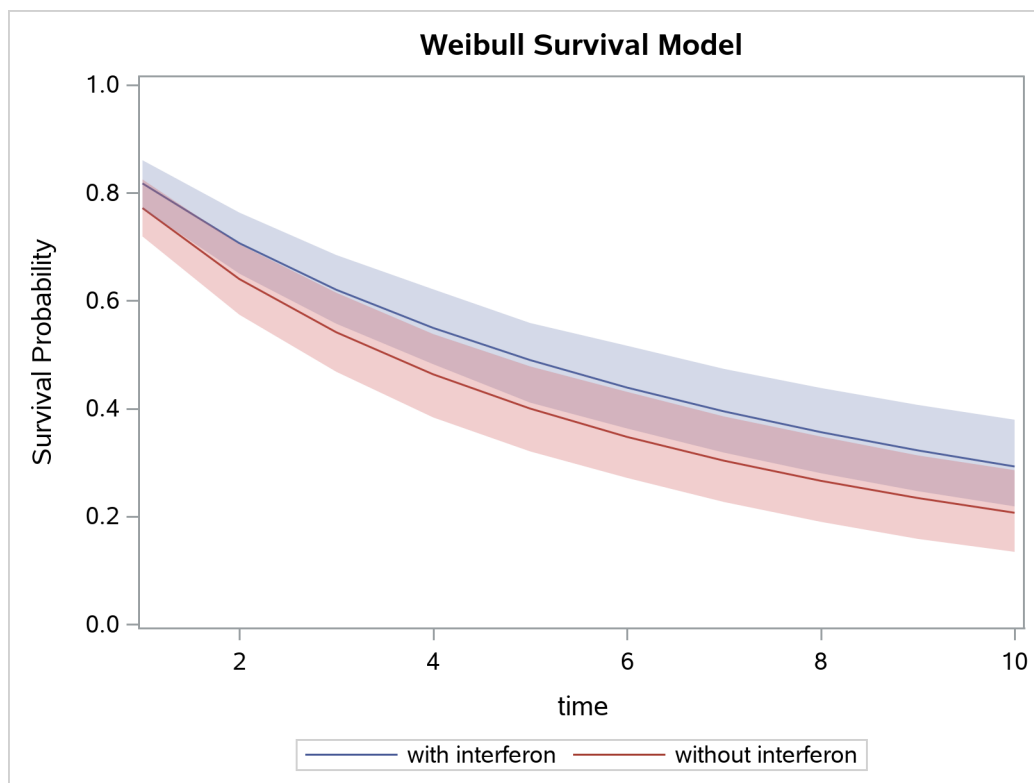
Output 79.13.7 Predicted Survival Probability Curves with 95% HPD Intervals
