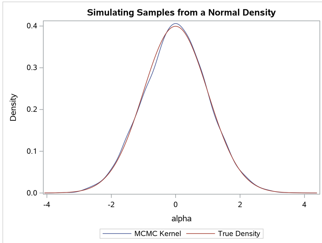
Output 79.1.4 Estimated Density versus the True Density
