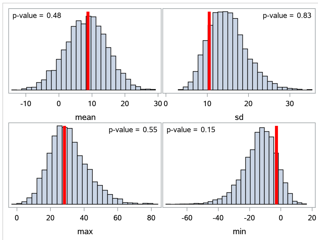
Figure 79.27 Posterior Predictive Distribution Check for the SAT example
