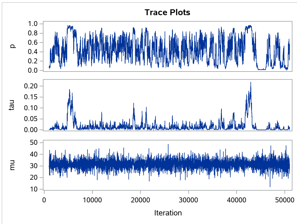
Output 79.20.1 Trace Plots
