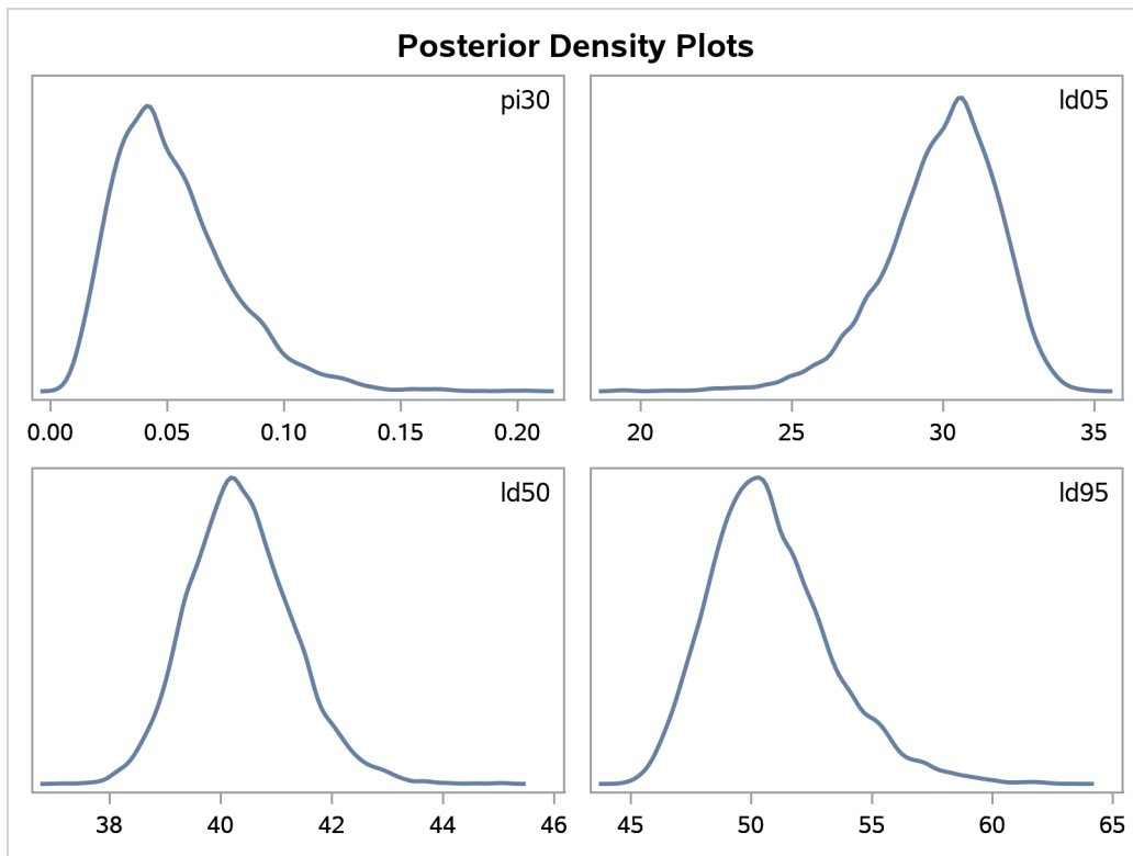
Output 79.3.5 Density Plots of Quantities of Interest in the Logistic Regression Example
