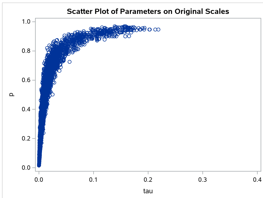
Output 79.20.3 Scatter Plot of \tau versus p
