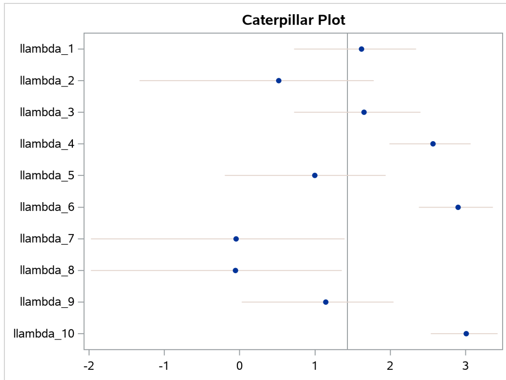
Output 79.8.4 Caterpillar Plots of the Random-Effects Parameters
