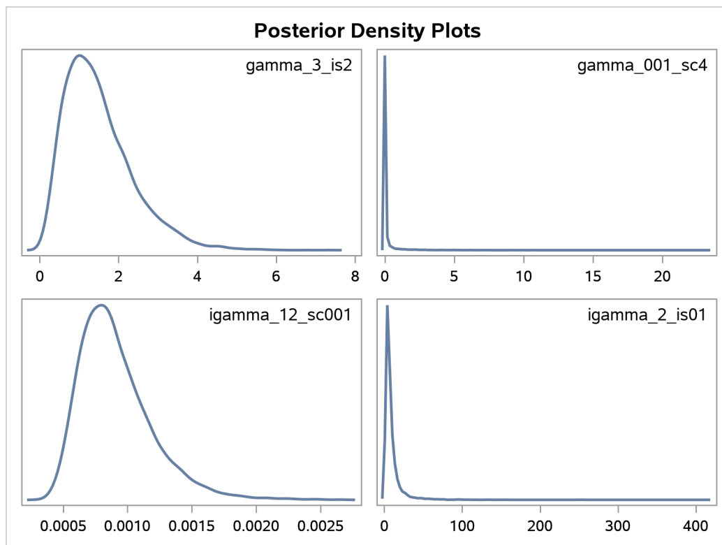
Figure 79.26 Density Plots of Different Gamma and Inverse Gamma Distributions
