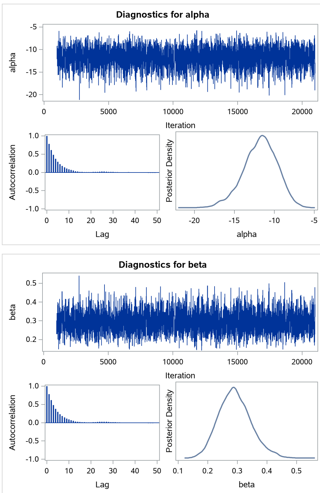
Output 79.3.2 Plots for Parameters in the Logistic Regression Example
