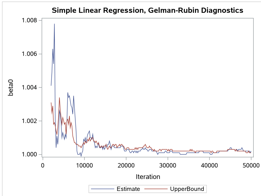
Output 79.21.3 PSRF Plot for Each Parameter
