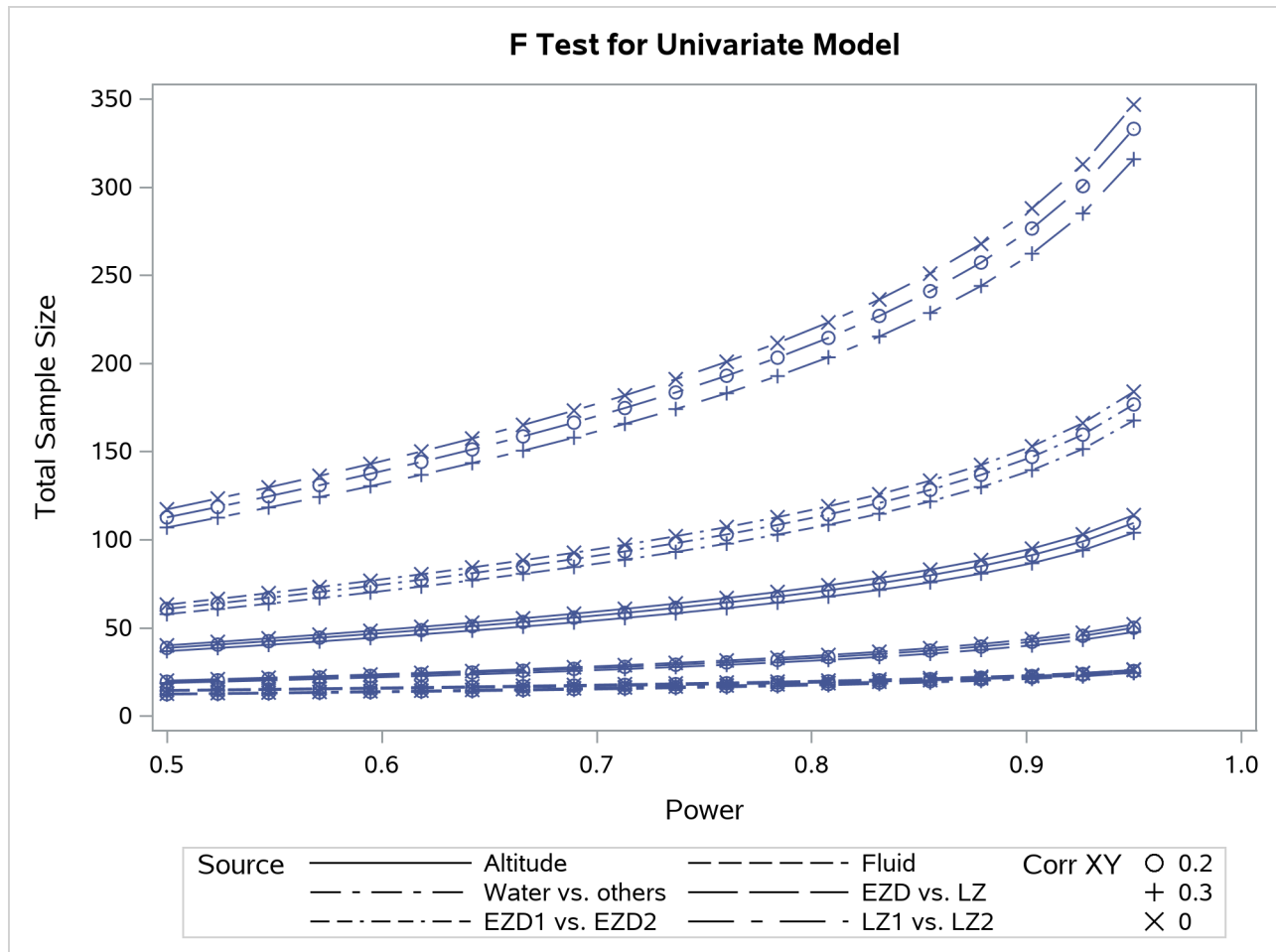
Output 54.2.2 Plot of Sample Size versus Power for Two-Way ANOVA Contrasts
