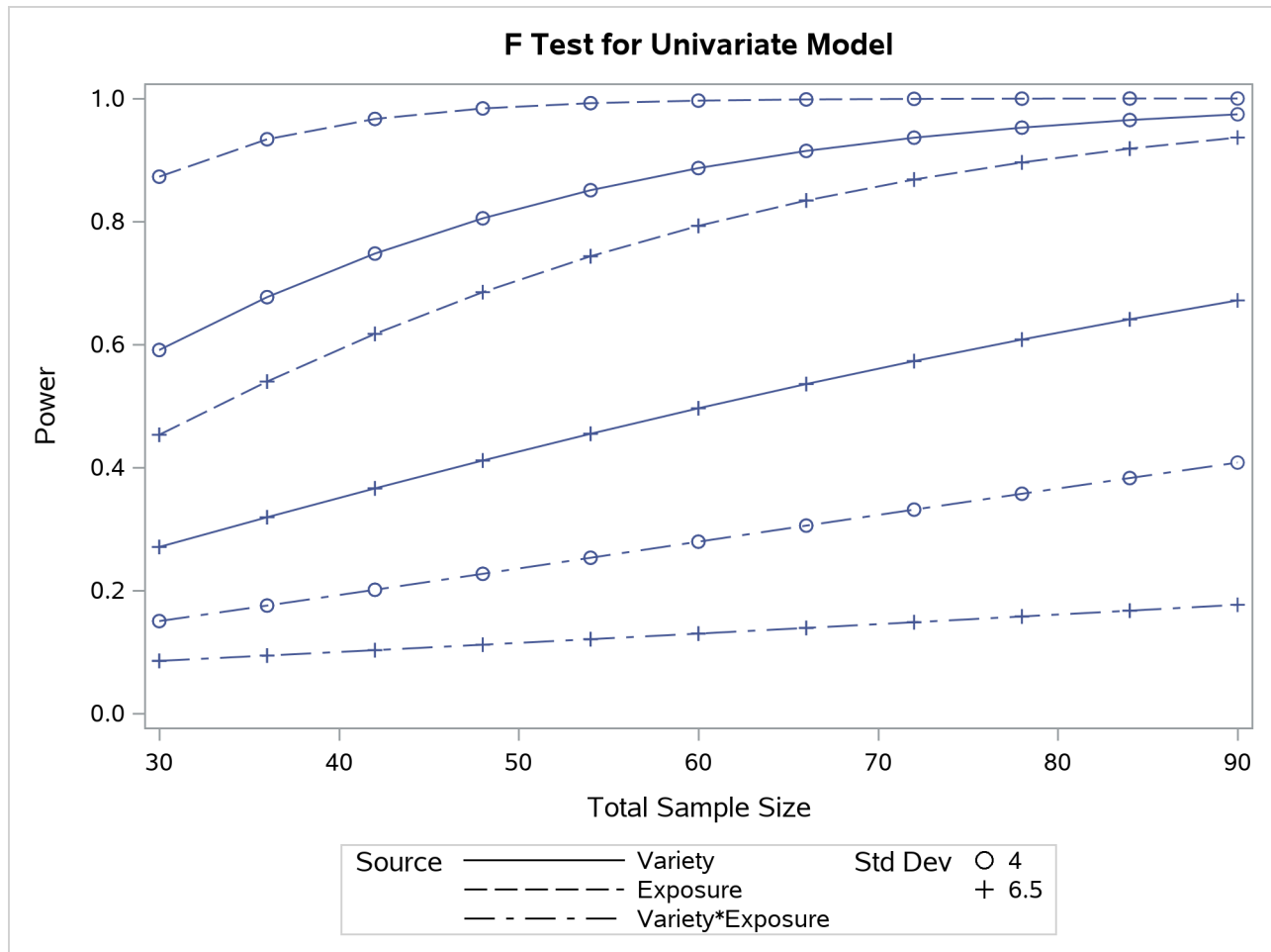
Figure 54.3 Plot of Power versus Sample Size for Two-Way ANOVA with Input Ranges
