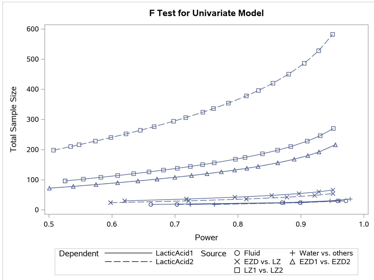
Output 54.1.2 Plot of Sample Size versus Power for One-Way ANOVA Contrasts
