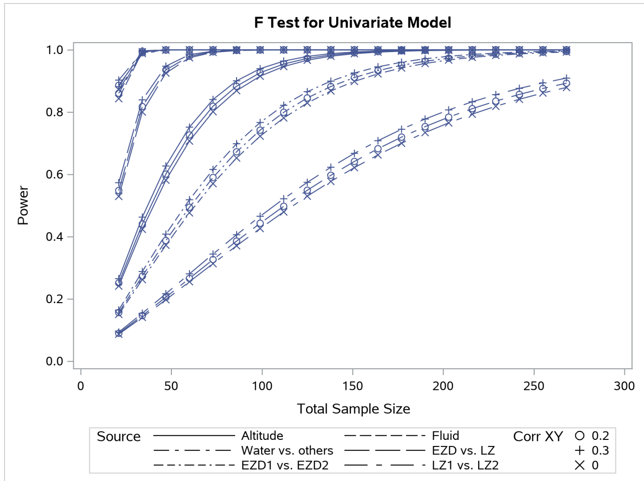
Output 54.2.3 Plot of Power versus Sample Size for Two-Way ANOVA Contrasts
