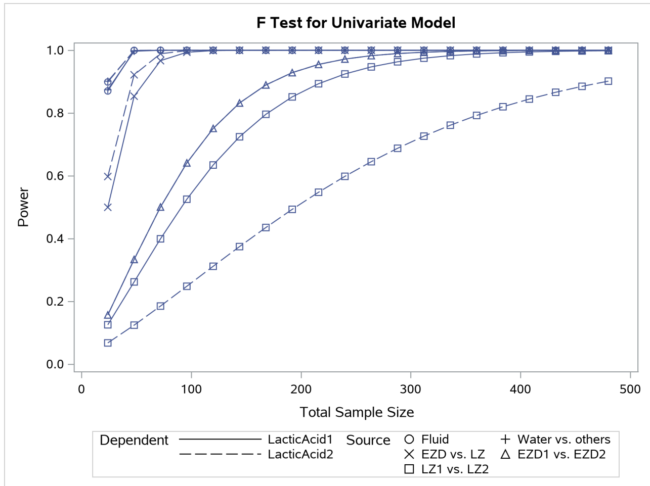
Output 54.1.3 Plot of Power versus Sample Size for One-Way ANOVA Contrasts
