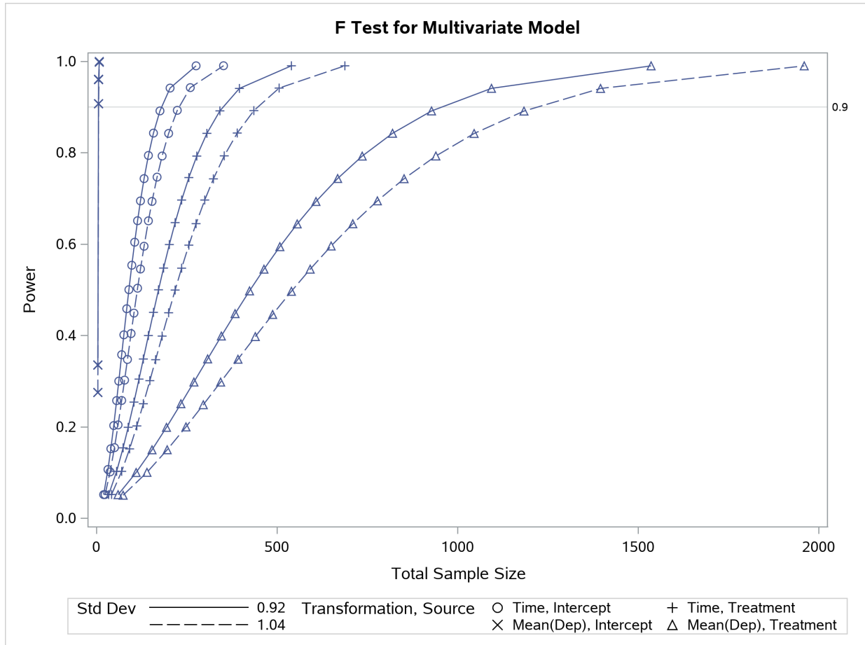
Output 54.3.2 Plot of Power versus Sample Size for Repeated Measures Analysis
