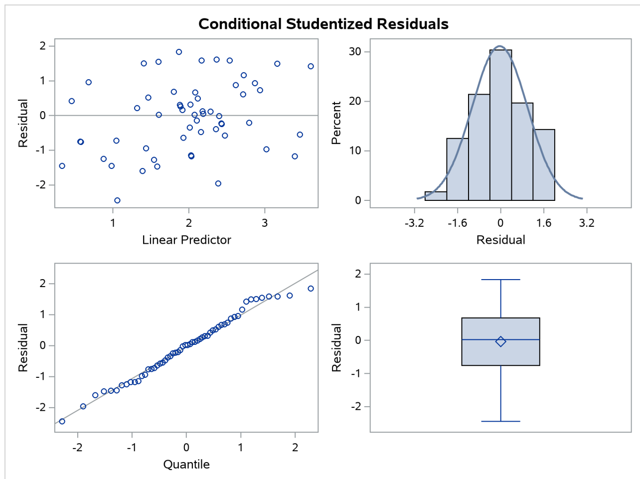
Output 51.3.6 Panel of Studentized Residuals
