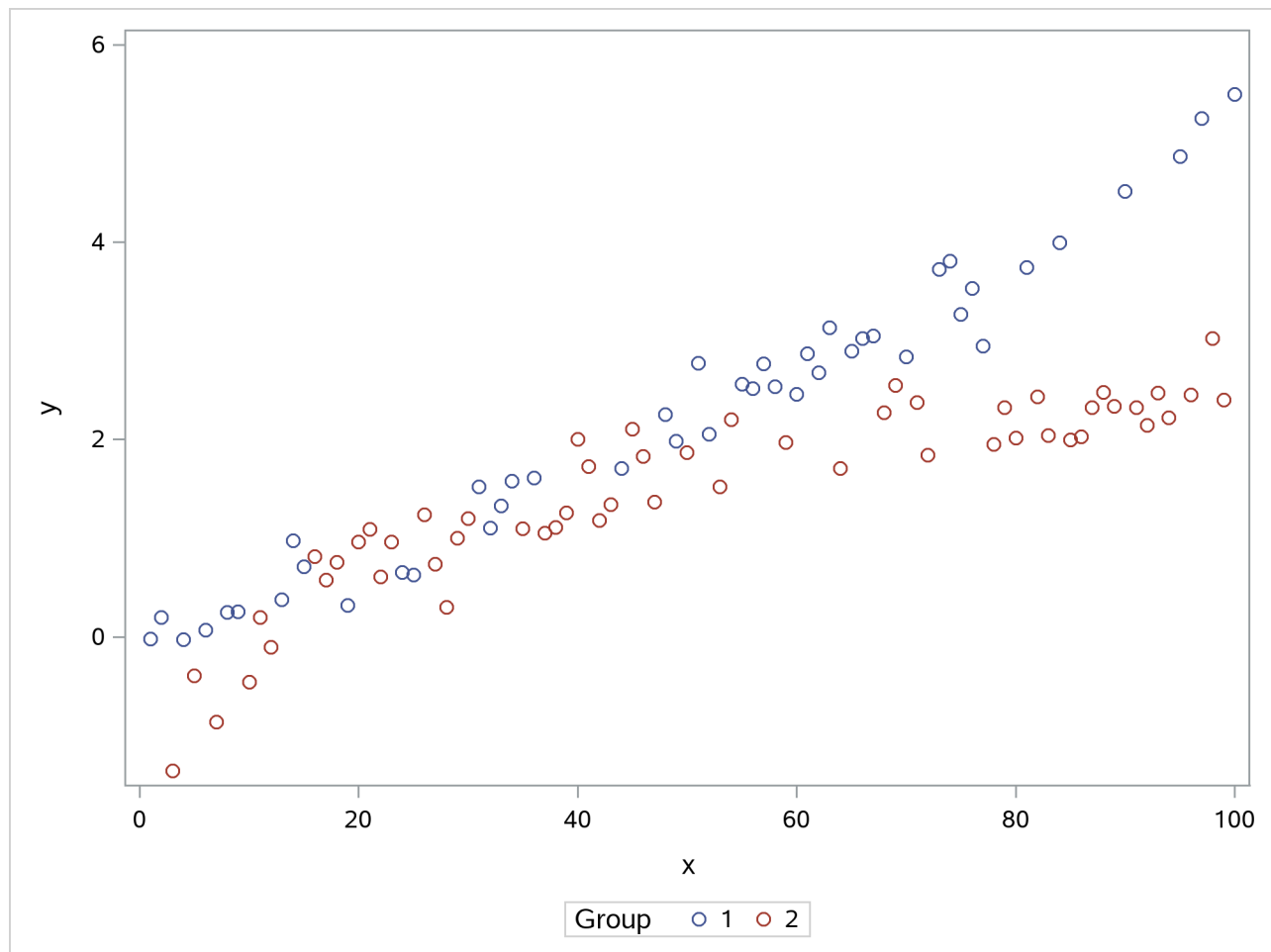
Output 51.15.1 Scatter Plot of Observed Data by Group
