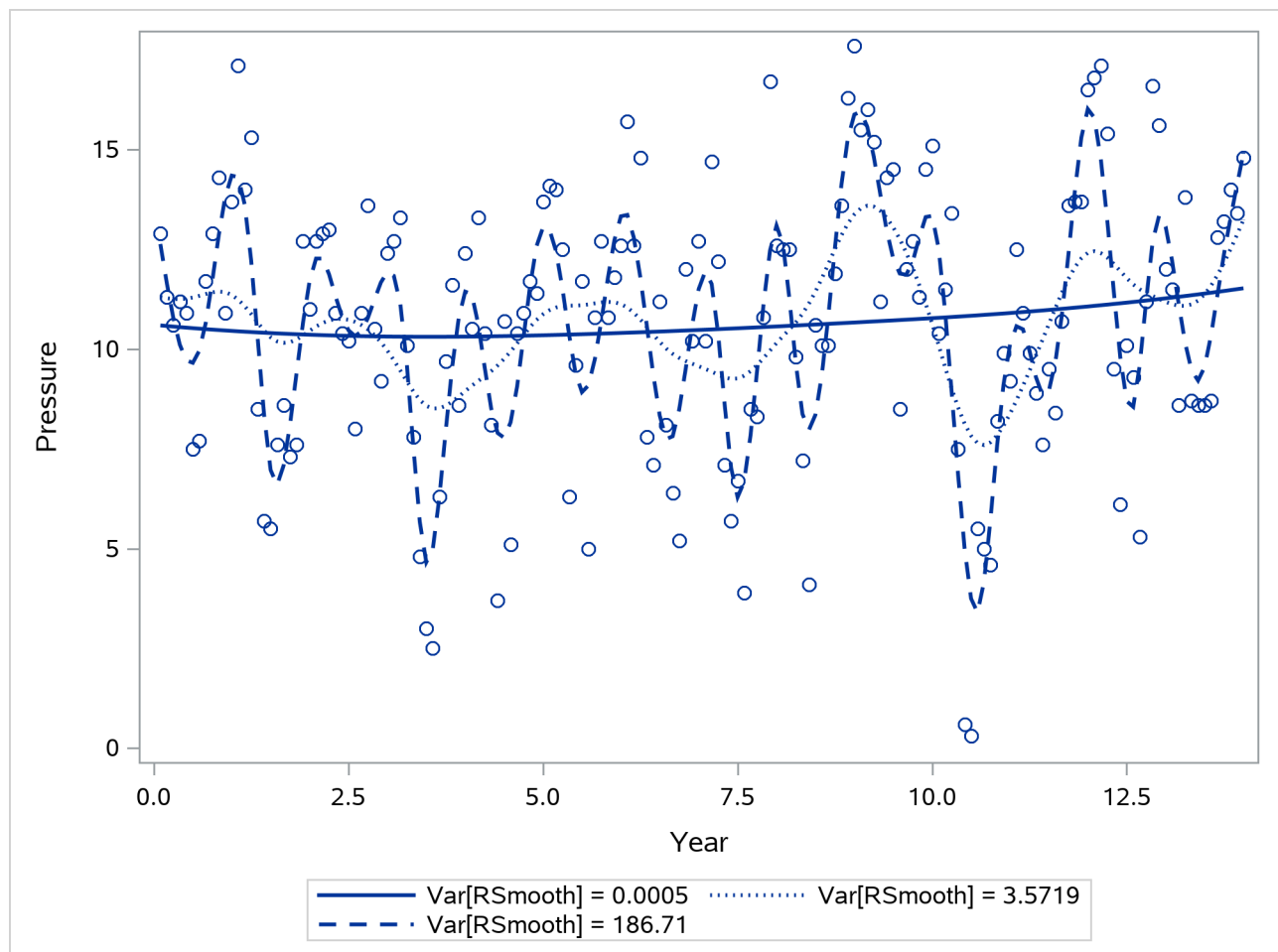
Output 51.10.4 Observed and Predicted Pressure Differences
