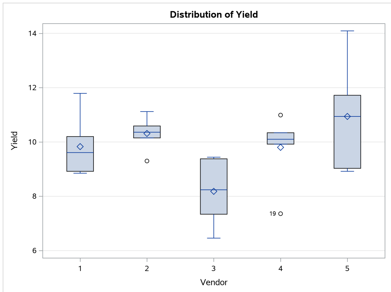
Figure 51.21 Box Plots of Observed Values
