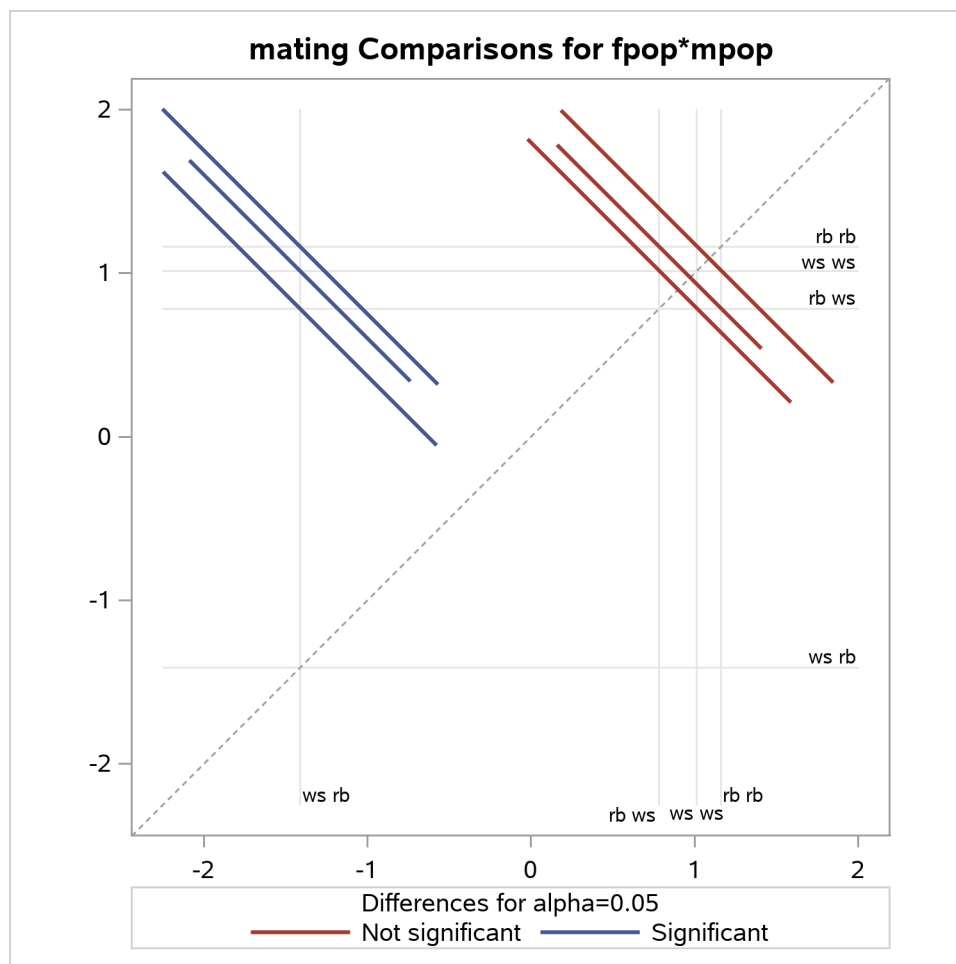
Output 51.2.10 LS-Means Diffogram
