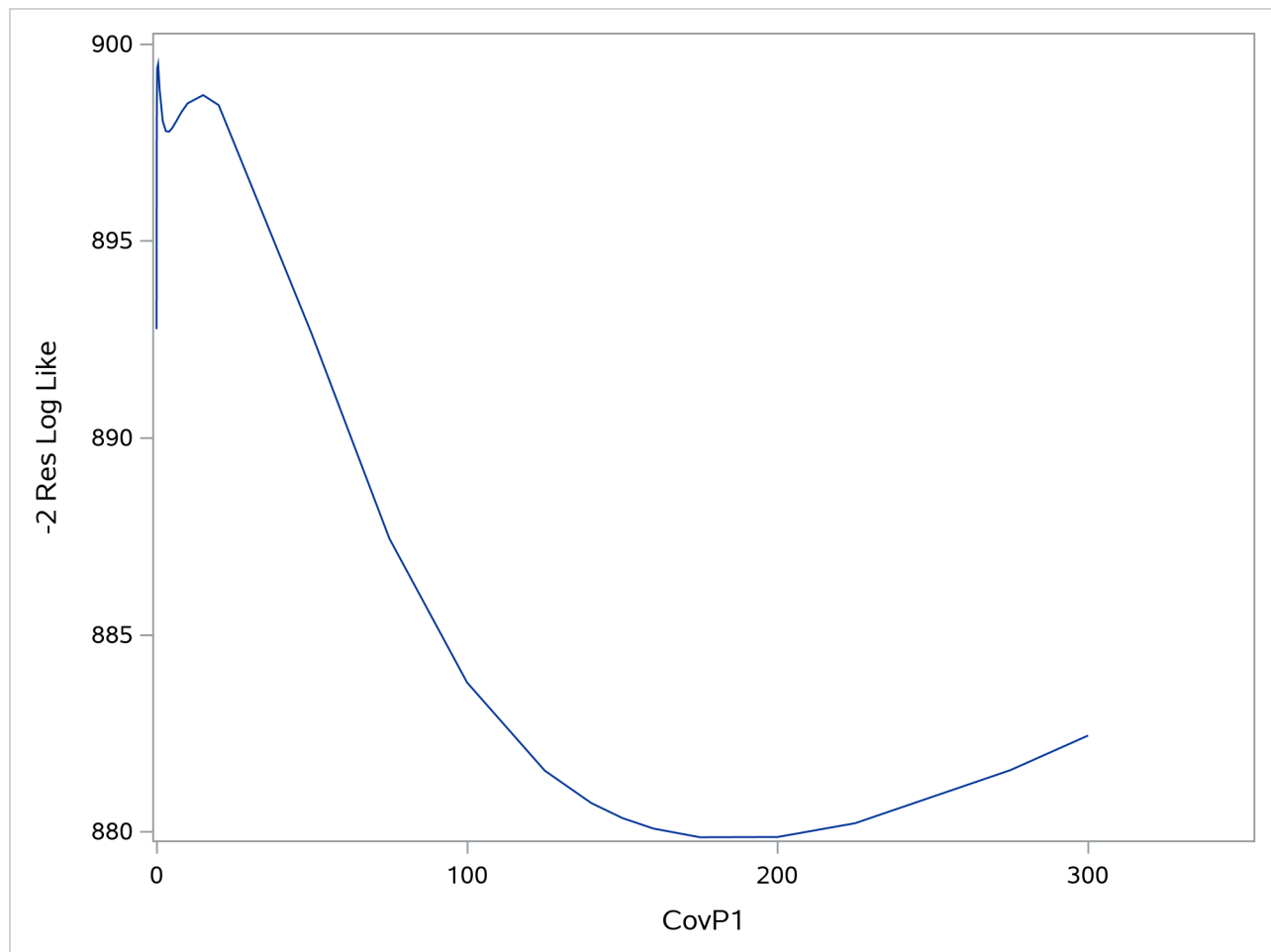
Output 51.10.3 -2 Restricted Profile Log Likelihood for Smoothing Variance
