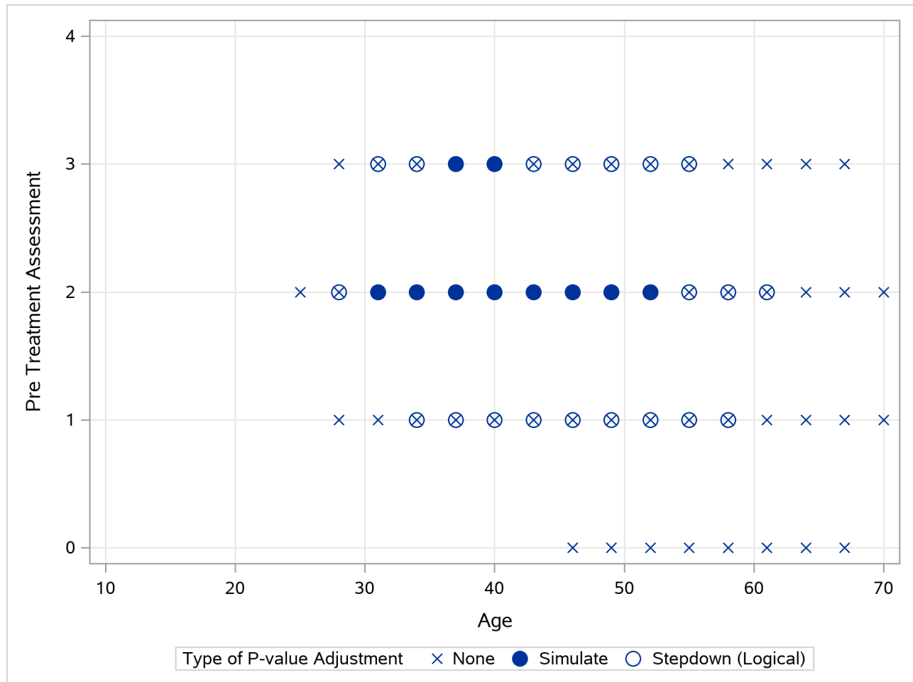
Output 51.13.2 Comparison of Significance Regions
