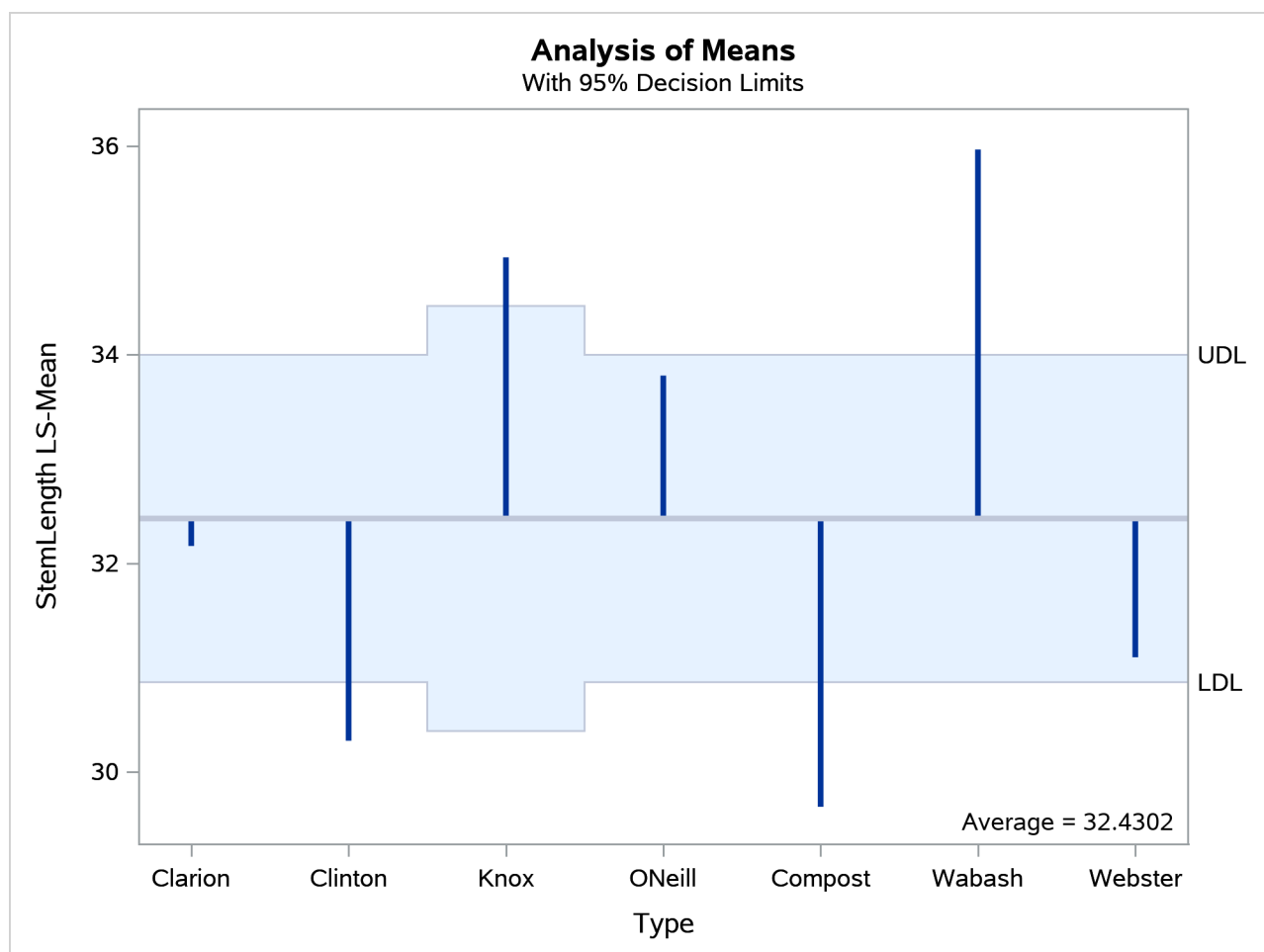
Figure 51.33 LS-Means Analysis of Means (ANOM) Plot
