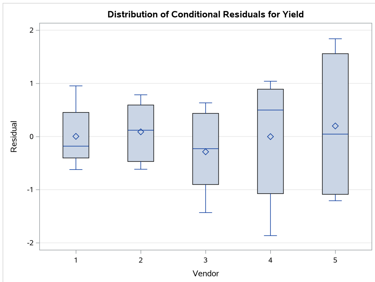
Figure 51.23 Box Plots of Conditional Residuals
