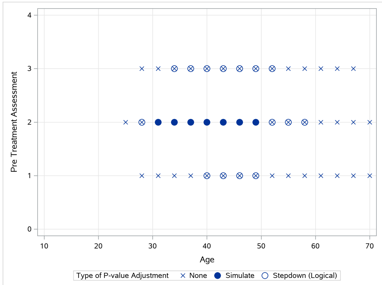
Output 51.13.5 Comparison of Significance Regions, Ordinal Analysis
