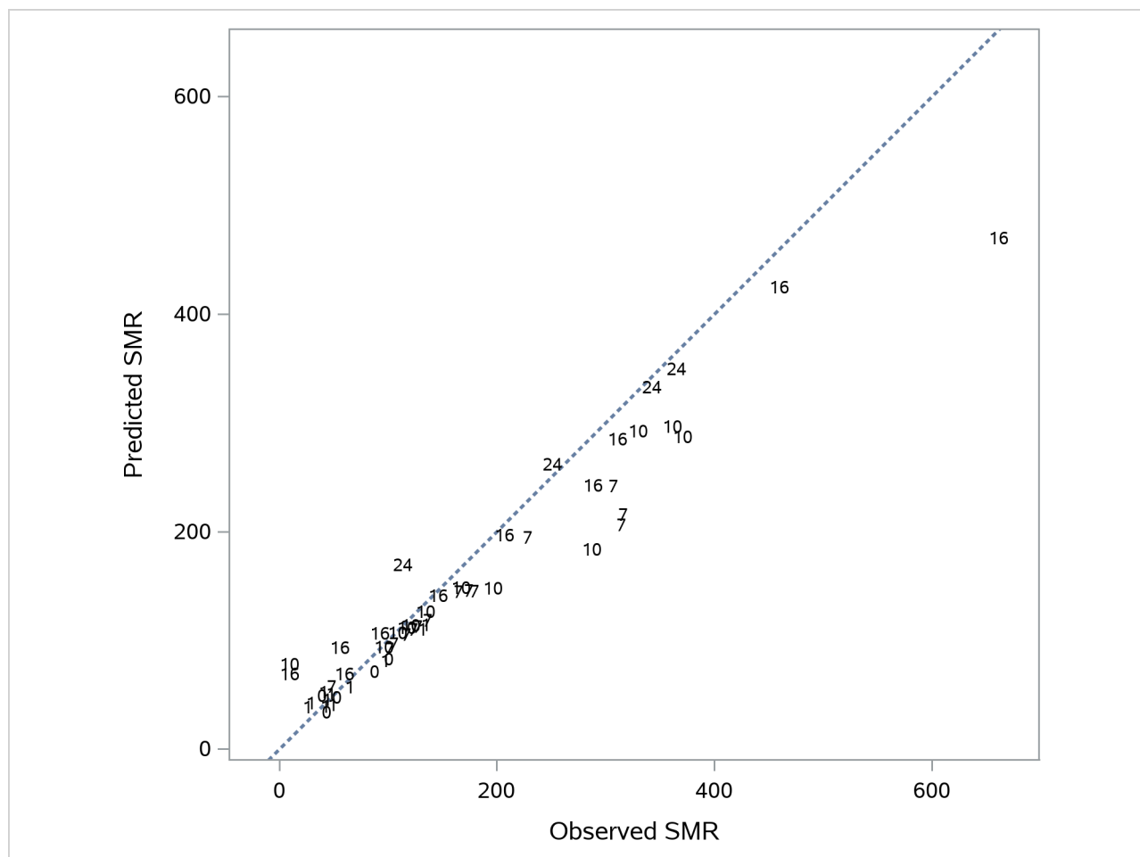
Output 51.3.7 Observed and Predicted SMRs; Data Labels Indicate Covariate Values
