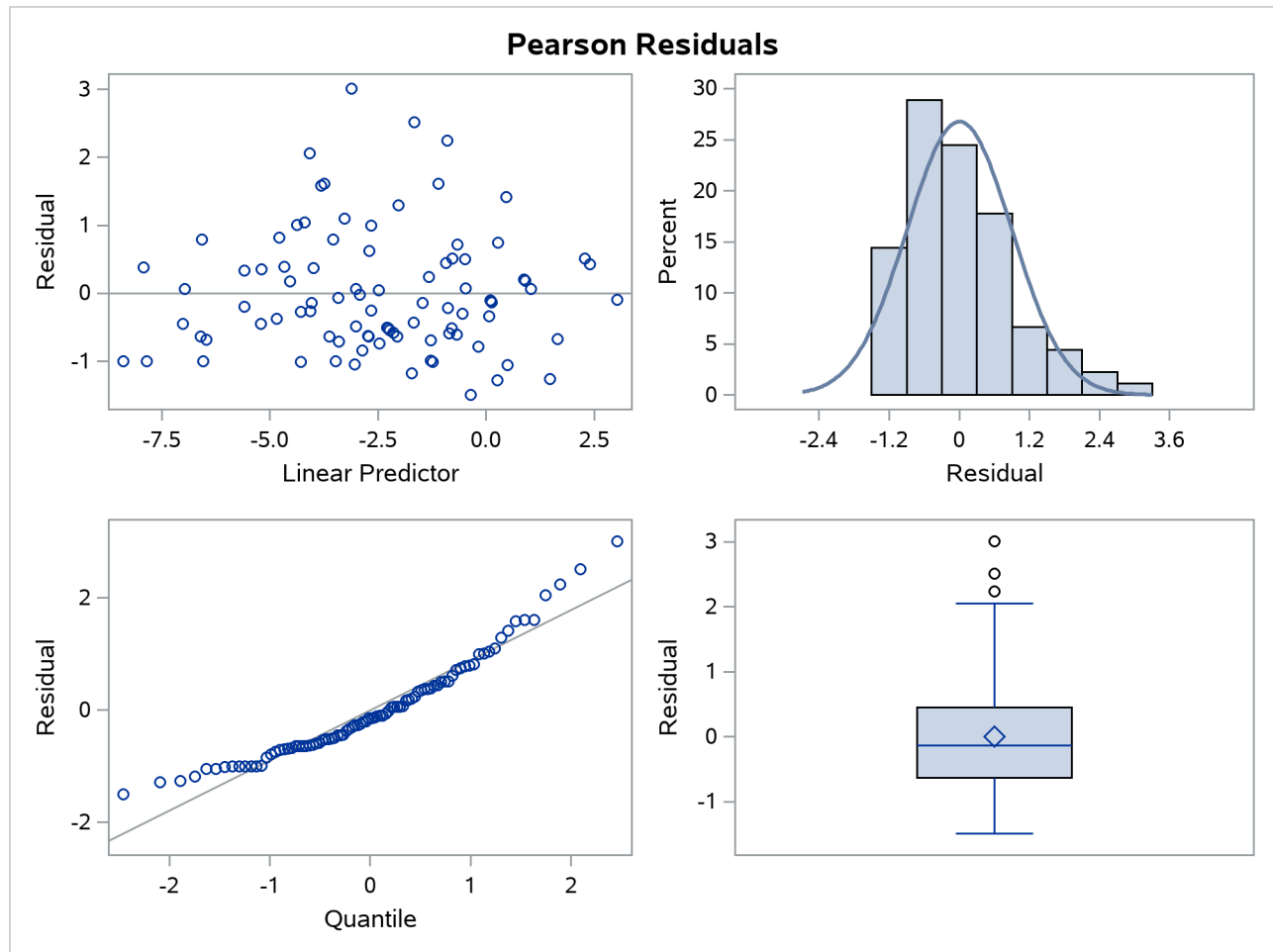
Output 51.4.10 Panel of Pearson-Type Residuals (Quasi-likelihood)
