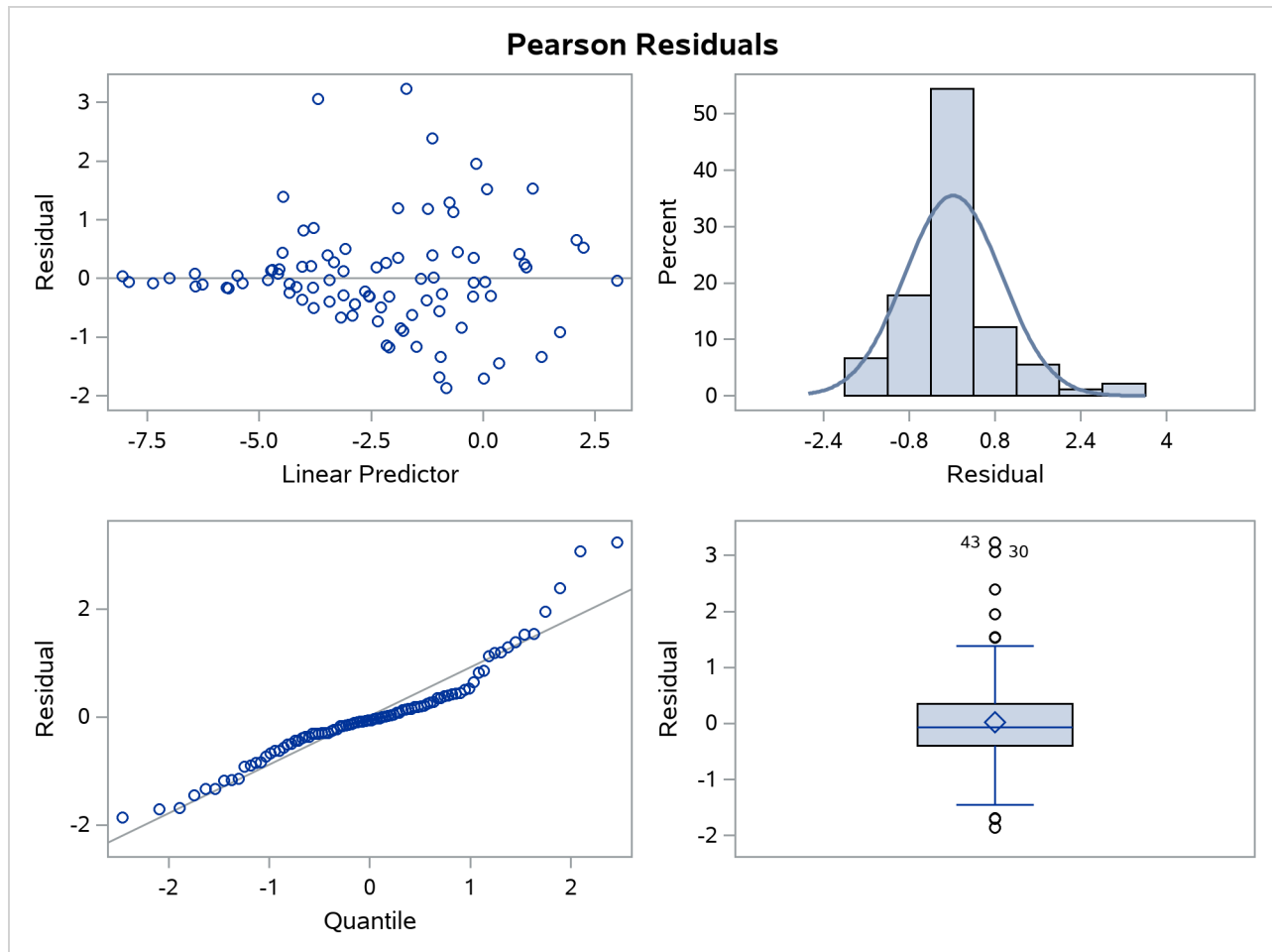
Output 51.4.7 Panel of Pearson-Type Residuals in Pseudo-binomial Analysis
