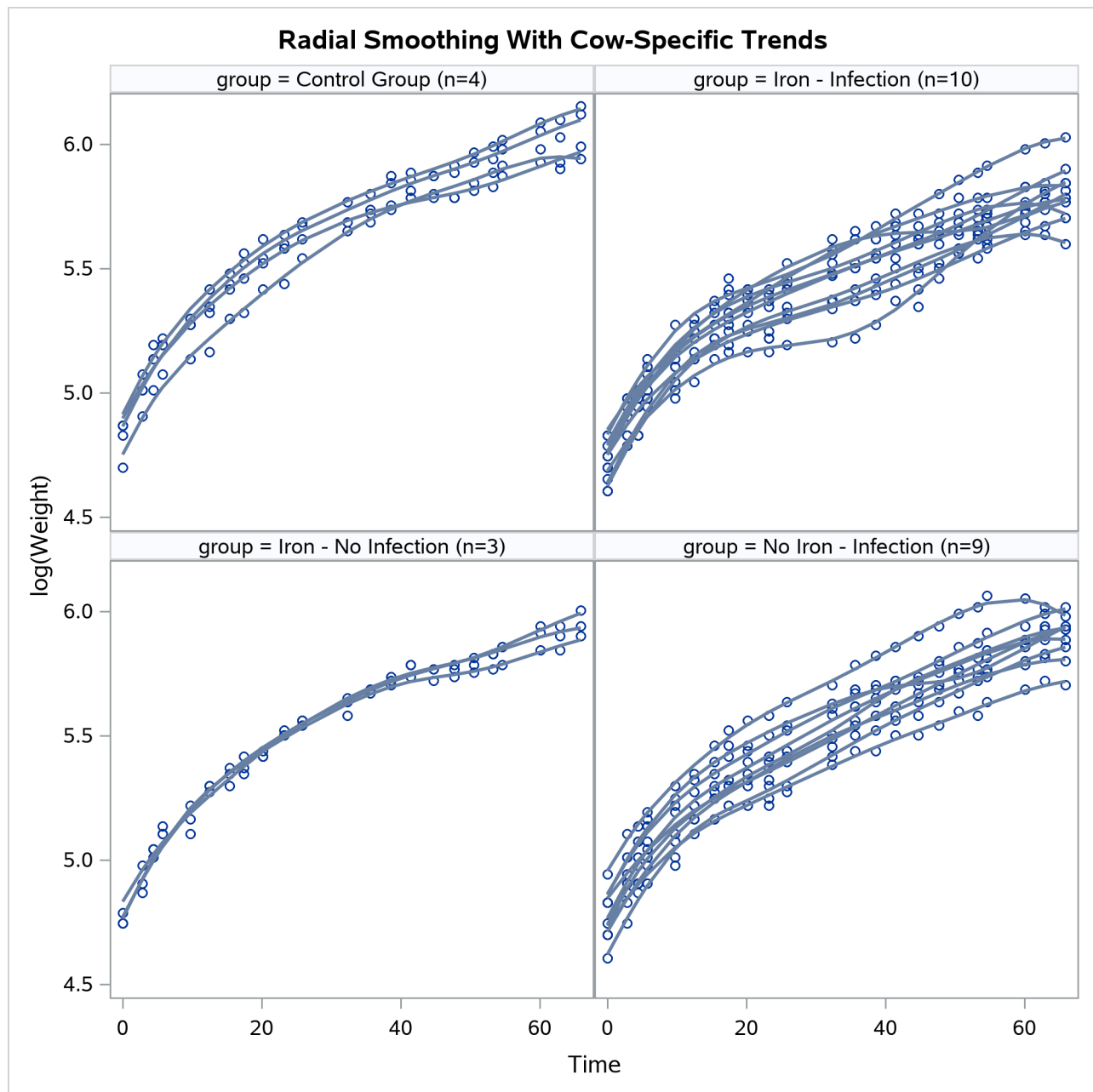
Output 51.6.9 Observed and Predicted Profiles
