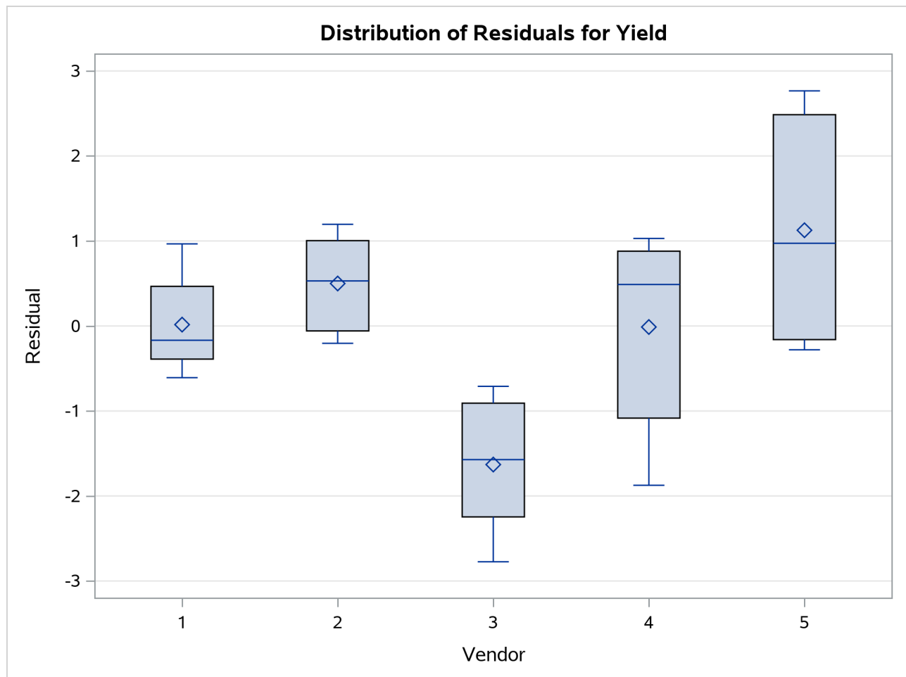
Figure 51.22 Box Plots of Marginal Residuals
