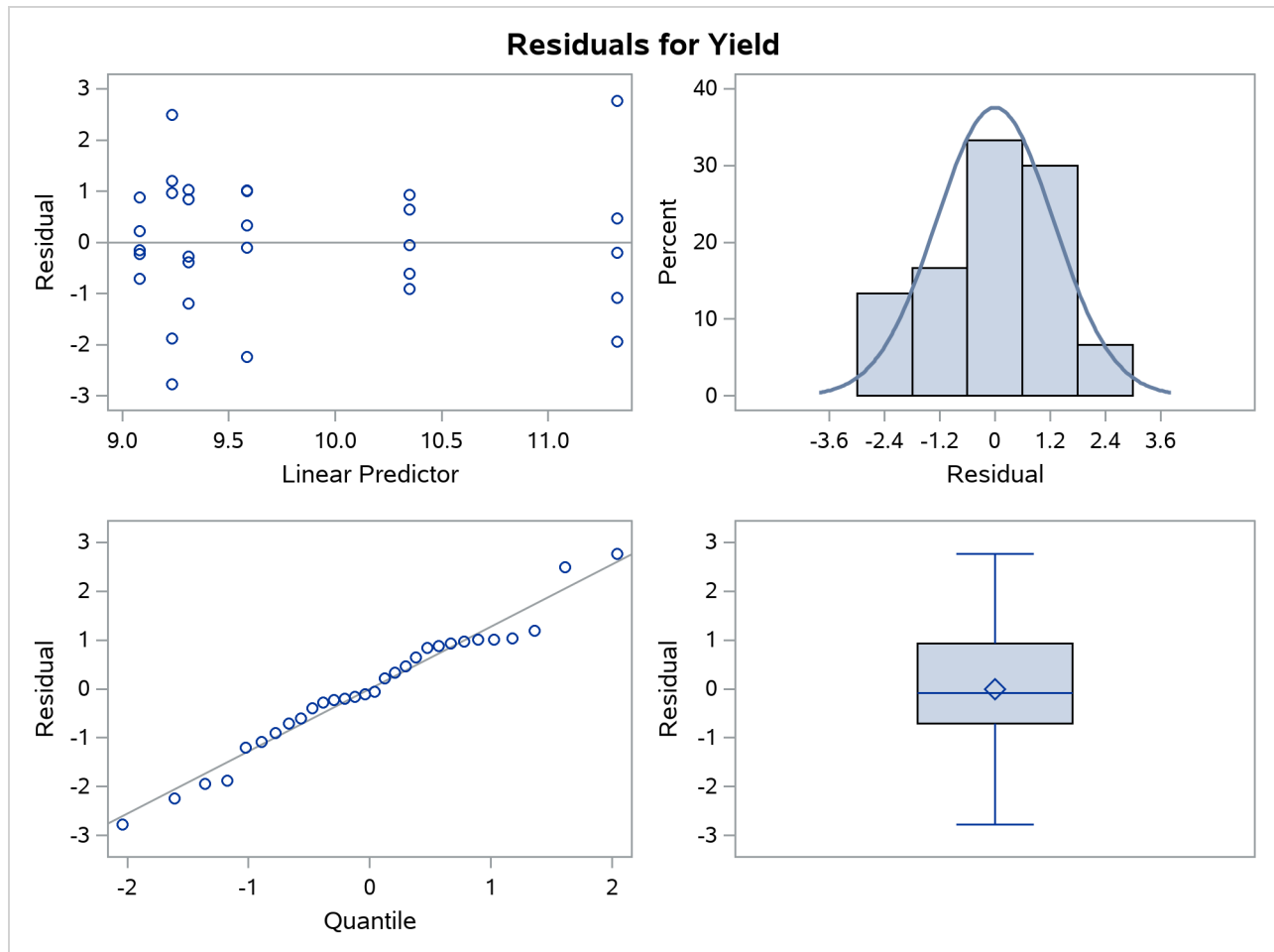
Figure 51.20 Marginal Residuals
