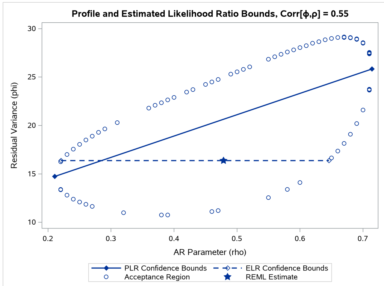
Figure 51.12 PLR and ELR Intervals, Large Correlation between Parameters
