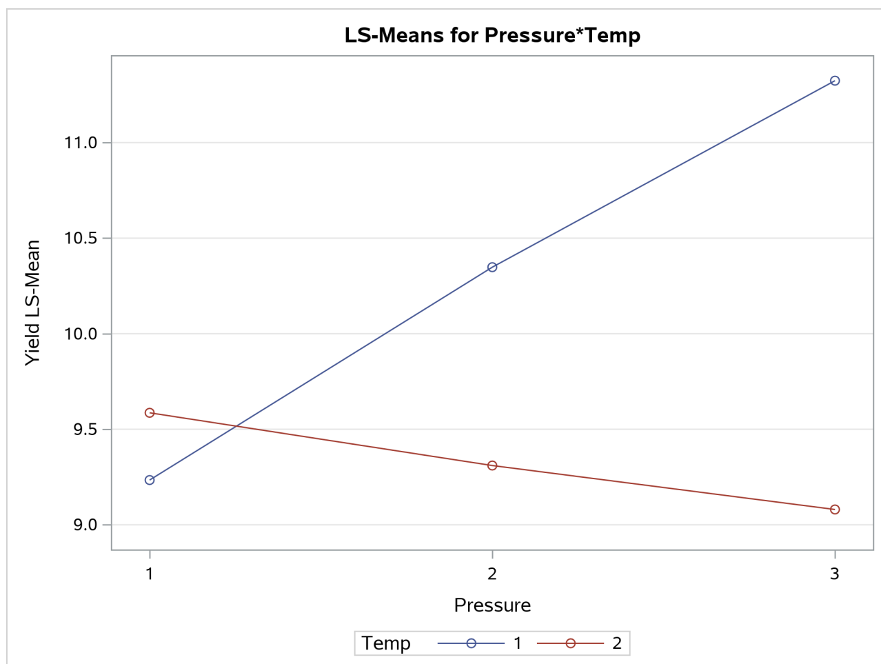
Figure 51.25 Interaction Plot for Pressure x Temperature
