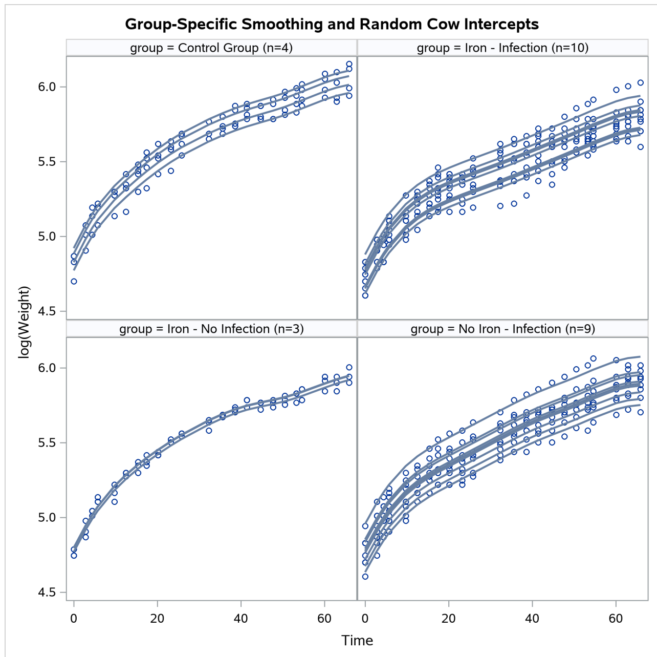
Output 51.6.12 Observed and Predicted Profiles
