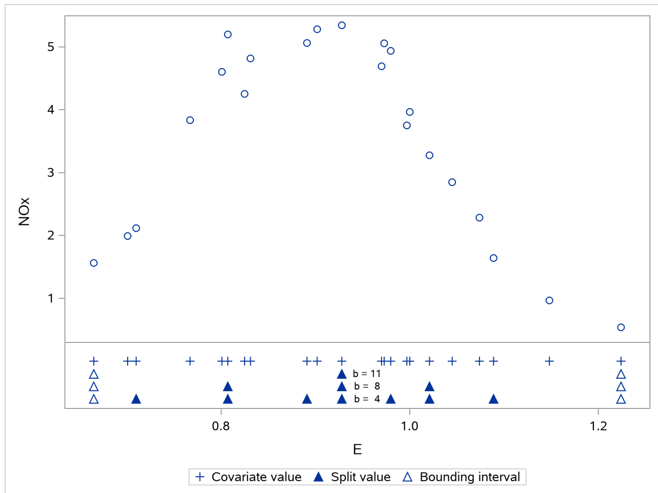
Figure 51.16 Vertices of k -d Trees for Various Bucket Sizes
