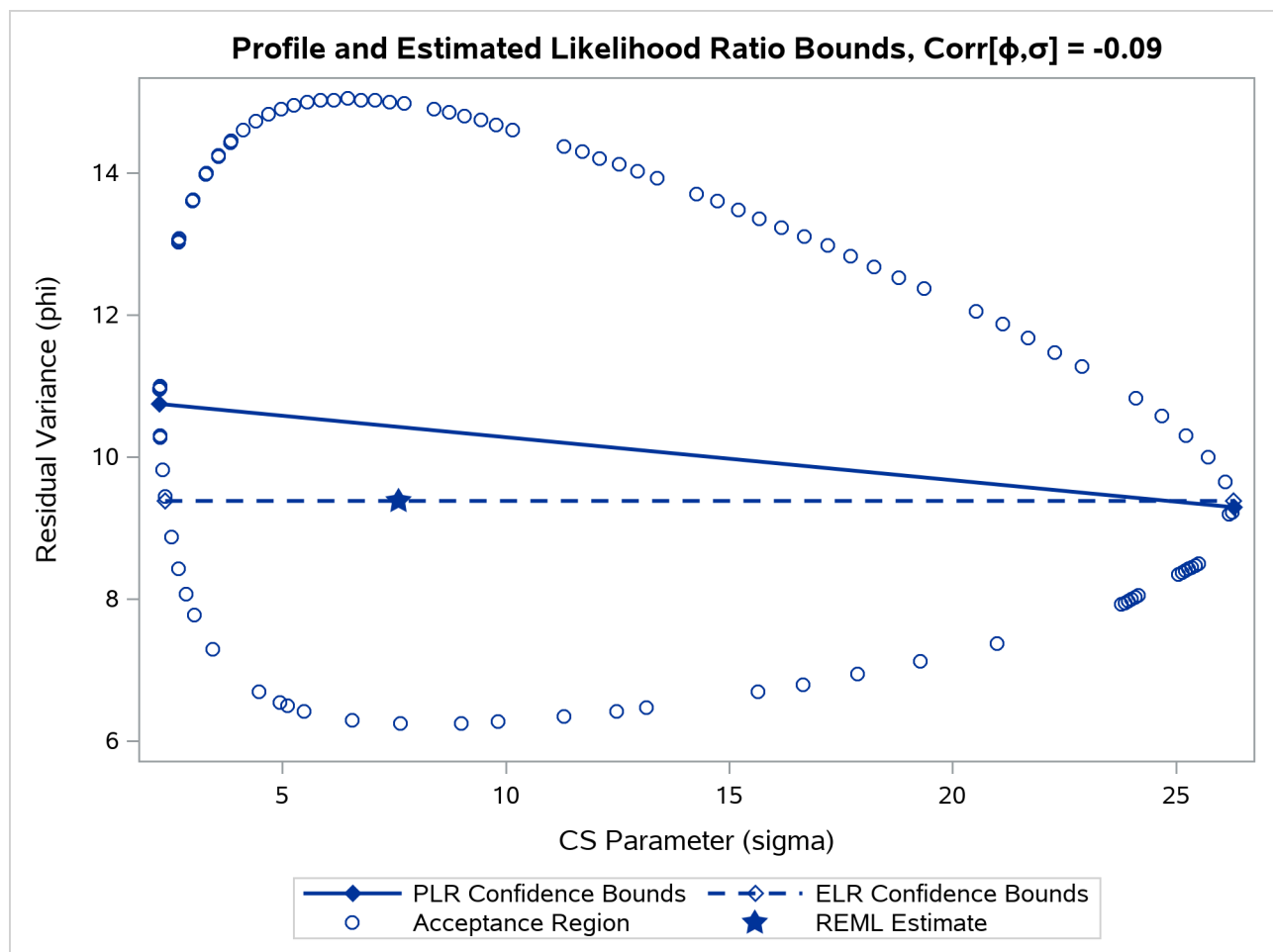
Figure 51.11 PLR and ELR Intervals, Small Correlation between Parameters
