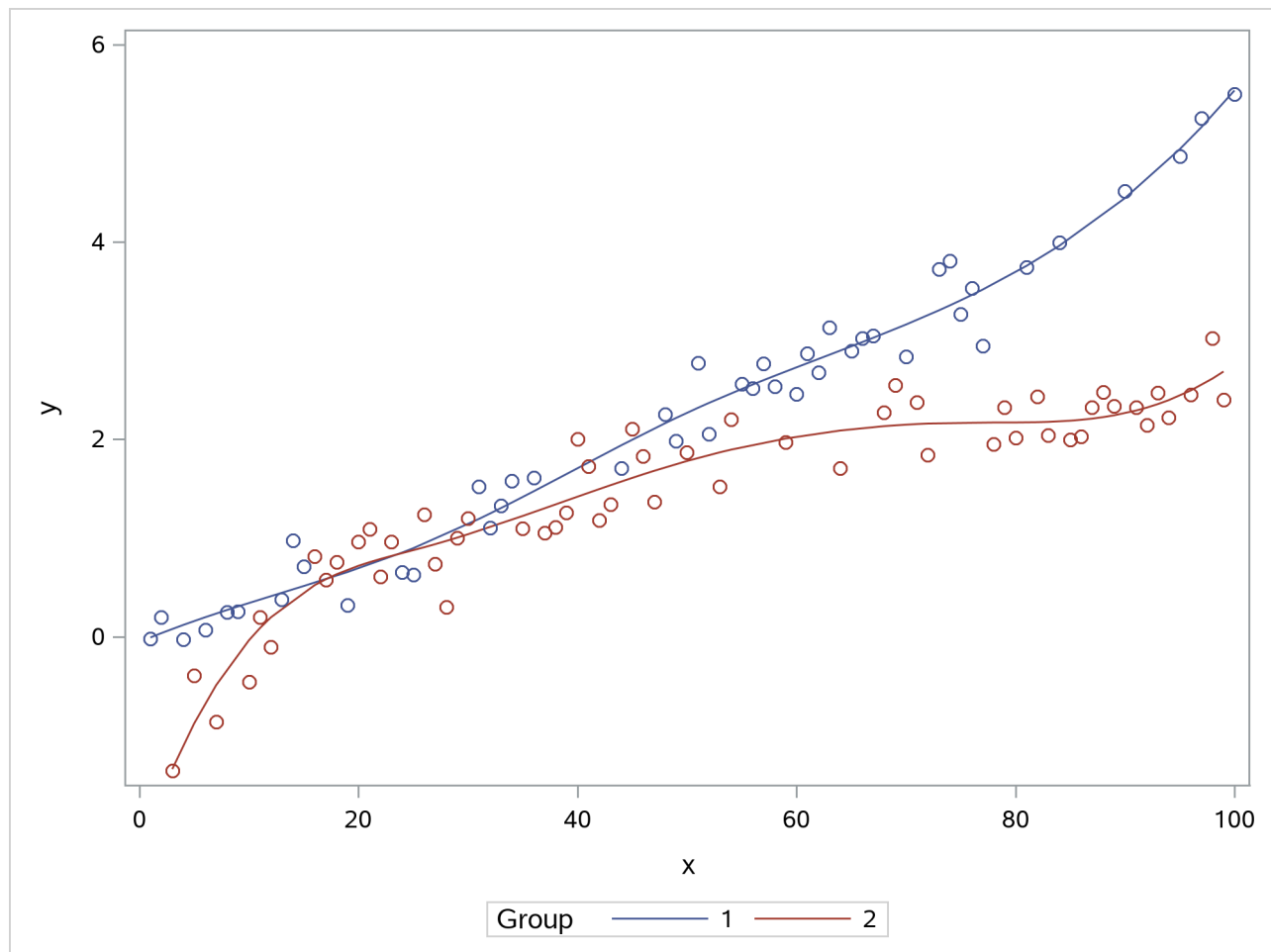
Output 51.15.3 Observed and Predicted Values by Group
