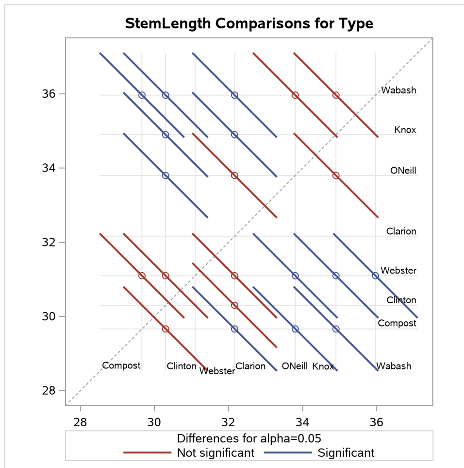
Figure 51.29 Diffogram with NOABS and CENTER Options
