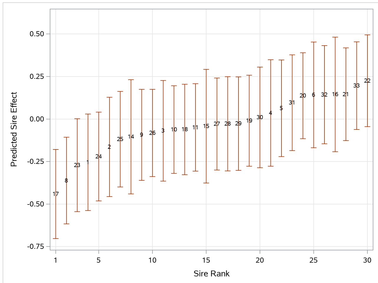
Output 51.11.6 Ranked Predicted Sire Effects and Prediction Standard Errors
