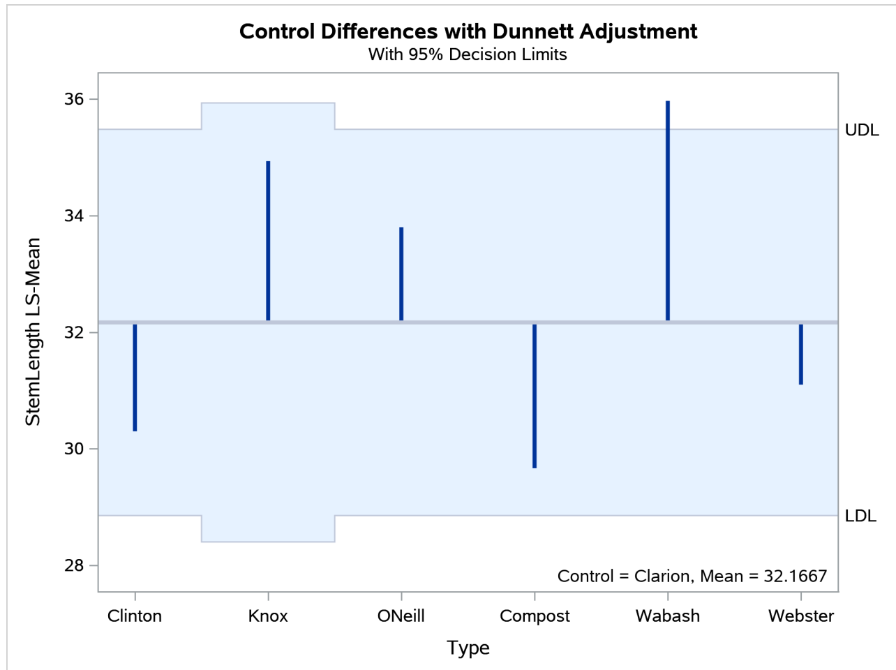
Figure 51.31 LS-Means Plot of Differences against a Control
