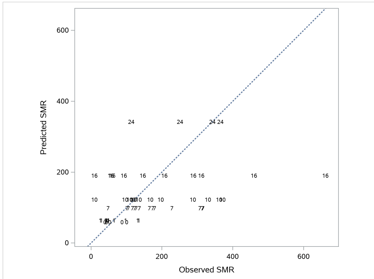
Output 51.3.12 Observed and Predicted SMRs in Poisson GLM
