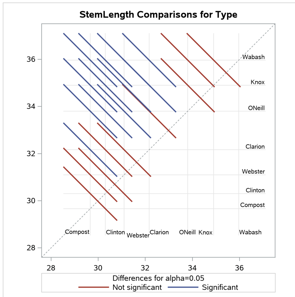
Figure 51.28 LS-Means Plot of Pairwise Differences
