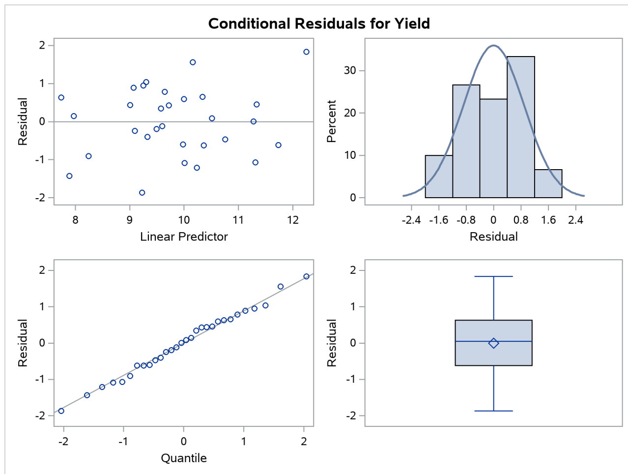
Figure 51.19 Conditional Residuals
