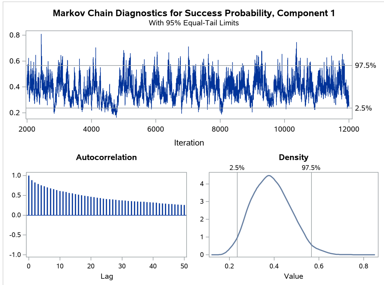
Figure 45.5 Trace Panel for Success Probability in First Component
