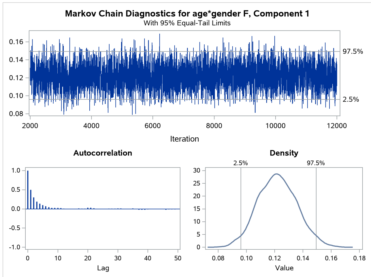
Figure 45.13 Trace Panels for Gender-Specific Slopes
