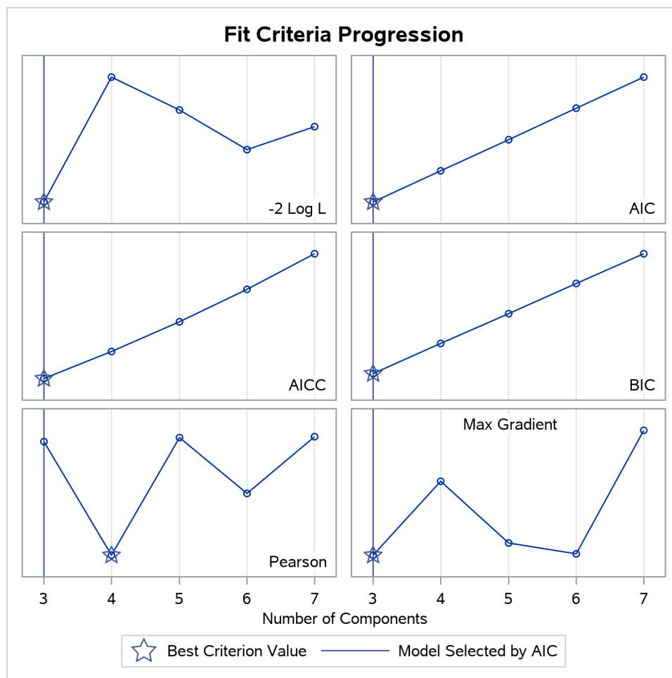
Figure 45.16 Criterion Panel Plot for Model Selection Assuming Unequal Variances
