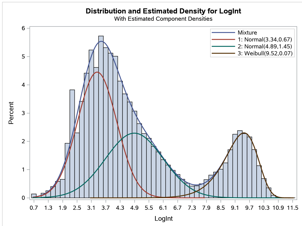
Output 45.2.5 Observed and Estimated Densities in the Three-Component Model
