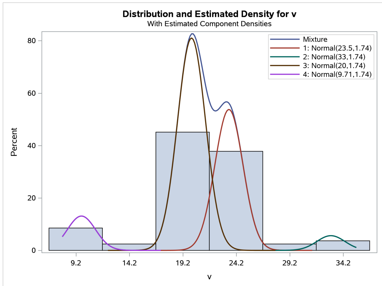
Figure 45.18 Density Plot for Best (Four-Component) Model Assuming Equal Variances
