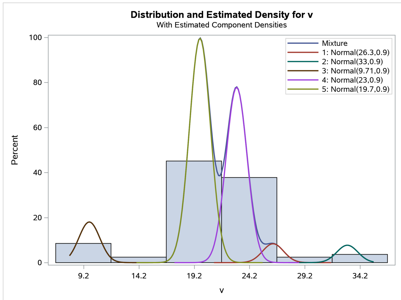
Figure 45.20 Density Plot for Roeder's Analysis
