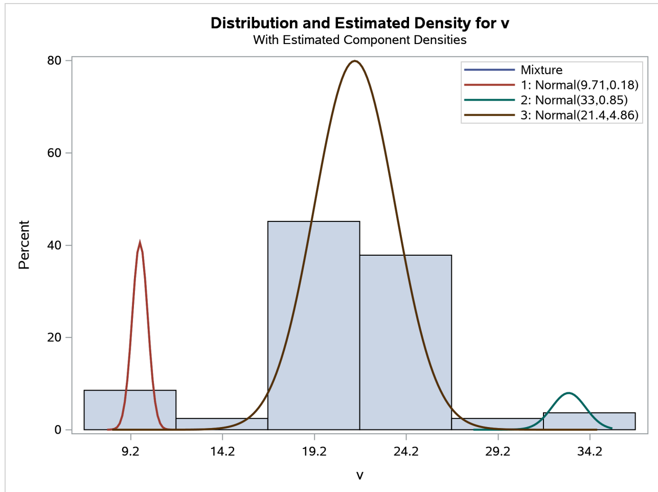
Figure 45.15 Density Plot for Best (Three-Component) Model Assuming Unequal Variances
