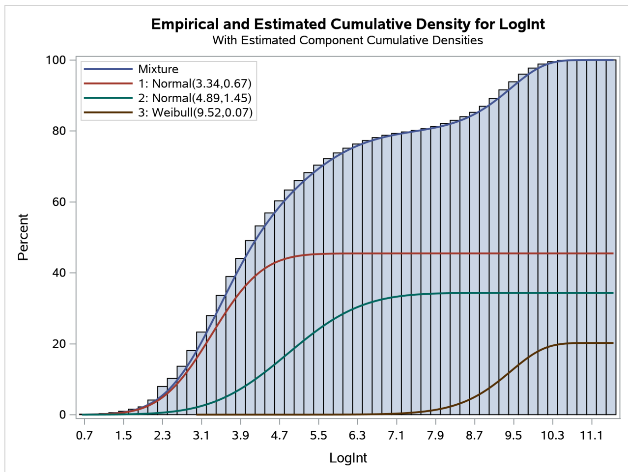
Output 45.2.6 Observed and Estimated Cumulative Densities in the Three-Component Model
