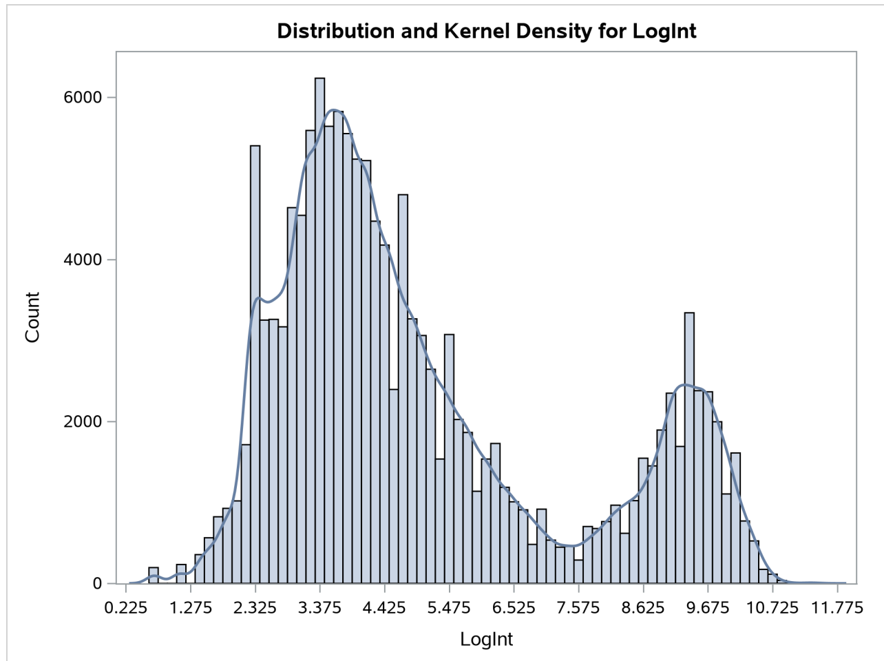
Output 45.2.1 Histogram and Kernel Density for LogInt
