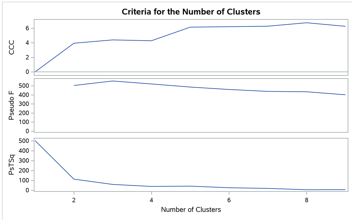
Output 39.3.12 Criteria for the Number of Clusters for Clustering Clusters from Ward's Method
