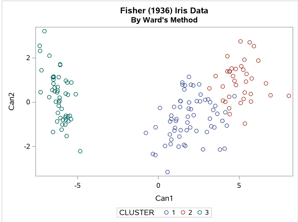
Output 39.3.4 Scatter Plot of Clusters for METHOD=WARD
