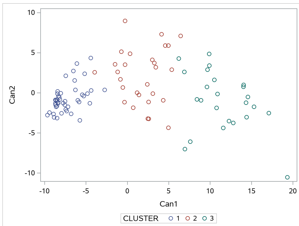
Figure 39.5 Plot of Canonical Variables and Cluster for Three Clusters
