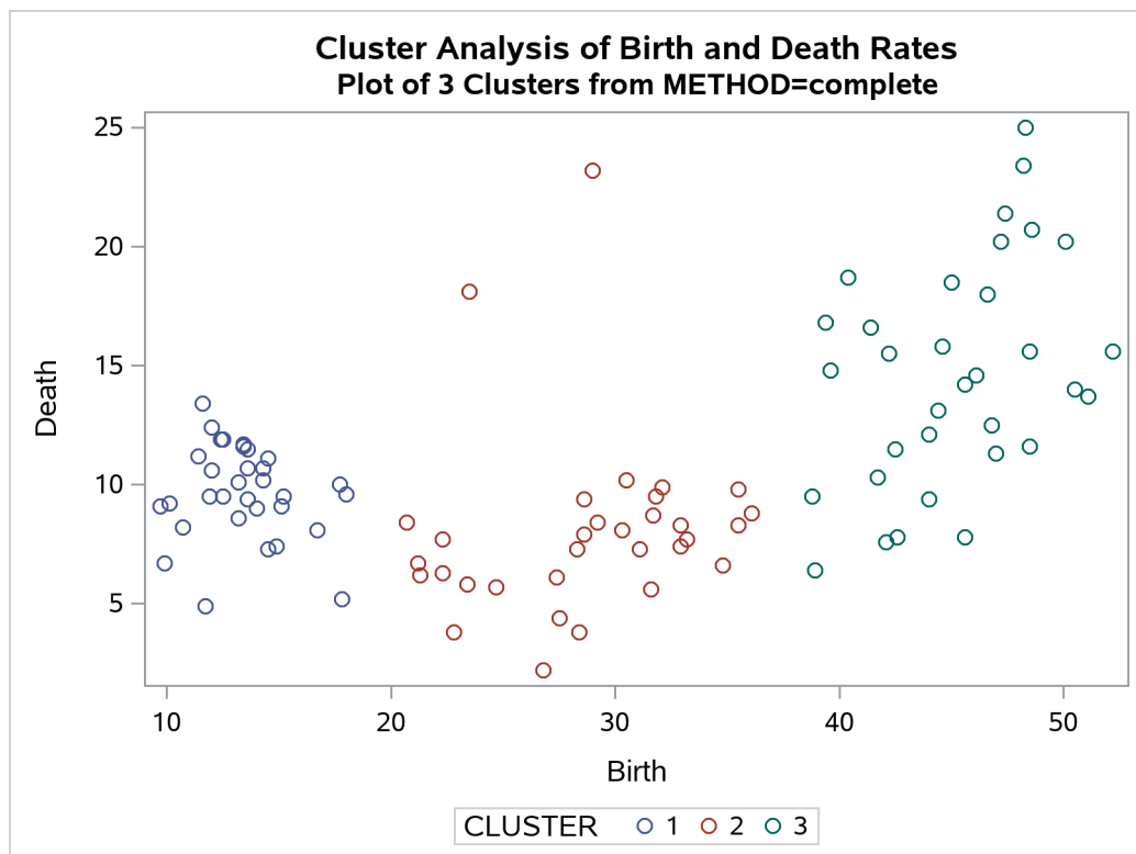
Output 39.2.7 Plot of Clusters for METHOD=COMPLETE
