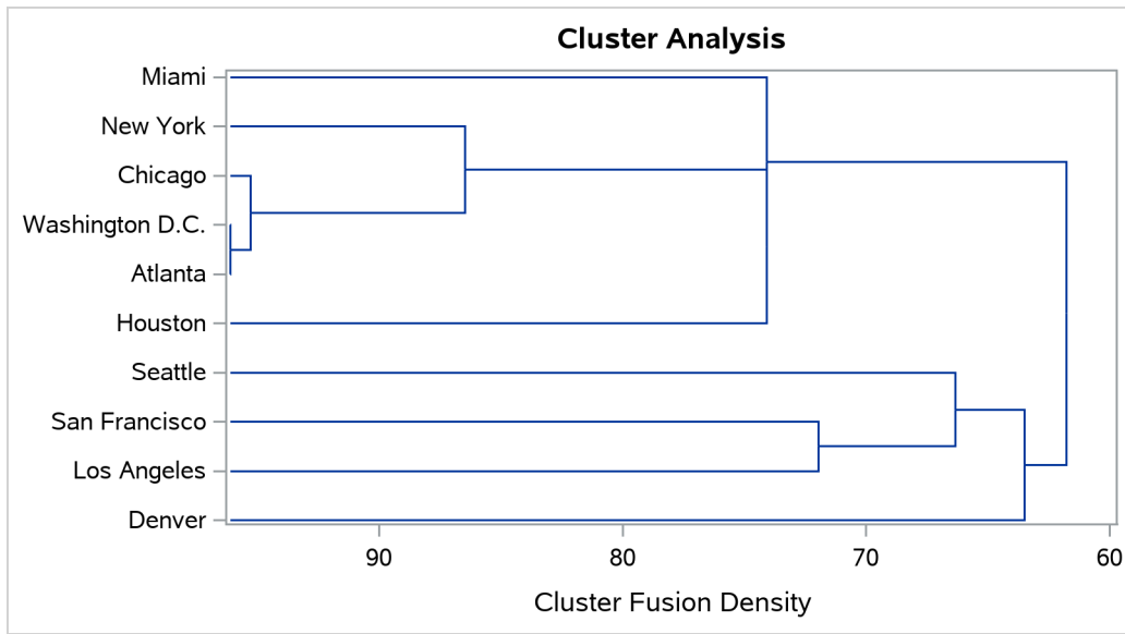
Output 39.1.7 Dendrogram Using METHOD=DENSITY K=3
