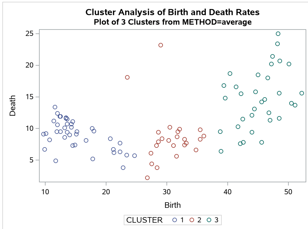
Output 39.2.3 Plot of Three Clusters: METHOD=AVERAGE
