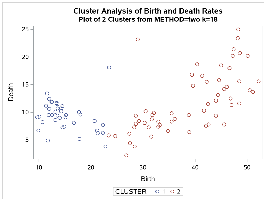
Output 39.2.14 Plot of Clusters for METHOD=TWOSTAGE K=18
