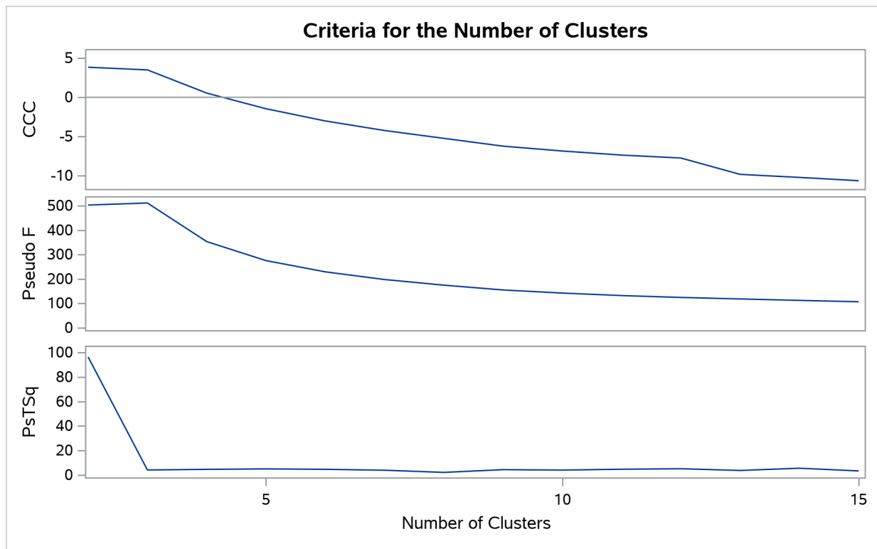
Output 39.3.6 Criteria for the Number of Clusters with METHOD=TWOSTAGE
