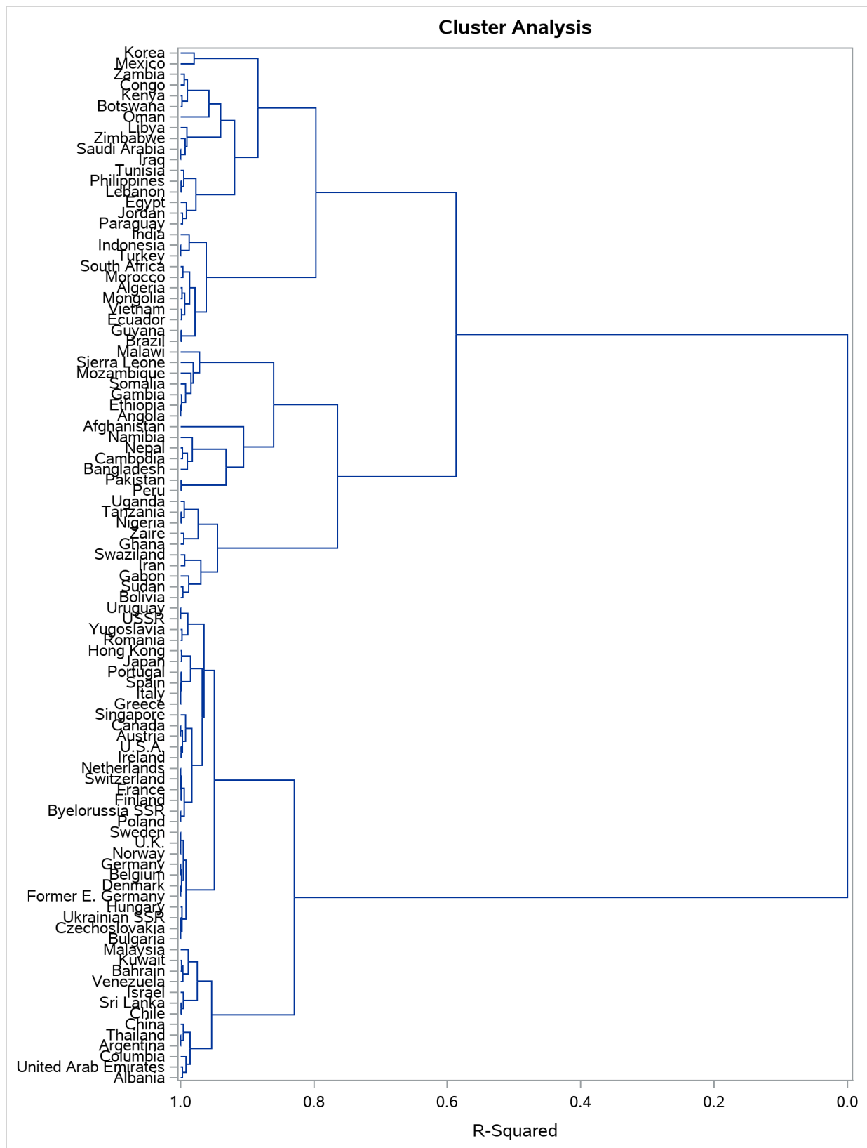
Figure 39.4 Dendrogram of Clusters versus R-Square Values
