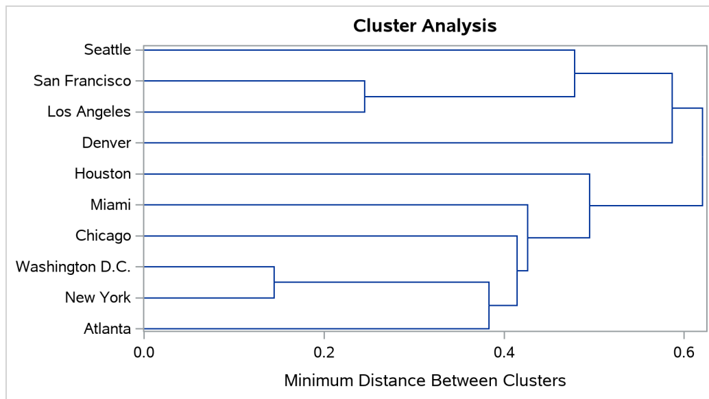
Output 39.1.9 Dendrogram Using METHOD=SINGLE
