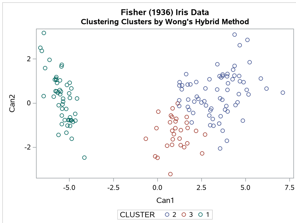
Output 39.3.17 Scatter Plot for Clustering Clusters using Wong's Hybrid Method
