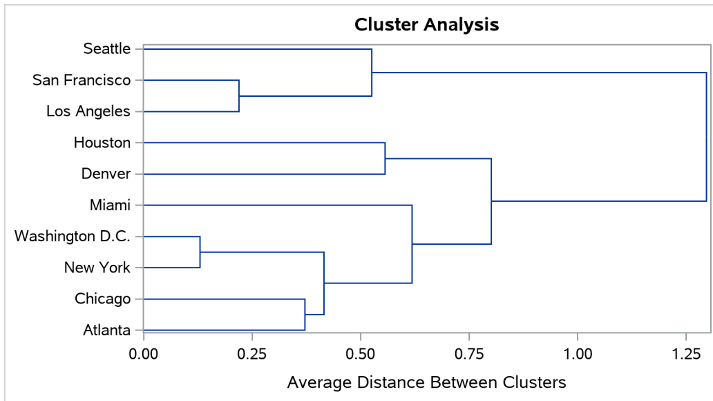
Output 39.1.3 Dendrogram Using METHOD=AVERAGE
