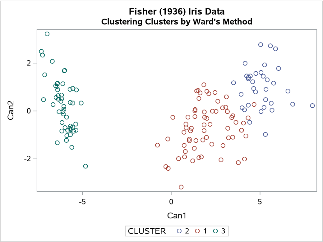
Output 39.3.14 Scatter Plot for Clustering Clusters using Ward's Method
