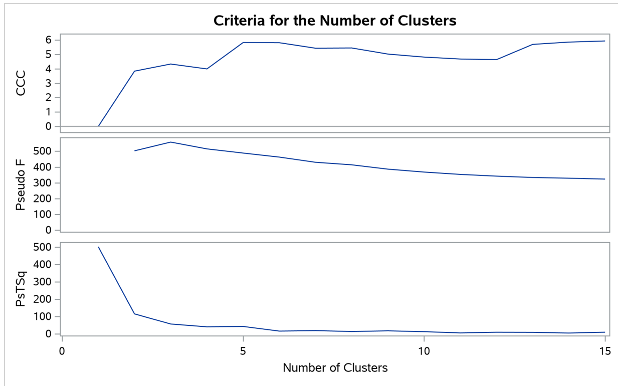
Output 39.3.2 Criteria for the Number of Clusters with METHOD=WARD
