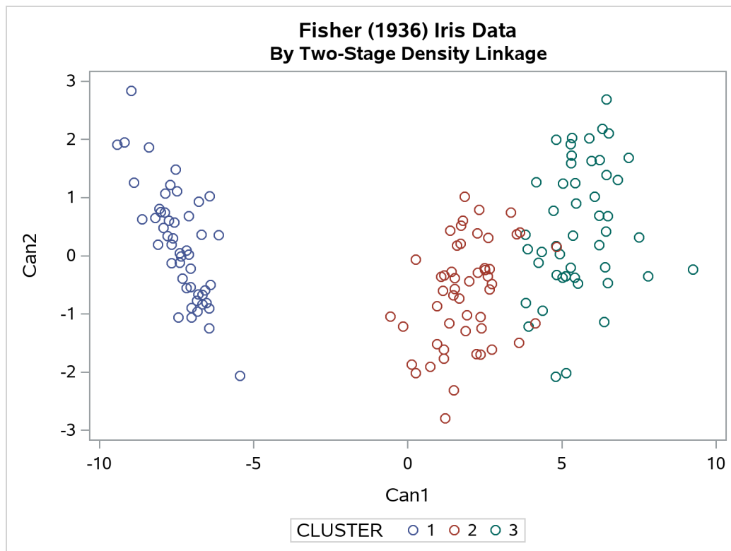
Output 39.3.8 Scatter Plot of Clusters for METHOD=TWOSTAGE
