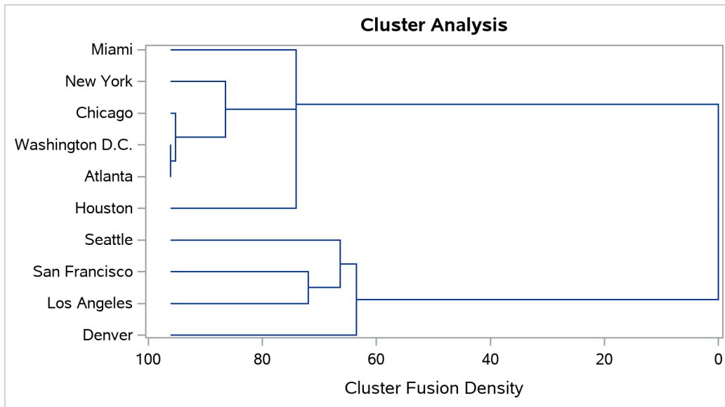
Output 39.1.11 Dendrogram Using METHOD=TWOSTAGE K=3
