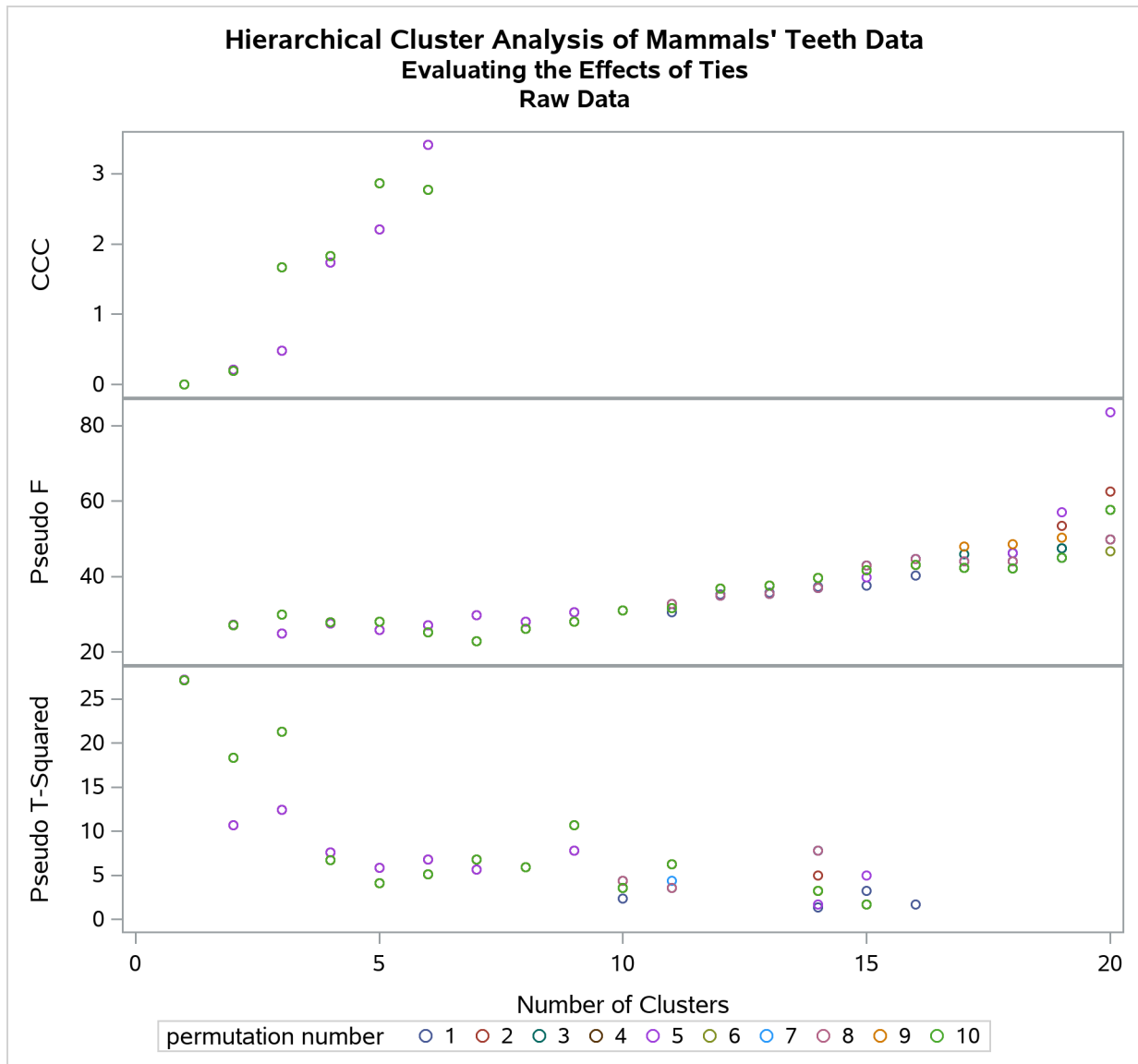
Output 39.4.3 Analysis of 10 Random Permutations of Raw Mammals' Teeth Data
