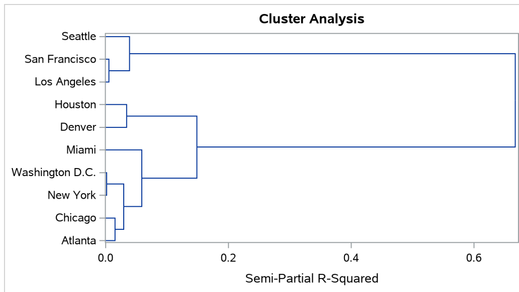
Output 39.1.13 Dendrogram Using METHOD=WARD
