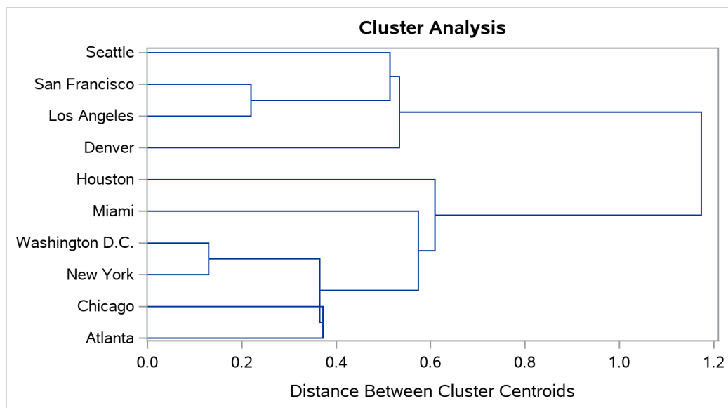
Output 39.1.5 Dendrogram Using METHOD=CENTROID
