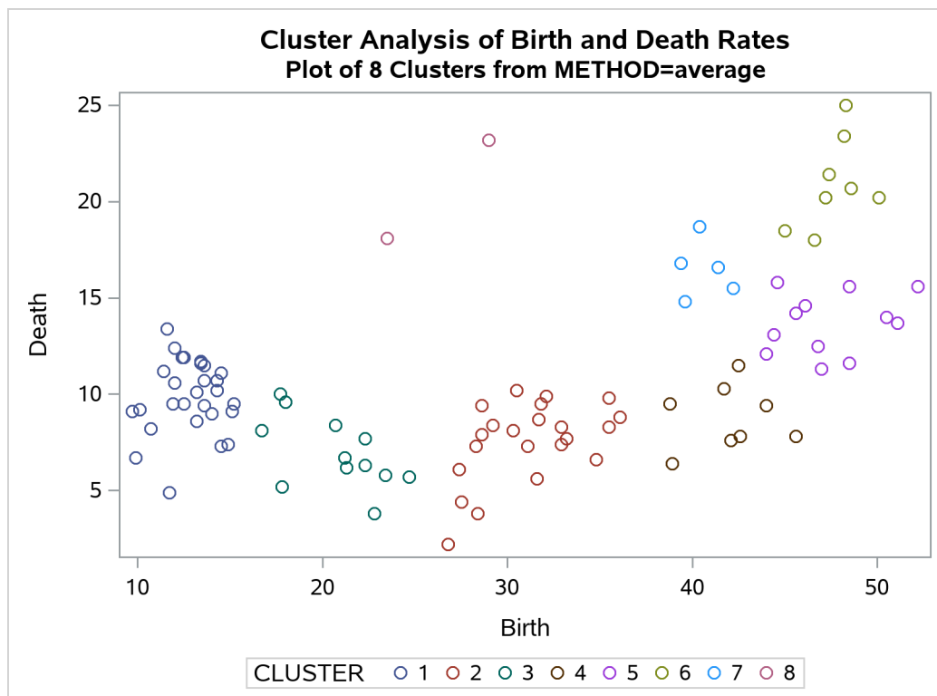
Output 39.2.4 Plot of Eight Clusters: METHOD=AVERAGE
