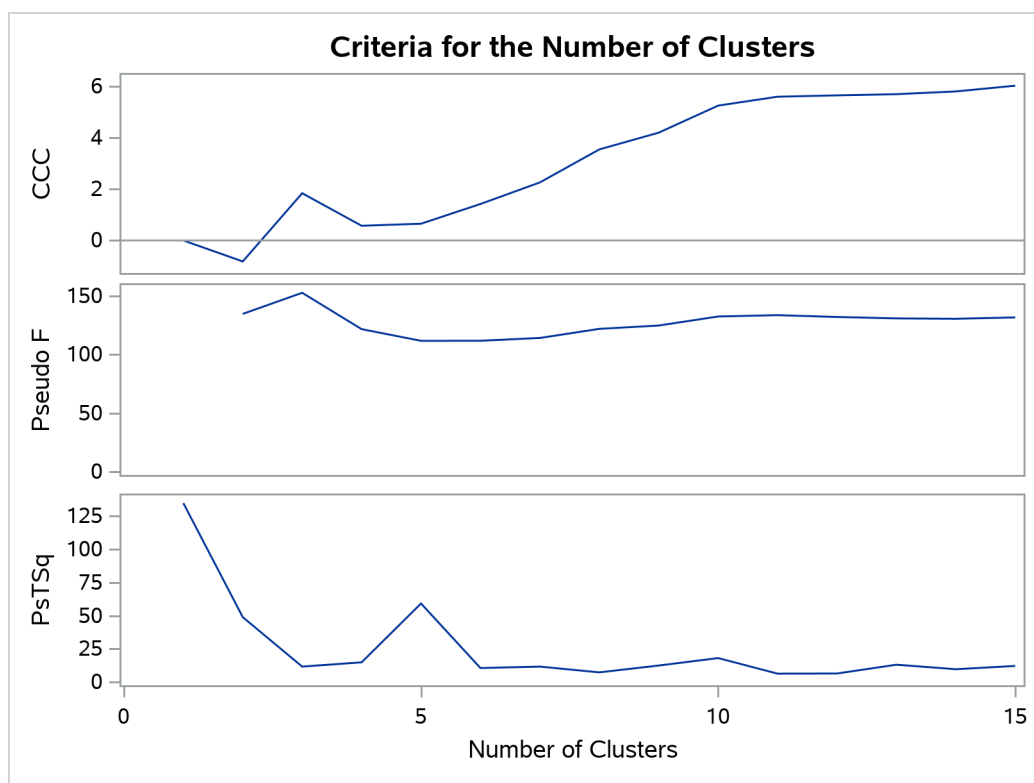
Figure 39.3 Plot of Statistics for Estimating the Number of Clusters
