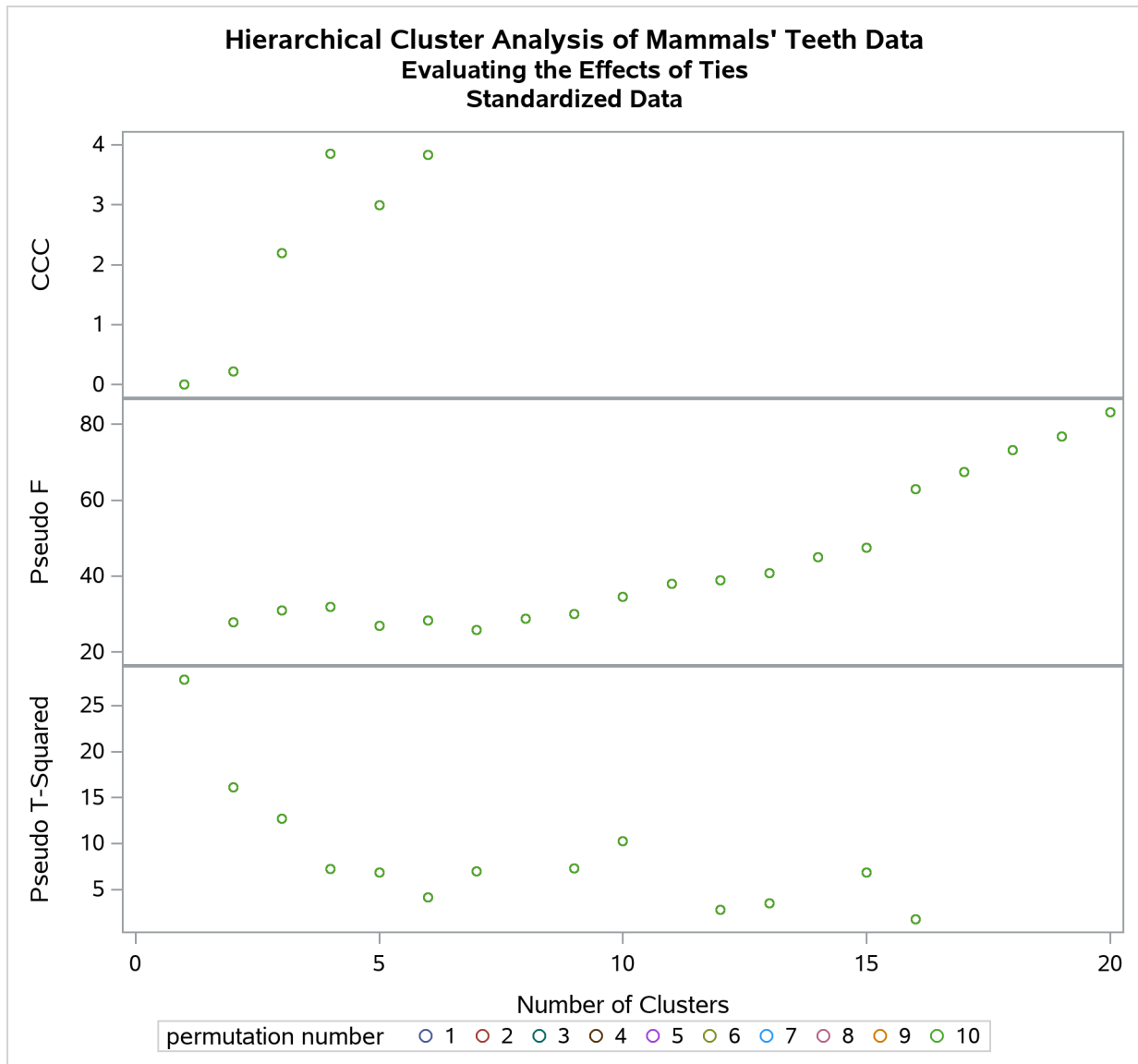
Output 39.4.5 Analysis of 10 Random Permutations of Standardized Mammals' Teeth Data
