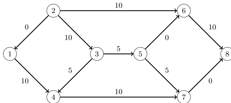
Figure 13.6 Minimum-Cost Network Flow Problem: Optimal Solution
