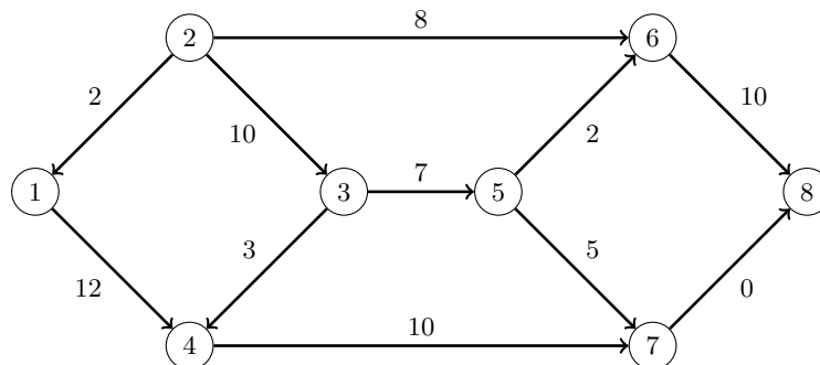
Figure 8.6 Minimum-Cost Network Flow Problem: Optimal Solution (with Budget Constraint)
