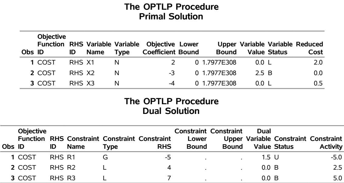
Figure 13.1 Primal and Dual Solution Output
