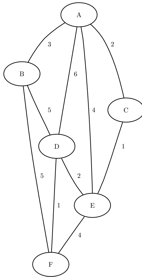
Figure 10.60 A Simple Undirected Graph G
