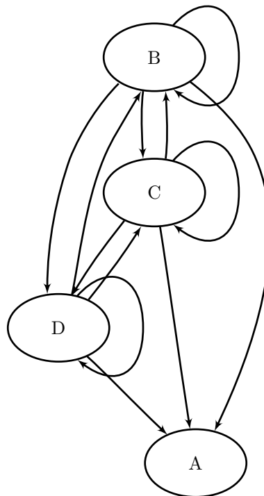
Figure 10.74 Transitive Closure of G
