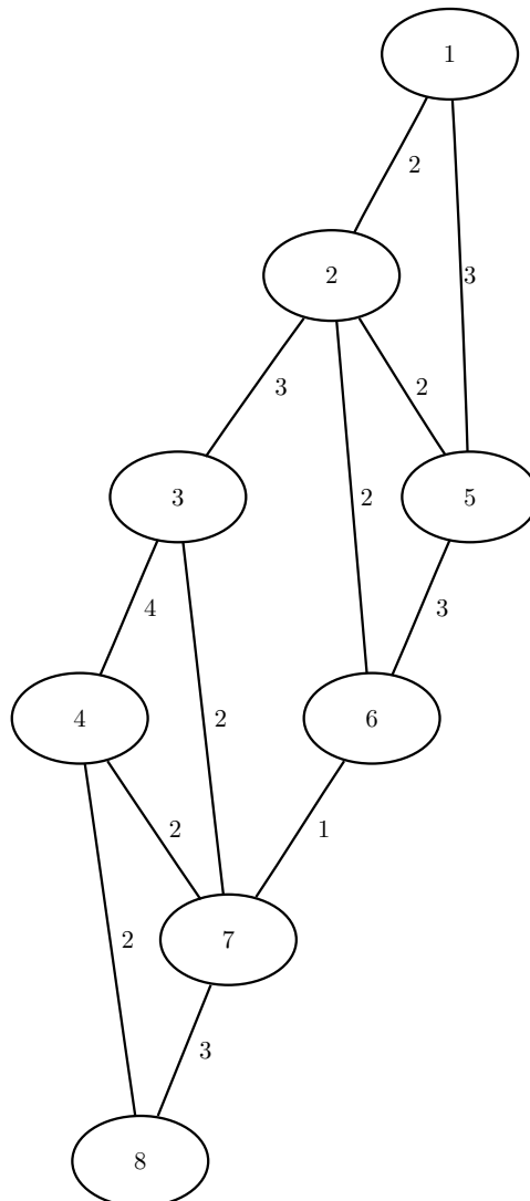
Figure 10.45 A Simple Undirected Graph
