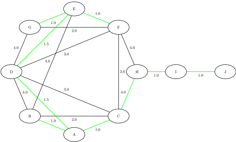
Figure 10.91 Minimum Spanning Tree for Office Computer Network
