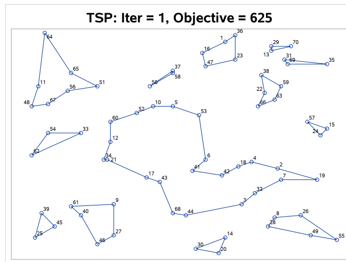
Output 9.4.1 Traveling Salesman Problem Iterative Solution
