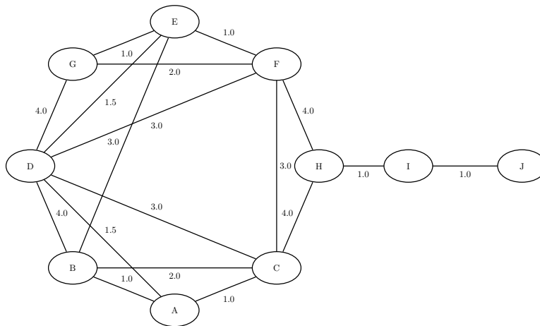
Figure 10.90 Potential Office Computer Network
