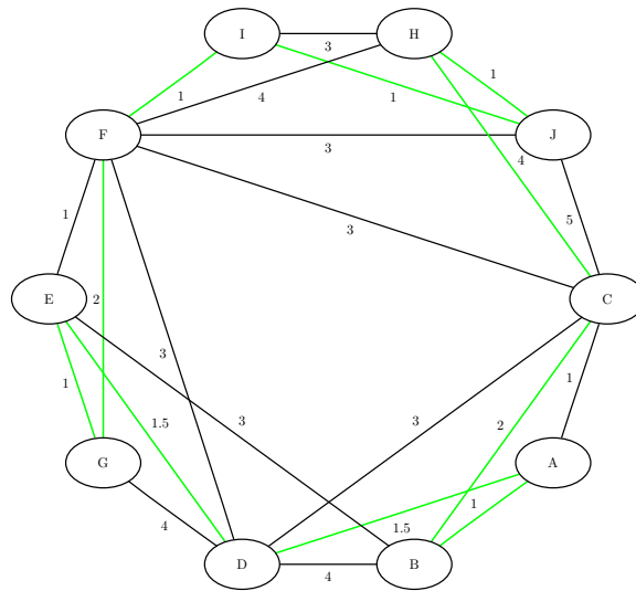
Figure 10.79 Optimal Traveling Salesman Tour
