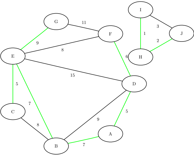
Figure 10.55 Minimum Spanning Forest
