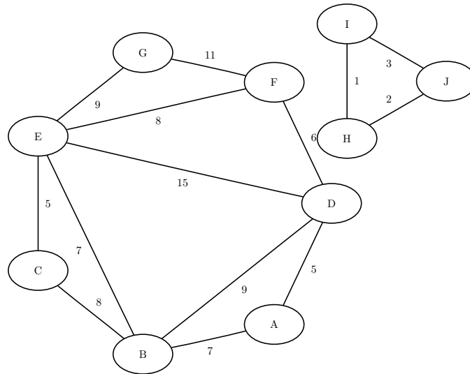
Figure 10.53 A Simple Undirected Graph
