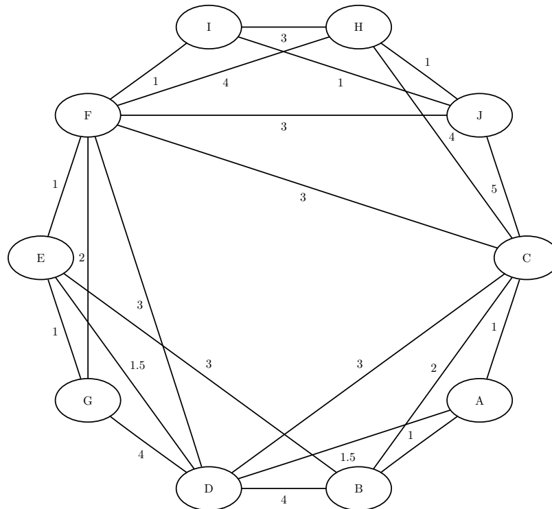
Figure 10.75 A Simple Undirected Graph
