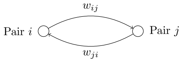
Figure 10.87 Kidney Donor Exchange Network
