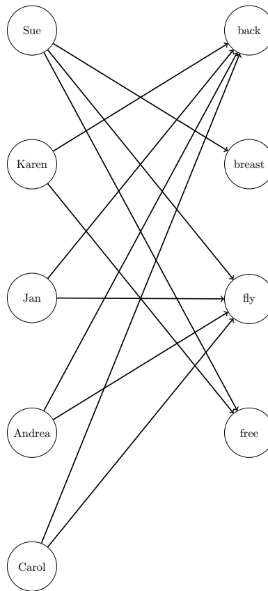
Figure 10.88 Bipartite Graph for Linear Assignment Problem
