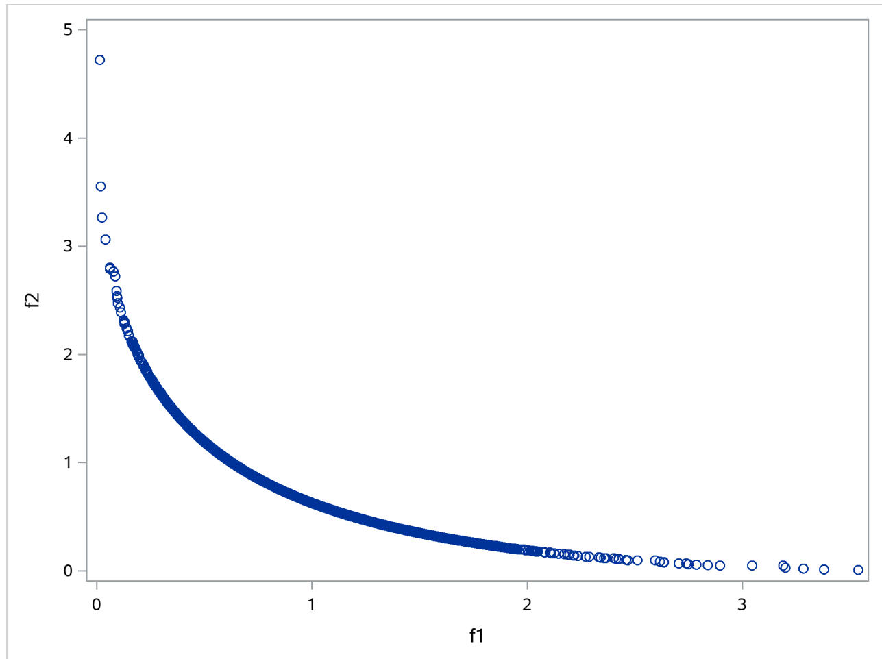
Output 6.7.3 Multiobjective: Plot of Pareto-Optimal Set
