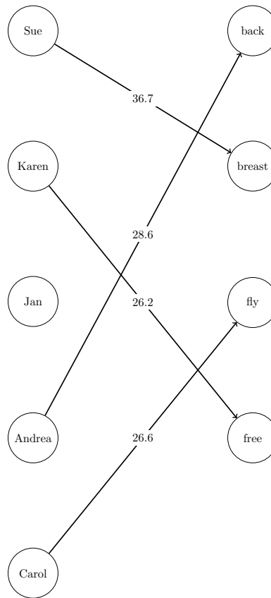
Figure 10.89 Optimal Assignments for Swim Times
