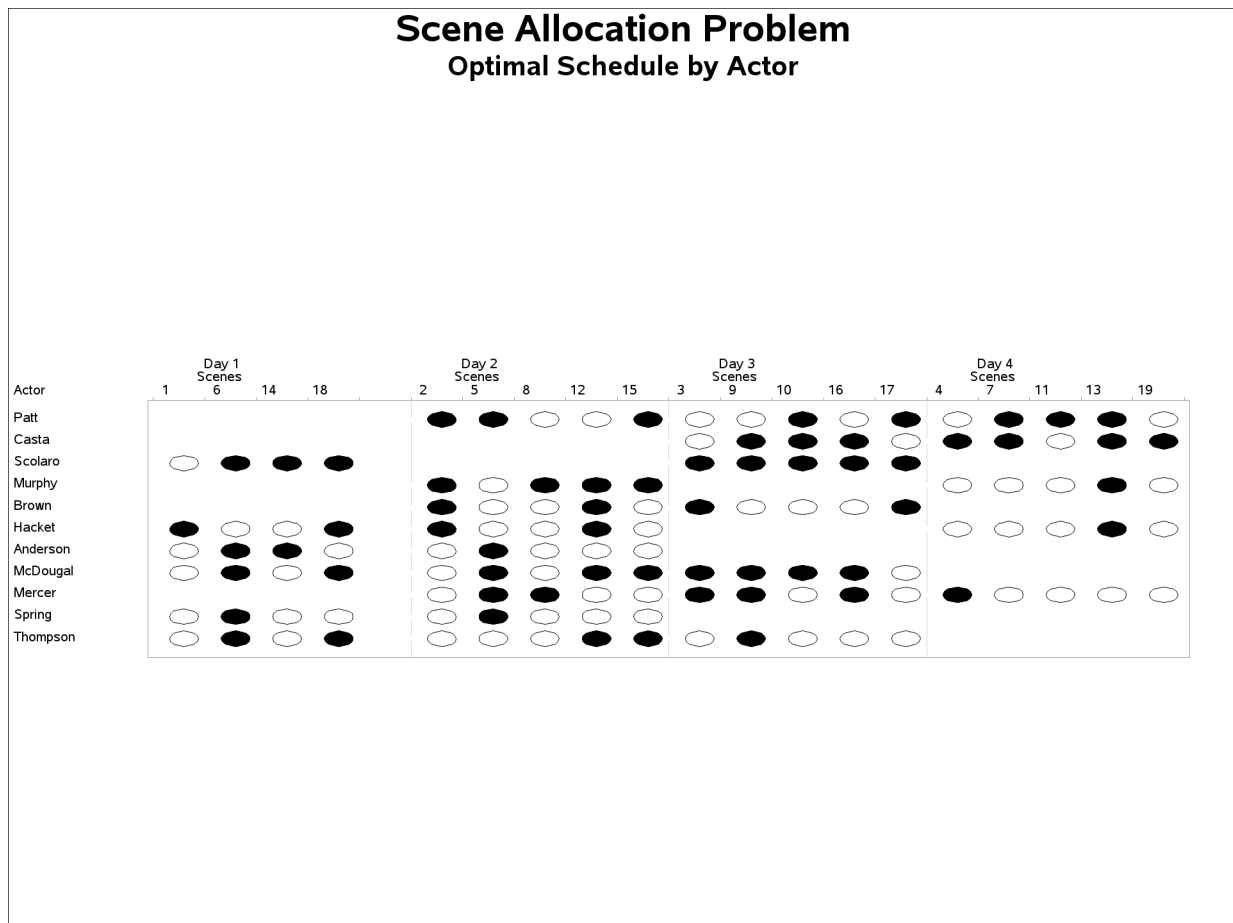
Output 7.6.2 Scene Allocation Problem: Actor Schedules
