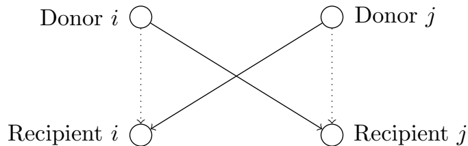
Figure 10.86 Kidney Donor Exchange Two-Way Swap
