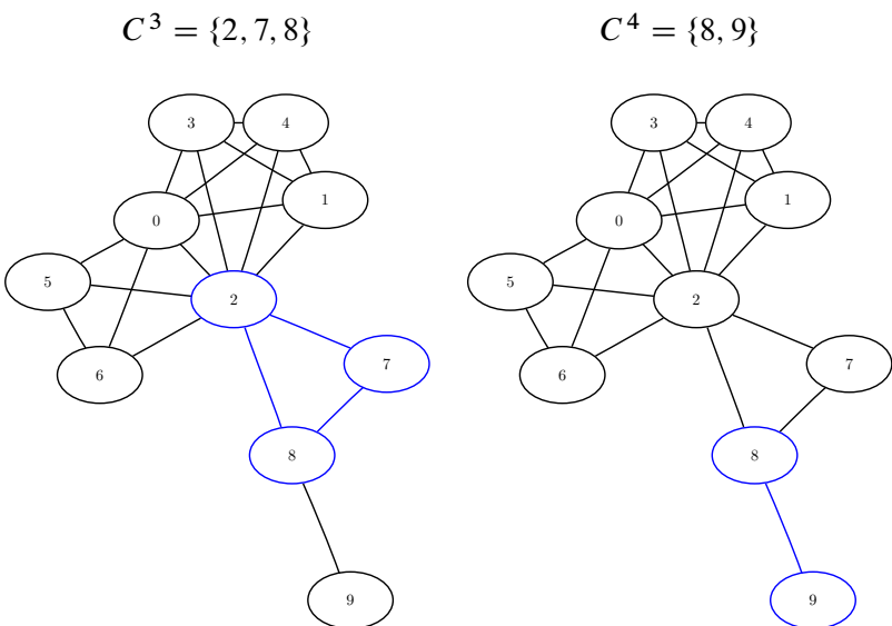
Figure 10.22 Maximal Cliques C^3 and C^4
