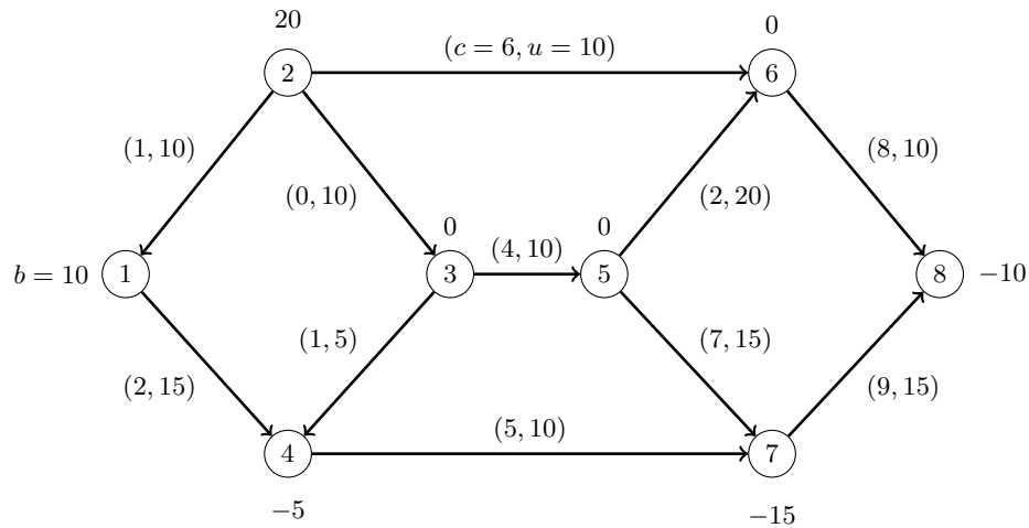
Figure 13.5 Minimum-Cost Network Flow Problem: Data
