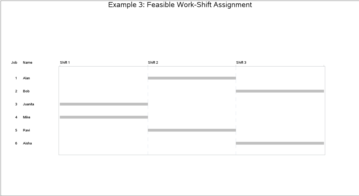
Output 7.3.2 Work-Shift Schedule
