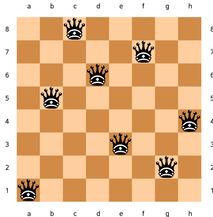
Figure 7.2 A Solution to the Eight Queens Problem
