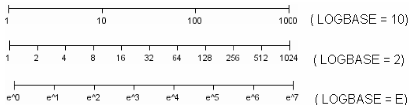
Figure 10.13 Graph Axes with LOGEXPAND
