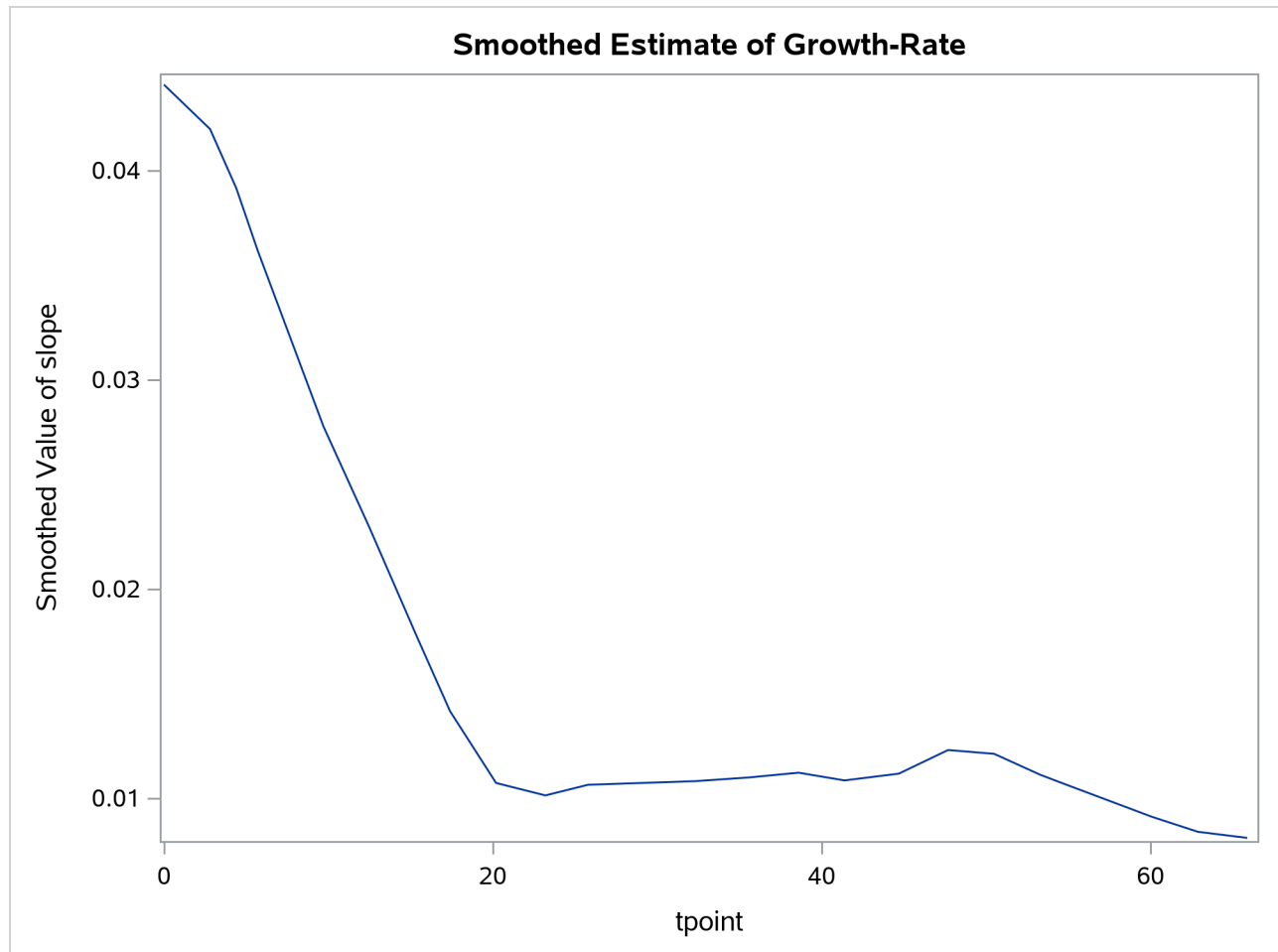
Output 34.5.4 Estimate of the slope Component
