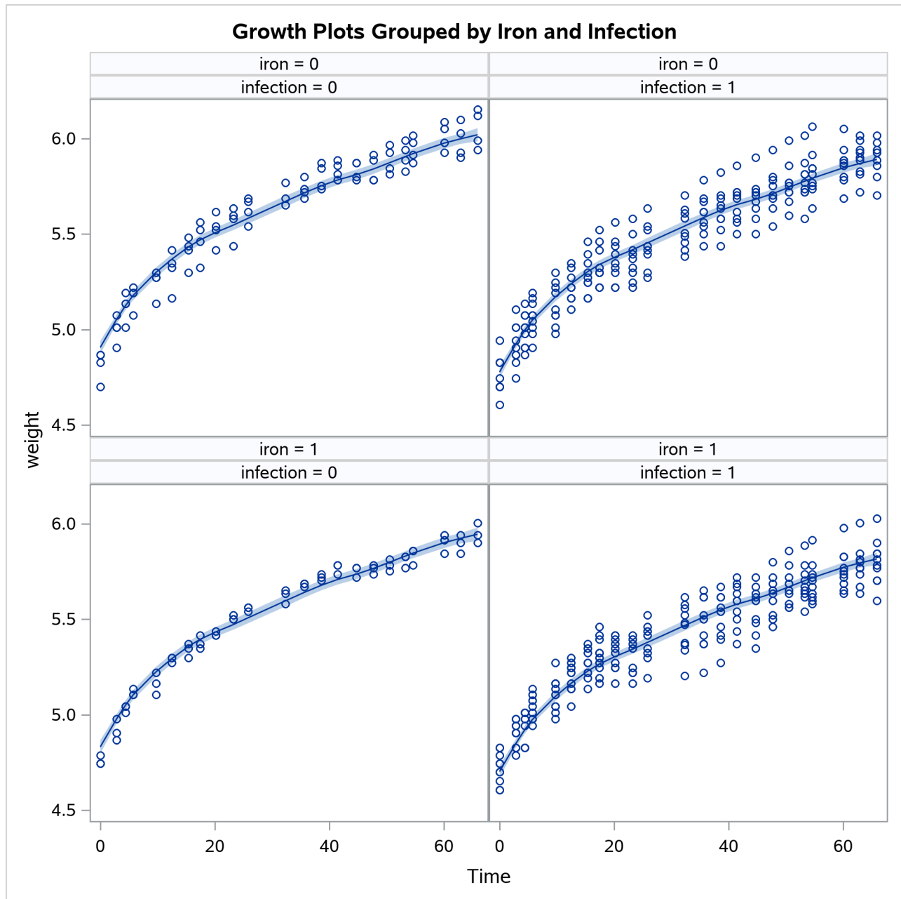
Output 34.4.6 Model 1: Smoothed Model Fit Lines
