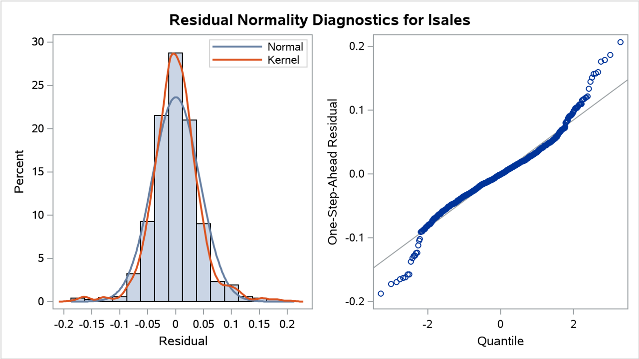
Figure 34.6 Residual Normality Check
