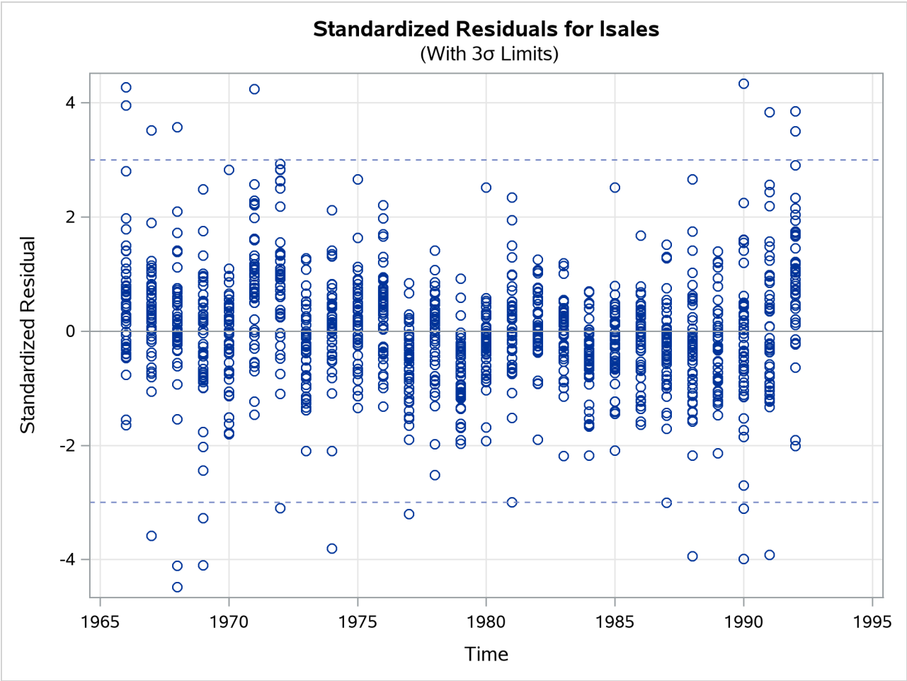
Figure 34.7 Standardized Residuals Plotted against Time
