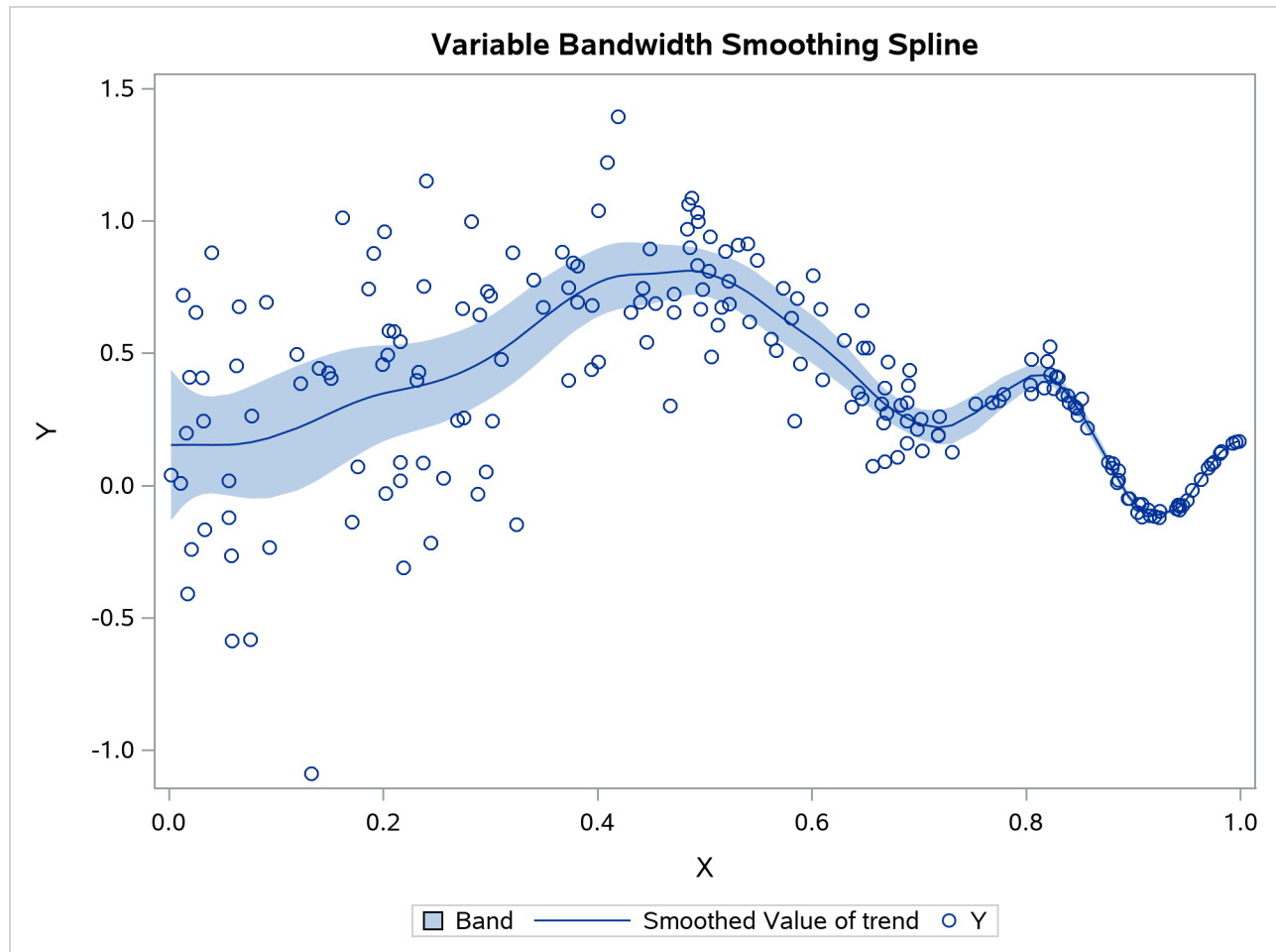
Output 34.9.4 Fitted Trend with 95% Confidence Band
