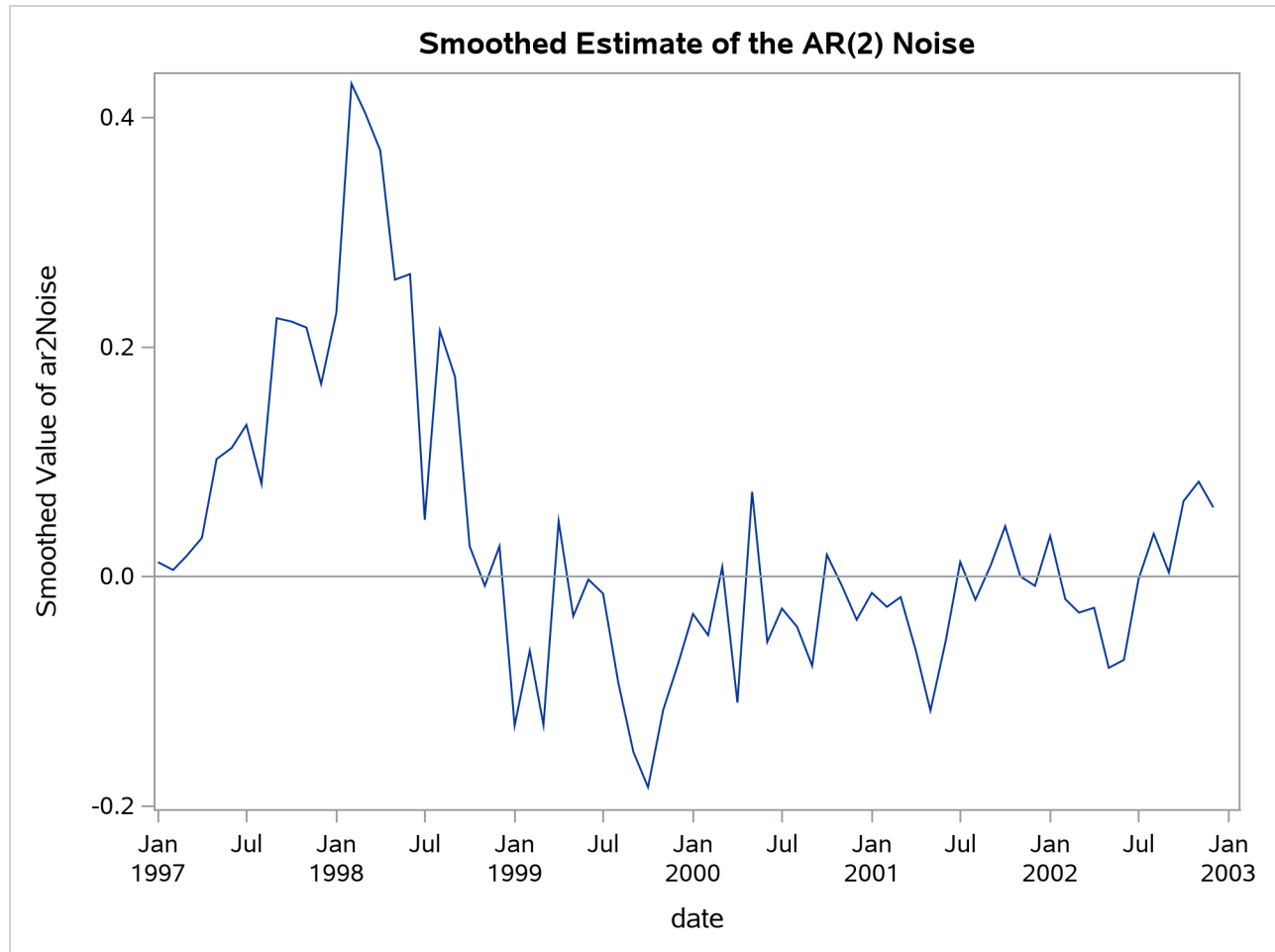
Output 34.6.4 Estimate of the ar2Noise Component
