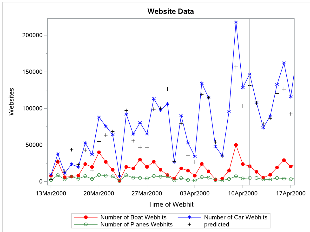
Output 15.4.1 Internet Data Forecast Plots
