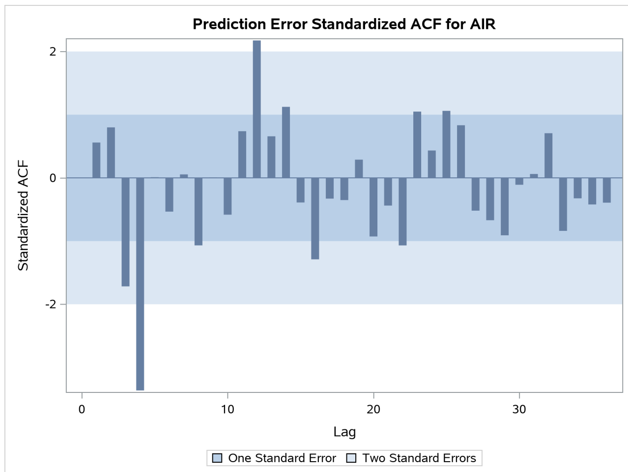
Output 15.5.3 Prediction Error Standardized ACF Plot
