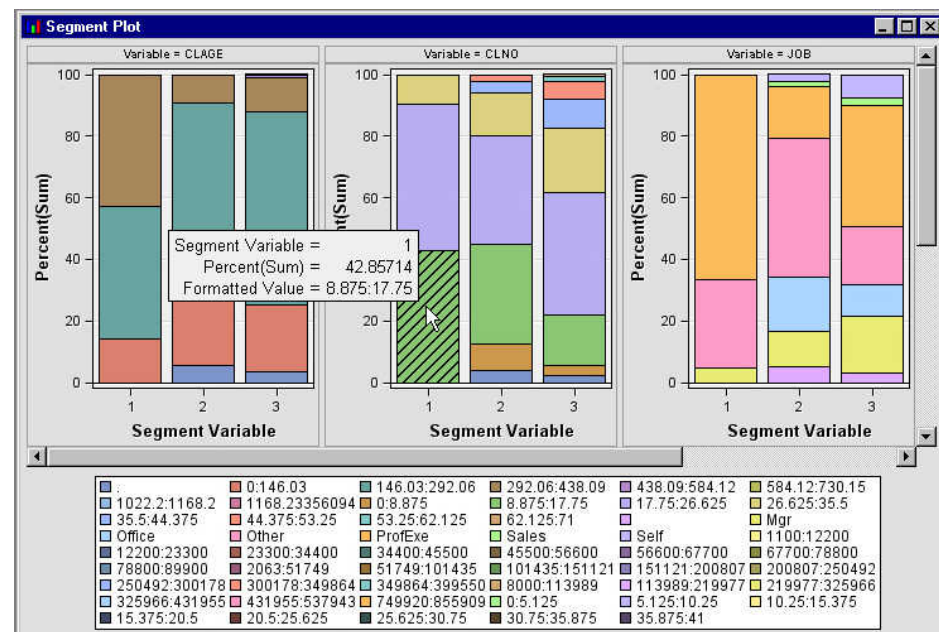
Figure 18.20 Cluster Segment Plot
