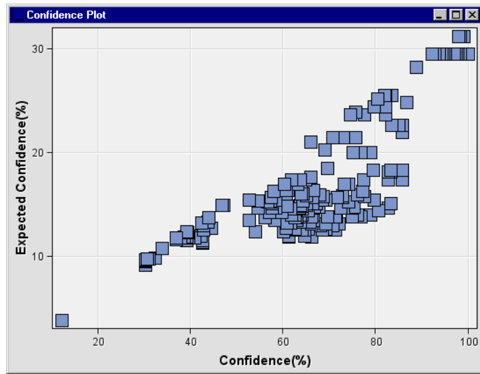
Figure 18.24 Confidence Plot
