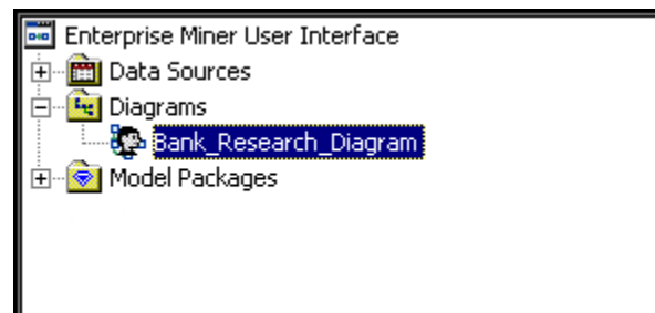
Figure 18.7 Created Diagram
