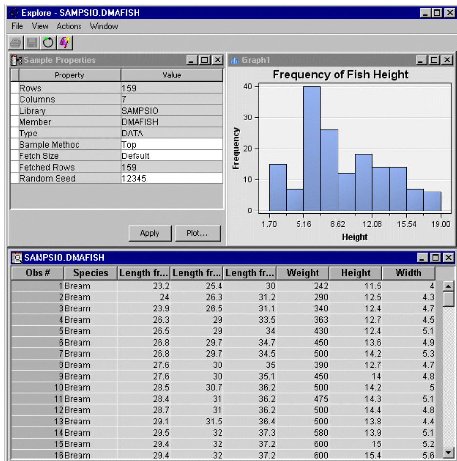
Figure 18.35 Explore Window
