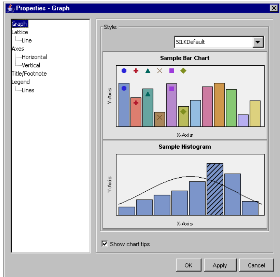
Figure 18.29 Graph
