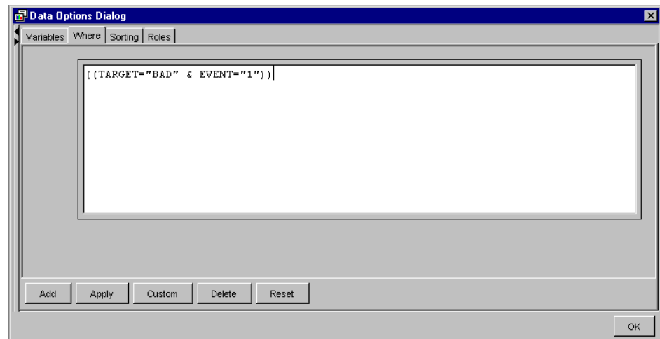
Figure 18.26 Where Tab
