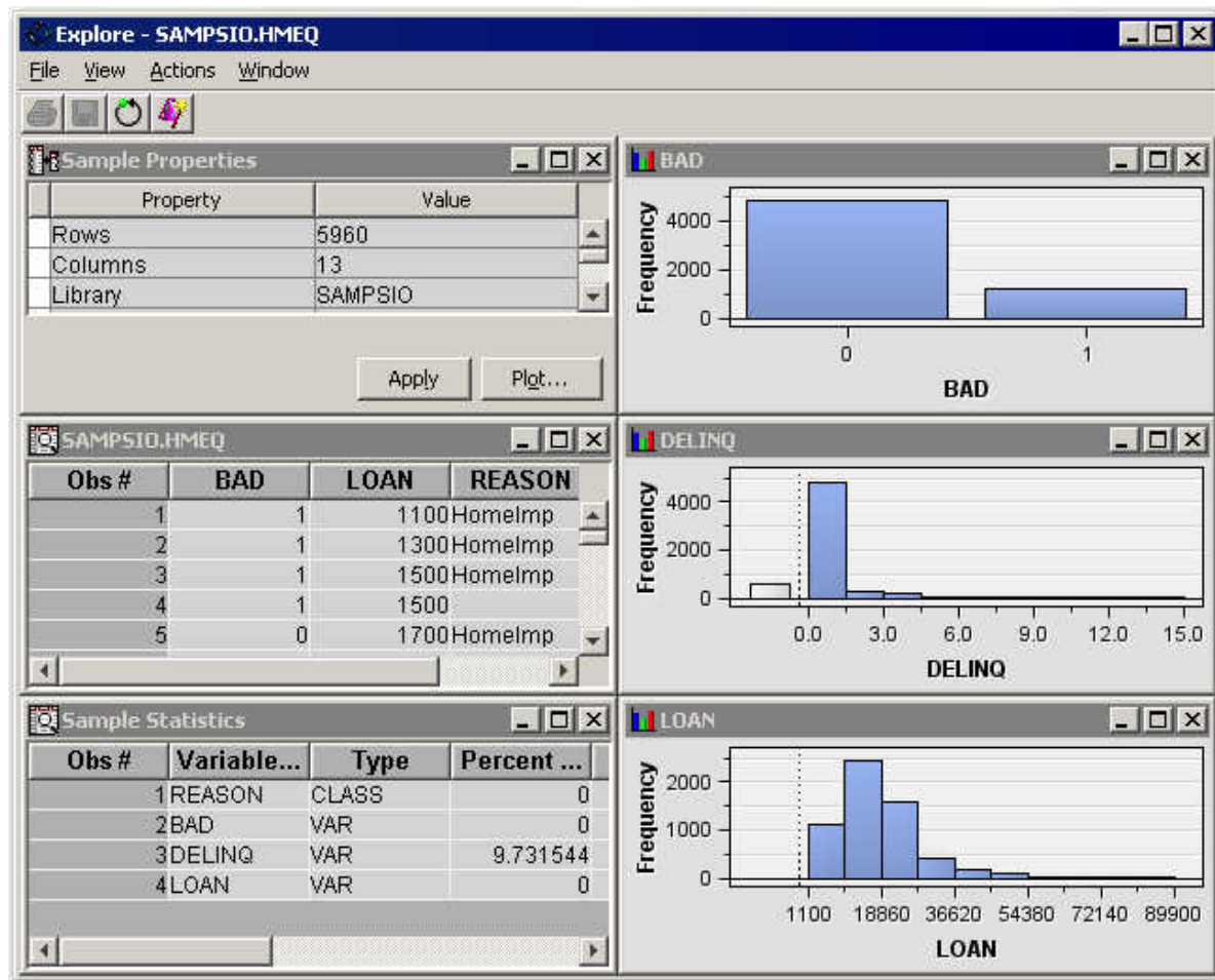
Figure 18.43 Explore Window
