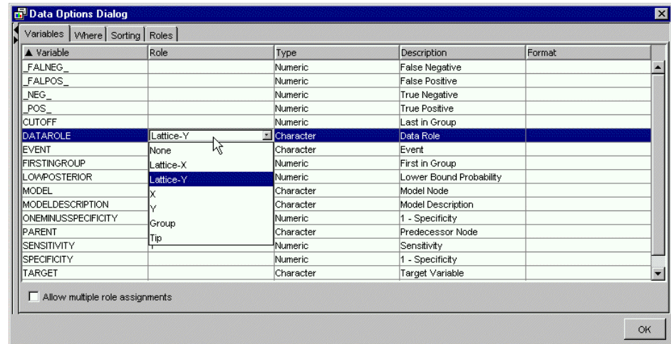
Figure 18.25 Variables Tab
