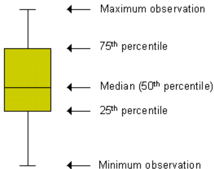
Figure 18.15 Elements
