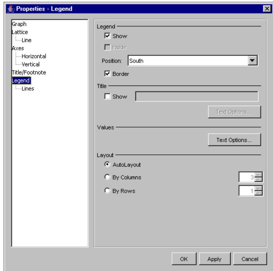
Figure 18.33 Legend
