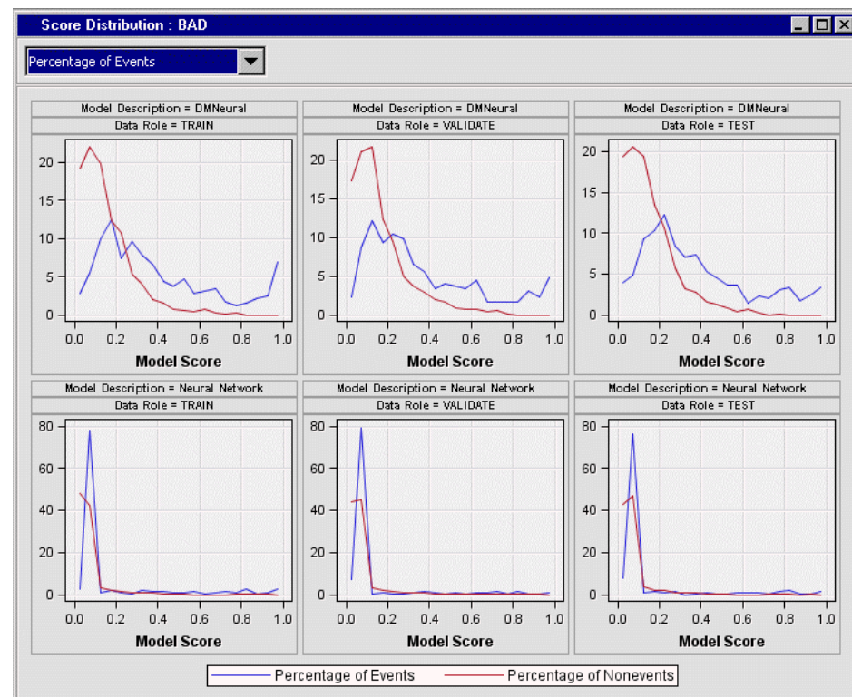
Figure 18.18 Score Distribution
