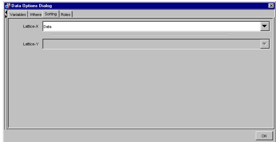
Figure 18.27 Sorting Tab
