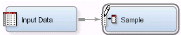
Figure 18.12 Drag Pointer
