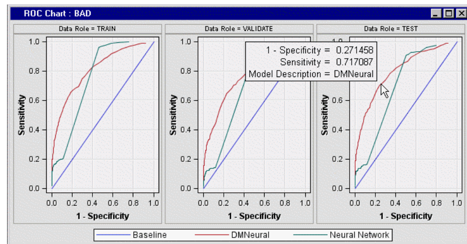
Figure 18.19 Receiver Operating Characteristic Chart
