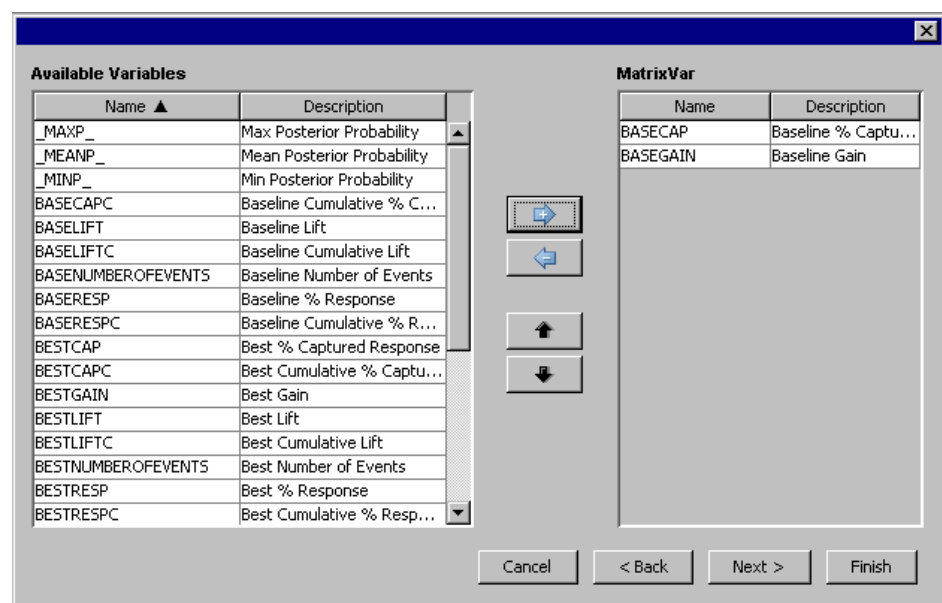
Figure 18.37 Select Variables
