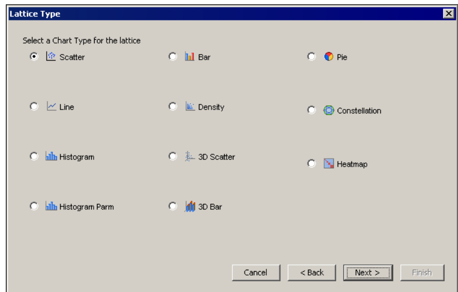
Figure 18.38 Lattice Type
