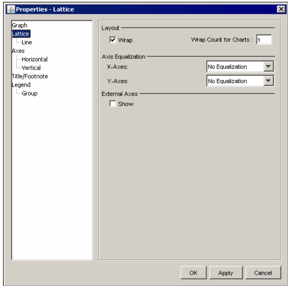
Figure 18.30 Lattice
