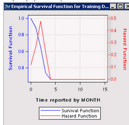
Figure 99.6 Empirical Survival Function Using Expanded Monthly Data
