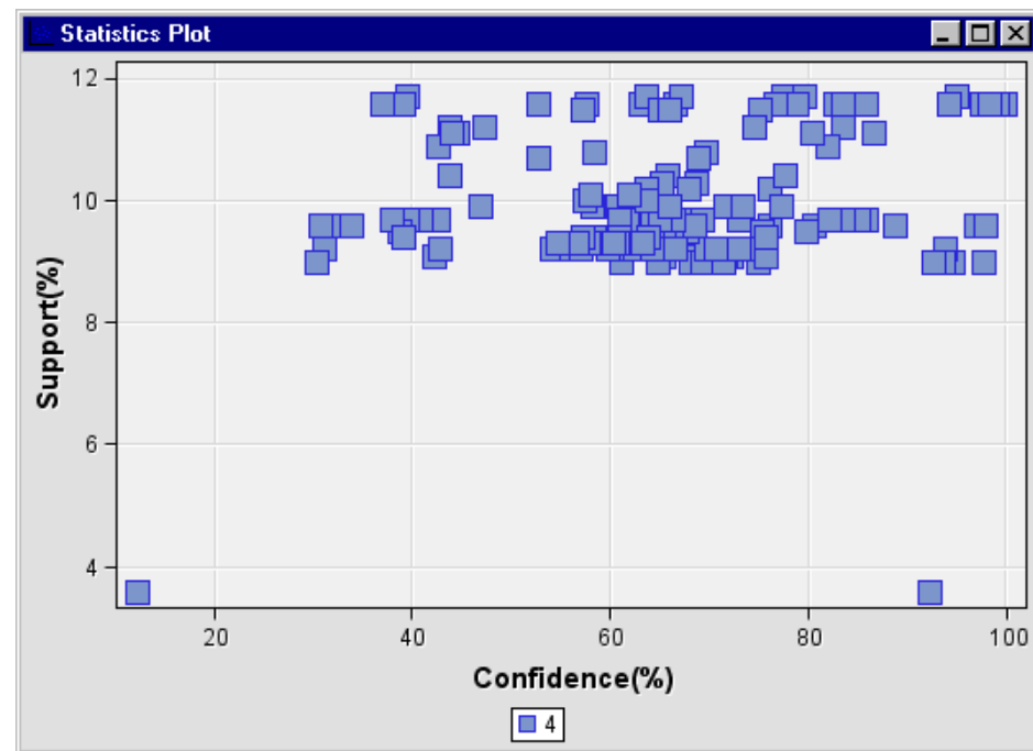
Figure 18.23 Statistics Plot
