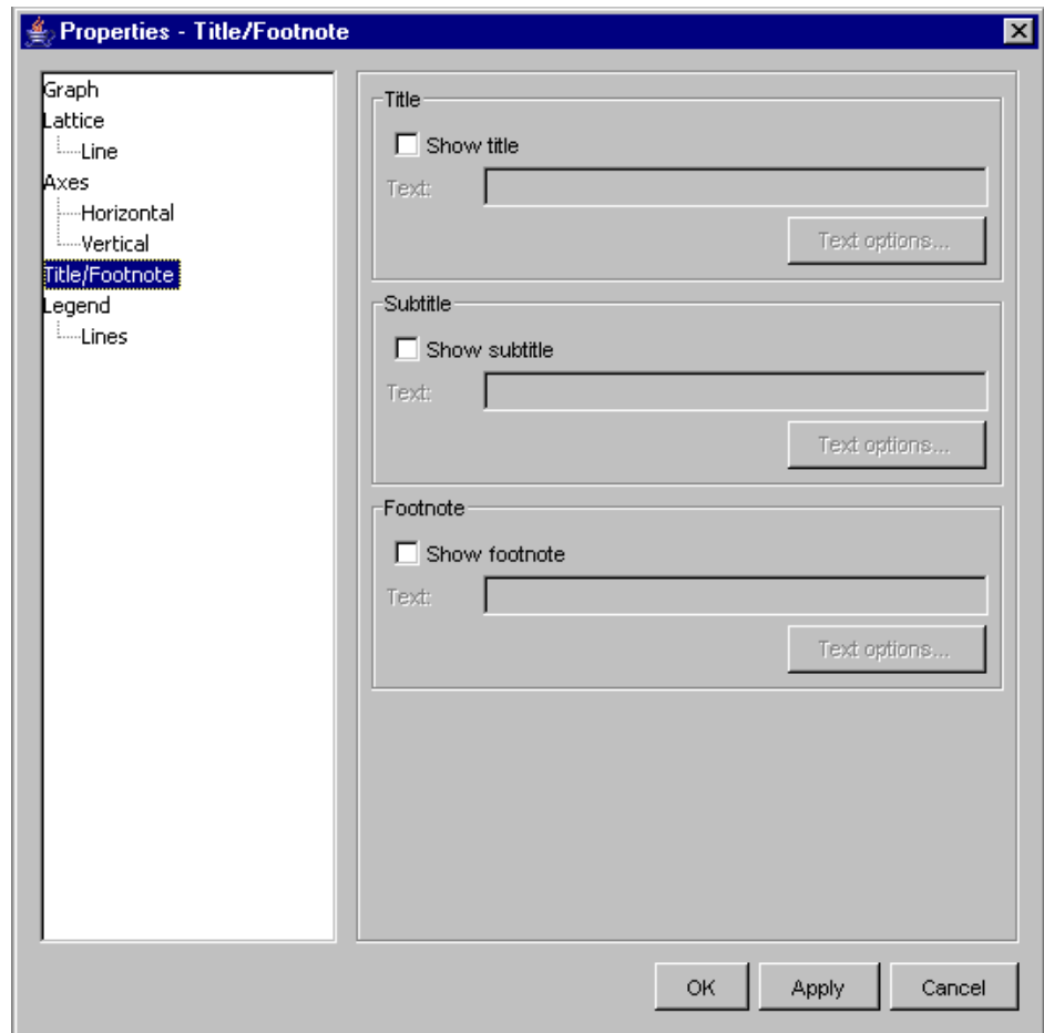
Figure 18.32 Title/Footnote
