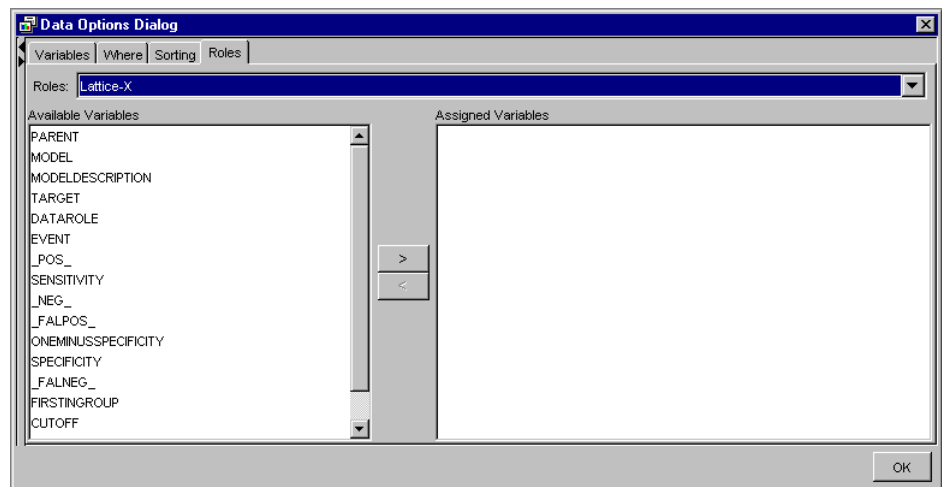
Figure 18.28 Roles Tab
