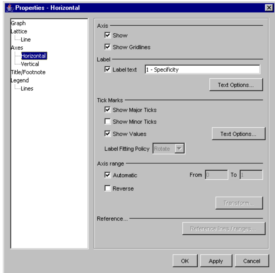
Figure 18.31 Axes
