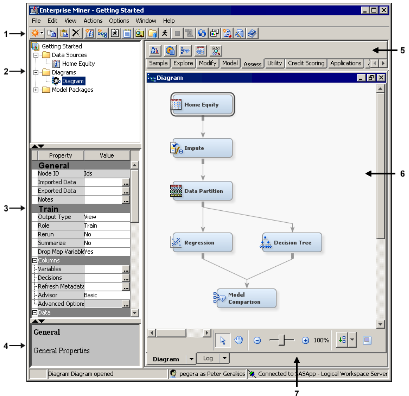
Figure 1.2 The SAS Enterprise Miner GUI
