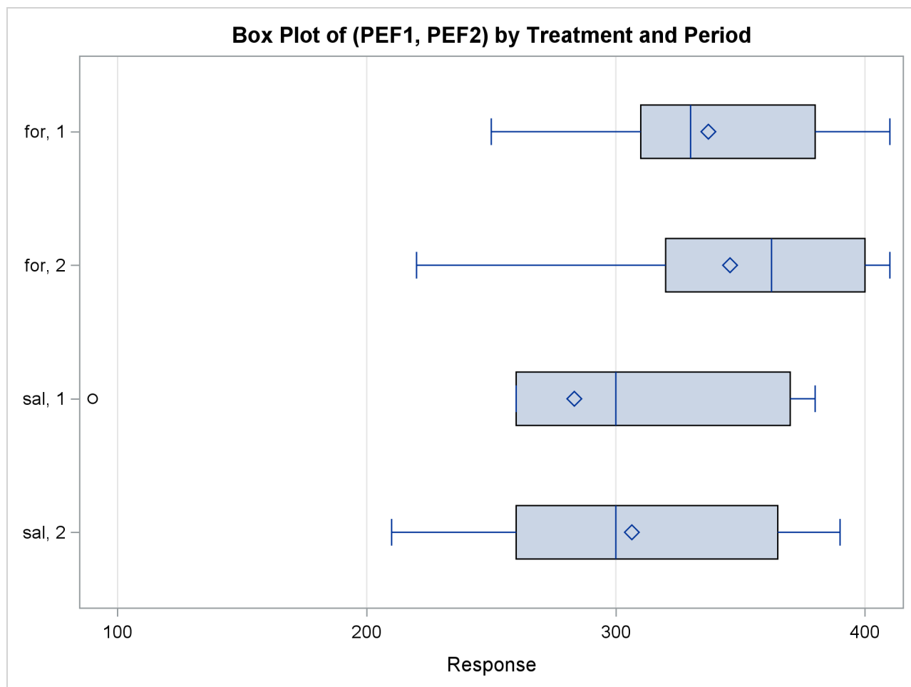
Output 121.4.8 Comparative Box Plots
