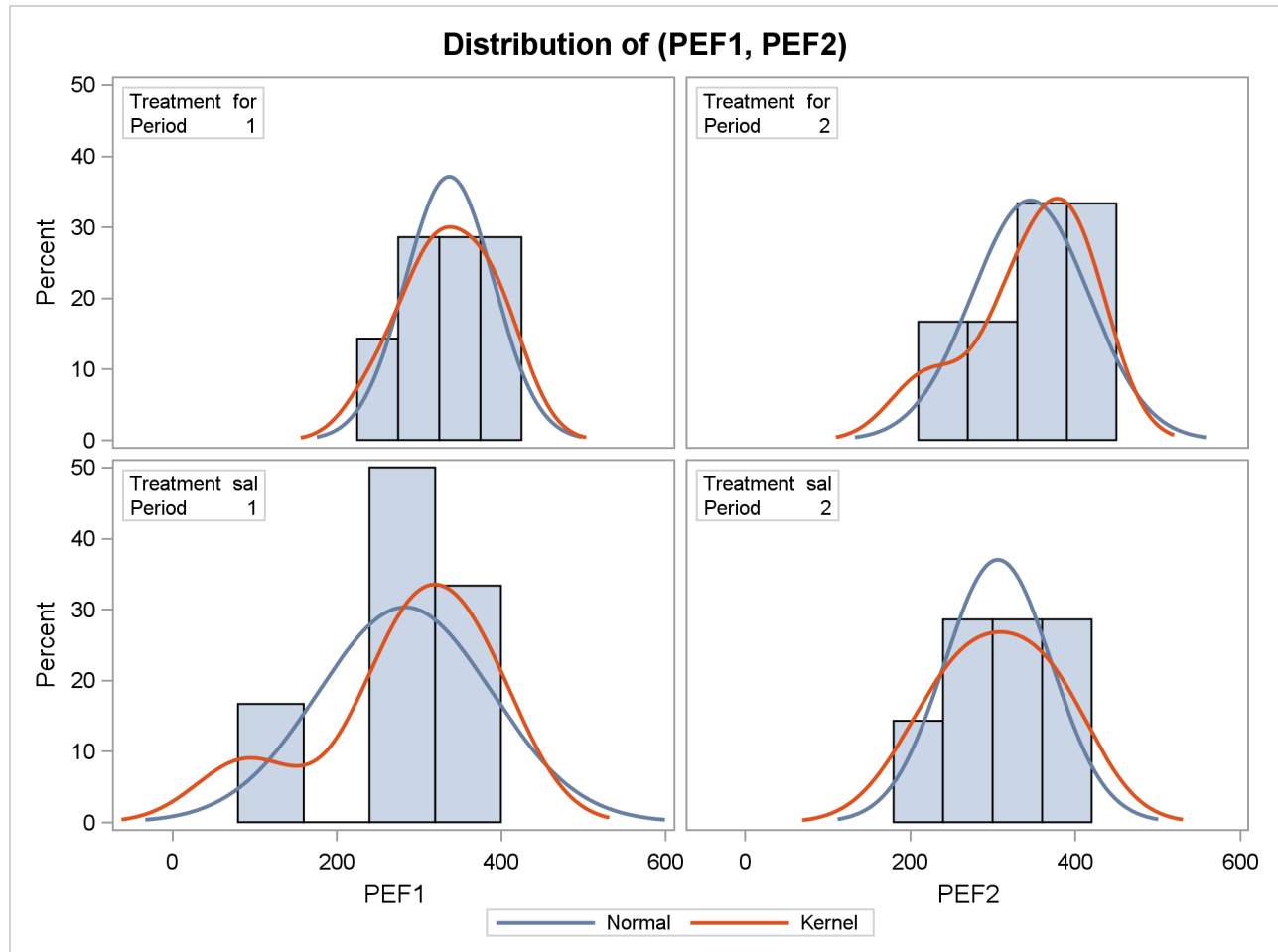
Output 121.4.7 Comparative Histograms
