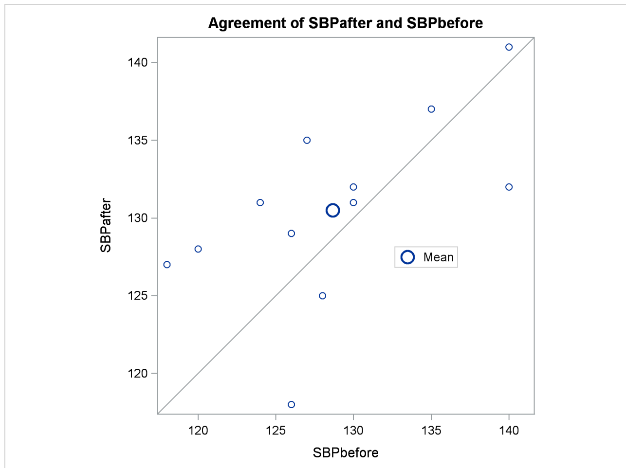
Output 121.3.3 Agreement of Treatments
