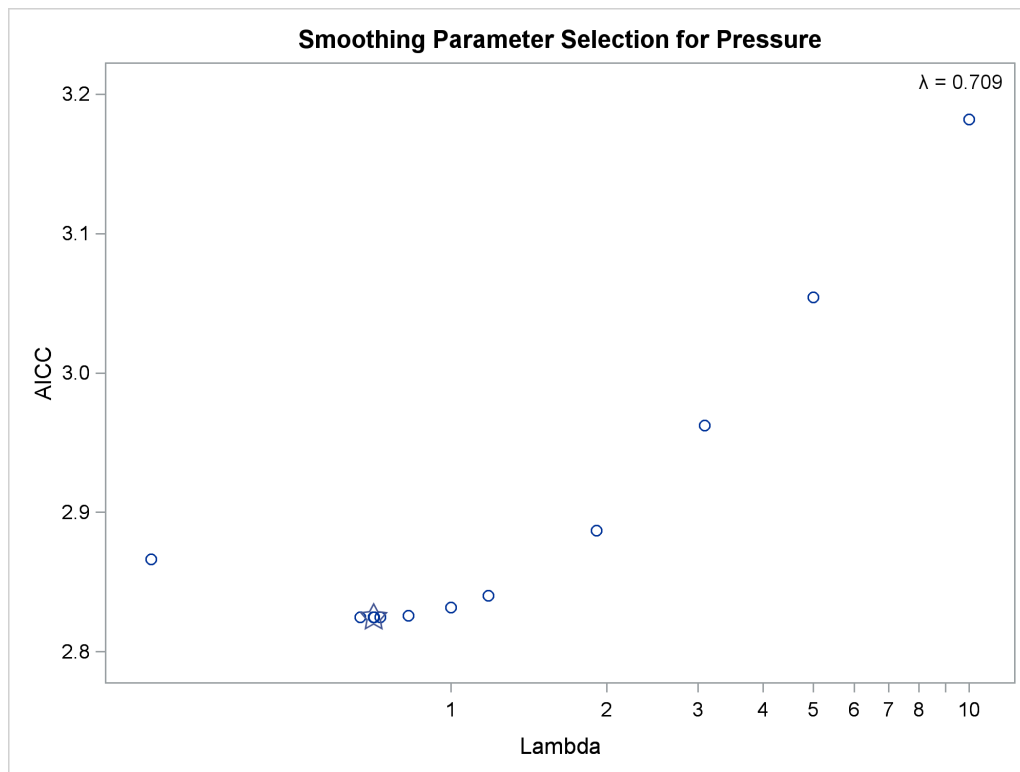
Output 119.3.1 Change in Atmospheric Pressure, AICC
