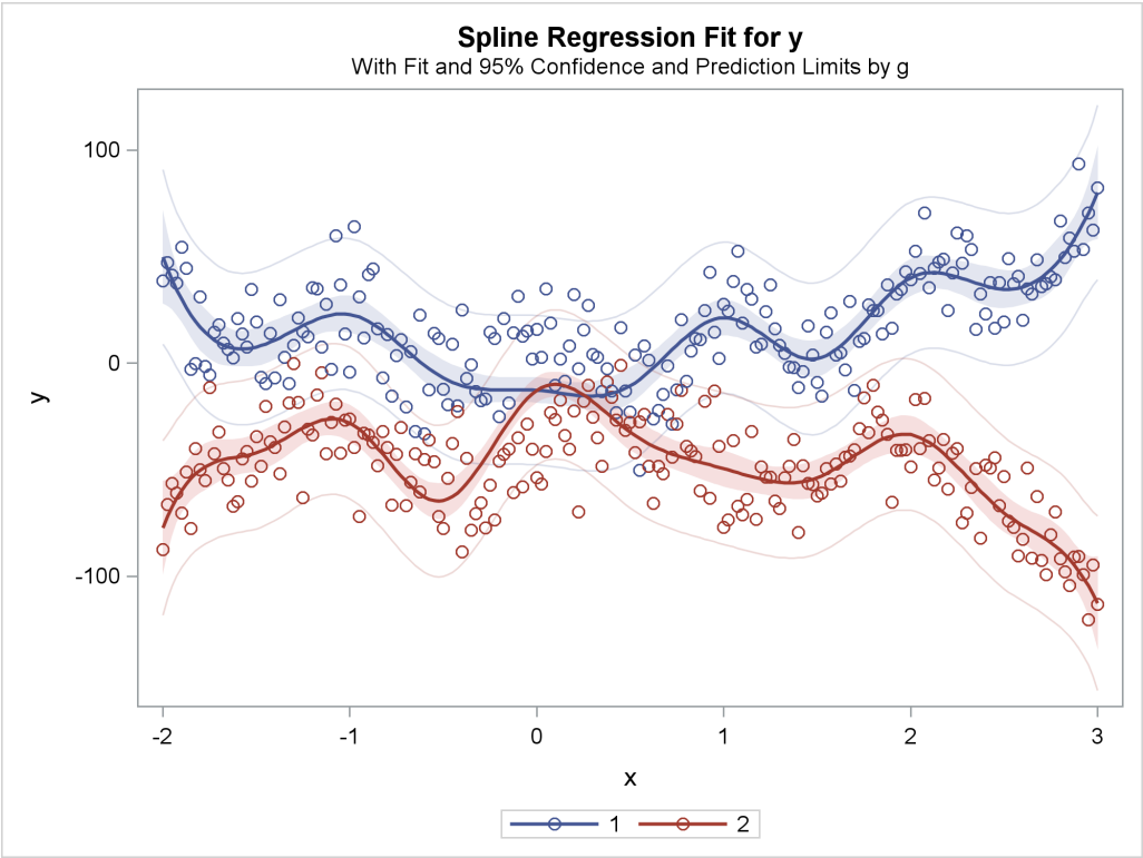
Figure 119.37 Separate Curves, Same Intercept
