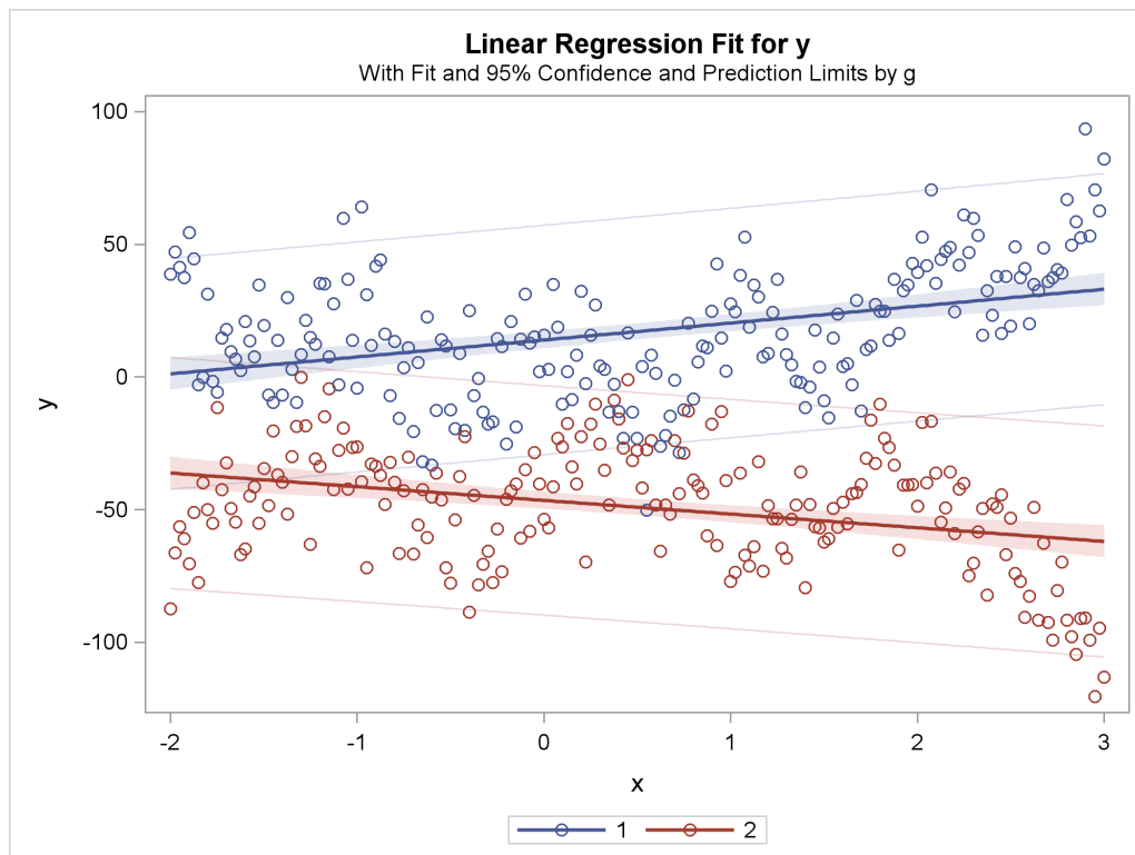
Figure 119.38 Separate Slopes, Separate Intercepts
