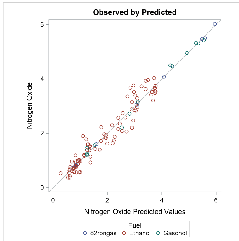
Figure 119.9 Observed by Predicted
