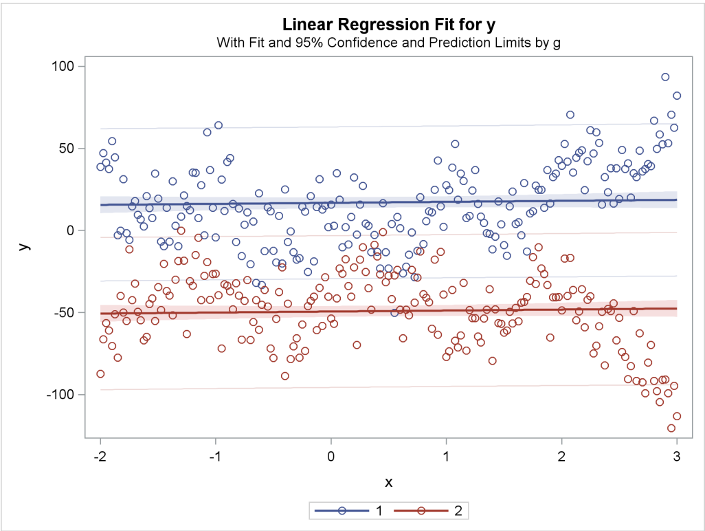
Figure 119.32 Parallel Lines, Separate Intercepts
