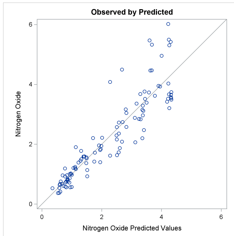
Figure 119.5 Observed by Predicted
