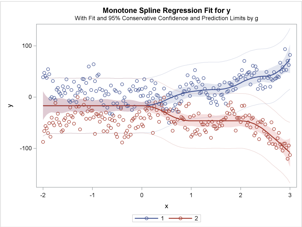
Figure 119.36 Separate Monotone Curves, Same Intercept
