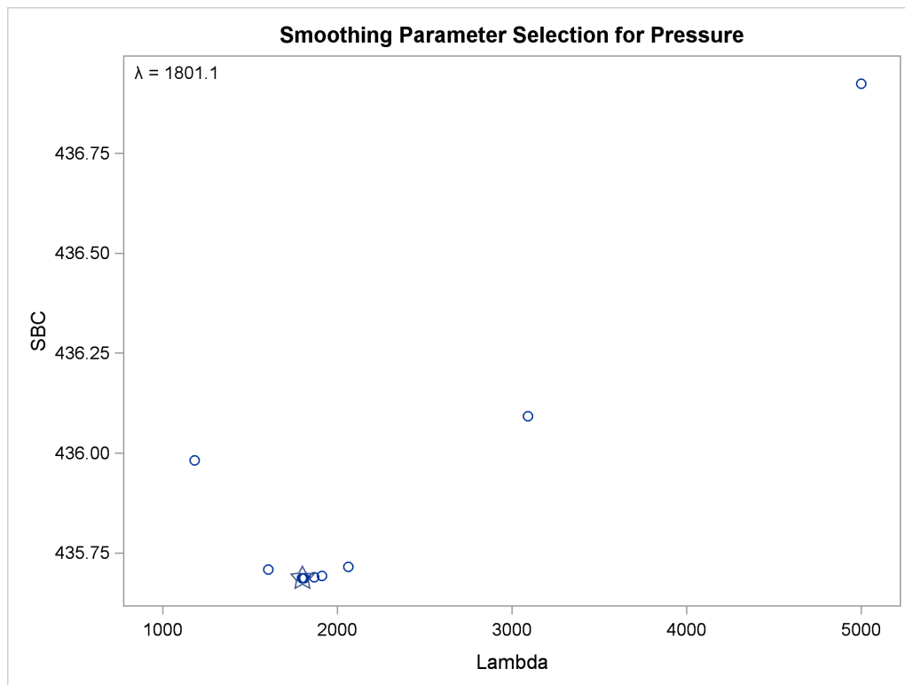
Output 119.3.3 Change in Atmospheric Pressure, SBC, Lambda > 1
