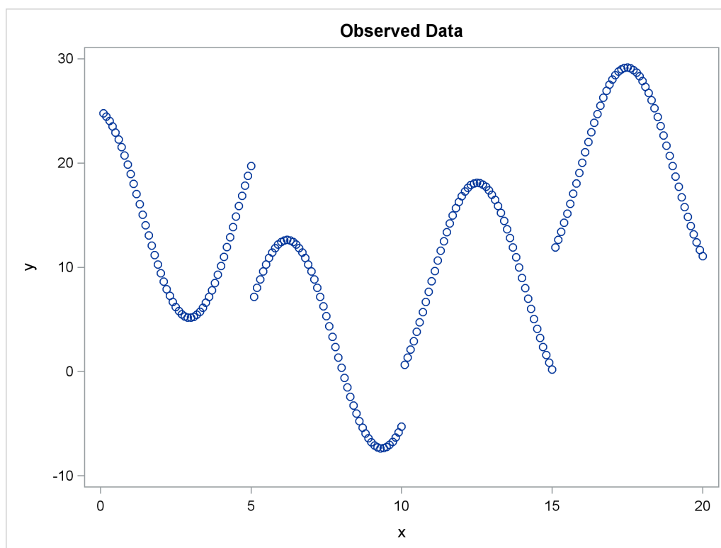
Figure 119.20 The Original Scatter Plot
