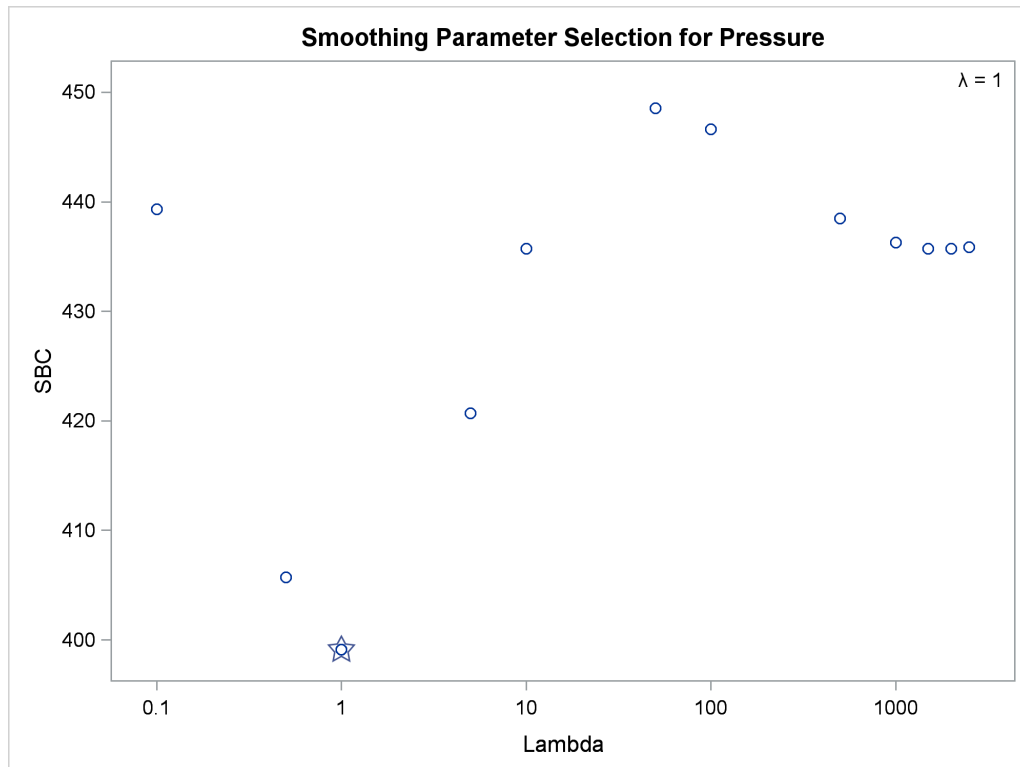
Output 119.3.4 Change in Atmospheric Pressure, SBC, Over the Range of Both Minima
