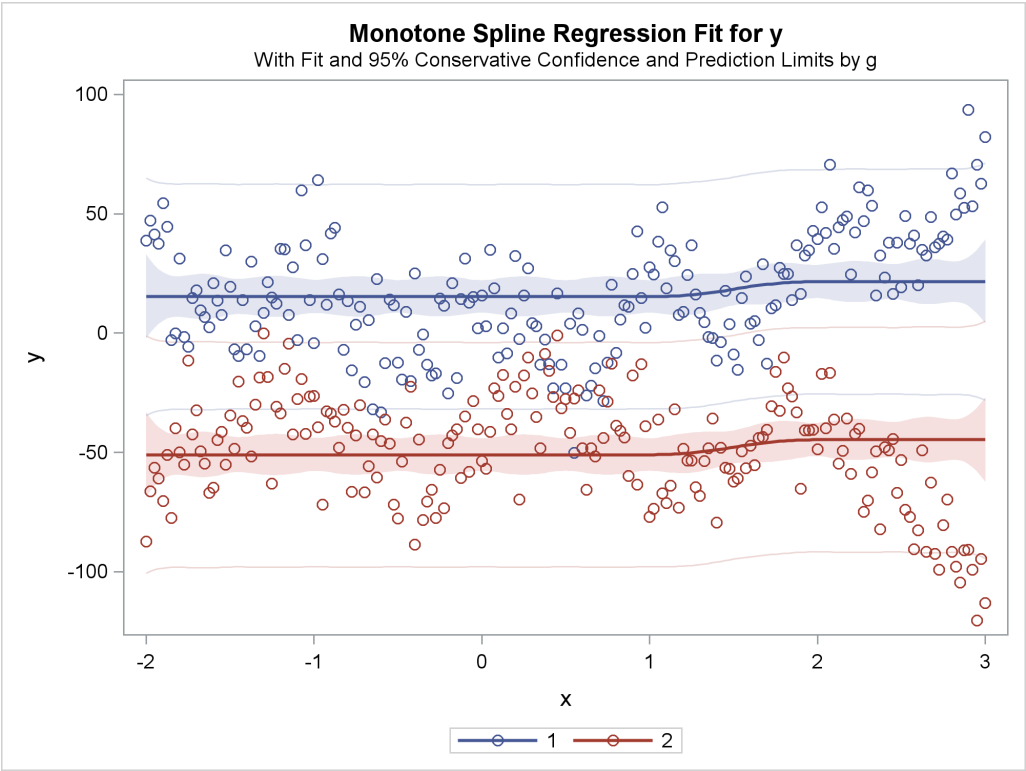
Figure 119.33 Parallel Monotone Curves, Separate Intercepts
