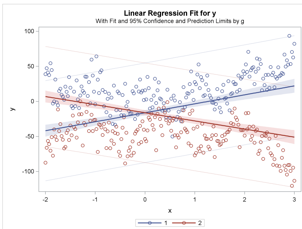
Figure 119.35 Separate Slopes, Same Intercept
