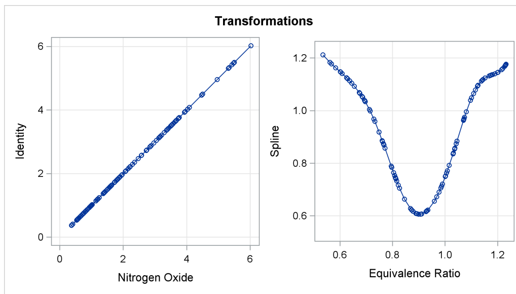
Figure 119.2 Transformations
