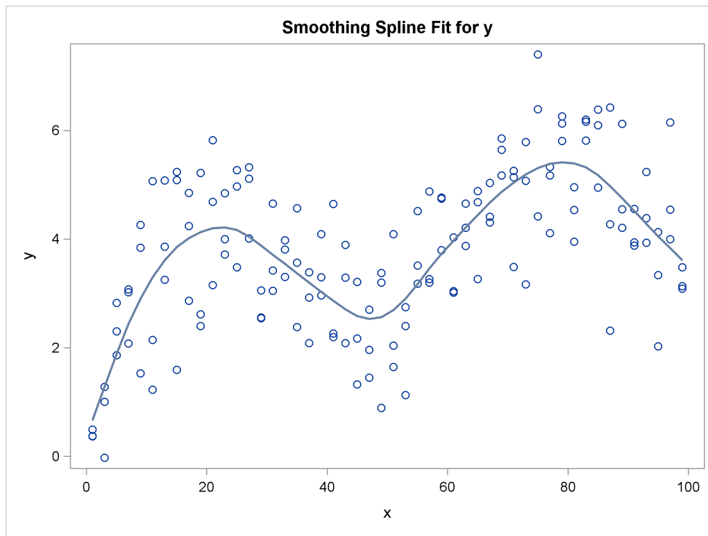
Figure 119.41 Smoothing Spline Displayed with ODS Graphics
