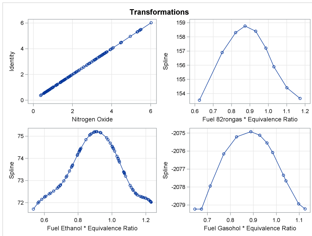
Figure 119.7 Transformations
