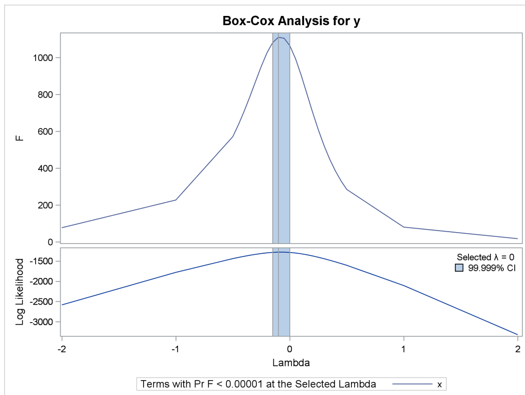
Figure 119.16 Basic Box-Cox Example, Several Options Demonstrated
