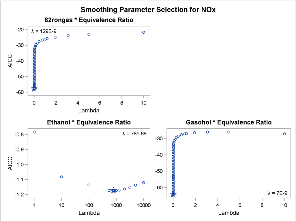
Figure 119.11 Penalized B-Splines
