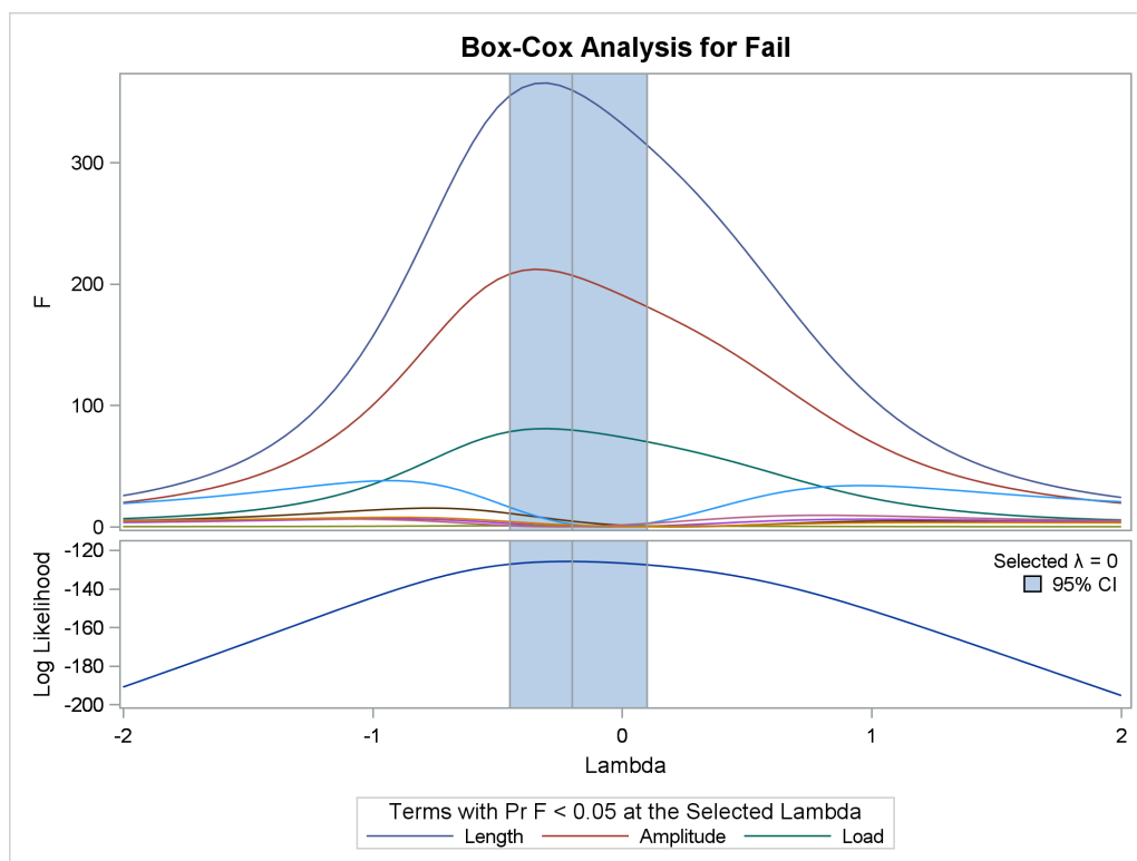
Output 119.2.1 Box-Cox Yarn Data
