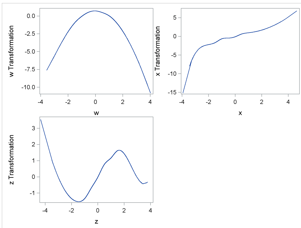
Figure 119.27 Scoring Spline Variables Example
