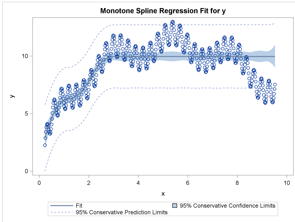
Figure 119.29 A Monotone Regression Function
