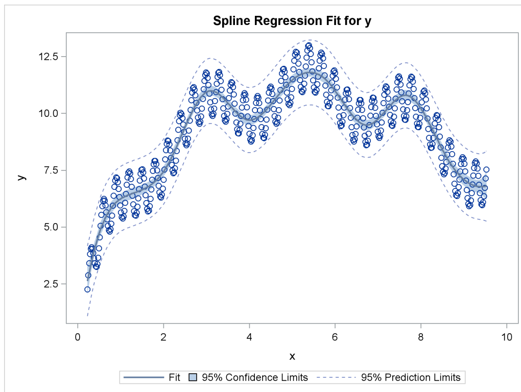
Figure 119.30 A Nonlinear Regression Function
