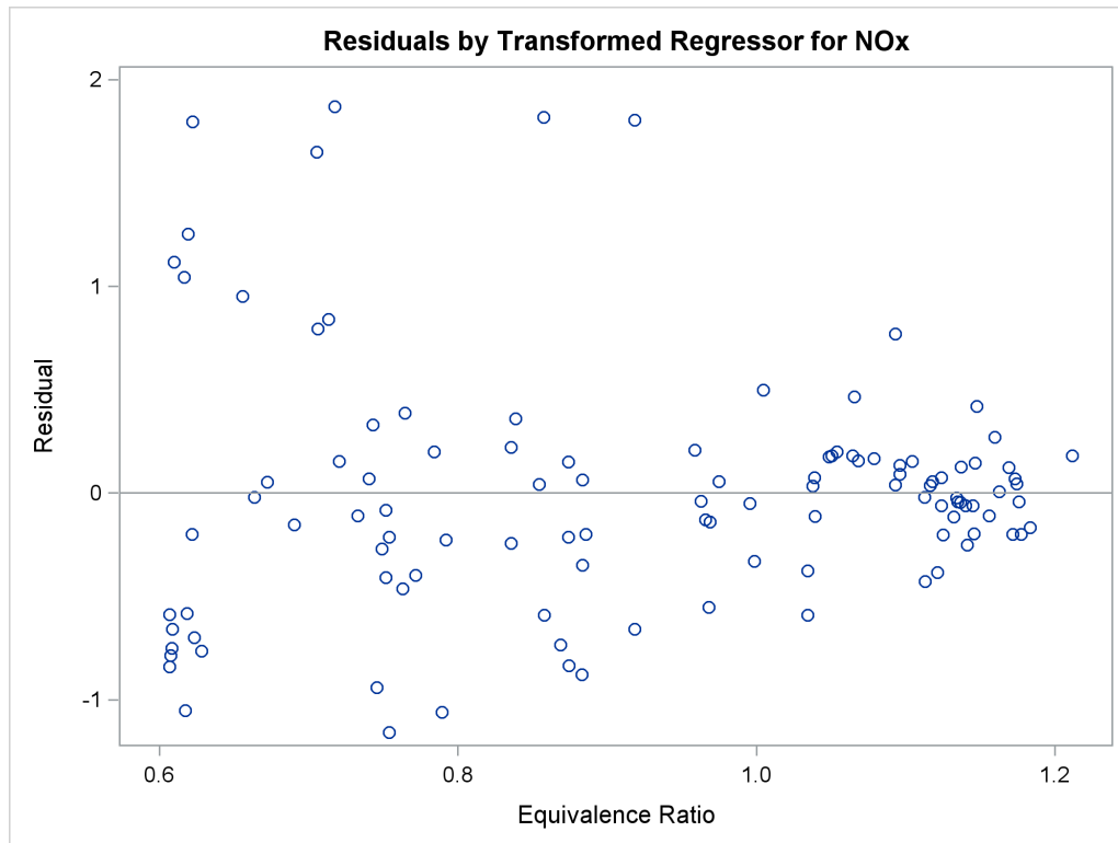
Figure 119.3 Residuals
