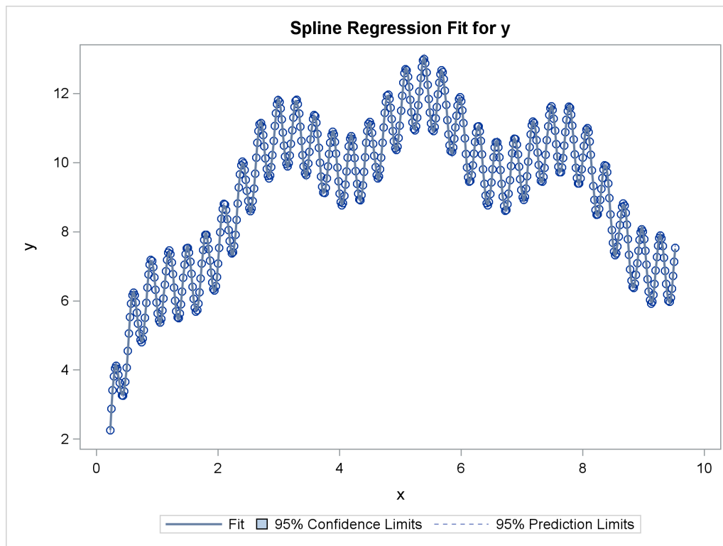
Figure 119.31 A Less-Smooth Nonlinear Regression Function
