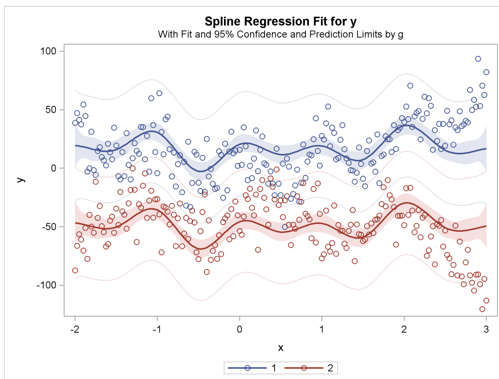
Figure 119.34 Parallel Curves, Separate Intercepts
