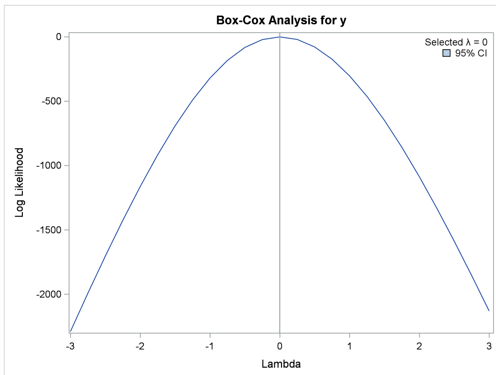
Figure 119.18 Box-Cox with No Independent Variable
