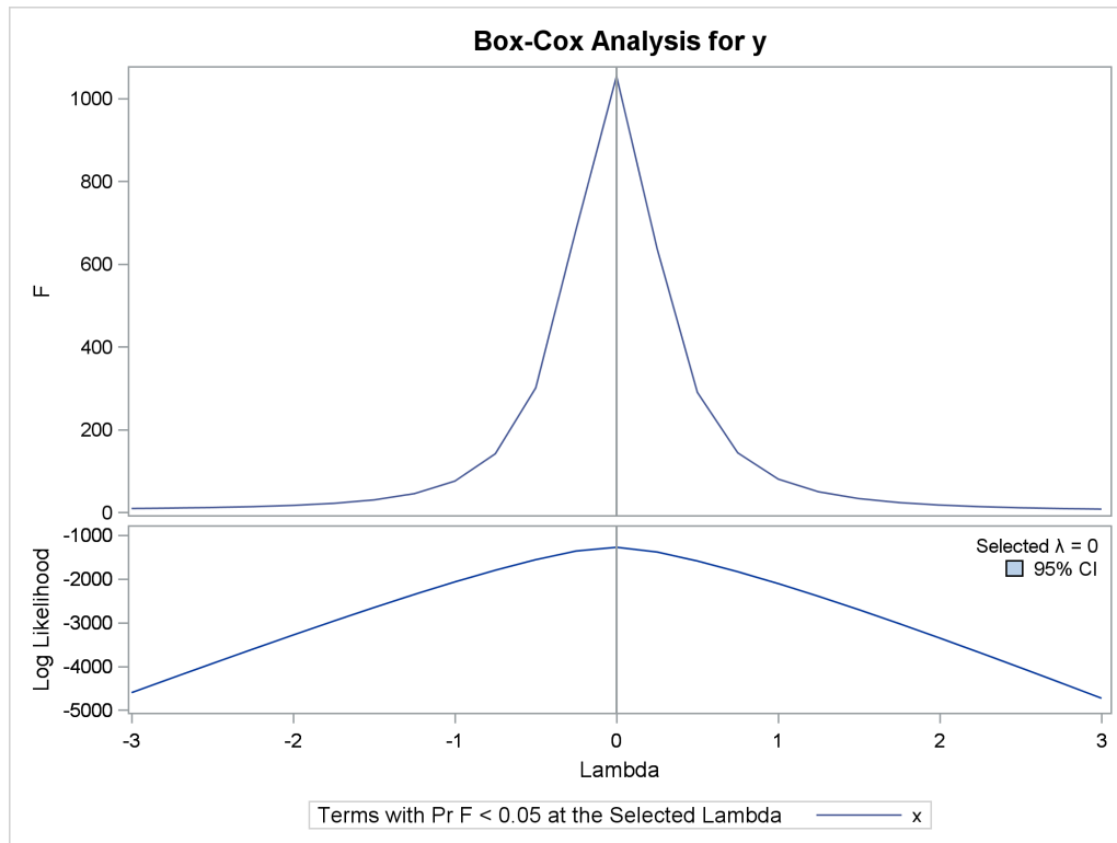
Figure 119.14 Basic Box-Cox Example, Default Output
