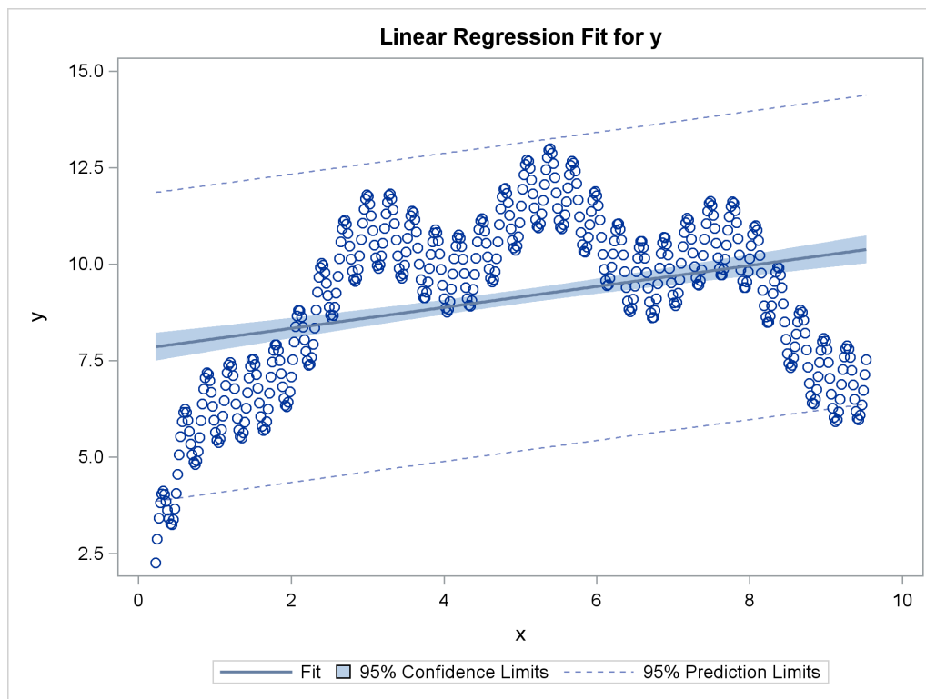
Figure 119.28 Linear Regression
