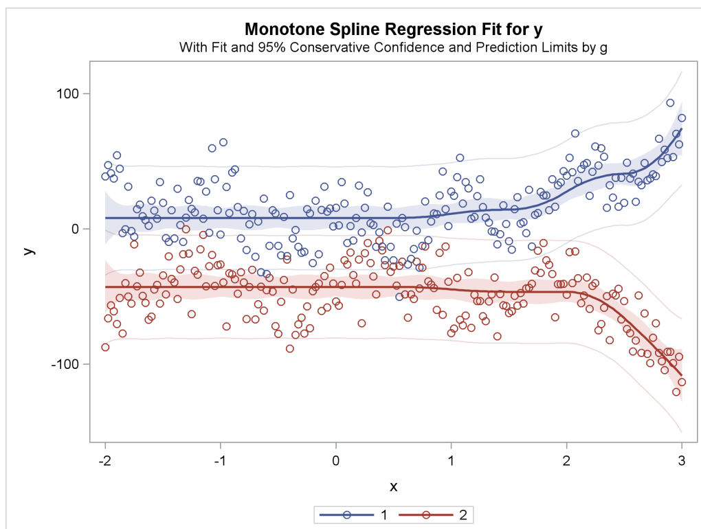
Figure 119.39 Separate Monotone Curves, Separate Intercepts
