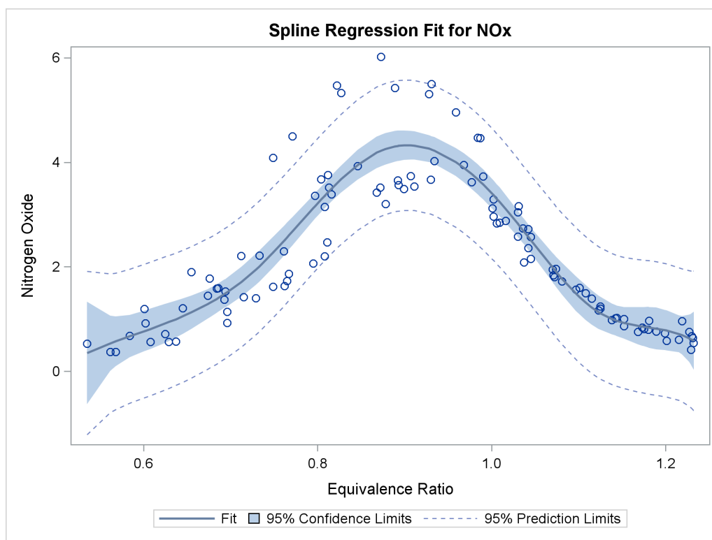
Figure 119.4 Fitting a Curve through a Scatter Plot
