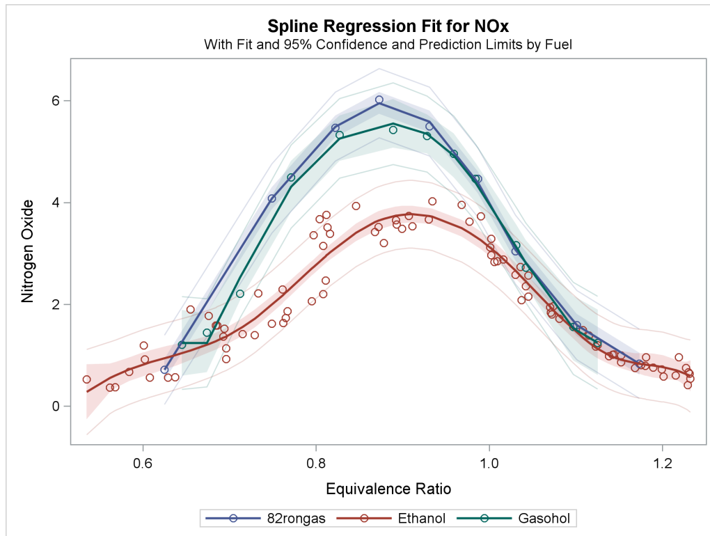
Figure 119.8 Fitting Curves through a Scatter Plot
