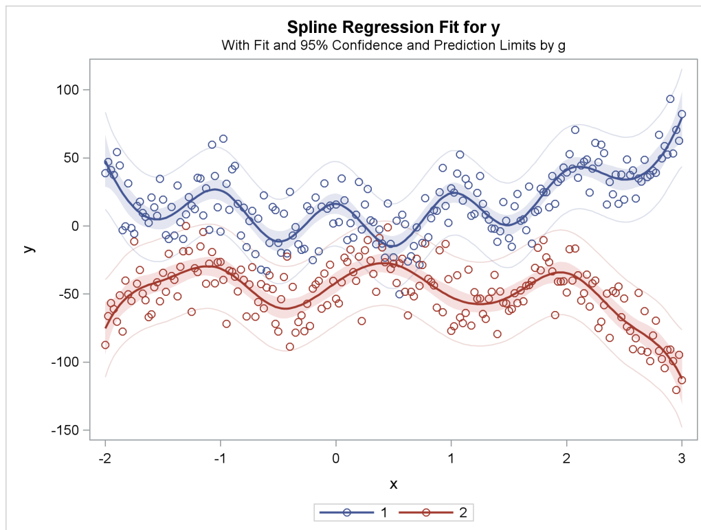
Figure 119.40 Separate Curves, Separate Intercepts
