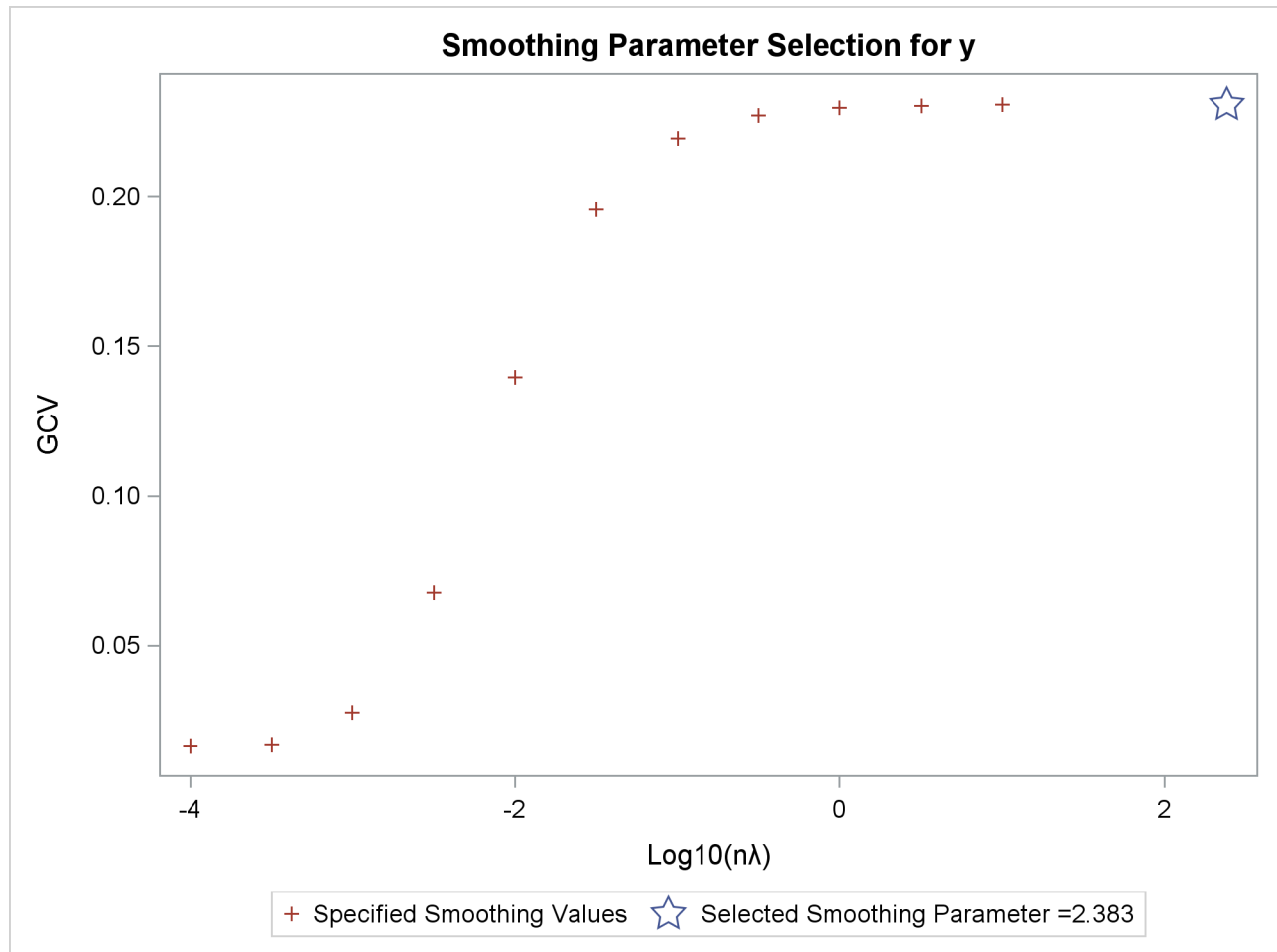
Output 118.2.4 Criterion Plot
