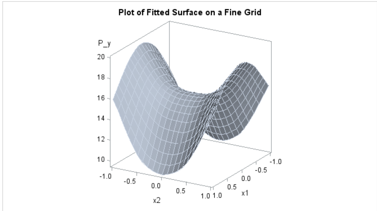
Figure 118.6 Plot of TPSPLINE Fit
