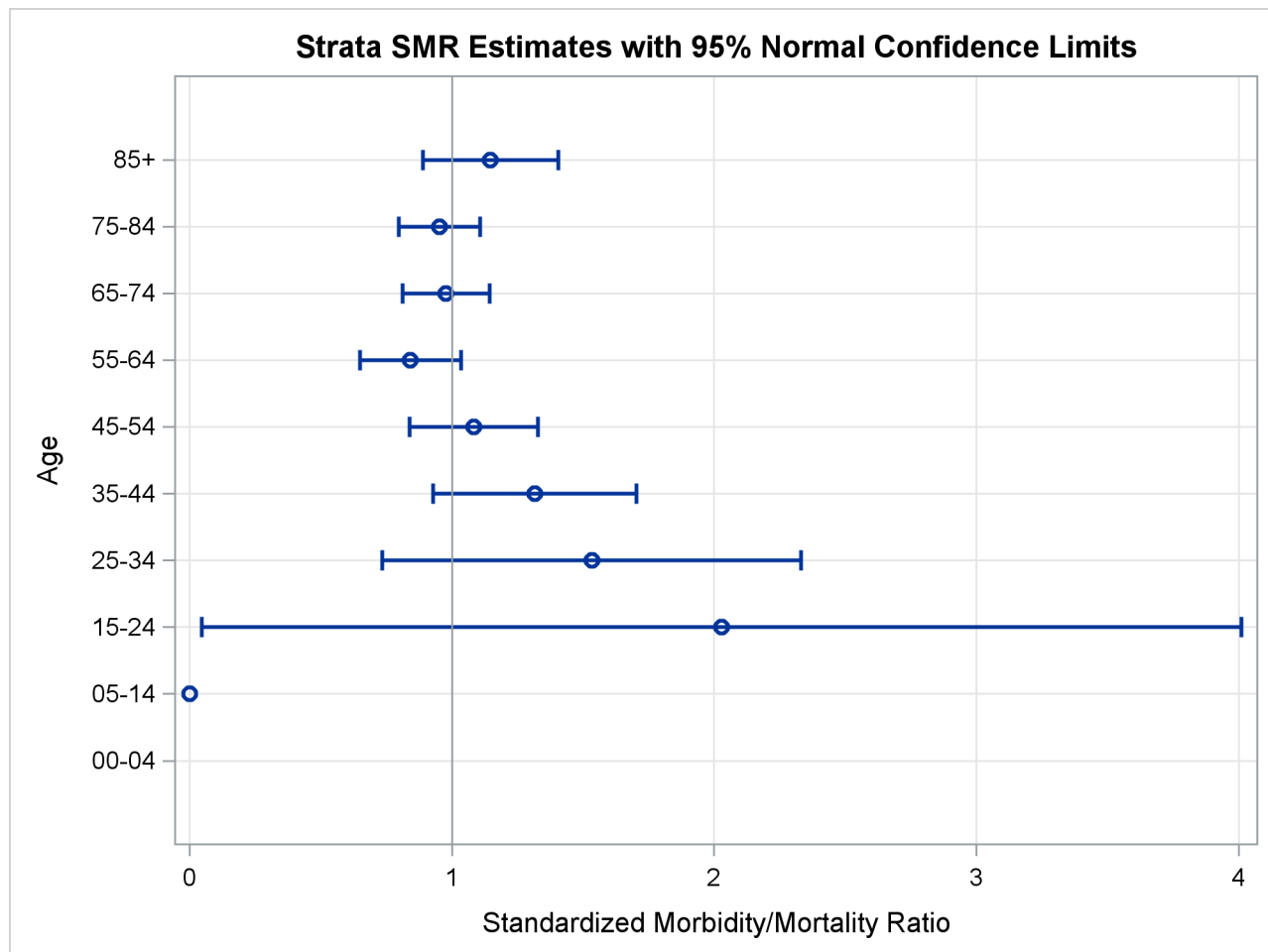
Figure 109.6 Strata SMR Plot
