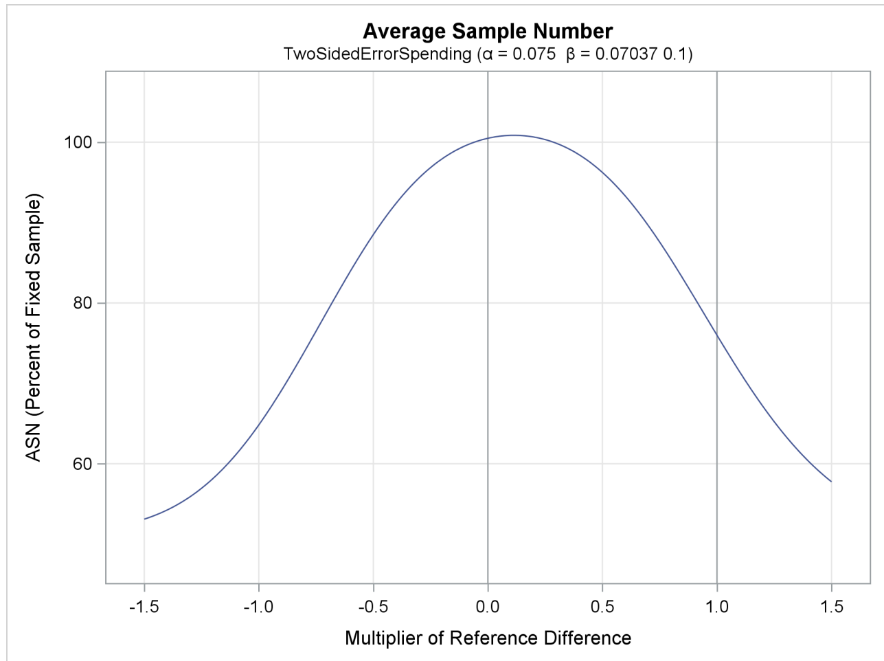
Output 103.11.6 ASN Plot
