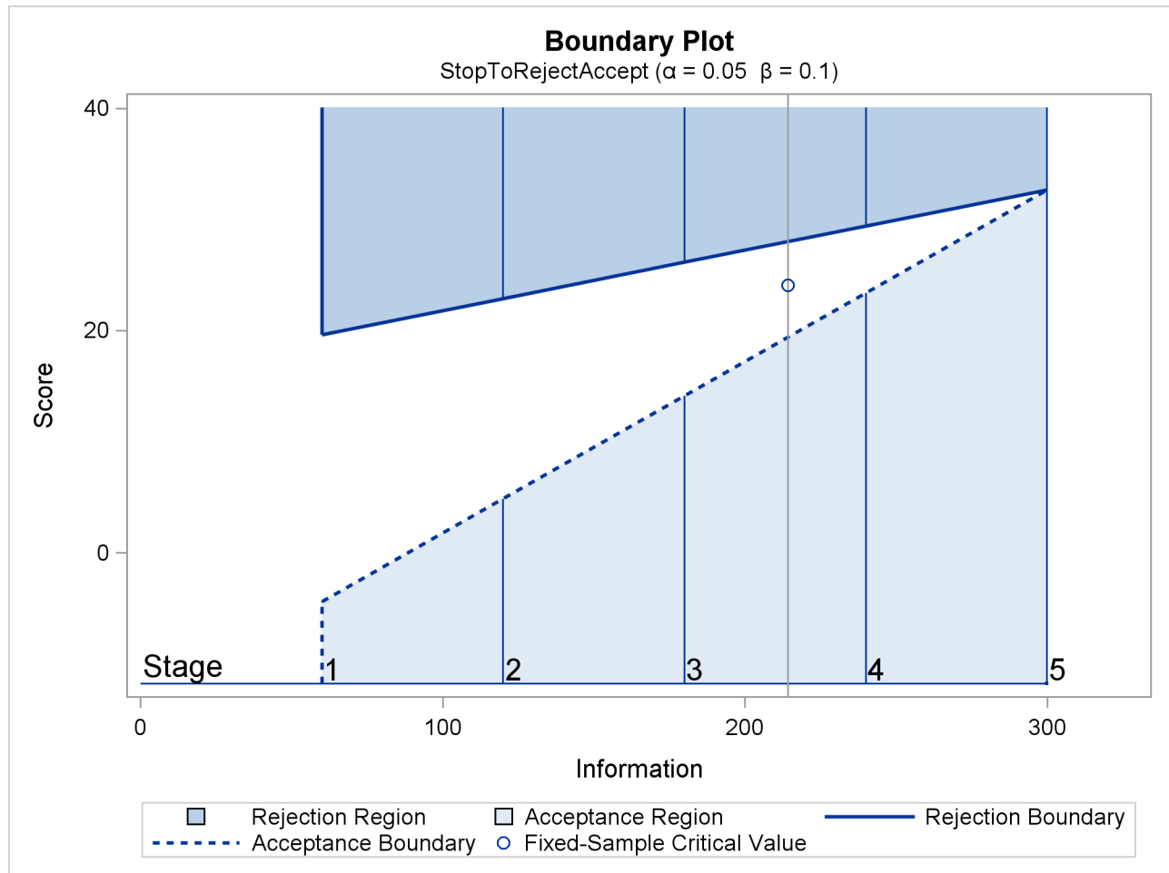
Output 103.6.5 Boundary Plot with Score Statistics
