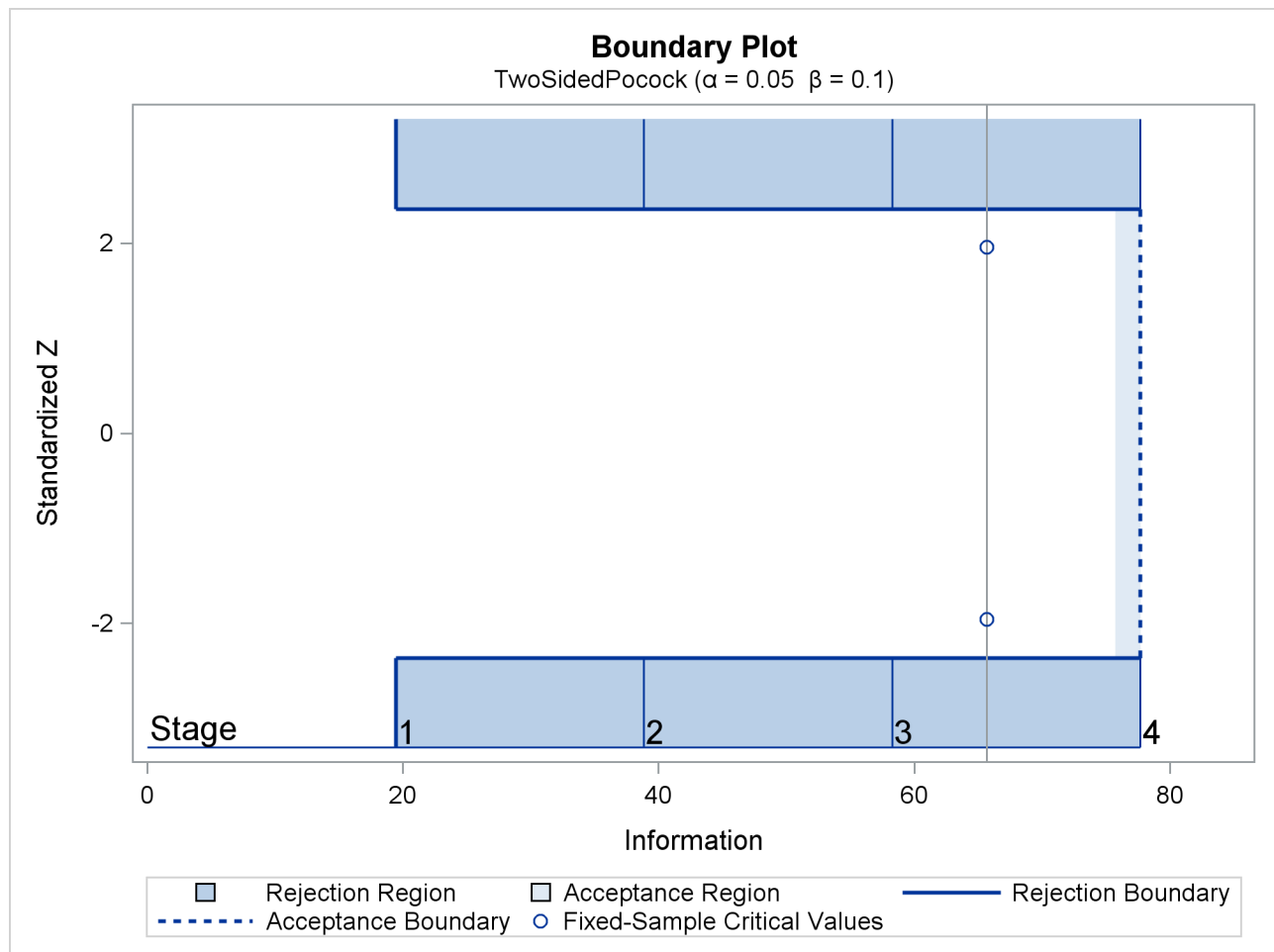
Output 103.4.1 Pocock Boundary Plot
