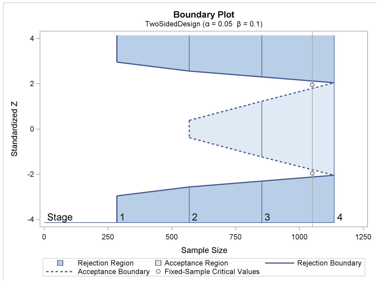
Figure 103.11 Boundary Plot for Two-Sided Test
