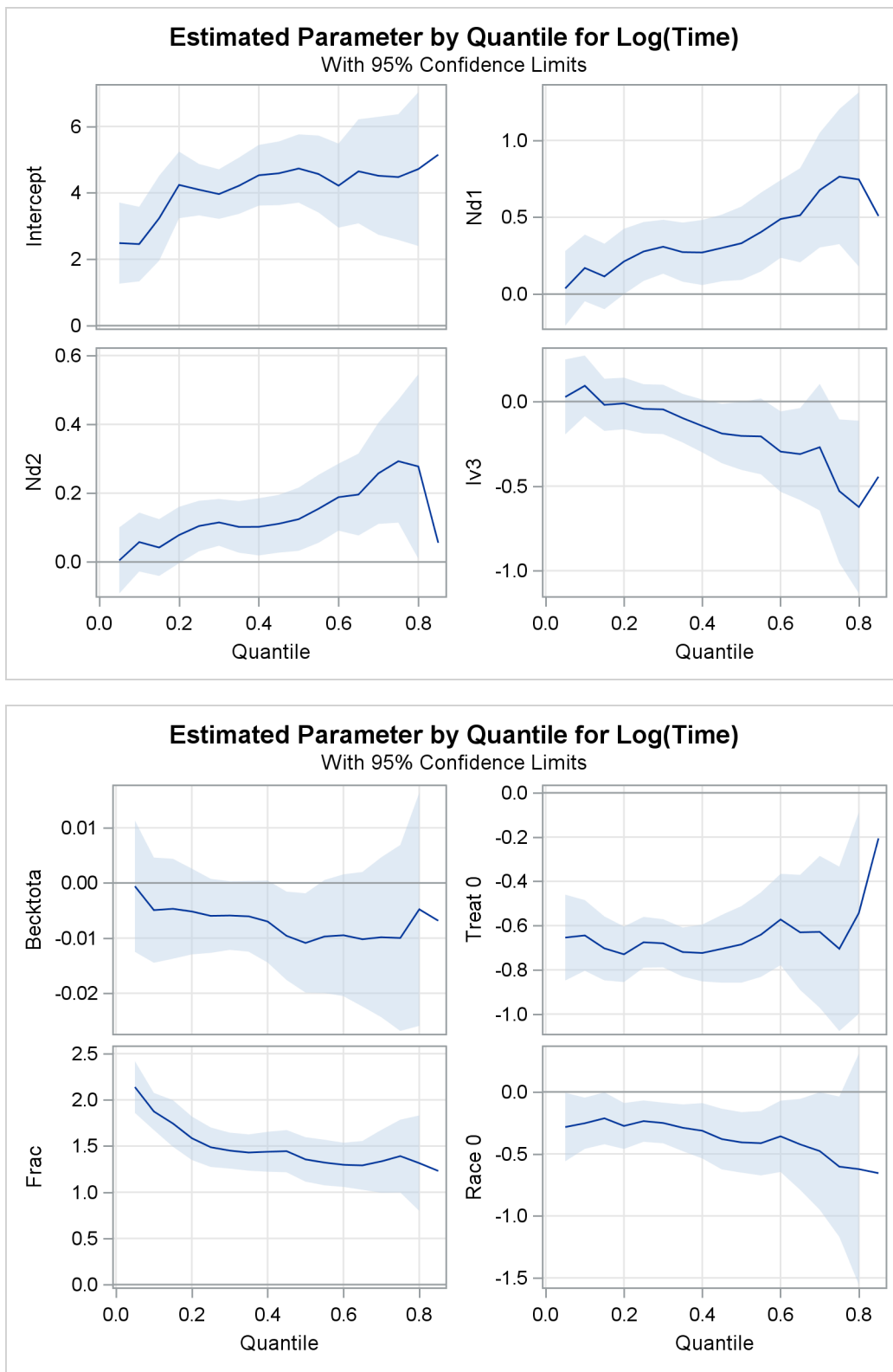
Output 96.2.2 Quantile Processes with 95% Confidence Bands
