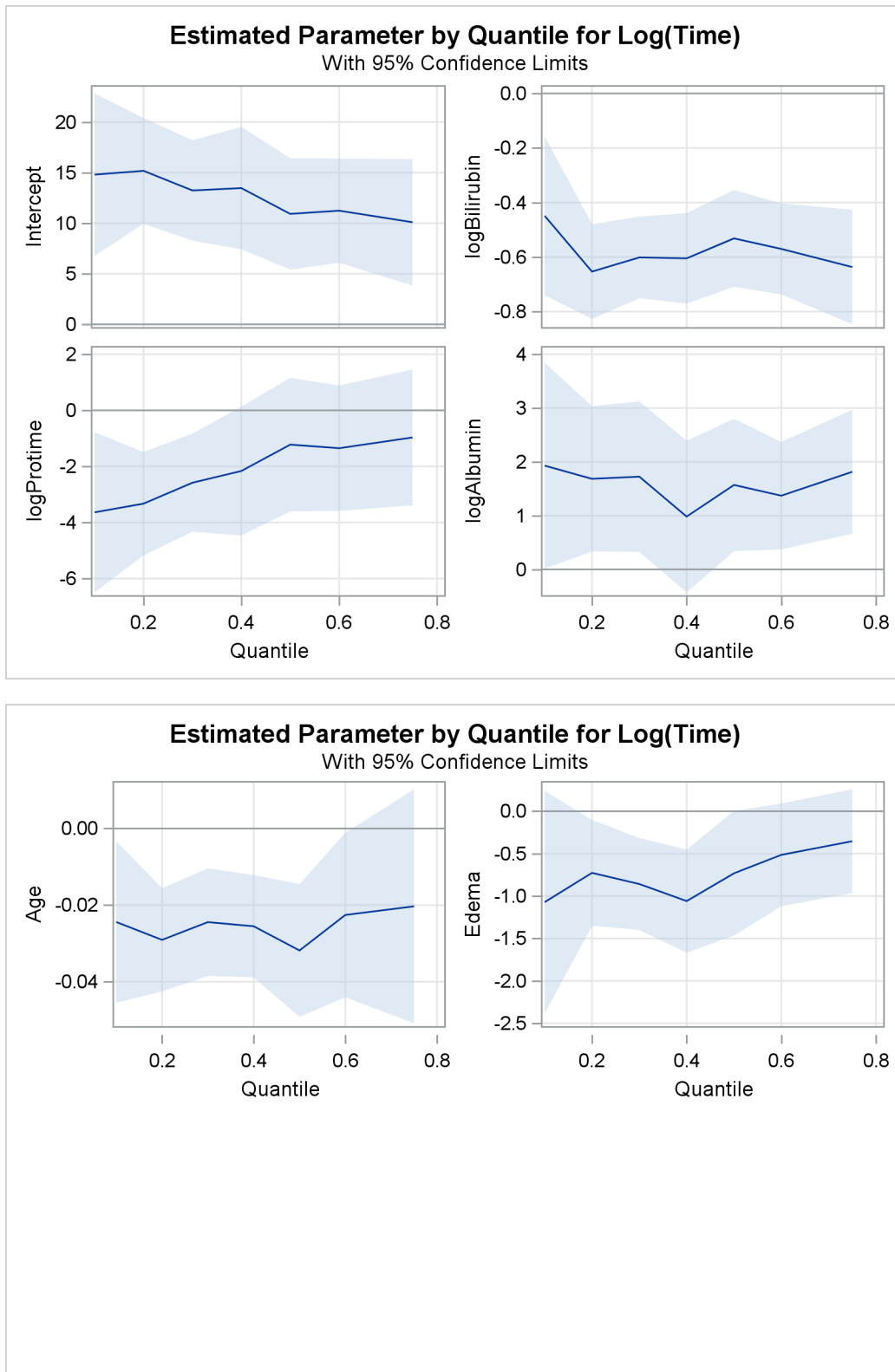
Output 96.1.4 Quantile Processes with 95% Confidence Bands
