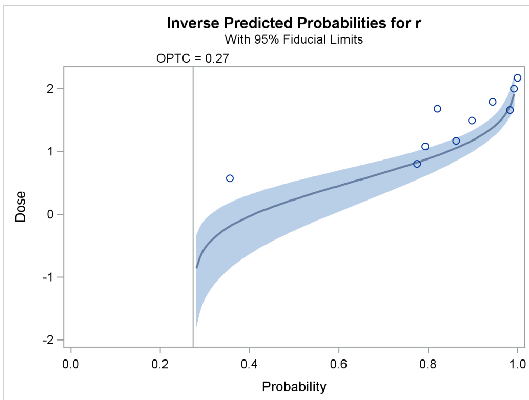
Output 94.4.12 Inverse Predicted Probability Plot
