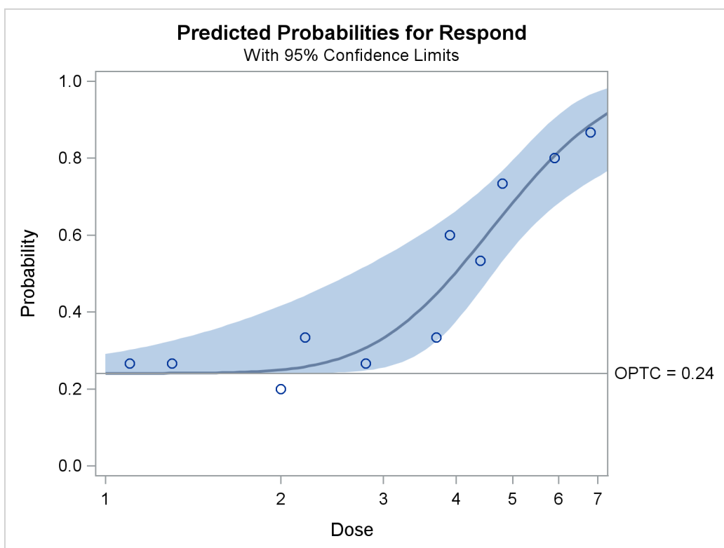
Figure 94.4 Plot of Observed and Fitted Probabilities versus Dose Level
