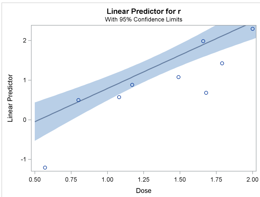
Output 94.4.13 Linear Predictor Plot
