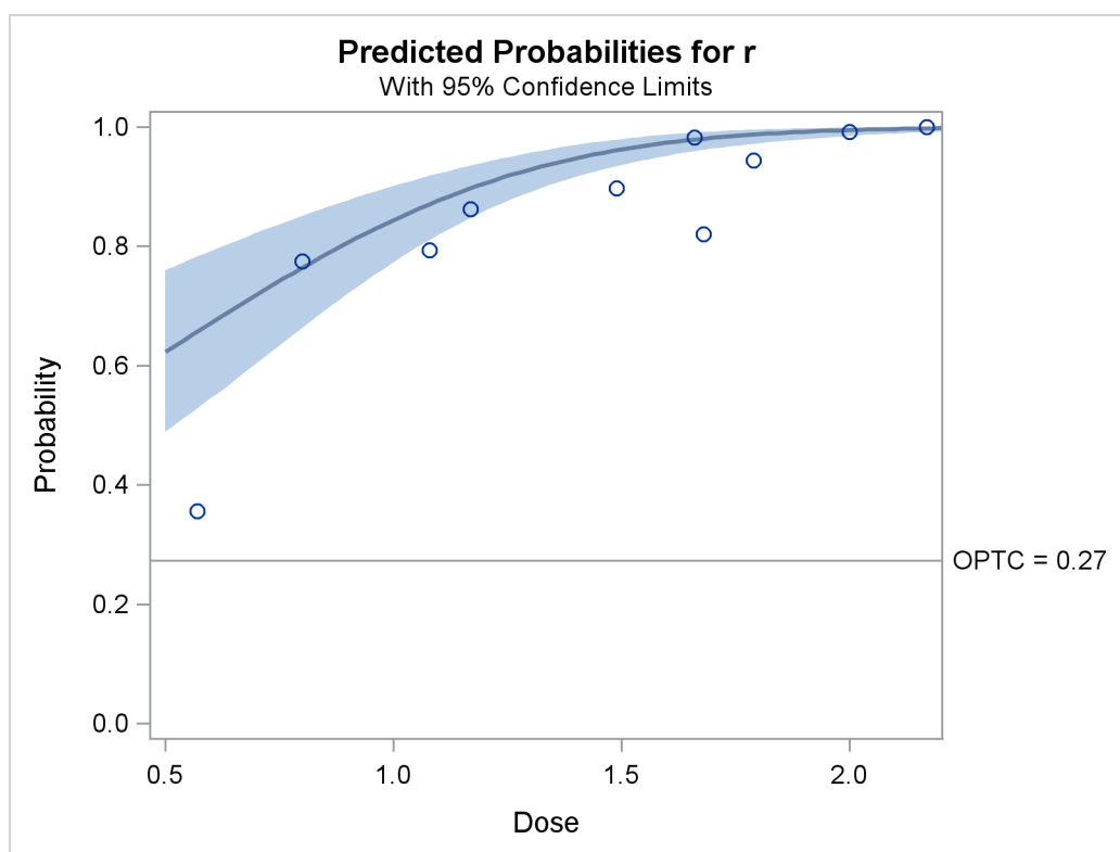
Output 94.4.11 Predicted Probability Plot
