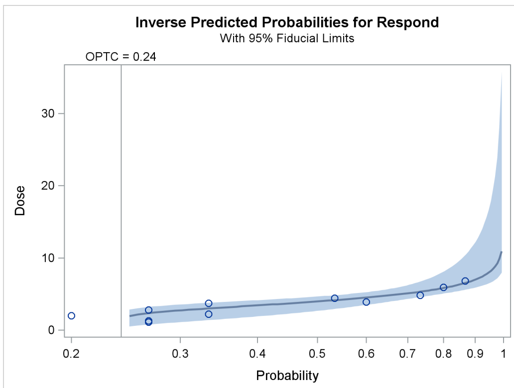
Figure 94.5 Inverse Predicted Probability Plot with Fiducial Limits
