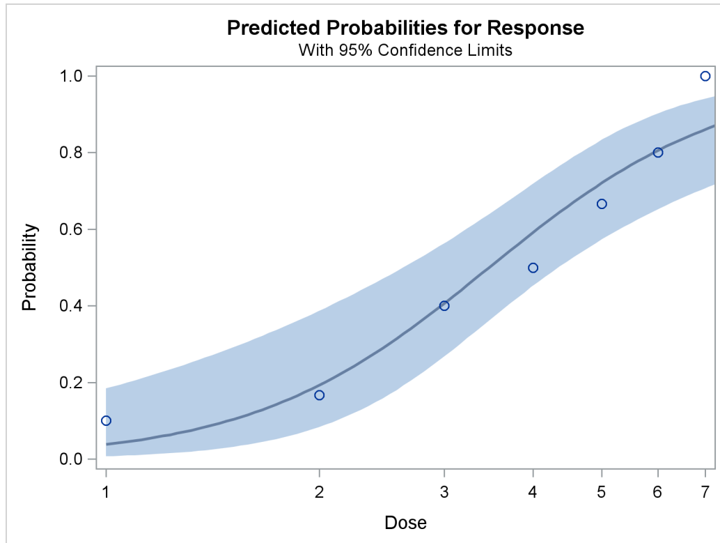
Output 94.1.7 Plot of Observed and Fitted Probabilities
