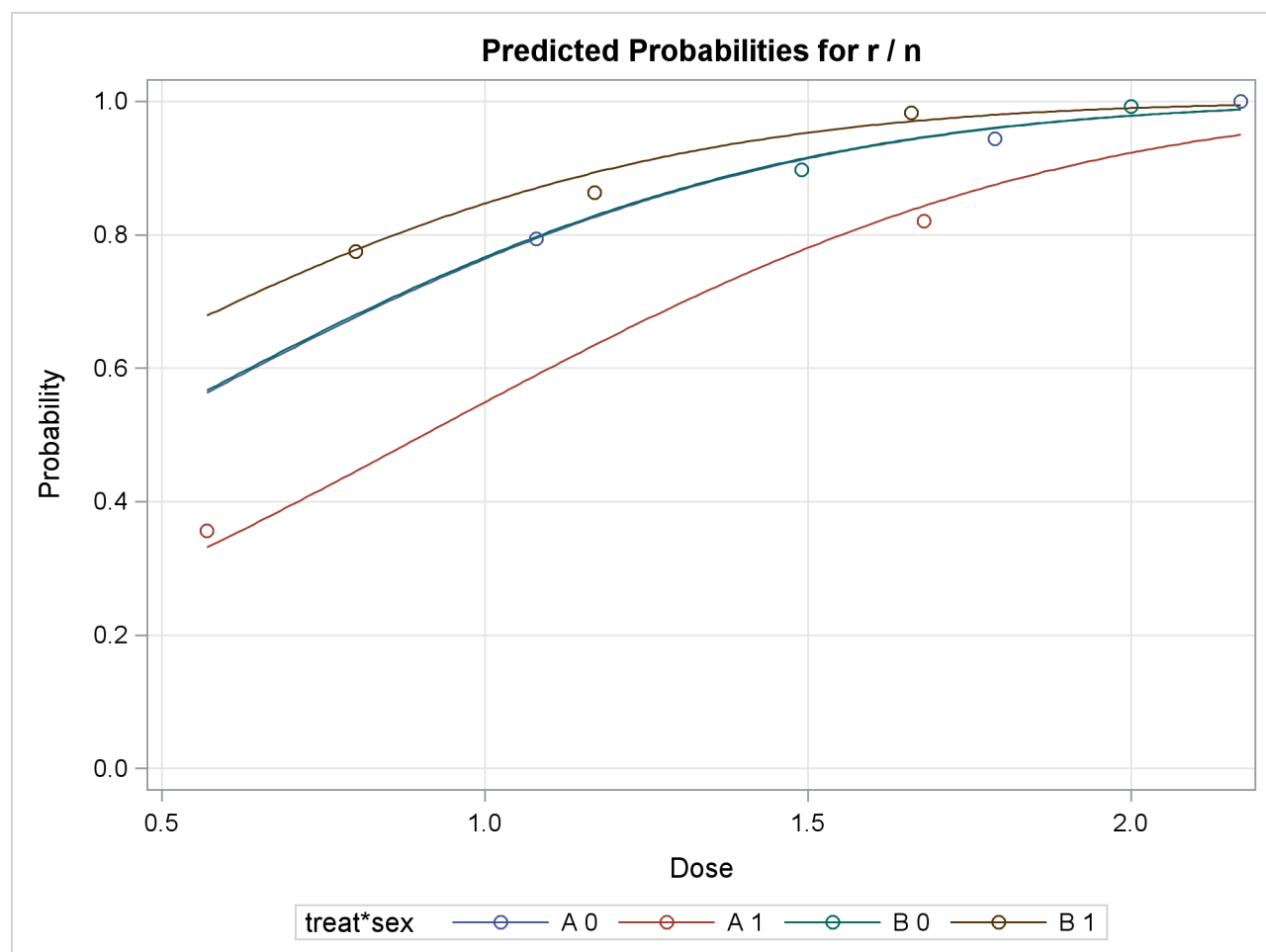
Output 94.5.3 Predicted Probability versus Dose Level by treat*sex
