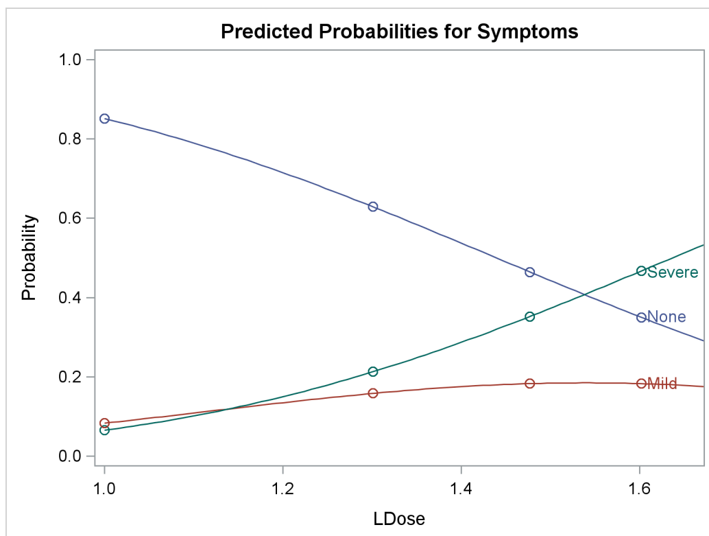
Output 94.2.3 Plot of Predicted Probabilities for the Test Preparation Group
