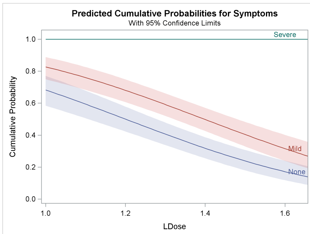
Output 94.2.6 Plot of Predicted Cumulative Probabilities for the Standard Preparation Group
