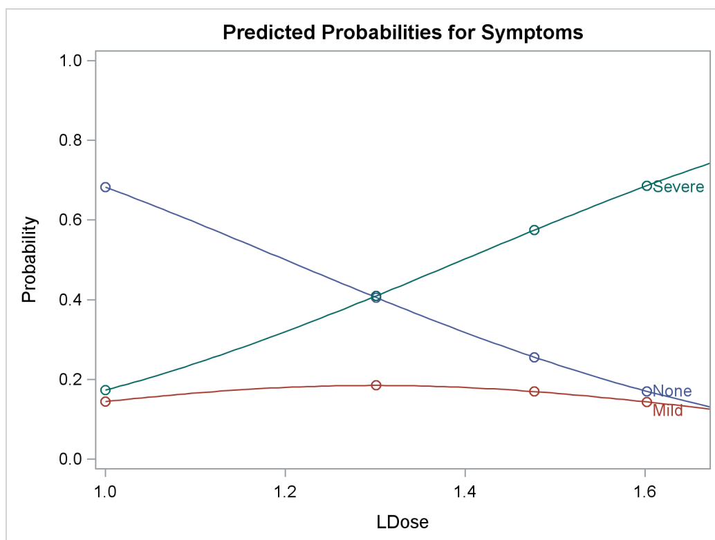
Output 94.2.5 Plot of Predicted Probabilities for the Standard Preparation Group
