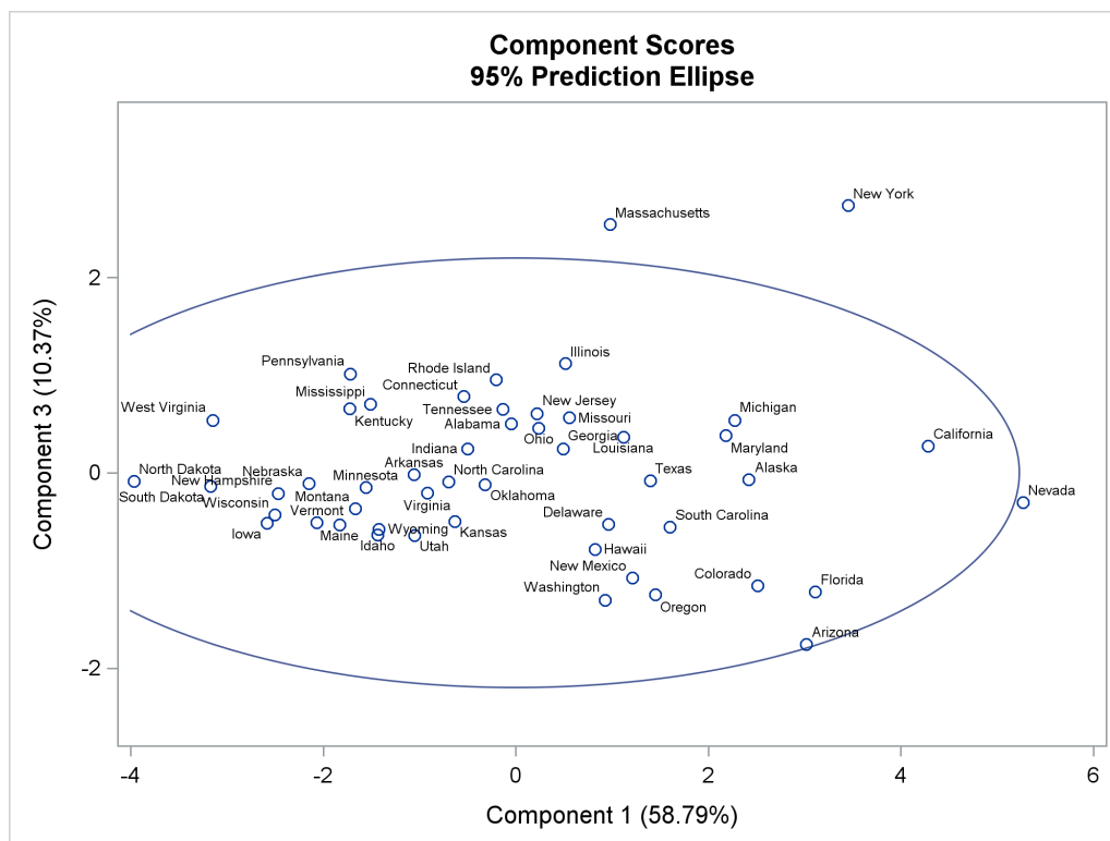
Figure 92.5 Plot of the First and Third Component Scores
