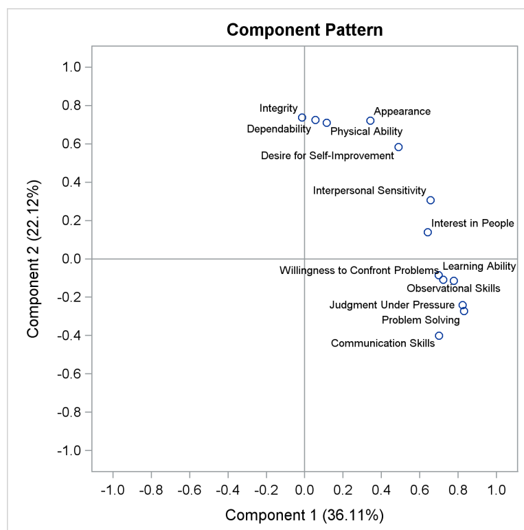
Output 92.3.5 Pattern Plot of Component 2 by Component 1
