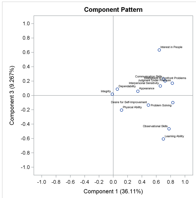
Output 92.3.6 Pattern Plot of Component 3 by Component 1
