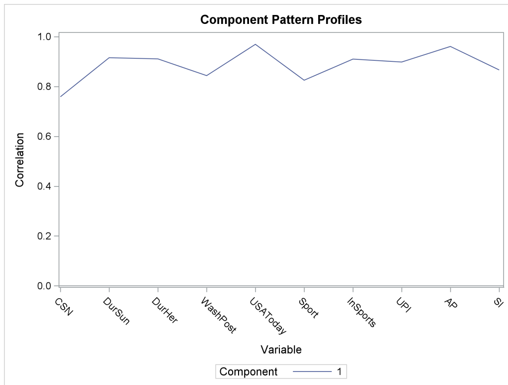
Output 92.2.3 Pattern Profile Plot
