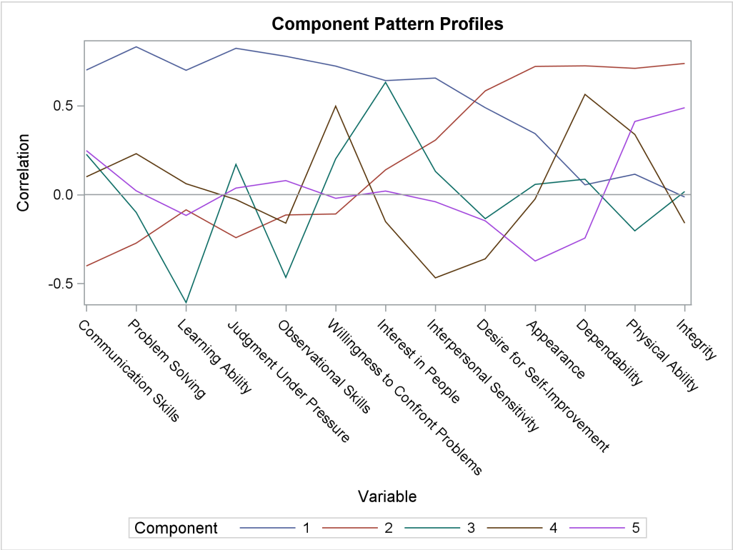
Output 92.3.8 Component Pattern Profile Plot from Using PROC PRINCOMP
