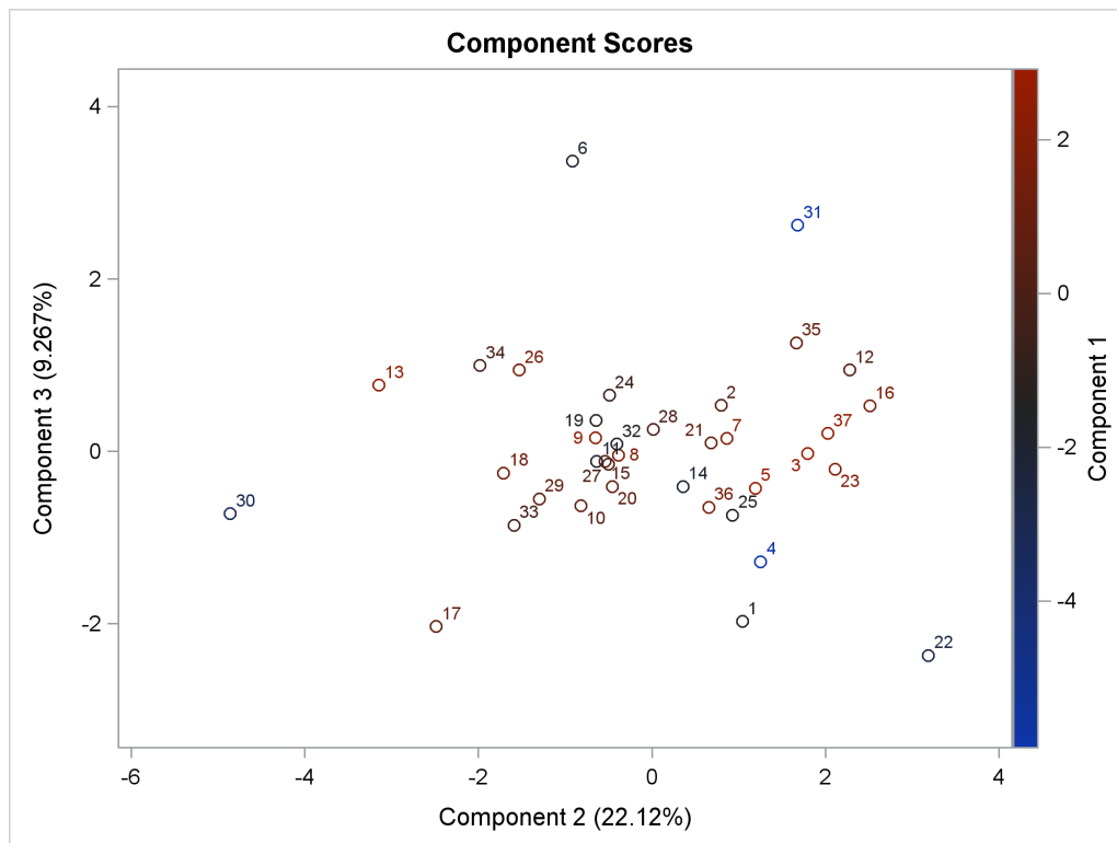
Output 92.3.12 Component 3 versus Component 2, Painted by Component 1
