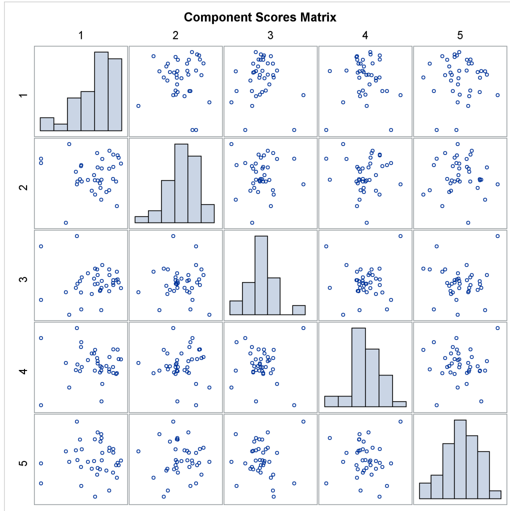
Output 92.3.4 Matrix Plot of Component Scores
