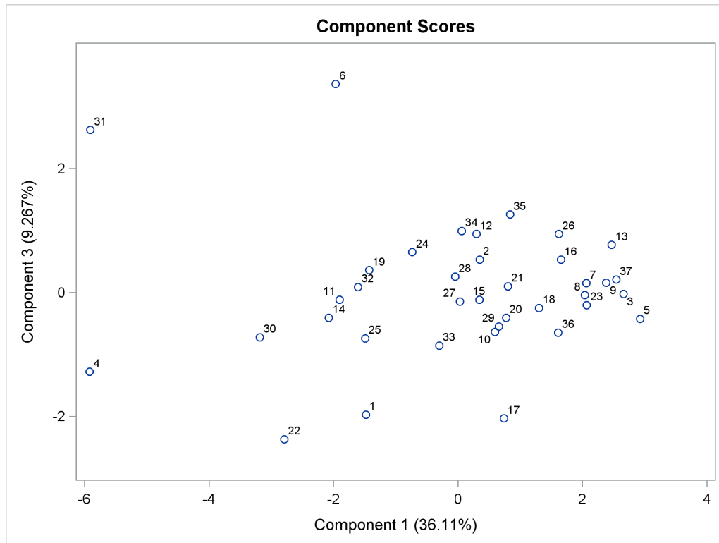
Output 92.3.10 Component 3 versus Component 1
