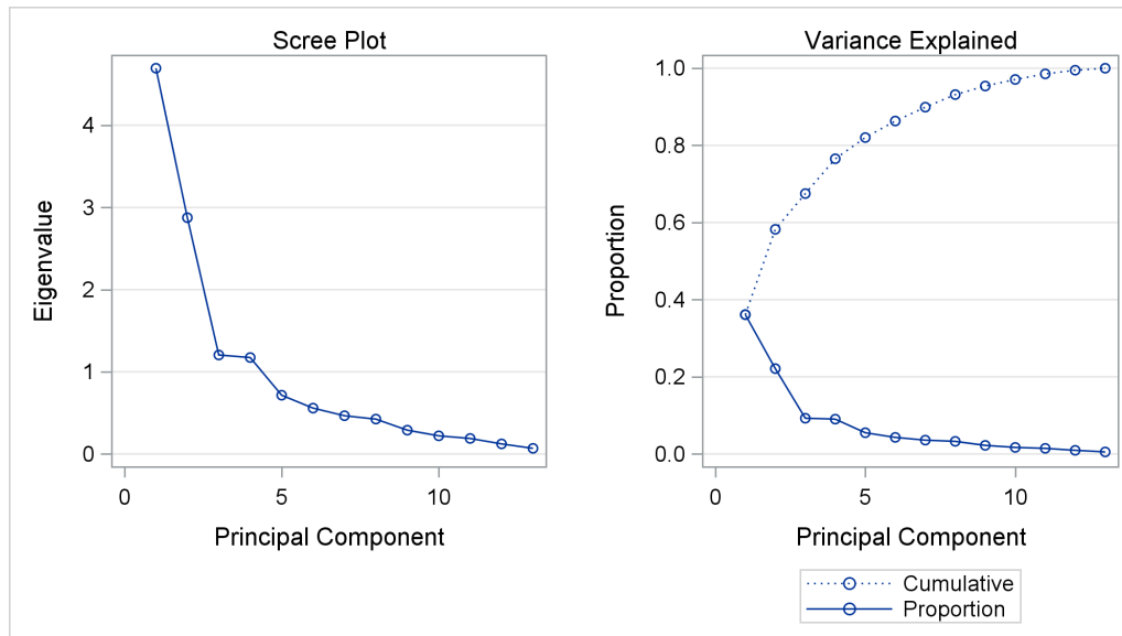
Output 92.3.3 Scree Plot from Using PROC PRINCOMP
