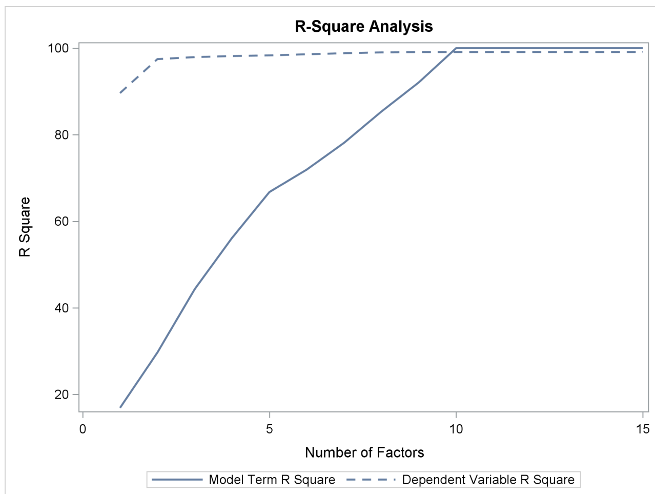
Output 89.1.2 Plot of Proportion of Variation Accounted For
