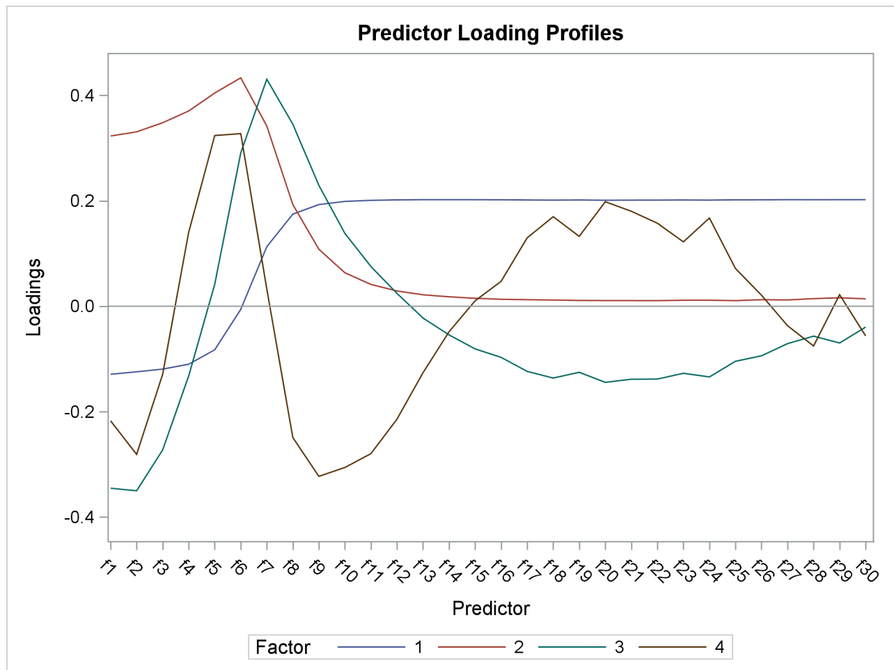
Output 89.3.5 Predictor Loadings across Frequencies
