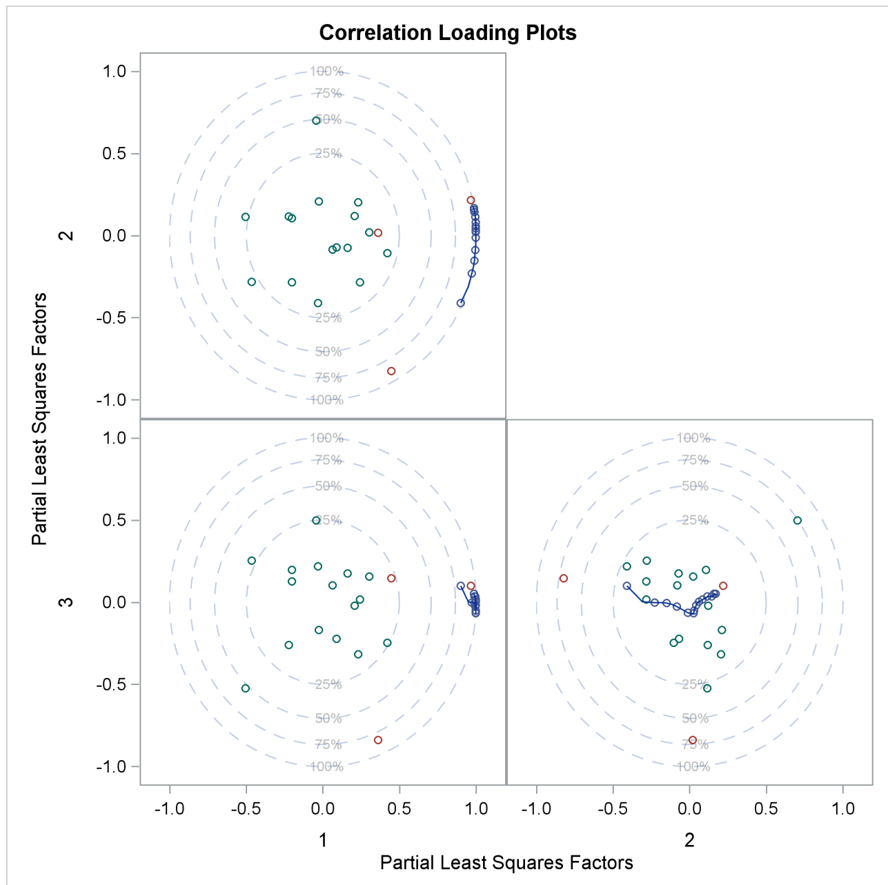
Figure 89.9 Correlation Loading Plot Matrix
