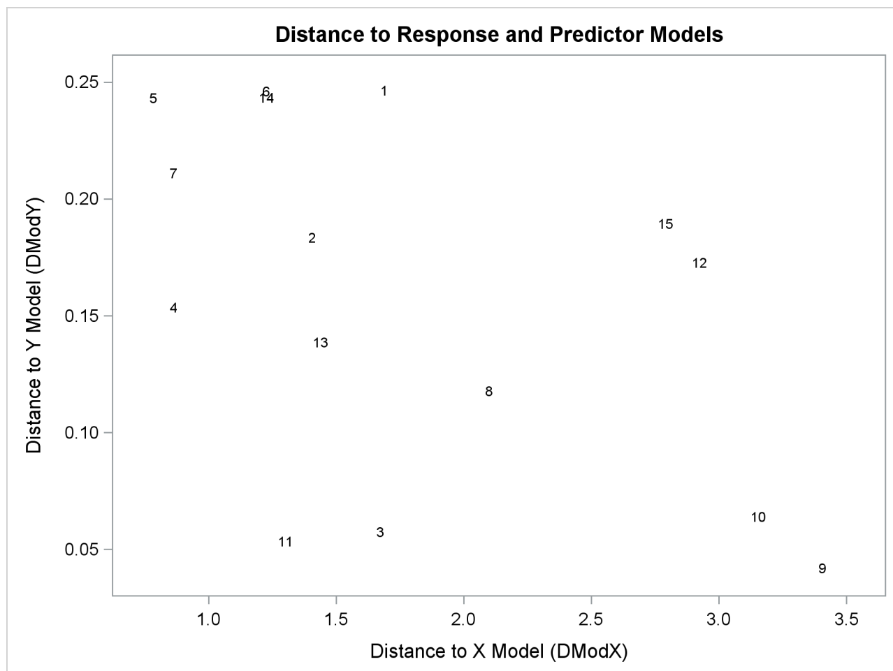
Output 89.2.2 Predictor versus Response Distances to the Model
