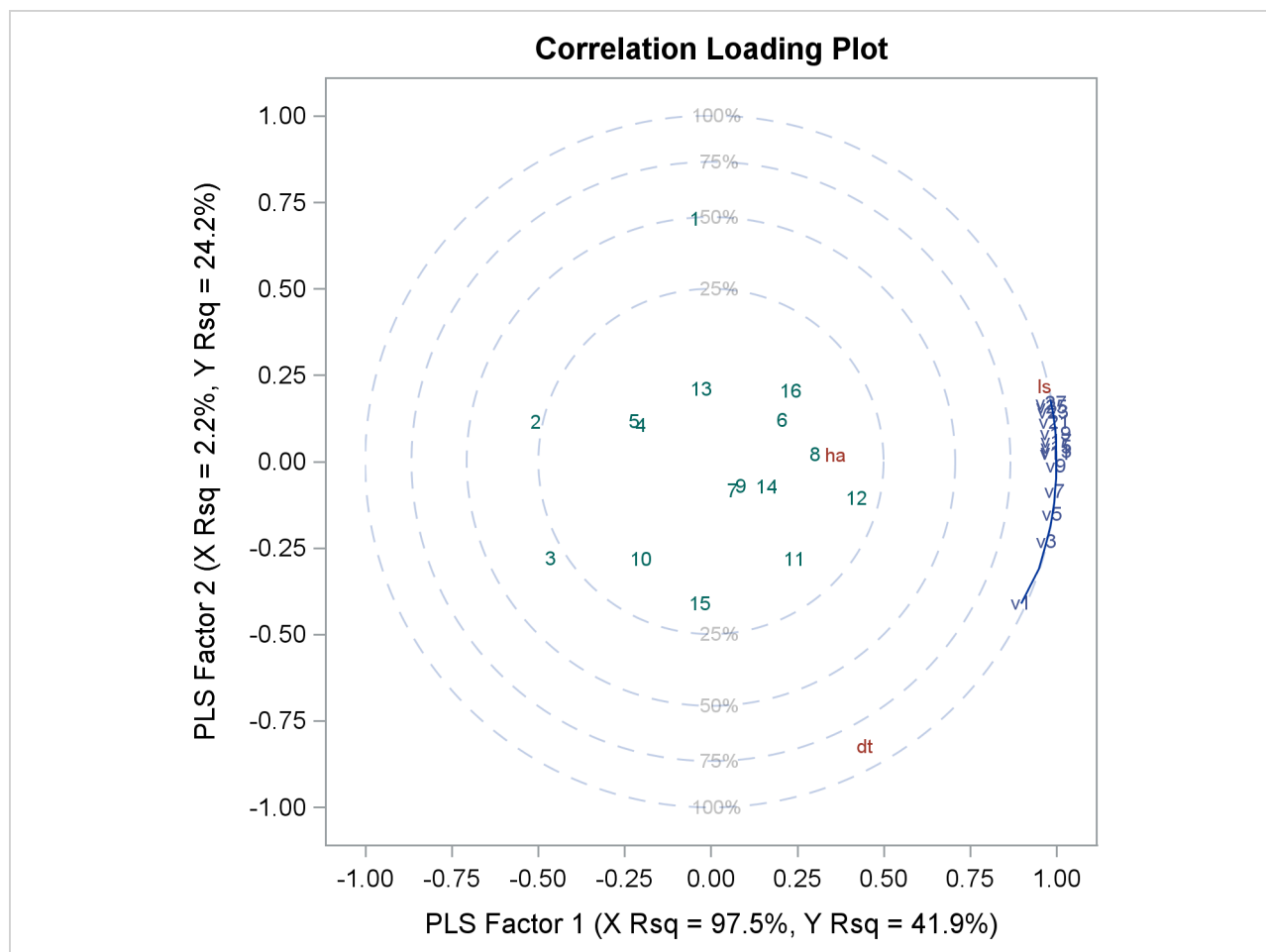
Figure 89.8 Correlation Loading Plot
