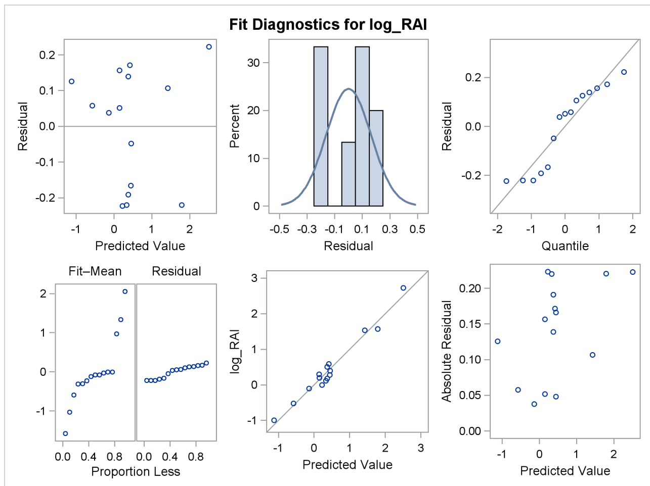
Output 89.2.1 Model Fit Diagnostics
