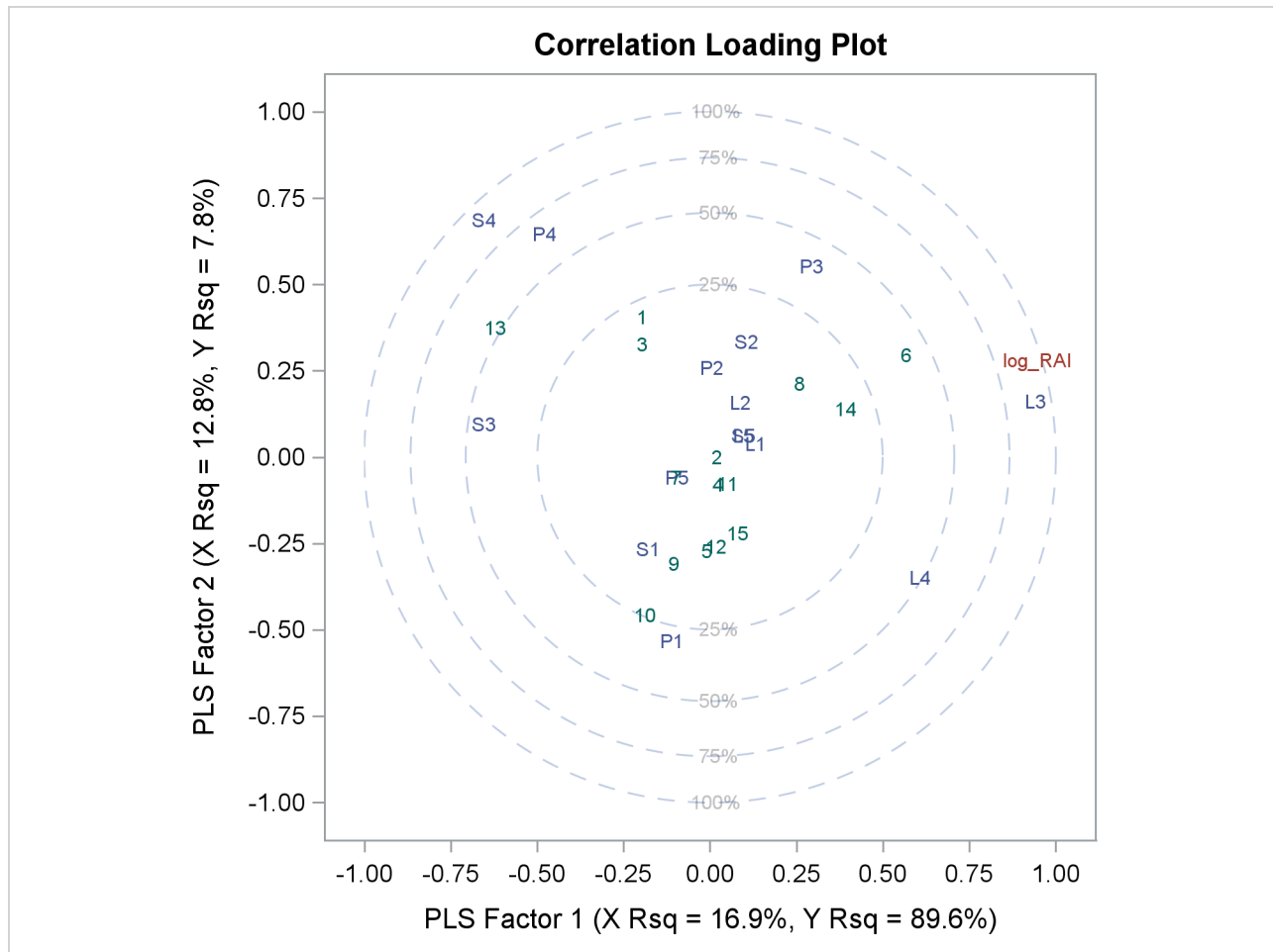
Output 89.1.3 Correlation Loading Plot
