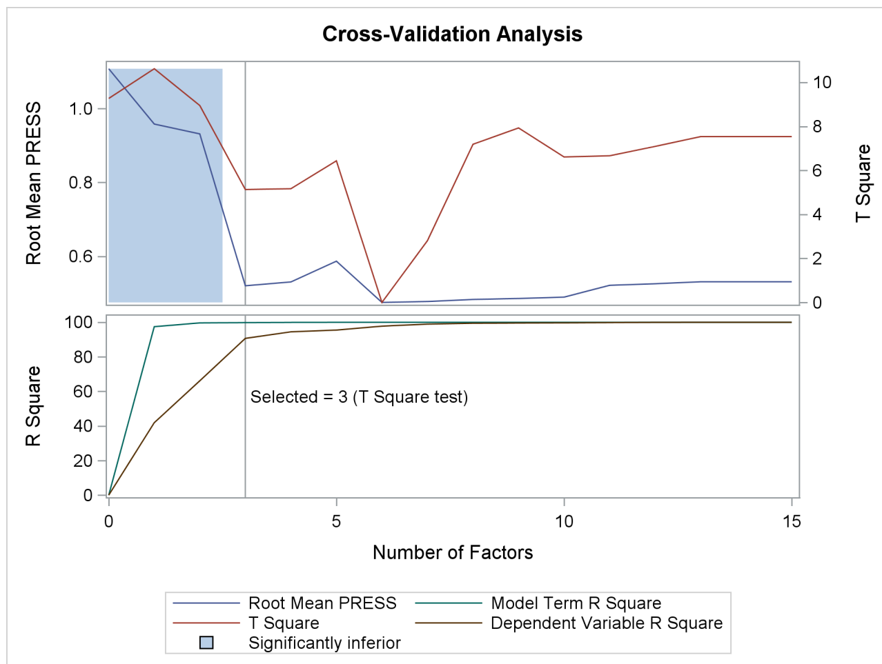
Figure 89.7 Split-Sample Cross Validation Plot
