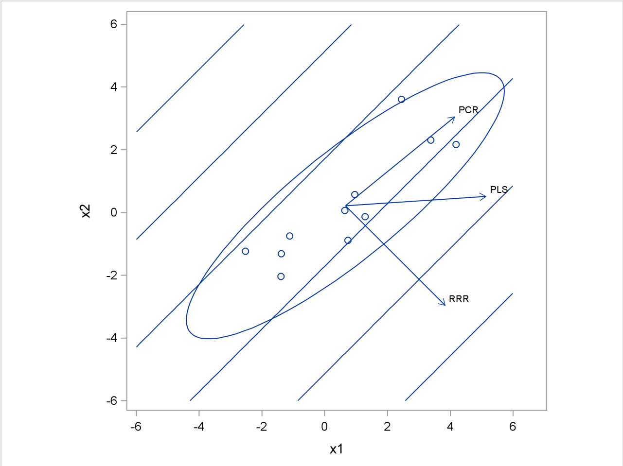
Figure 89.13 Depiction of First Factors for Three Different Regression Methods
