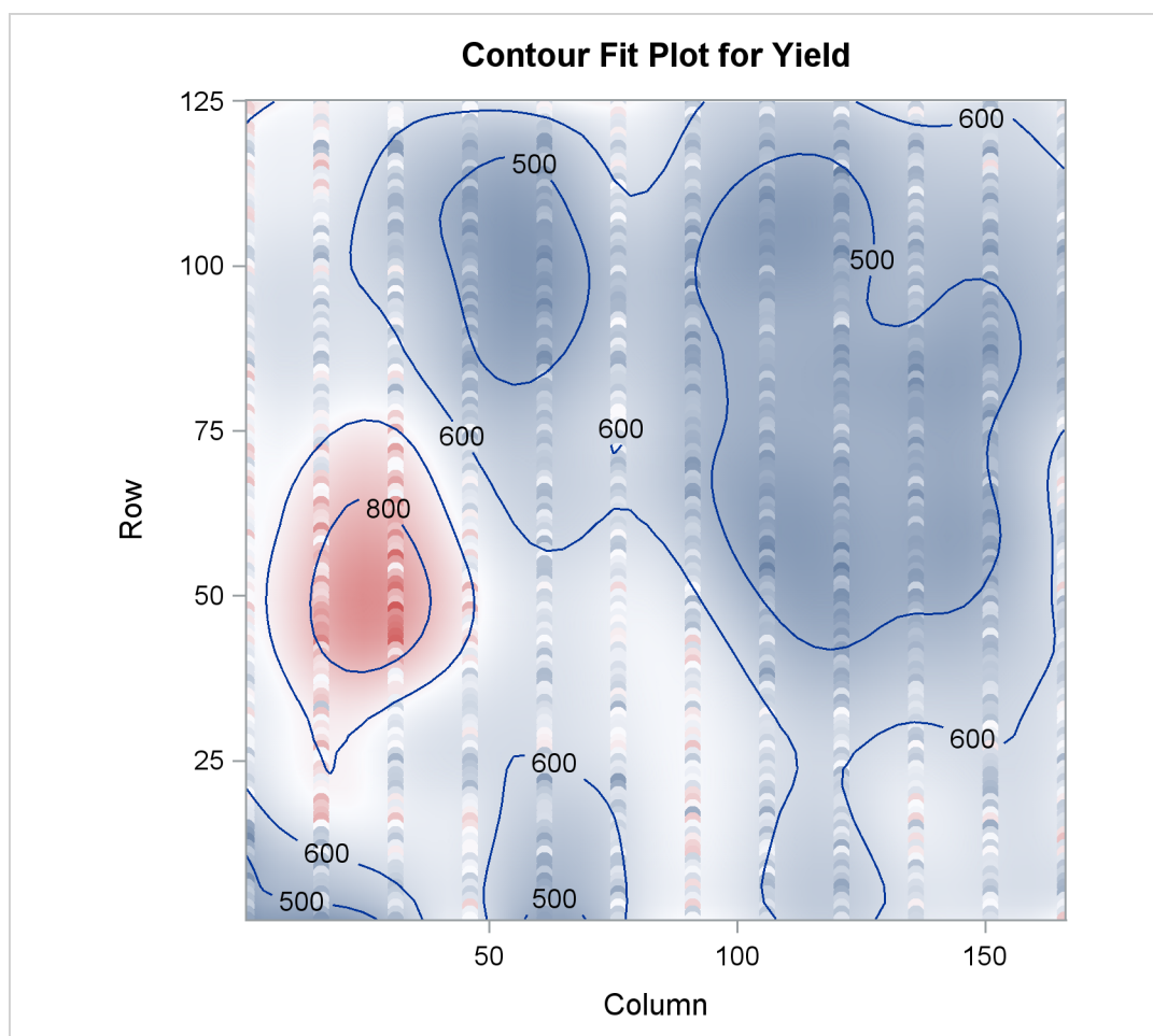
Output 89.4.8 More Granular Spline Basis: Smoothed Yield
