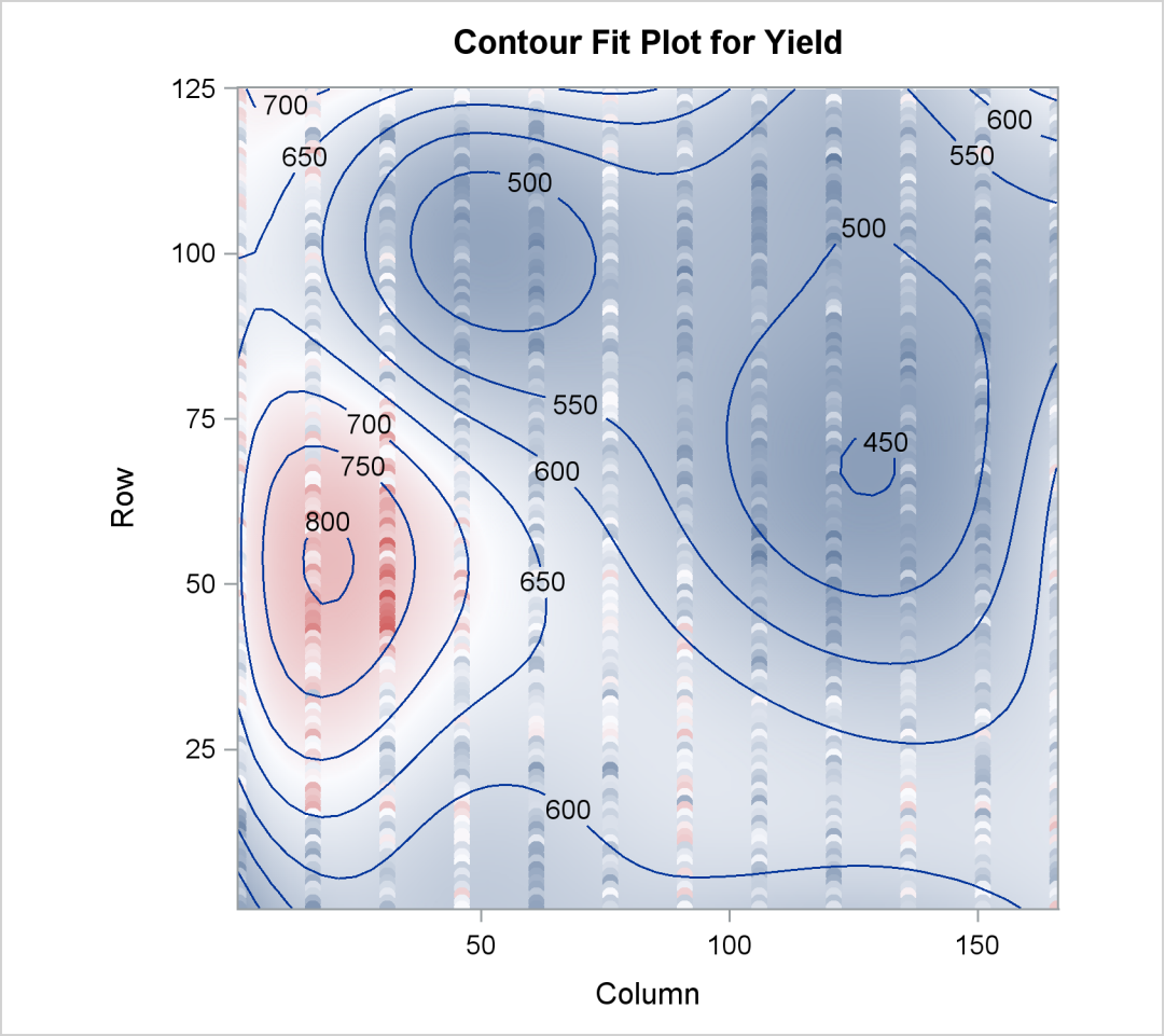
Output 89.4.4 Default Spline Basis: Smoothed Yield
