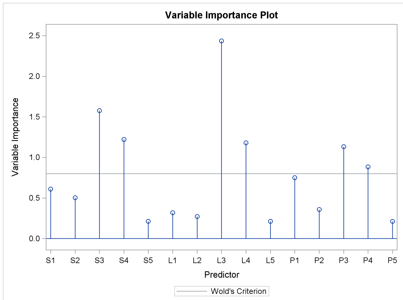
Output 89.1.5 Variable Importance Plots
