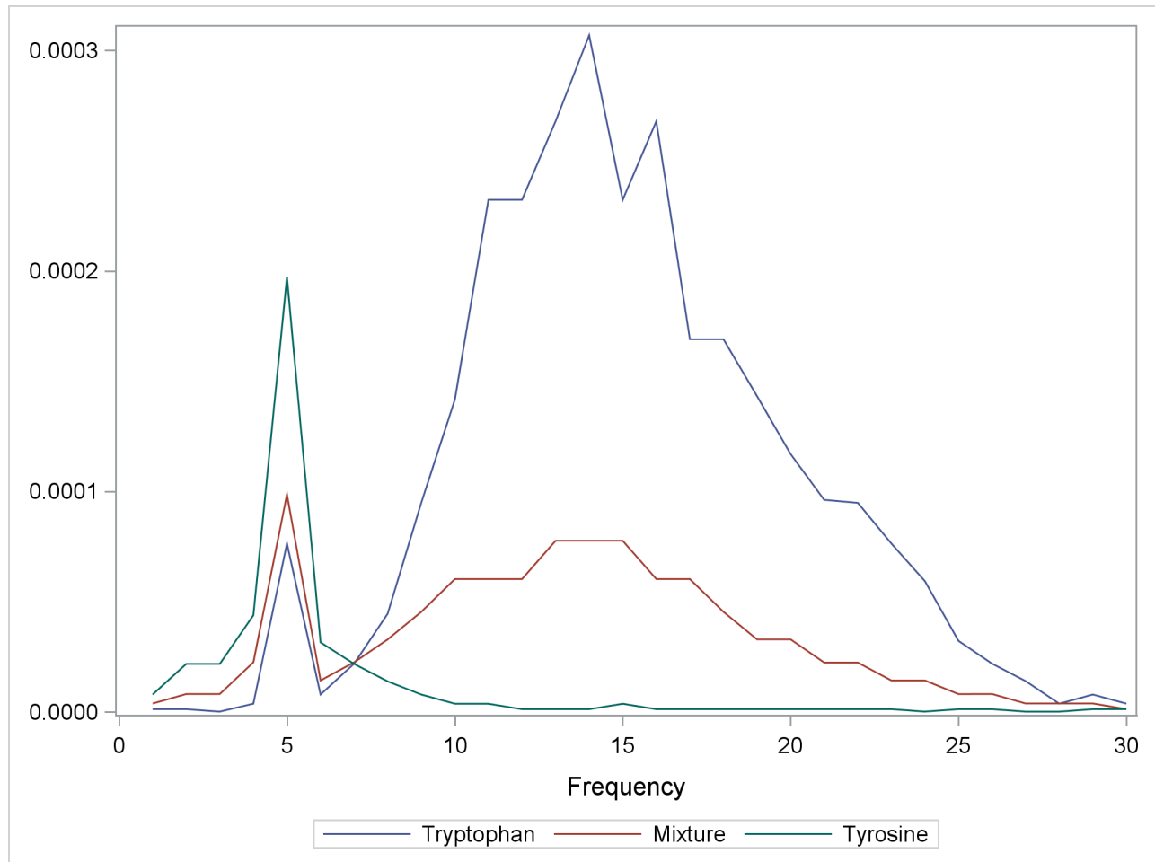
Output 89.3.1 Spectra for Three Samples of Tyrosine and Tryptophan
