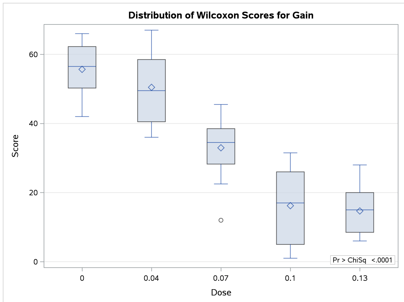
Figure 84.7 Box Plot of Wilcoxon Scores
