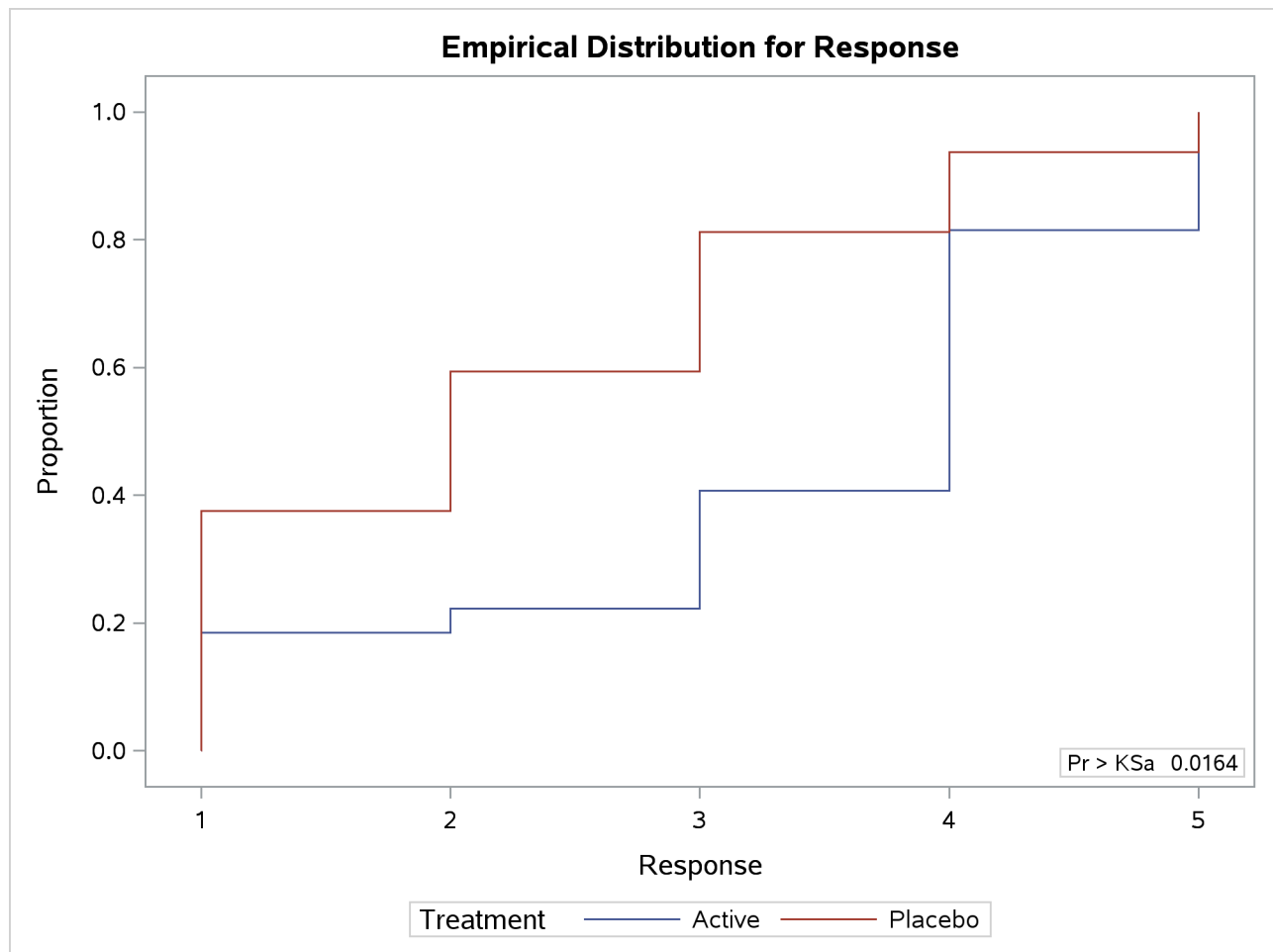
Output 84.2.2 Empirical Distribution Function Plot
