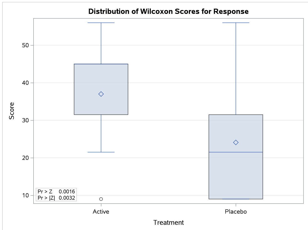
Output 84.1.2 Box Plot of Wilcoxon Scores
