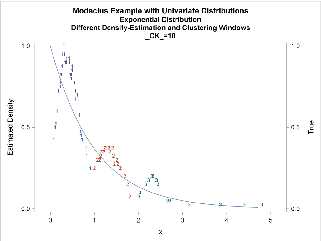
Output 79.1.10 True Density, Estimated Density, and Cluster Membership by _R_=0.2 with Various _CK_ Values
