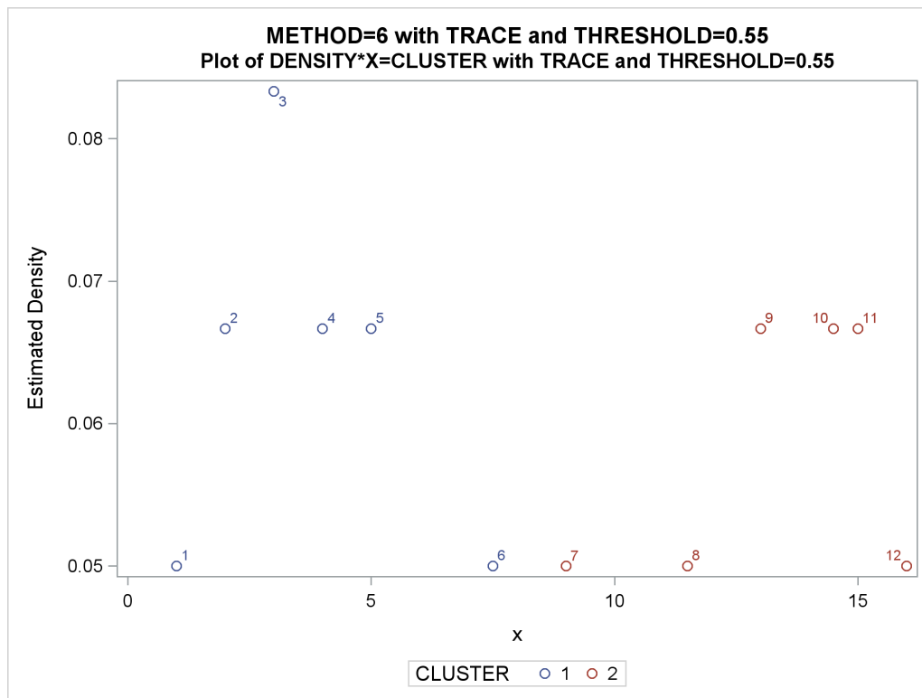
Output 79.5.4 Density Plot
