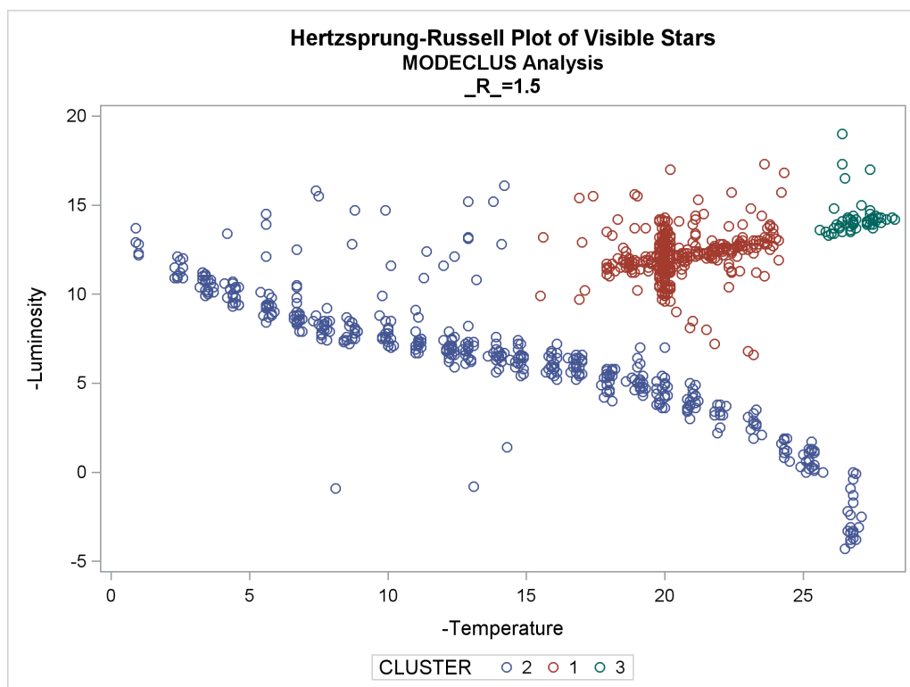
Output 79.4.4 Scatter Plots of Cluster Memberships by \_R\_ = 1.5
