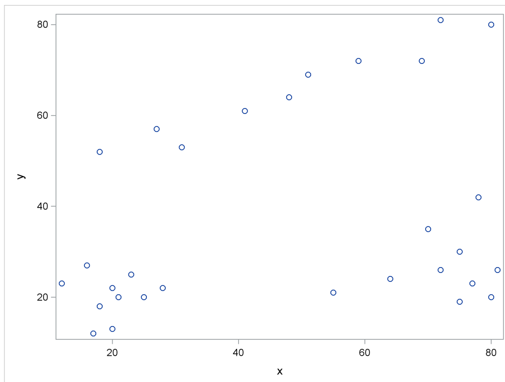
Figure 79.1 Scatter Plot of Data
