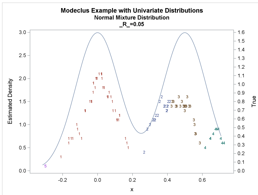
Output 79.1.16 True Density, Estimated Density, and Cluster Membership by Various \_R\_ = Values
