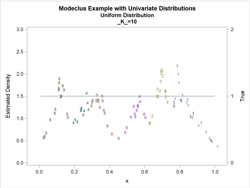
Output 79.1.2 True Density, Estimated Density, and Cluster Membership by Various _K_ Values
