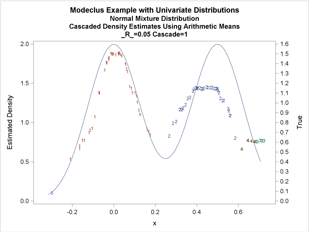
Output 79.1.18 True Density, Estimated Density, and Cluster Membership by _R_=0.05 with Various _CASCAD_ Values
