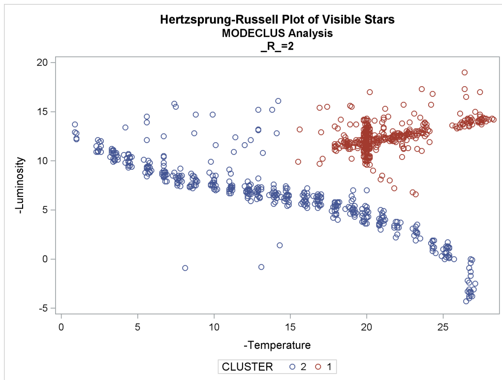
Output 79.4.5 Scatter Plots of Cluster Memberships by _R_=2
