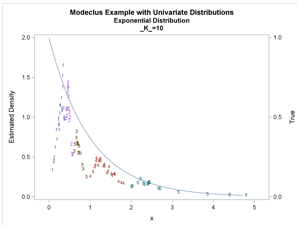
Output 79.1.6 True Density, Estimated Density, and Cluster Membership by Various _K_ Values
