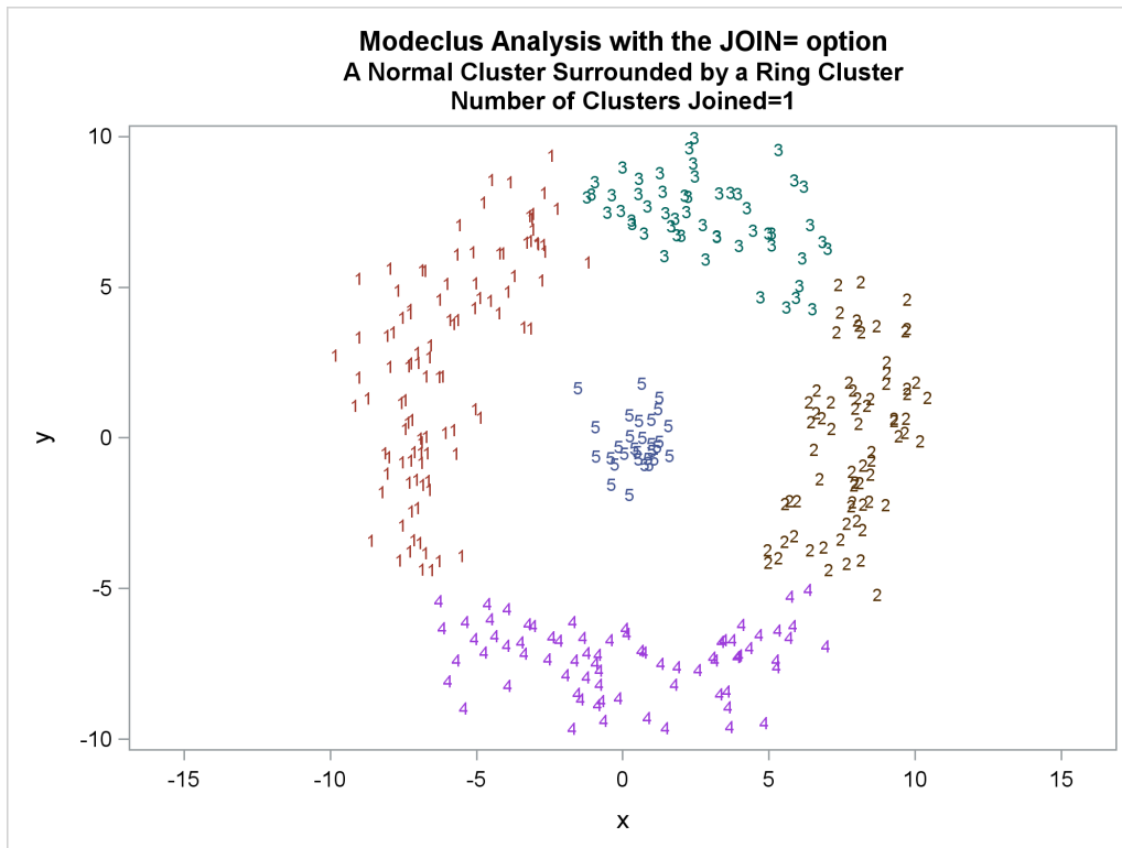
Output 79.3.4 Cluster Memberships When Number of Clusters Joined=1
