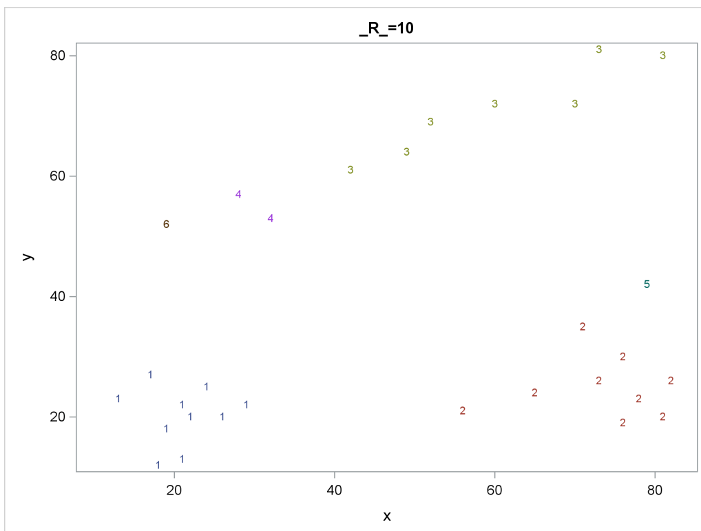
Figure 79.6 Scatter Plots of Cluster Memberships with _R_=10
