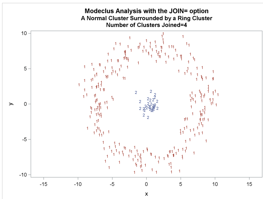
Output 79.3.7 Cluster Memberships When Number of Clusters Joined=4
