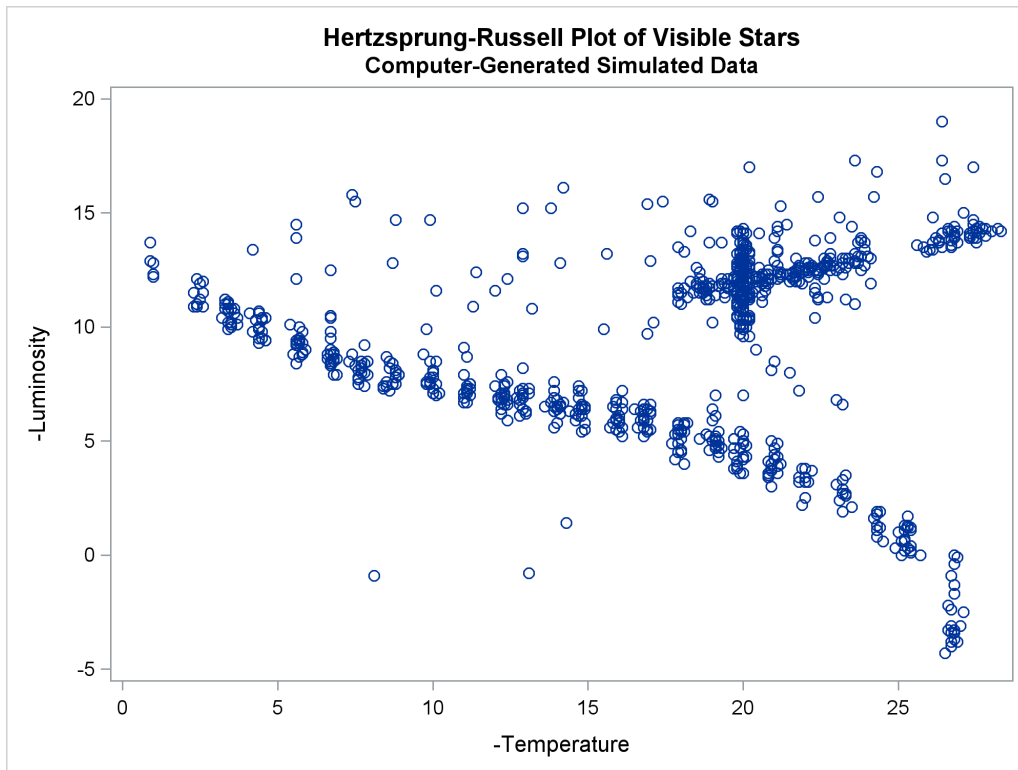
Output 79.4.1 Scatter Plot of Data
