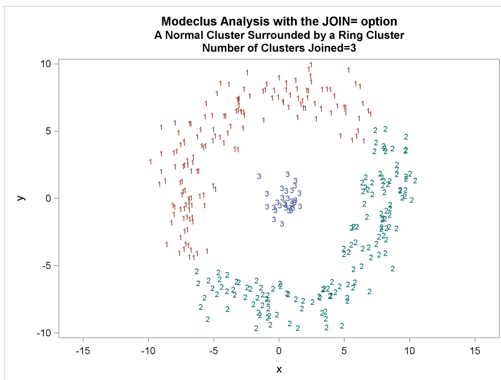
Output 79.3.6 Cluster Memberships When Number of Clusters Joined=3
