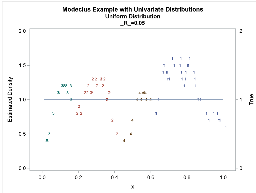
Output 79.1.4 True Density, Estimated Density, and Cluster Membership by Various \_R\_ Values
