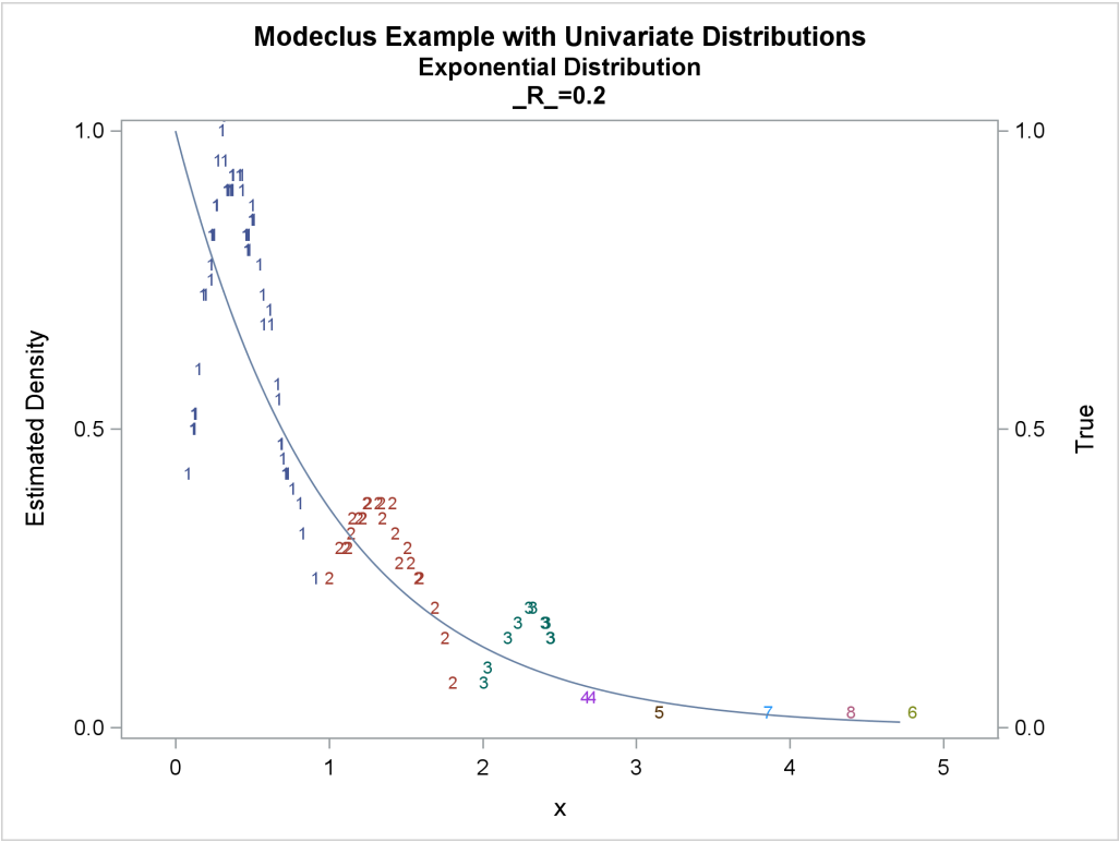
Output 79.1.8 True Density, Estimated Density, and Cluster Membership by Various _R_ Values
