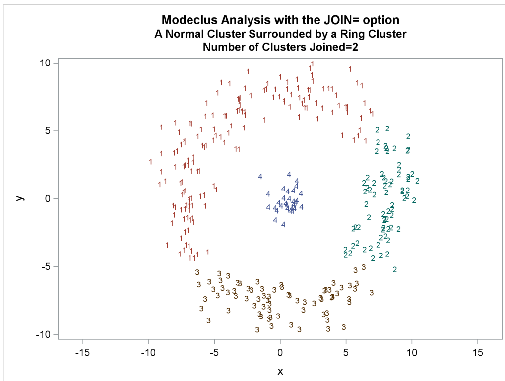
Output 79.3.5 Cluster Memberships When Number of Clusters Joined=2
