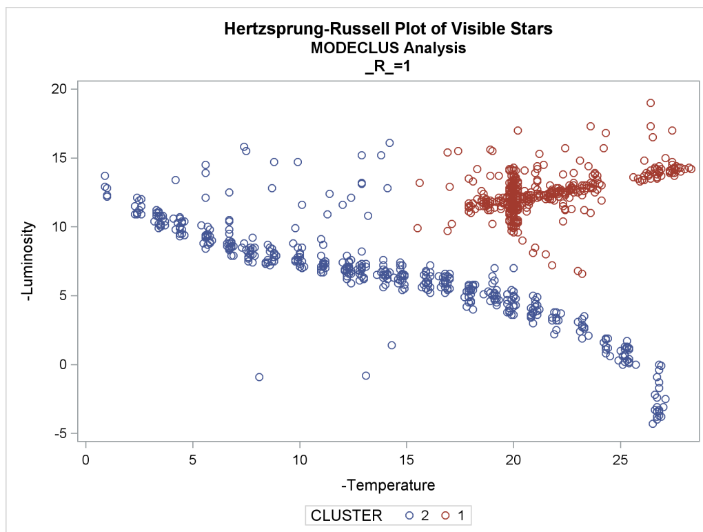
Output 79.4.3 Scatter Plots of Cluster Memberships by \_R\_ = 1
