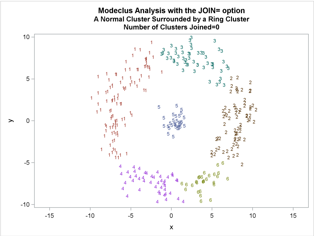
Output 79.3.3 Cluster Memberships When Number of Clusters Joined=0
