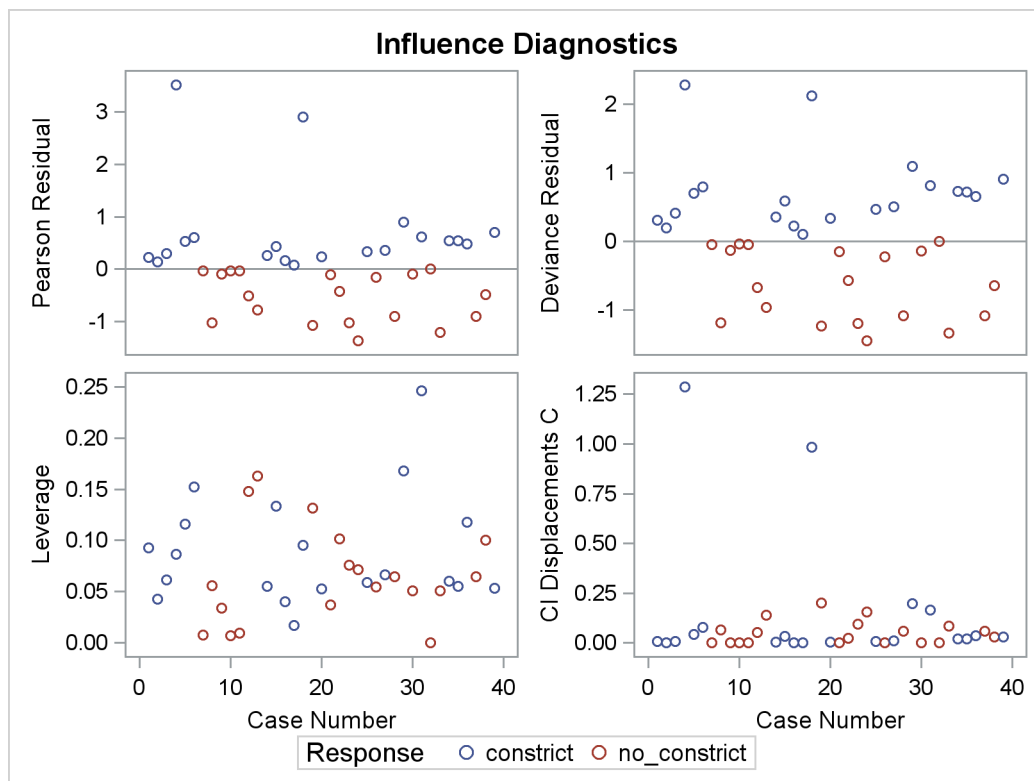
Output 73.6.3 Residuals, Hat Matrix, and CI Displacement C
