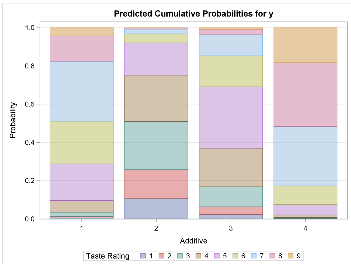
Output 73.3.5 Model-Predicted Probabilities
