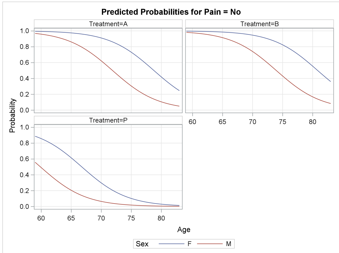
Output 73.2.12 Model-Predicted Probabilities by Treatment
