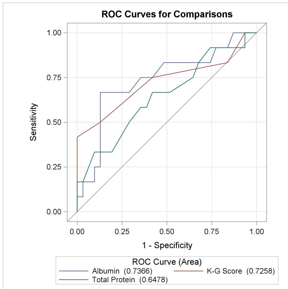
Output 73.8.8 Overlay of All Models Being Compared
