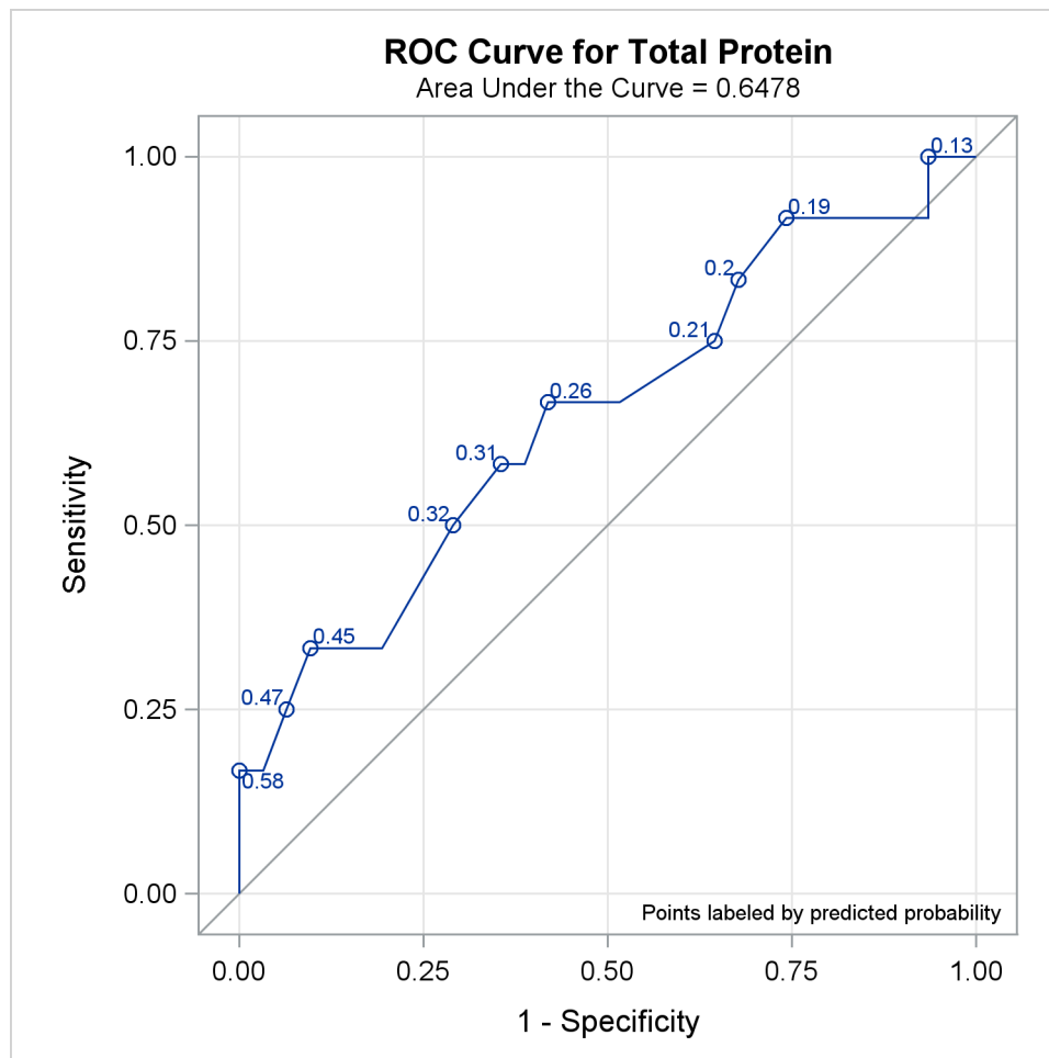
Output 73.8.7 ROC Curve for Popind=Tp
