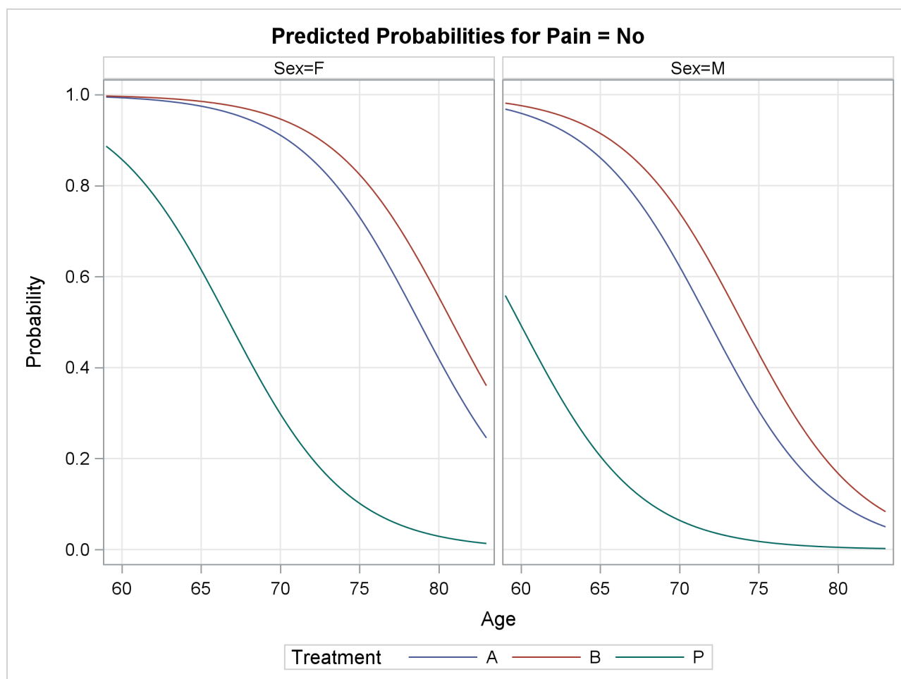
Output 73.2.11 Model-Predicted Probabilities by Sex
