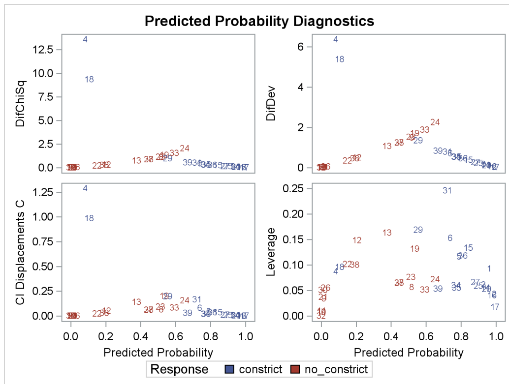
Output 73.6.6 Diagnostics versus Predicted Probability
