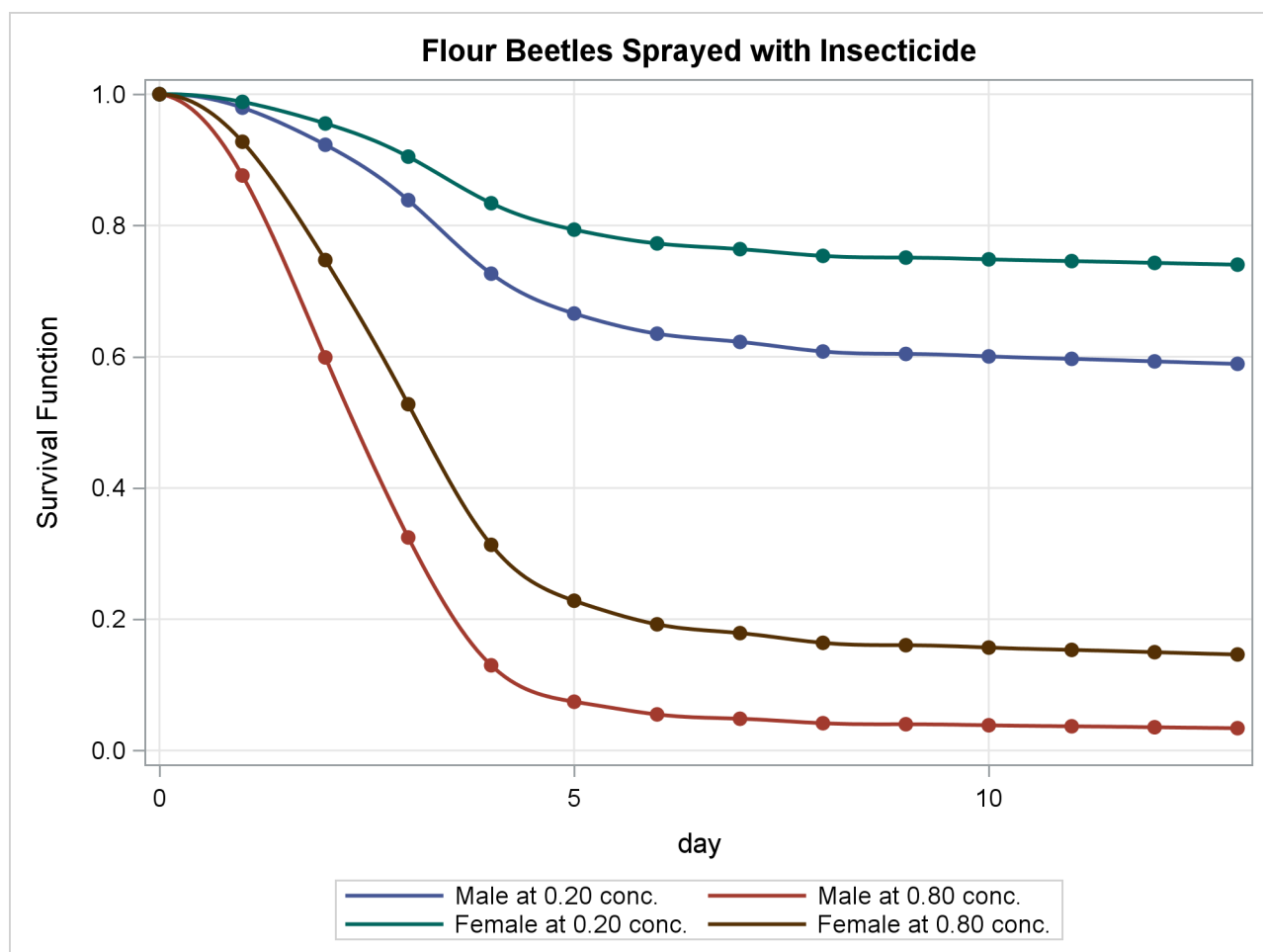
Output 73.15.4 Predicted Survival at Insecticide Concentrations of 0.20 and 0.80 mg/cm 2
