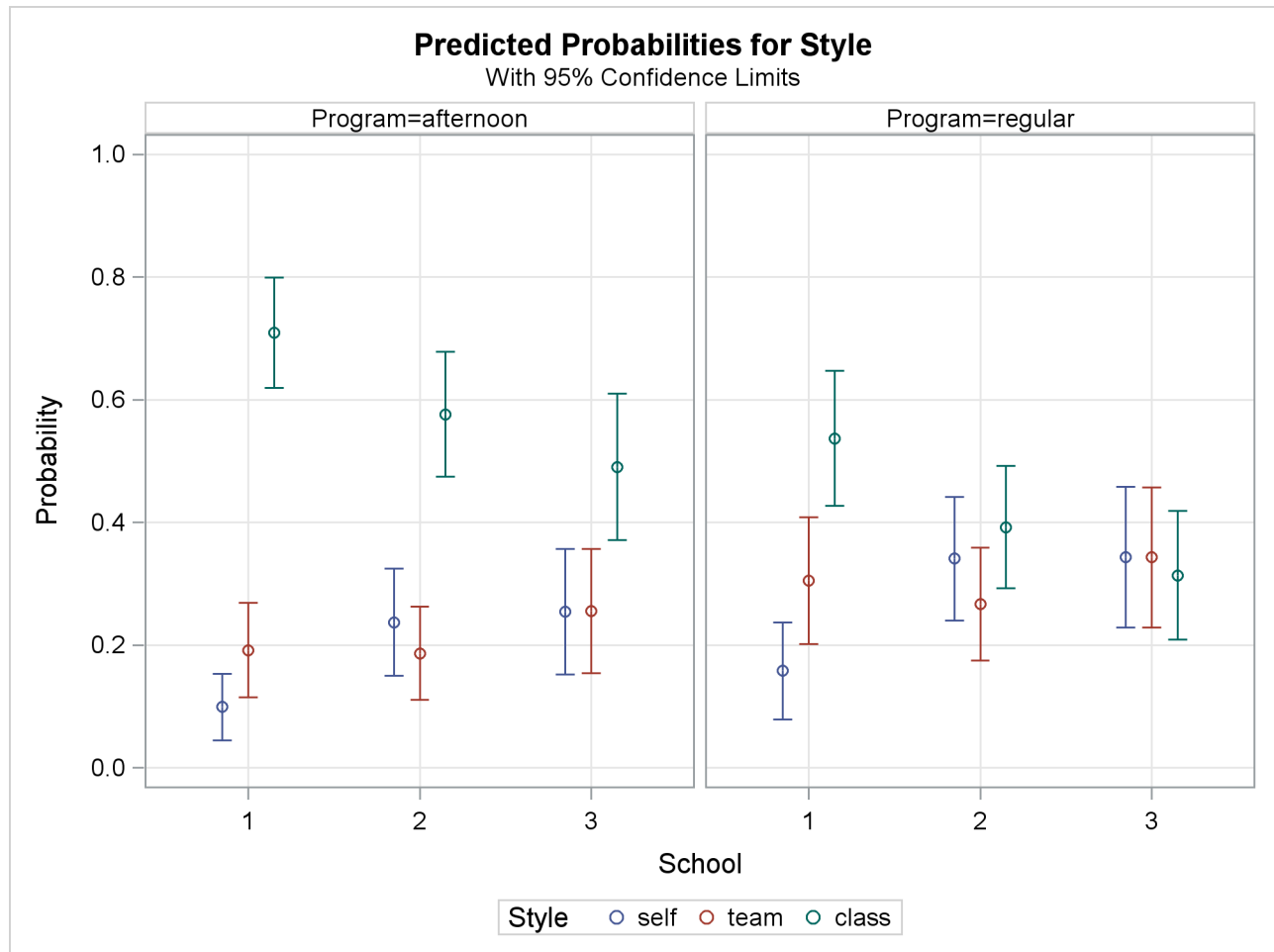
Output 73.4.8 Model-Predicted Probabilities
