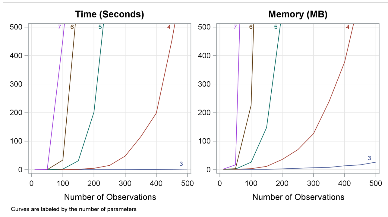
Figure 73.11 Mean Time and Memory Required
