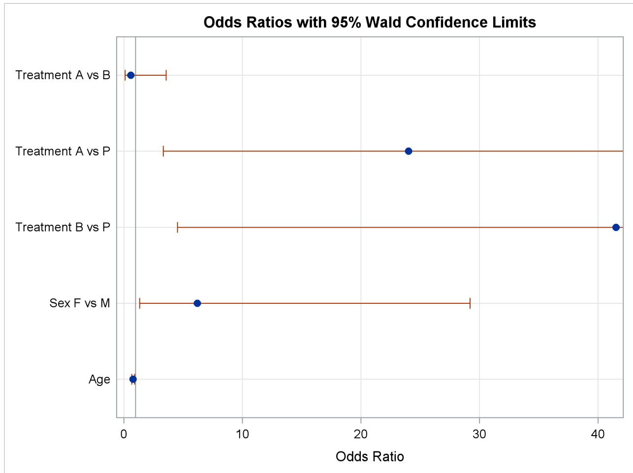
Output 73.2.9 Plot of the ODDSRATIO Statement Results
