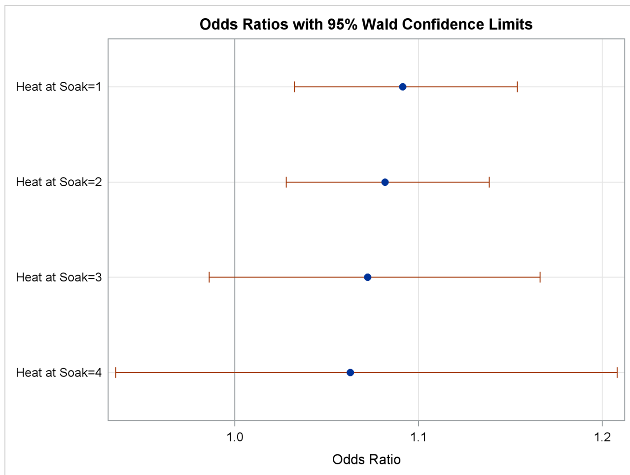
Figure 73.7 Plot of Odds Ratios of Heat at Several Values of Soak
