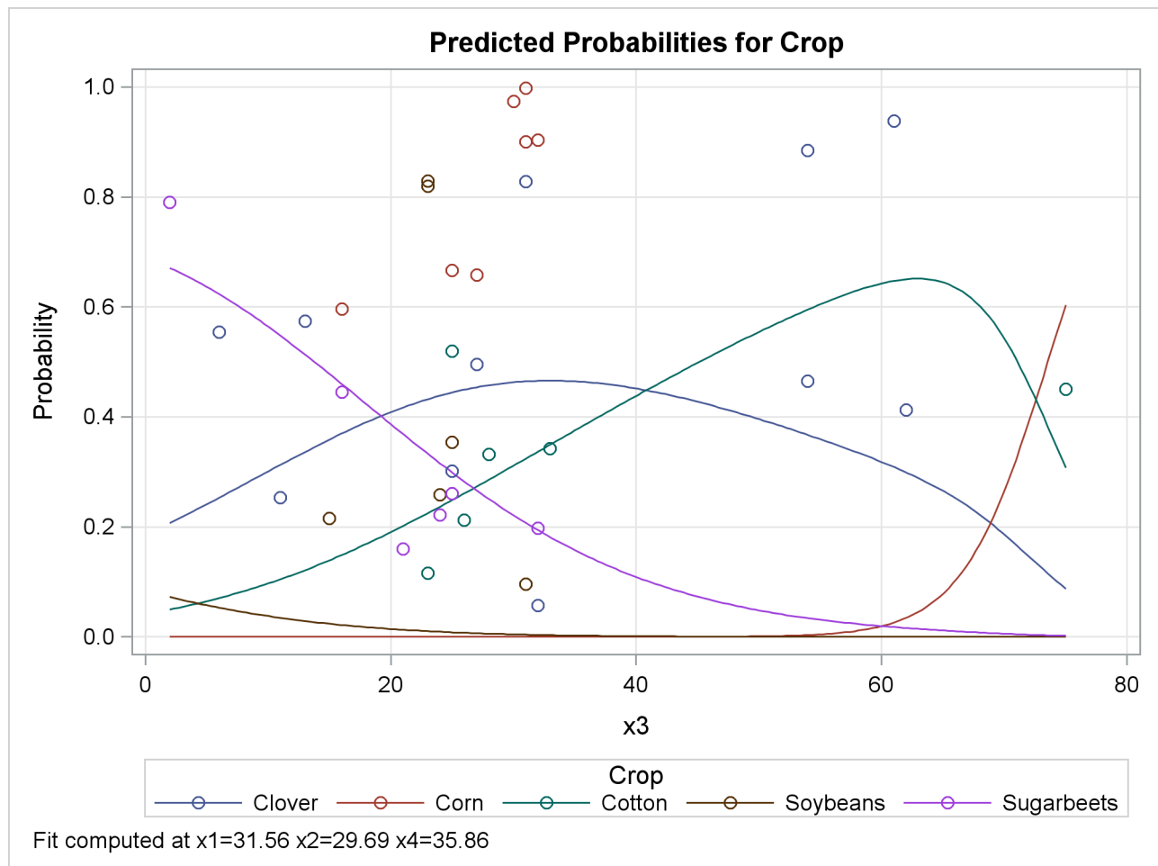
Output 73.16.4 Model-Predicted Probabilities
