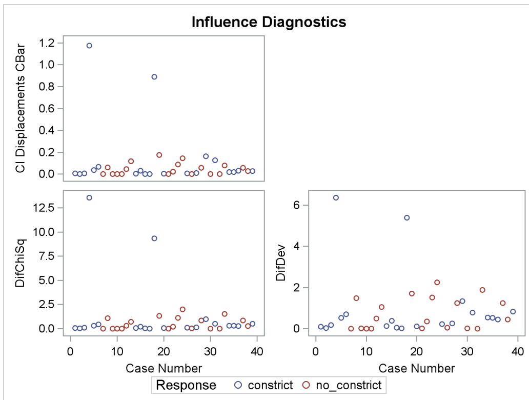
Output 73.6.4 CI Displacement CBar, Change in Deviance and Pearson Chi-Square
