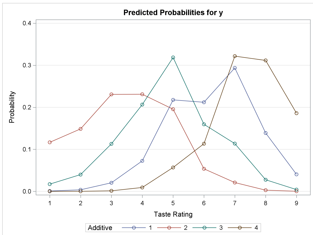
Output 73.3.8 Model-Predicted Probabilities
