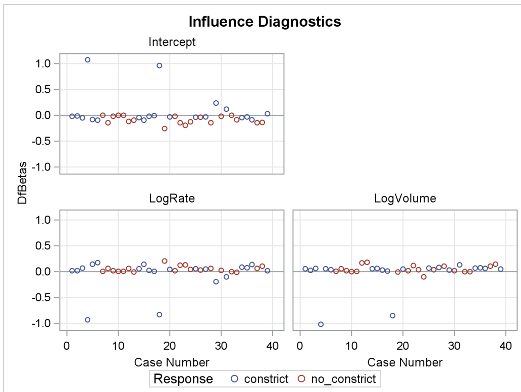
Output 73.6.5 DFBETAS Plots
