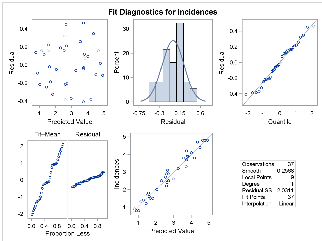
Figure 72.12 Fit Diagnostics
