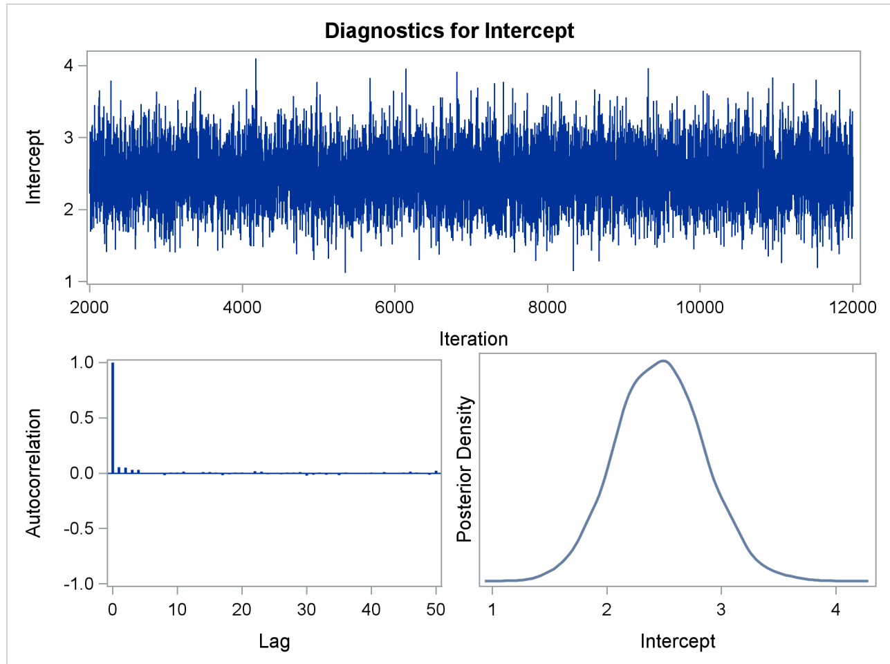
Output 70.7.6 Diagnostic Plots
