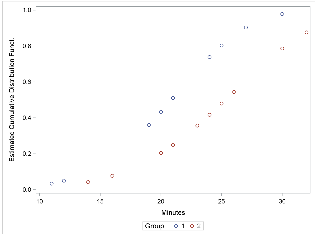
Figure 70.5 Plot of the Estimated Cumulative Distribution Function
