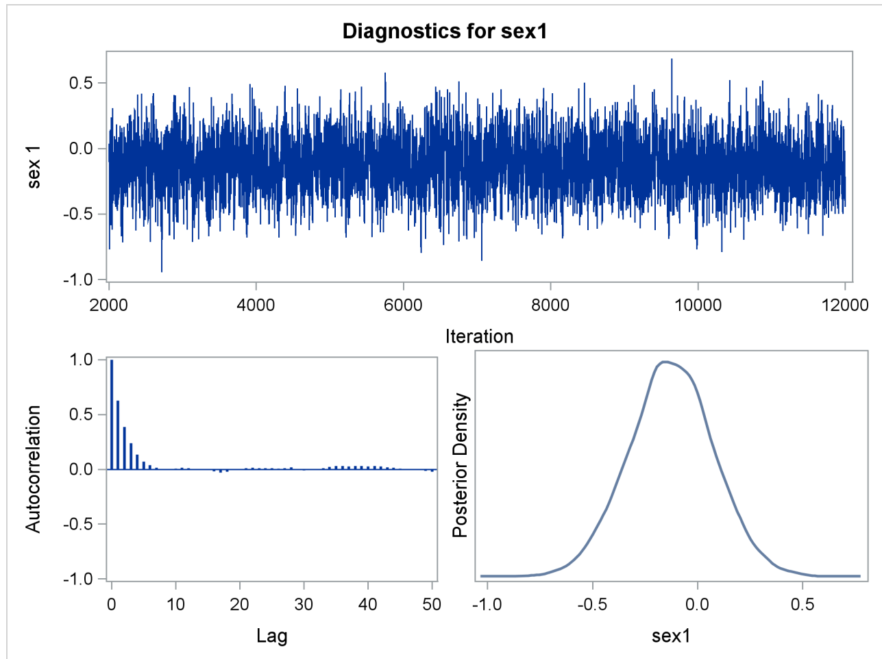
Output 70.7.8 Diagnostic Plots
