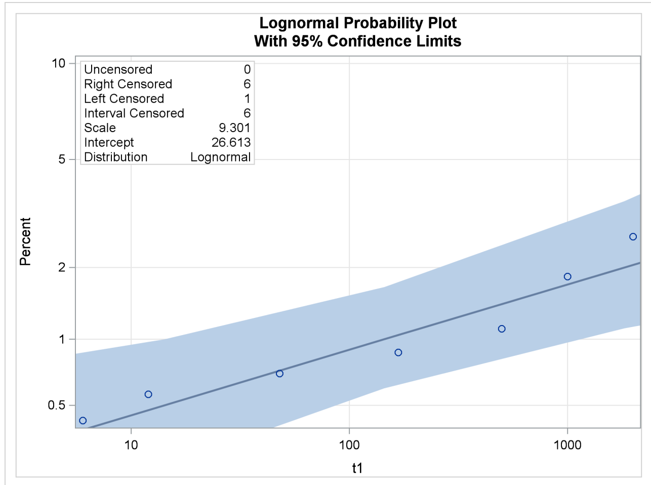
Output 70.6.4 Lognormal Probability Plot for the Microprocessor Data
