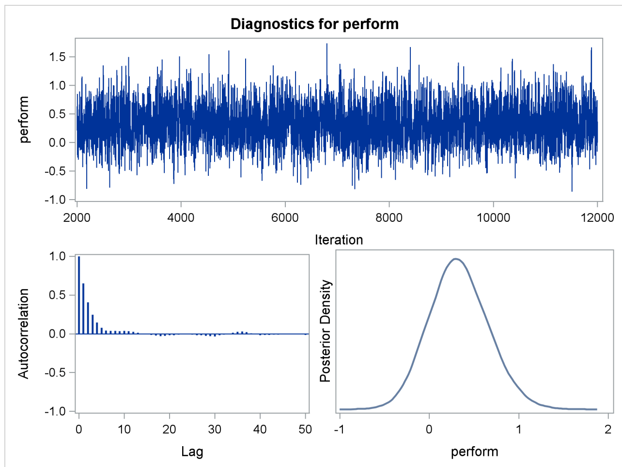
Output 70.7.9 Diagnostic Plots
