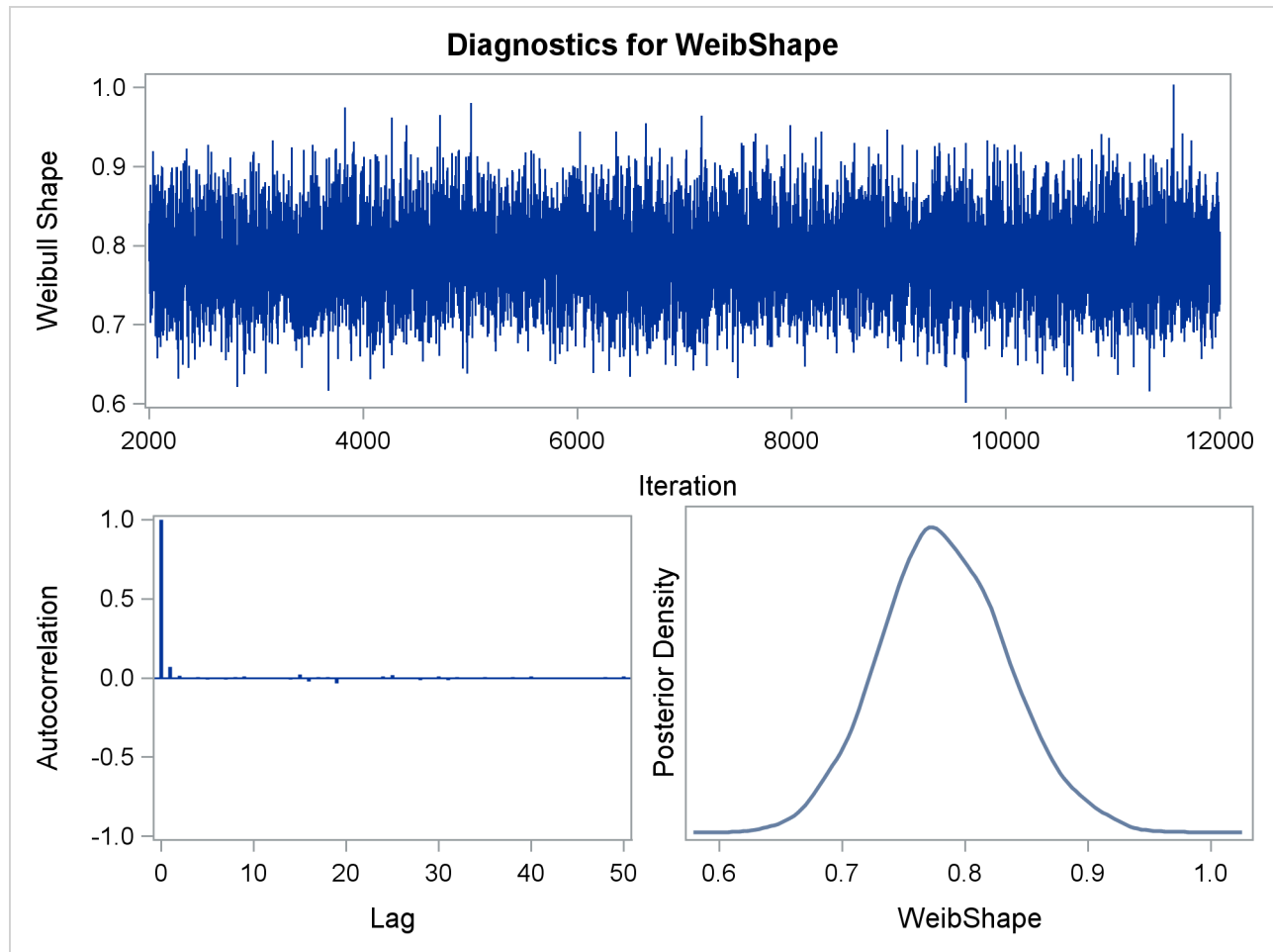
Output 70.7.10 Diagnostic Plots
