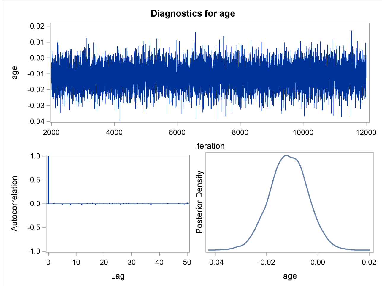
Output 70.7.7 Diagnostic Plots
