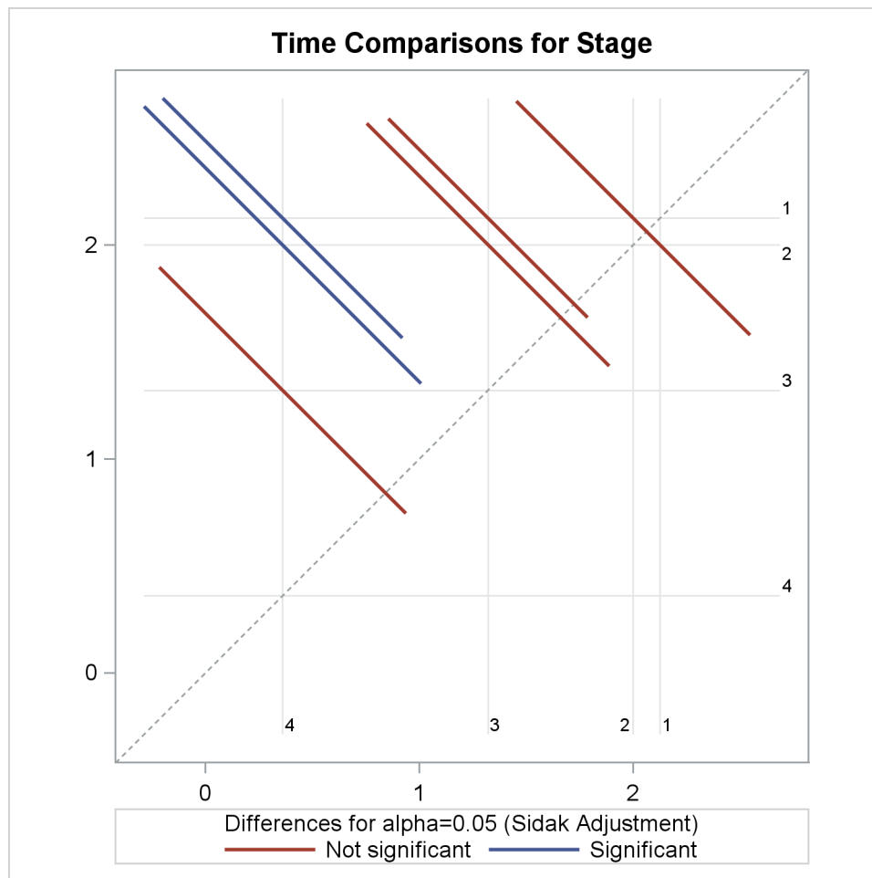
Output 70.8.2 Plot of Pairwise LS-Means Differences
