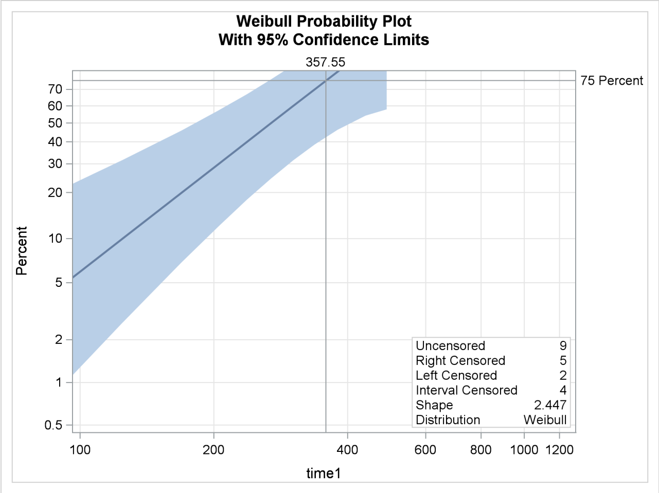
Output 70.4.2 Probability Plot for Recovery Time with sex = 1, age = 50
