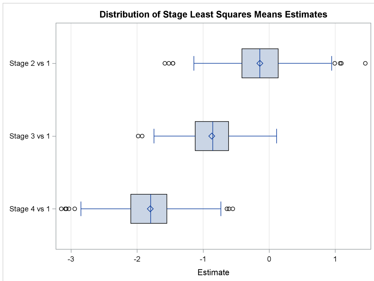
Output 70.8.7 Box Plot of Sampled LS-Means Differences
