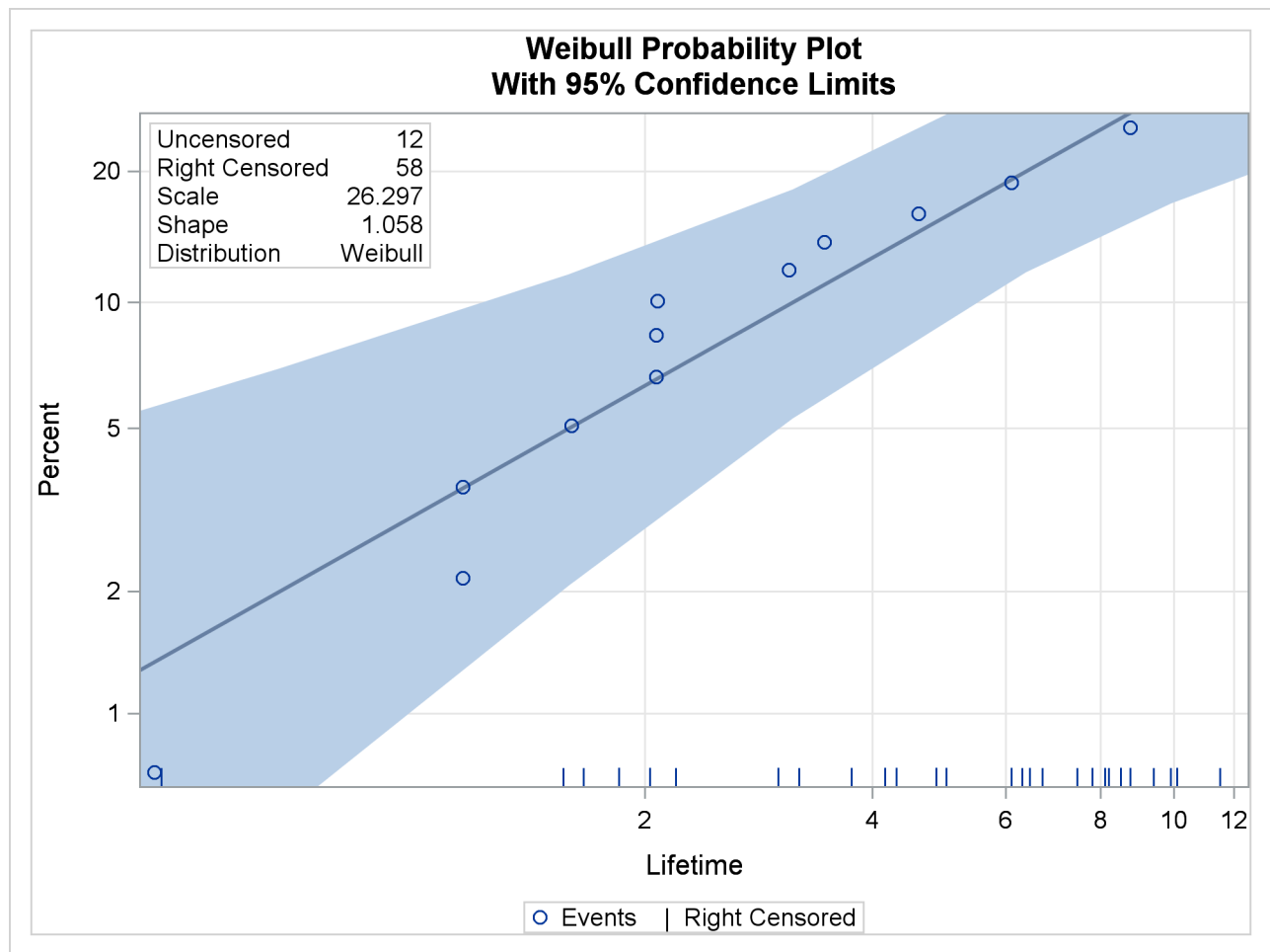
Output 70.5.1 Probability Plot for the Fan Data
