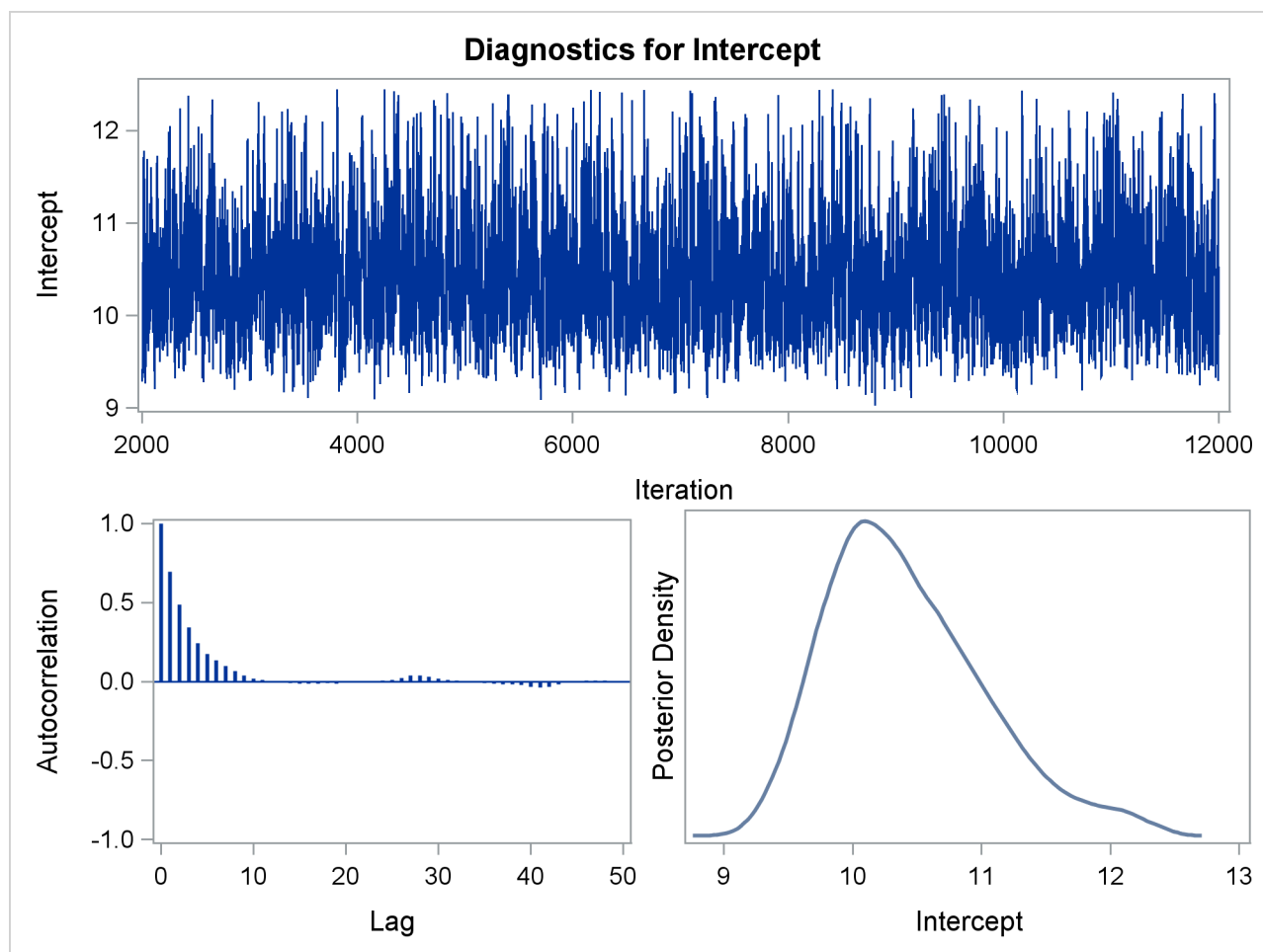
Figure 70.11 Diagnostic Plots
