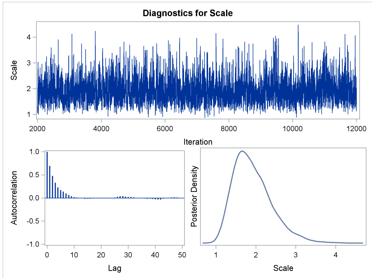
Figure 70.12 Diagnostic Plots
