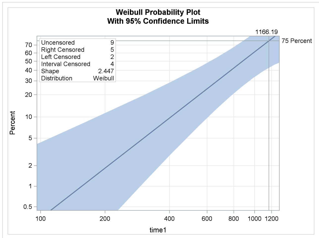
Output 70.4.3 Probability Plot for Recovery Time with sex = 2, age = 60.6
