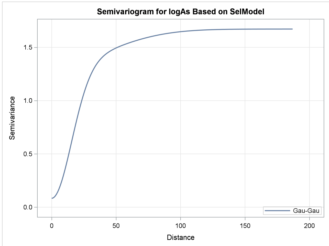
Output 68.1.6 Gaussian-Gaussian Semivariogram Model Used in Kriging Predictions
