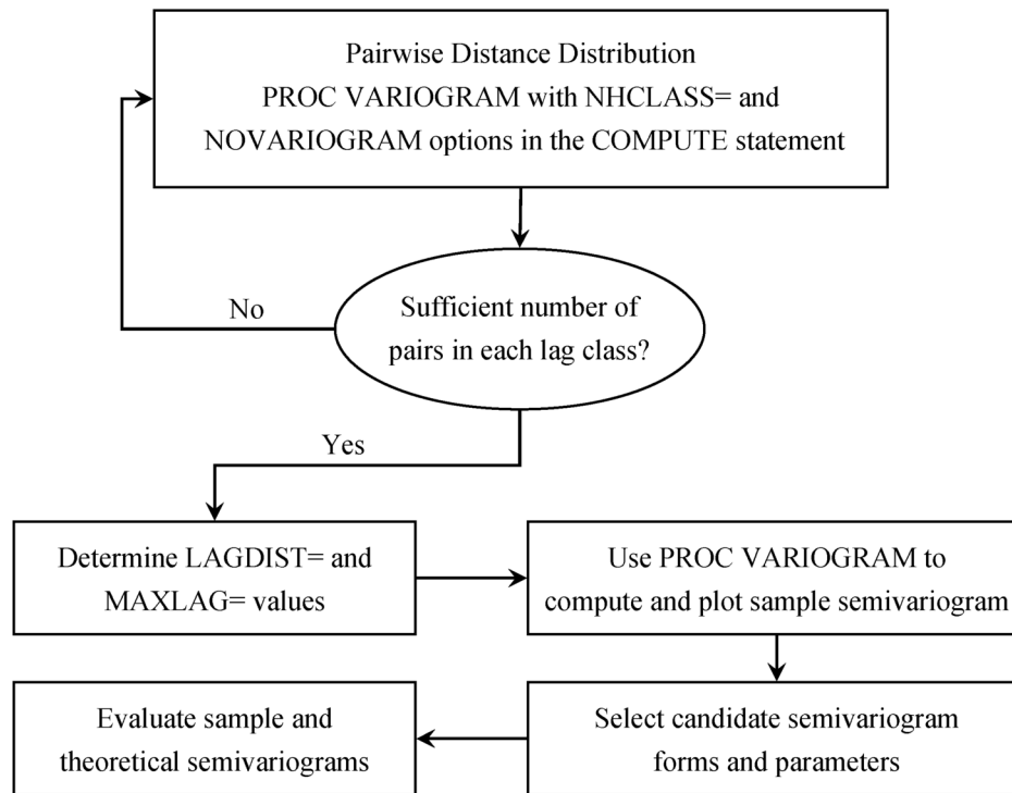
Figure 68.5 Flowchart for Semivariogram Selection
