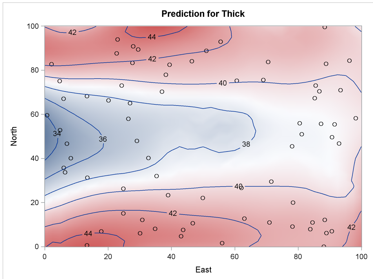
Output 68.3.3 Surface Plot and Contours of Kriged Coal Seam Thickness
