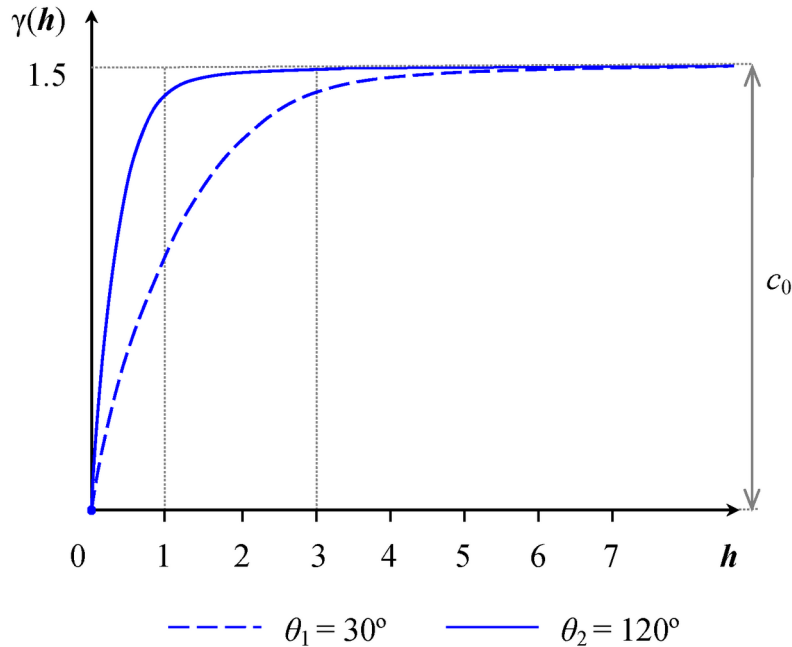
Figure 68.12 Geometric Anisotropy with Major Axis in the Direction \theta_1 = 30^\circ
