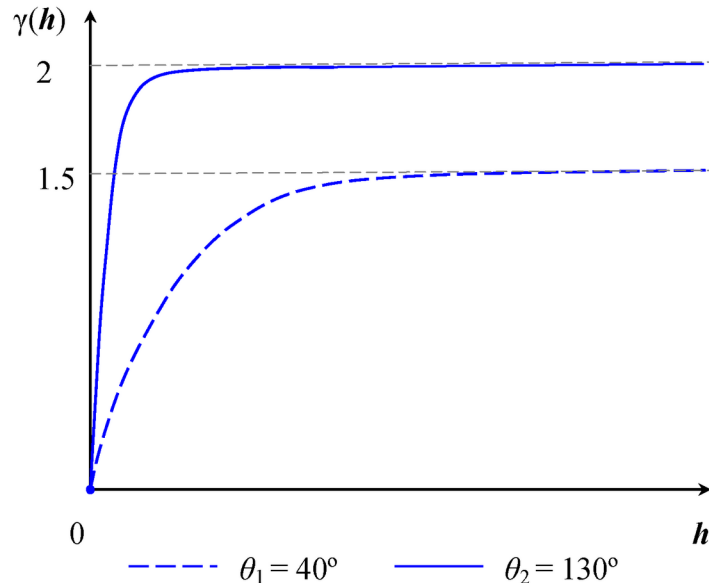
Figure 68.14 Zonal Anisotropy in Two Directions
