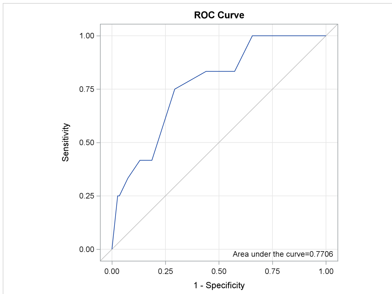
Output 55.2.11 Receiver Operating Characteristics Curve
