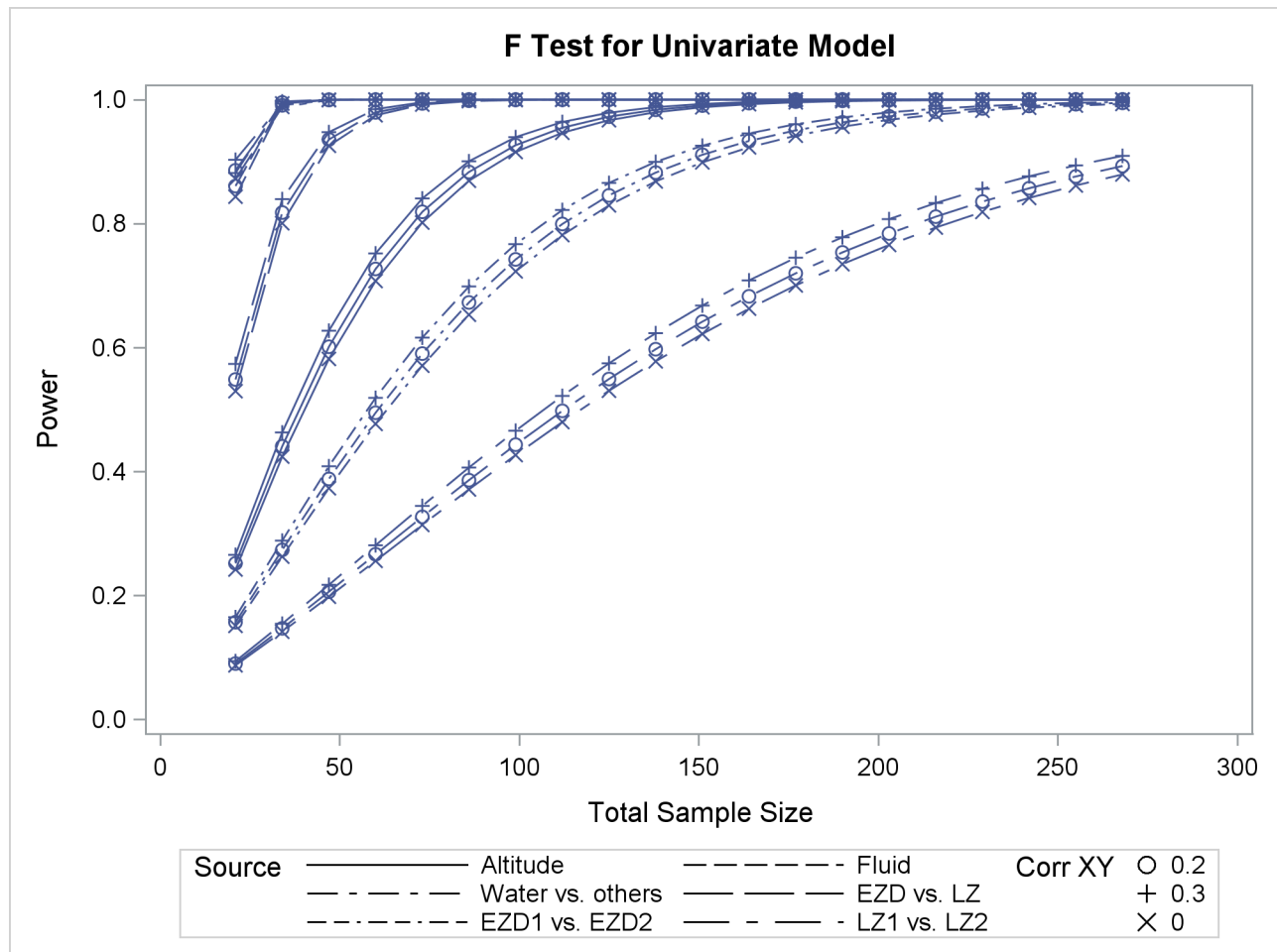
Output 49.2.3 Plot of Power versus Sample Size for Two-Way ANOVA Contrasts
