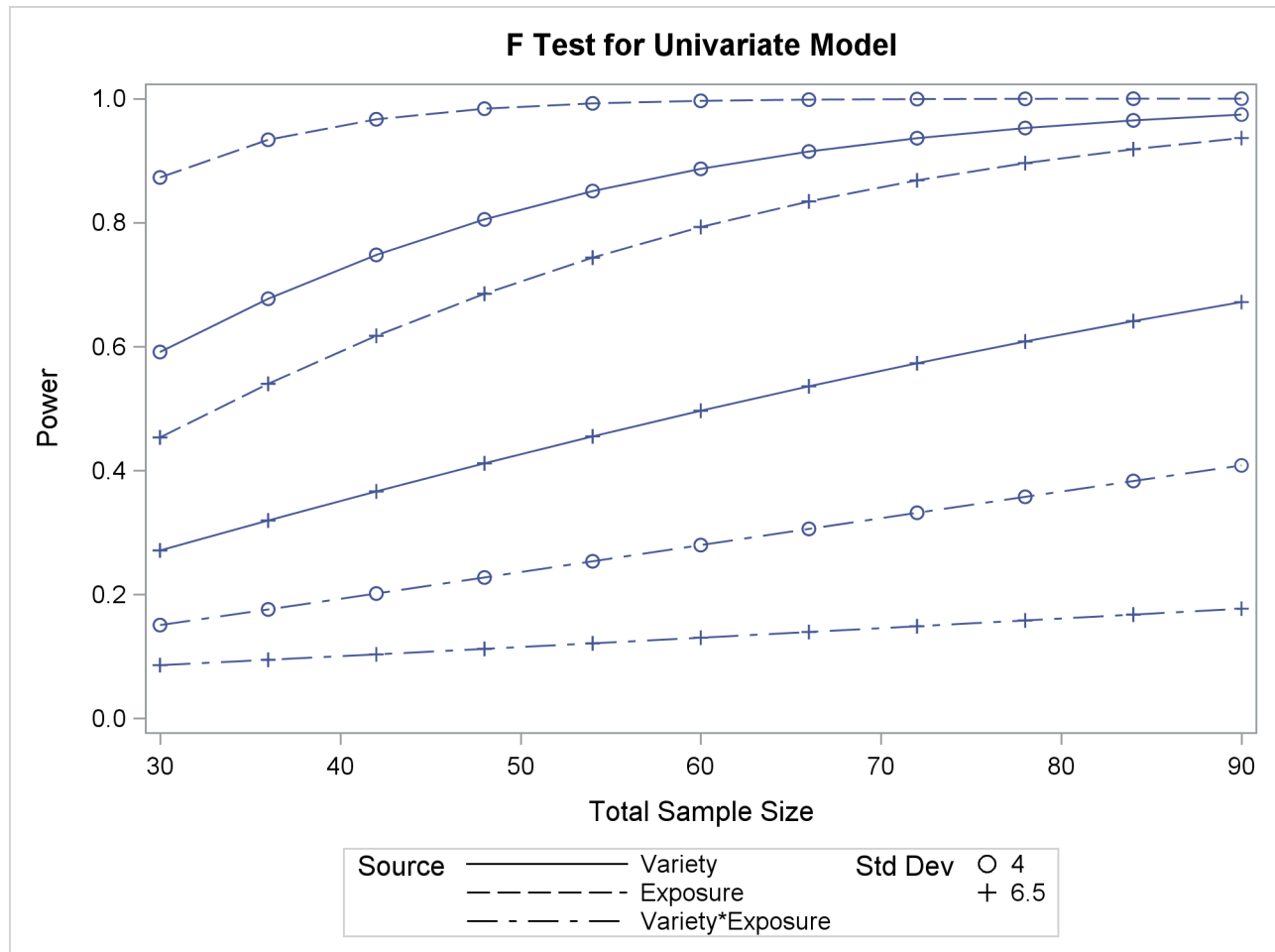
Figure 49.3 Plot of Power versus Sample Size for Two-Way ANOVA with Input Ranges
