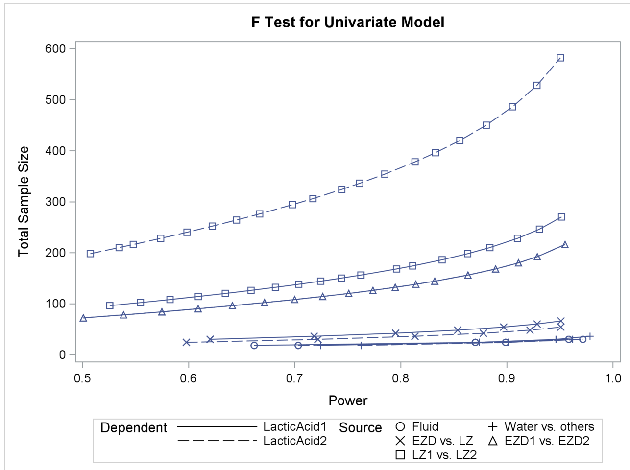
Output 49.1.2 Plot of Sample Size versus Power for One-Way ANOVA Contrasts
