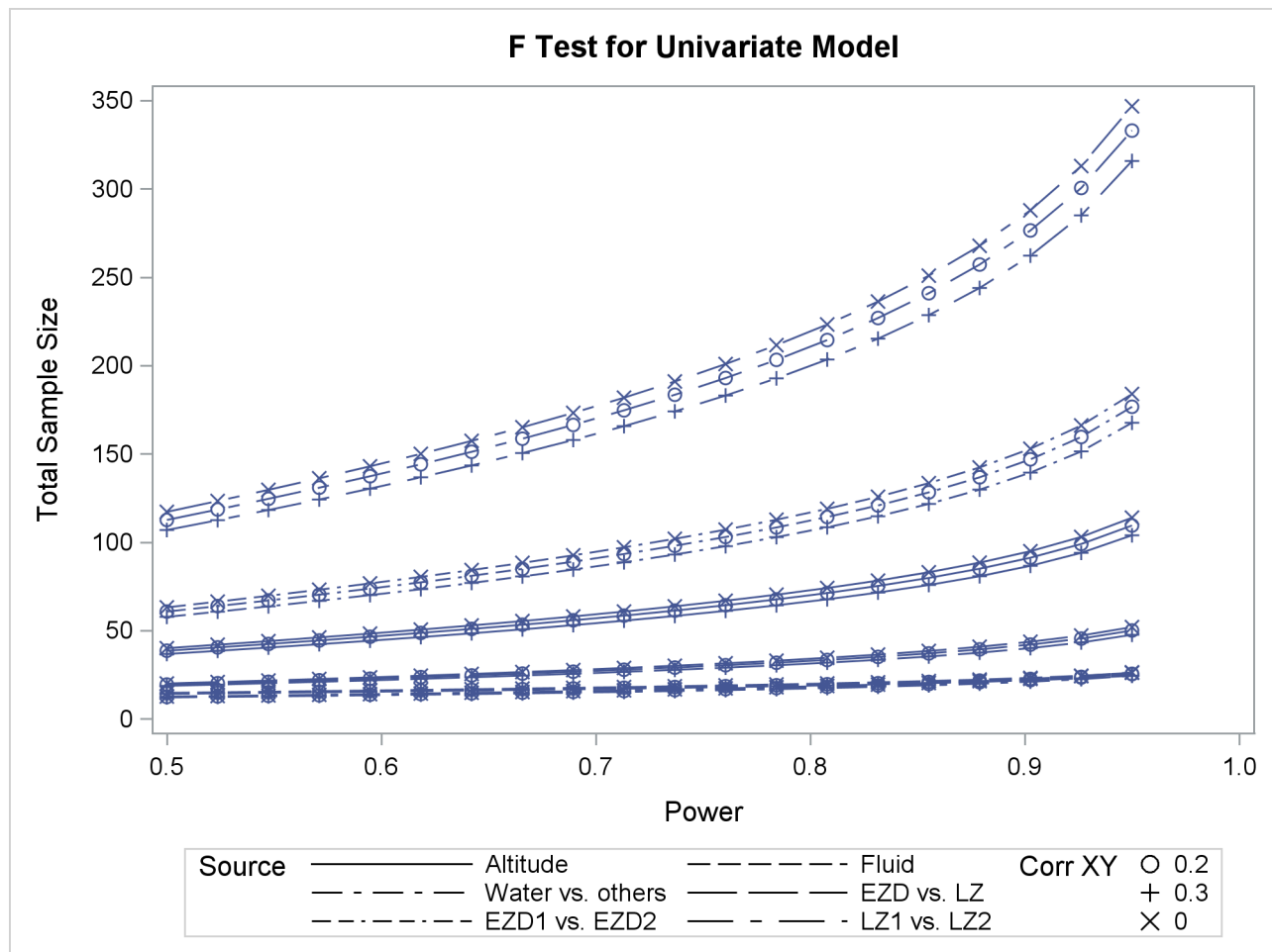
Output 49.2.2 Plot of Sample Size versus Power for Two-Way ANOVA Contrasts
