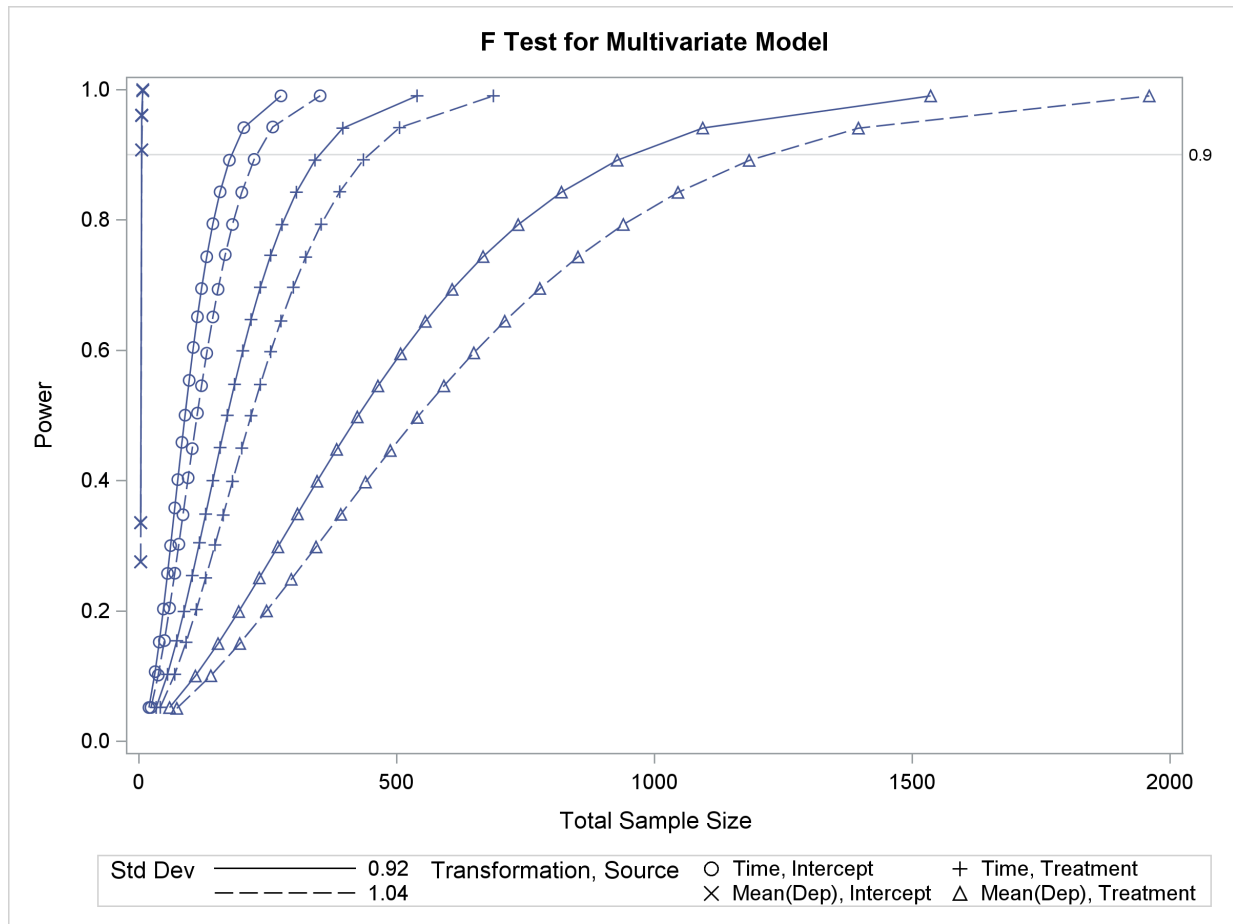
Output 49.3.2 Plot of Power versus Sample Size for Repeated Measures Analysis
