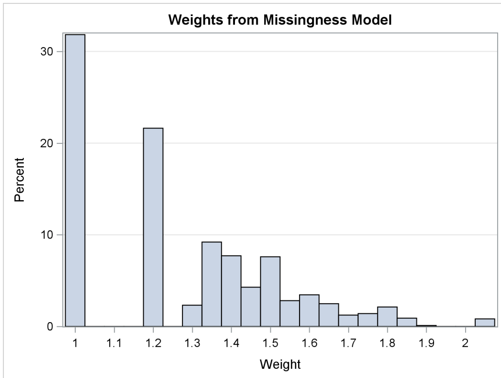
Output 44.3.3 Histogram of Estimated Weights
