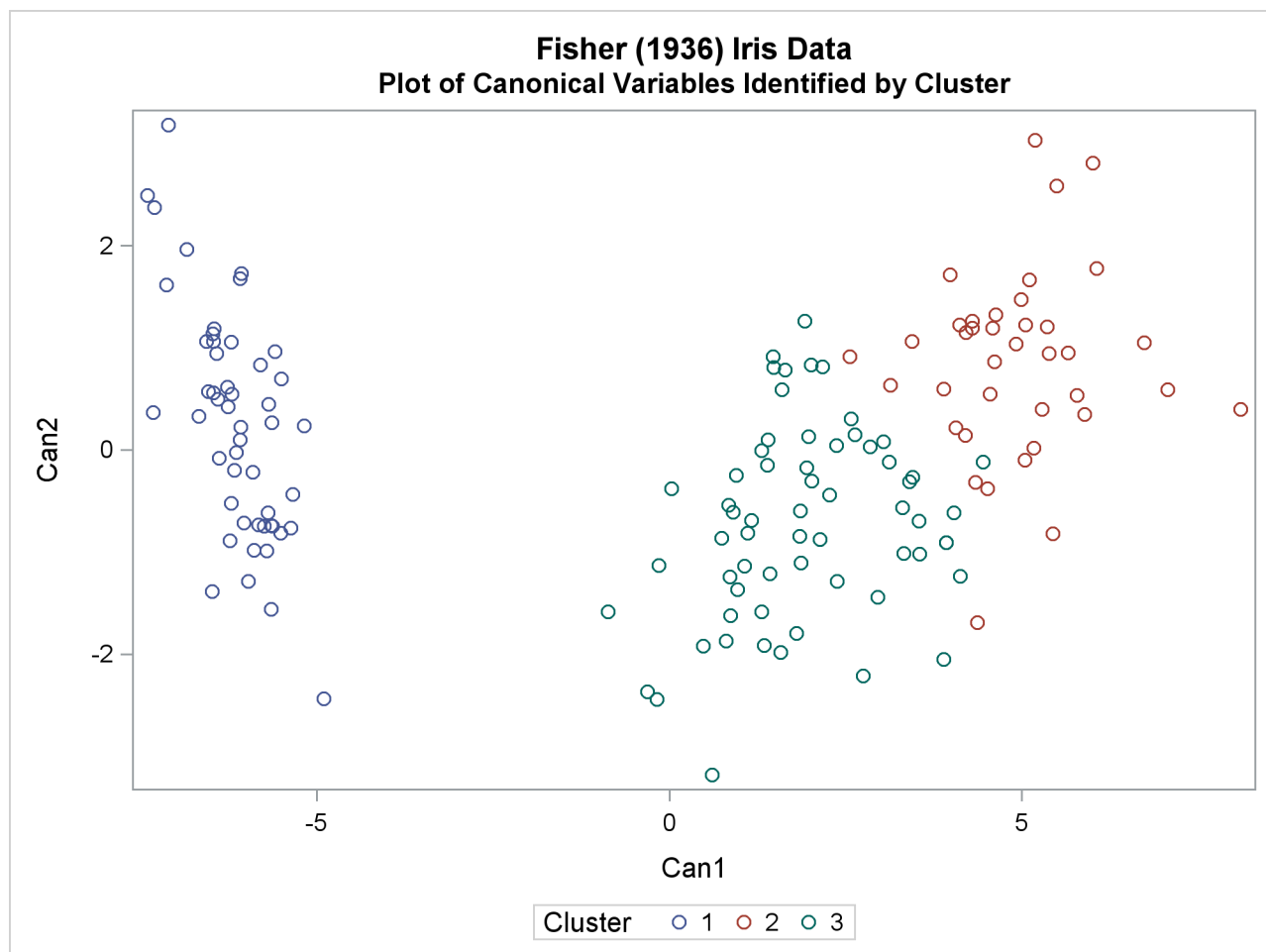
Output 39.1.4 Plot of Fisher's Iris Data using PROC CANDISC
