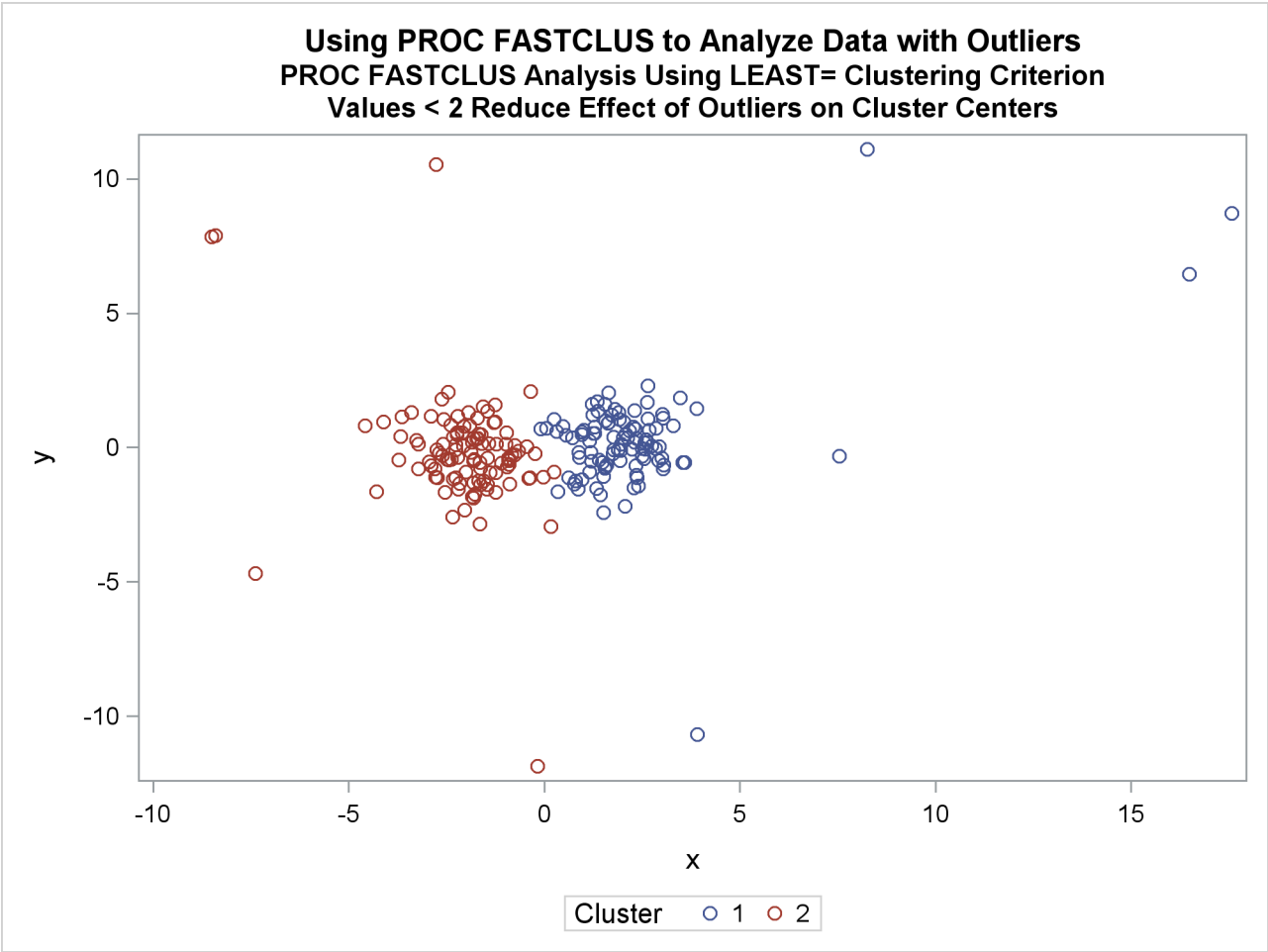
Output 39.2.4 Analysis Plot of Data with Outliers
