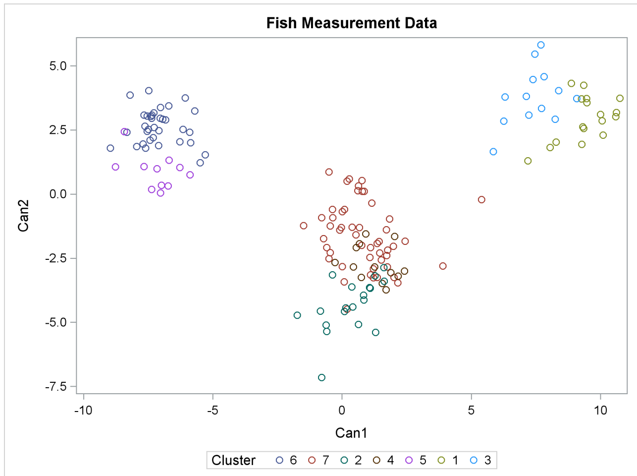
Figure 39.6 Plot of Canonical Variables and Cluster Value
