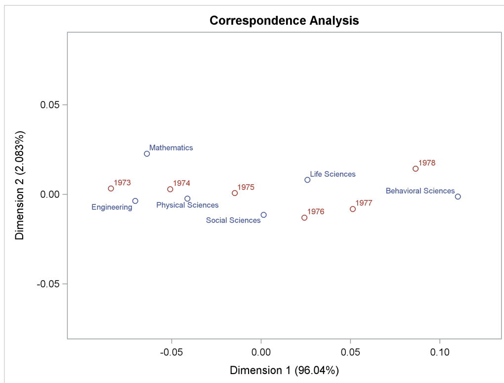
Figure 35.2 Correspondence Analysis of Ph.D. Data
