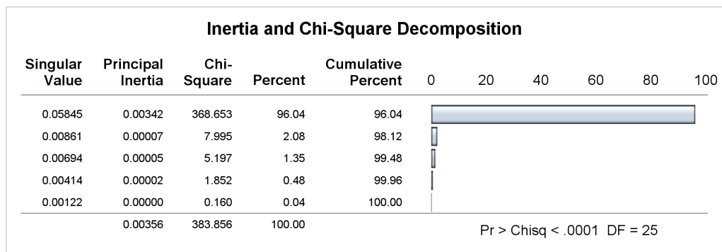
Figure 35.1 Inertia and Chi-Square Decomposition
