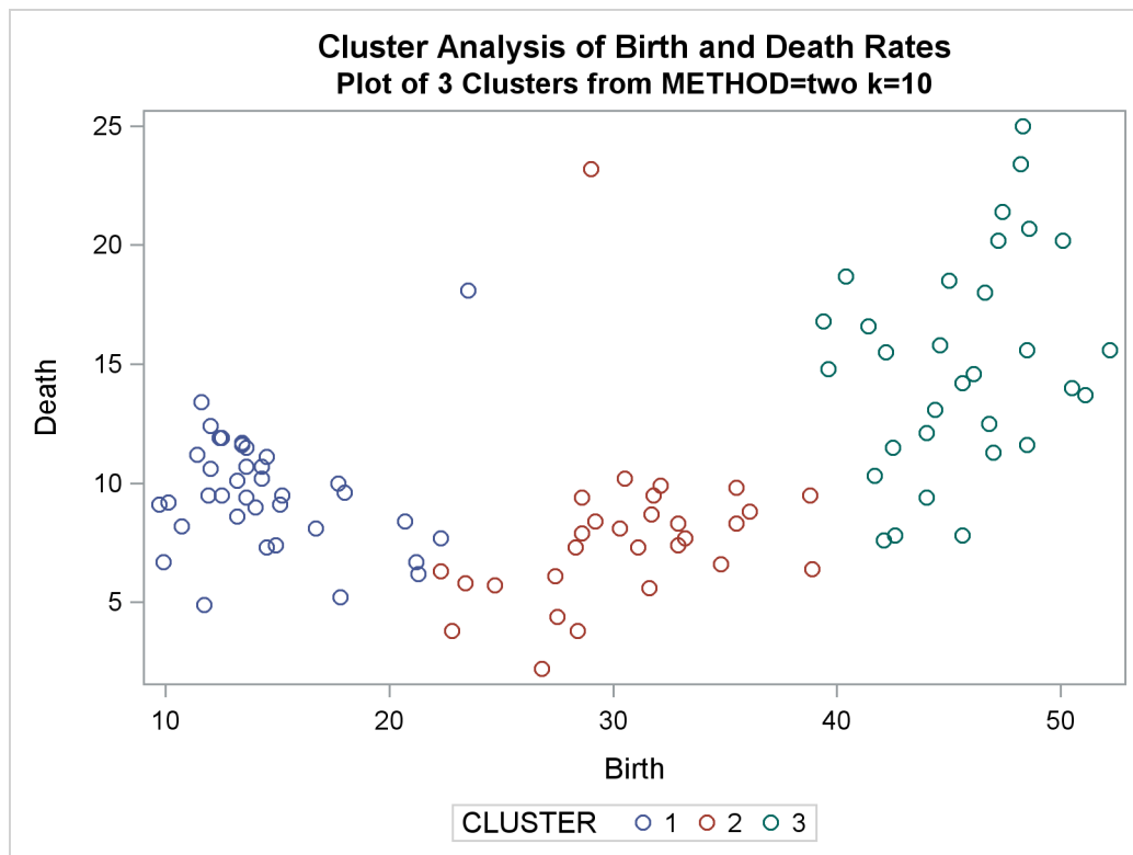
Output 34.2.13 Plot of Clusters for METHOD=TWOSTAGE K=10
