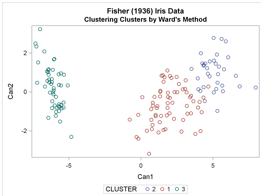
Output 34.3.14 Scatter Plot for Clustering Clusters using Ward's Method
