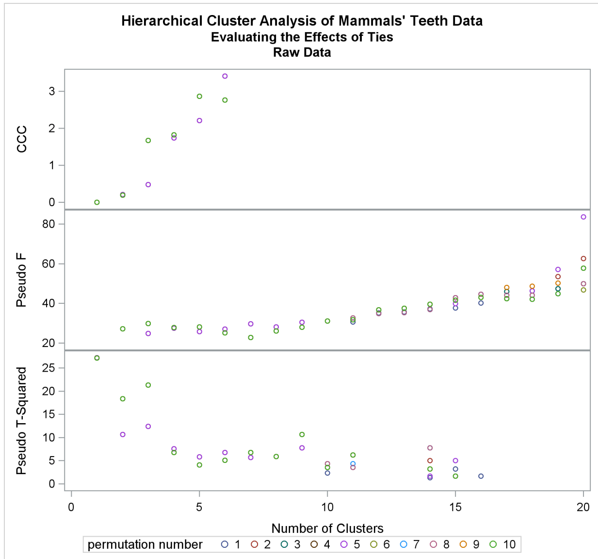
Output 34.4.3 Analysis of 10 Random Permutations of Raw Mammals' Teeth Data
