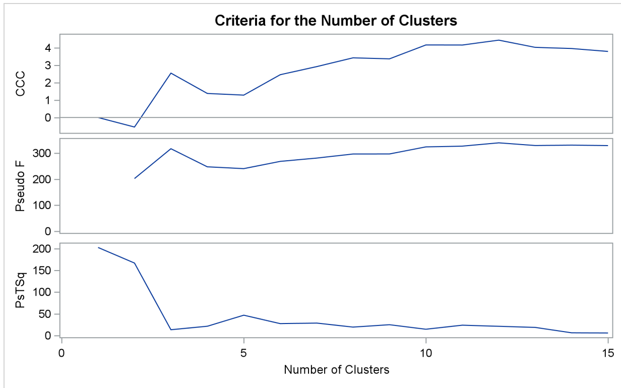
Output 34.2.6 Criteria for the Number of Clusters: METHOD=COMPLETE
