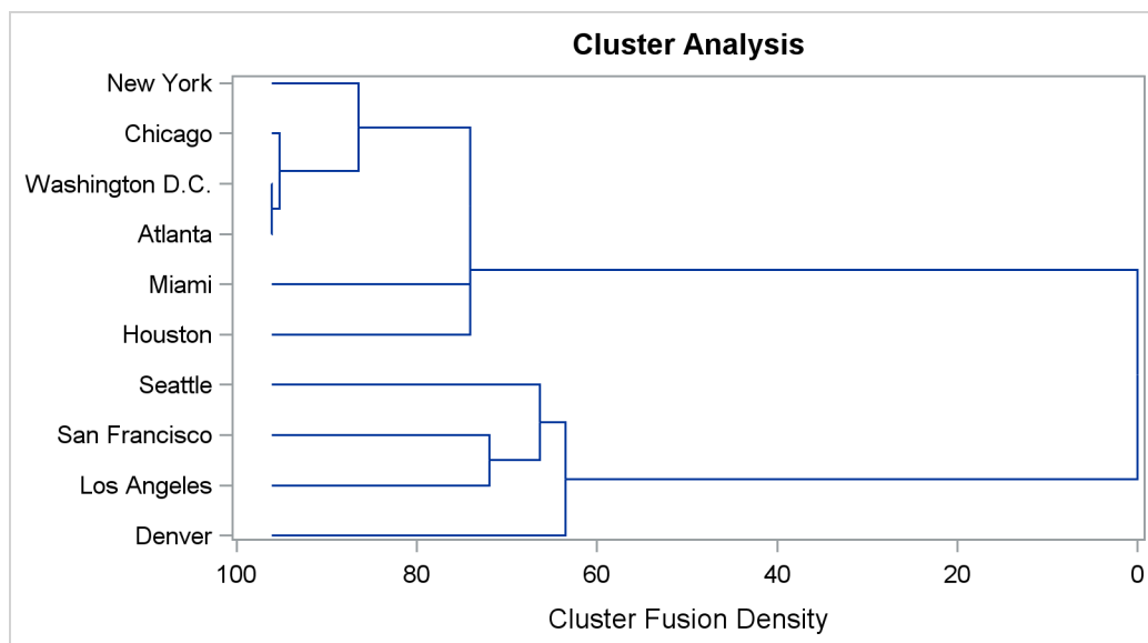
Output 34.1.11 Dendrogram Using METHOD=TWOSTAGE K=3
