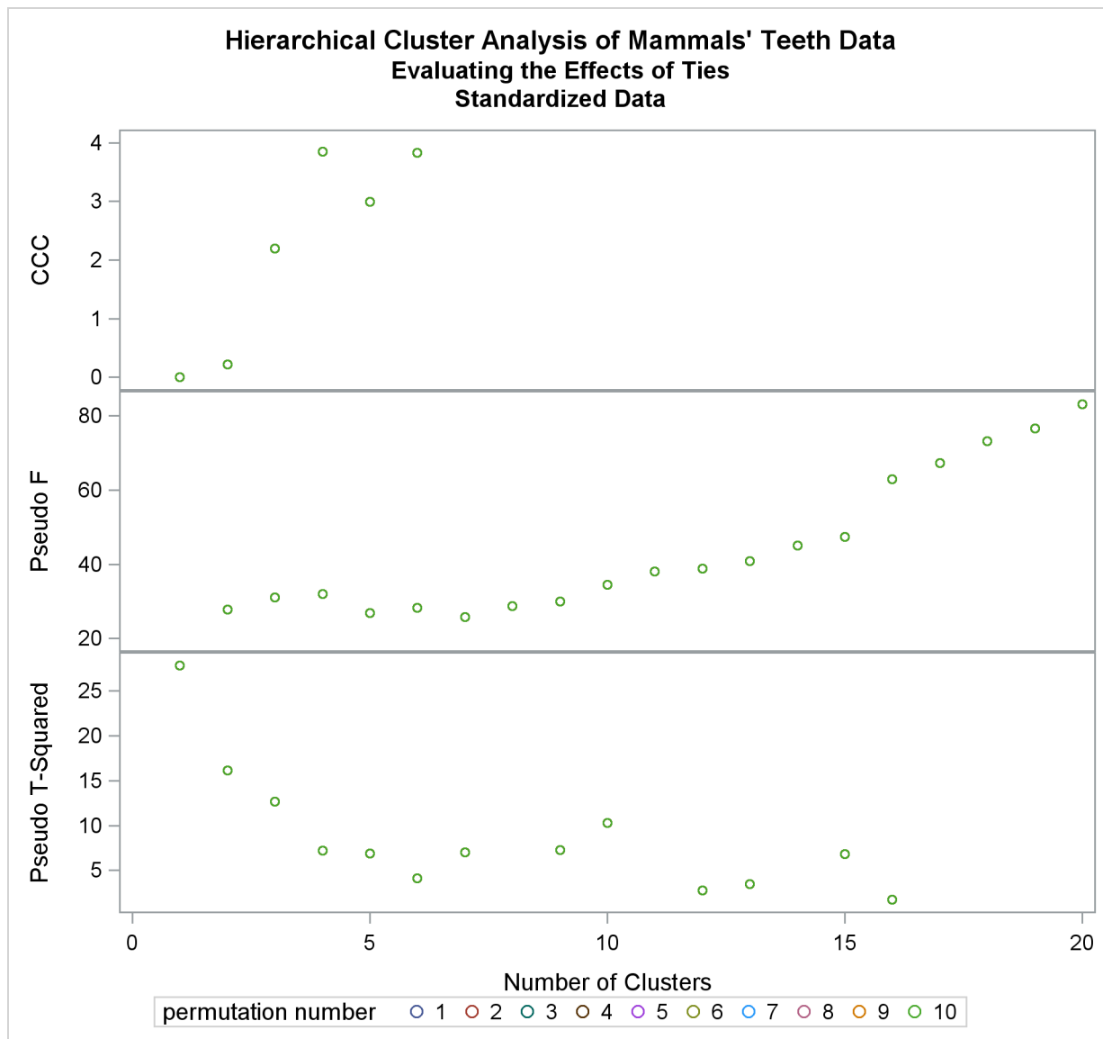
Output 34.4.5 Analysis of 10 Random Permutations of Standardized Mammals' Teeth Data
