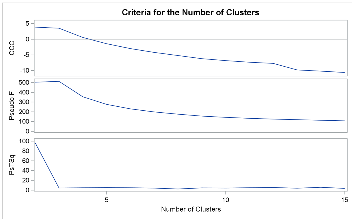
Output 34.3.6 Criteria for the Number of Clusters with METHOD=TWOSTAGE
