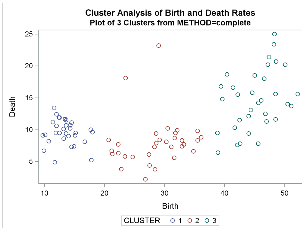
Output 34.2.7 Plot of Clusters for METHOD=COMPLETE
