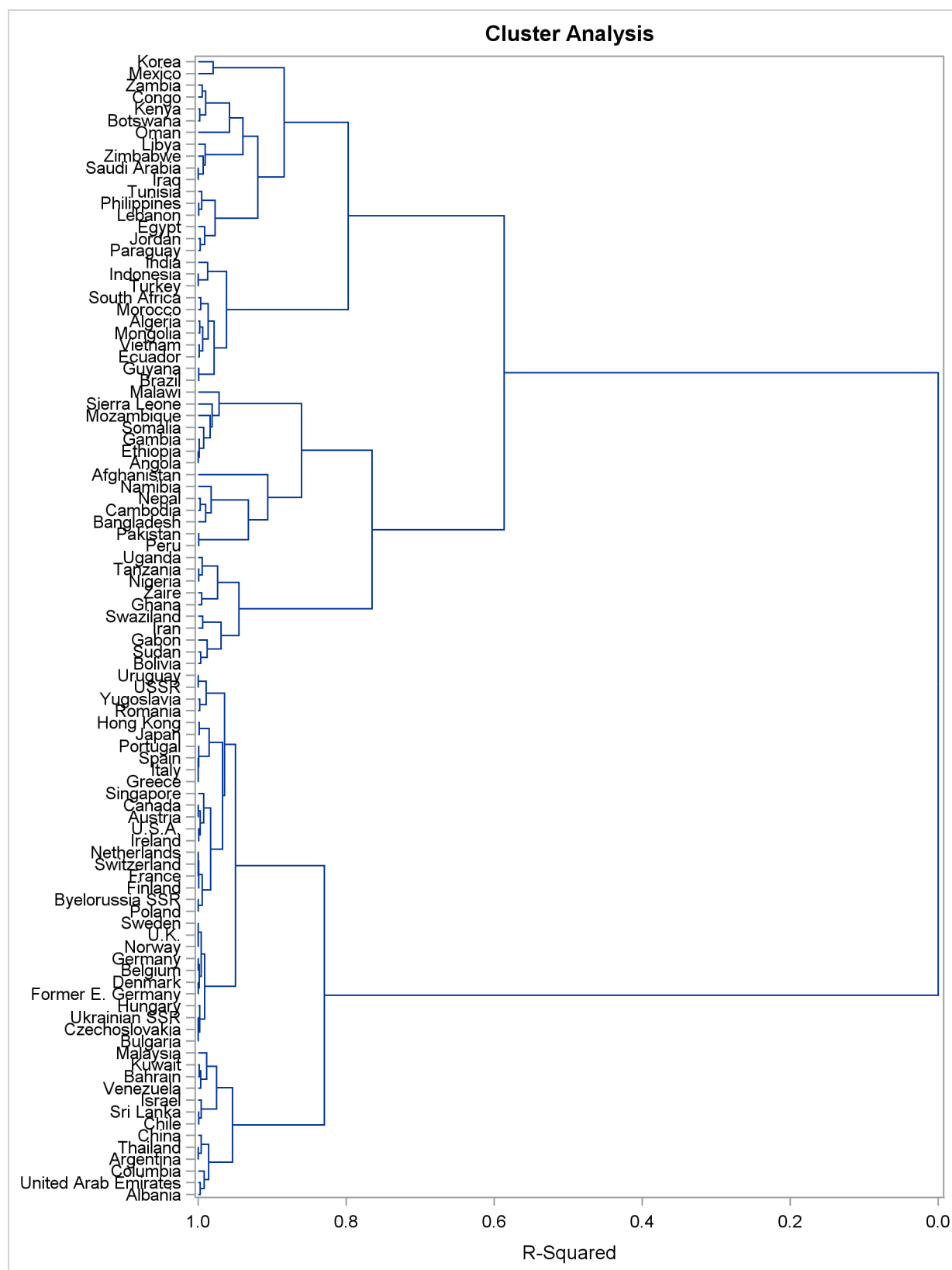
Figure 34.4 Dendrogram of Clusters versus R-Square Values
