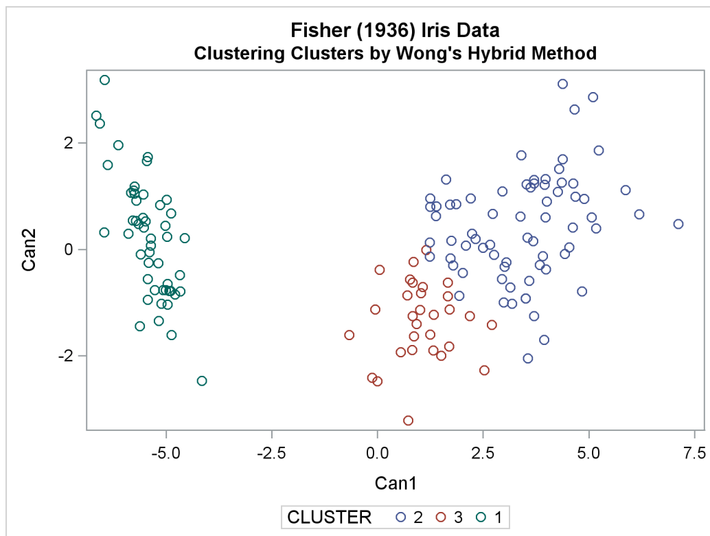
Output 34.3.17 Scatter Plot for Clustering Clusters using Wong's Hybrid Method
