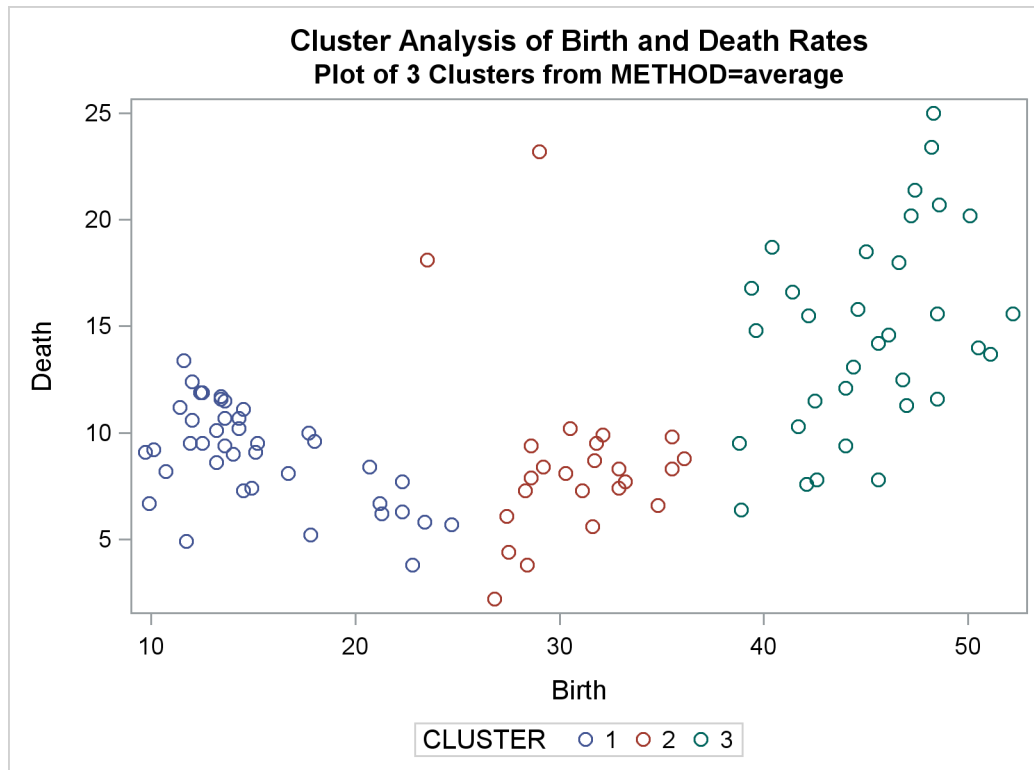
Output 34.2.3 Plot of Three Clusters: METHOD=AVERAGE
