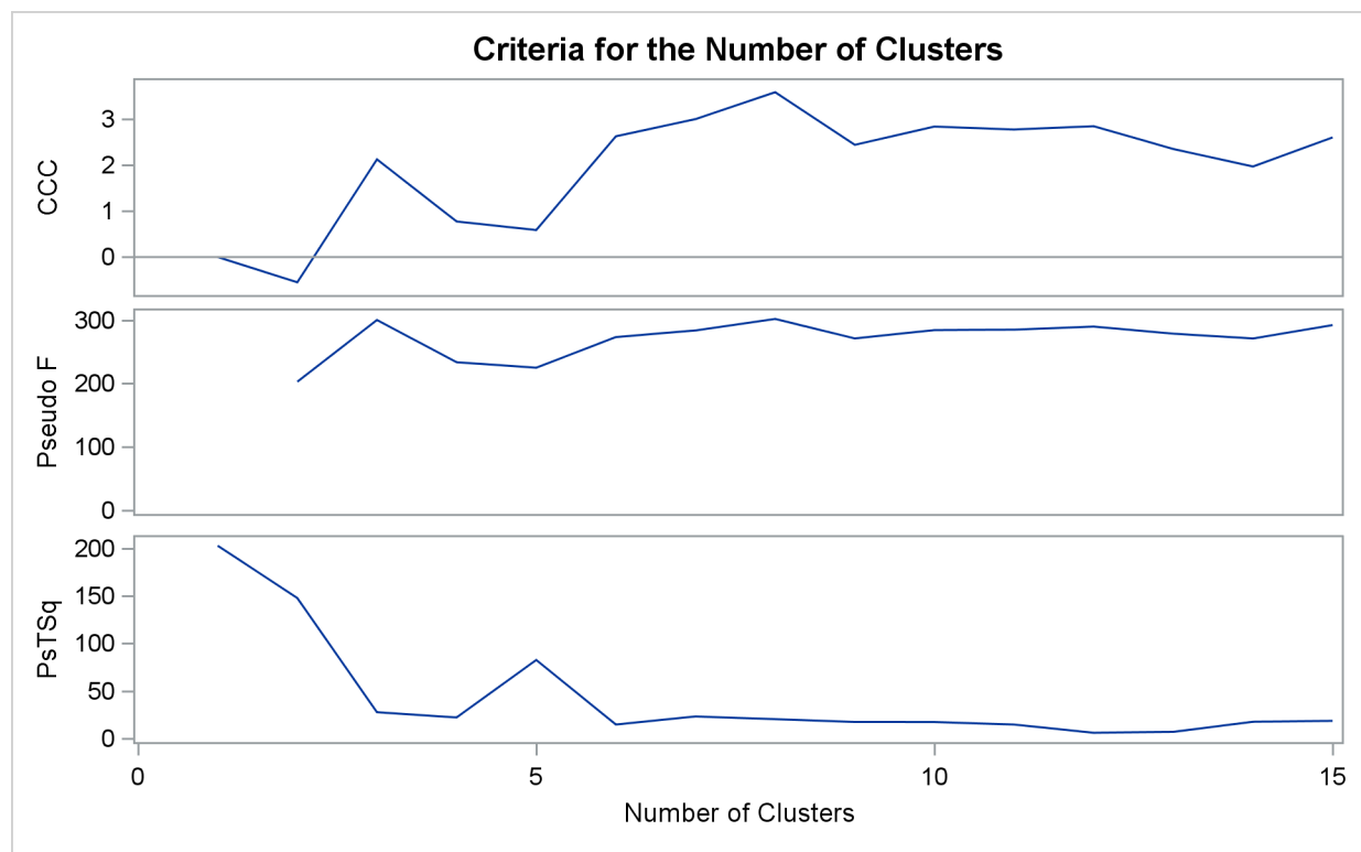
Output 34.2.2 Criteria for the Number of Clusters: METHOD=AVERAGE
