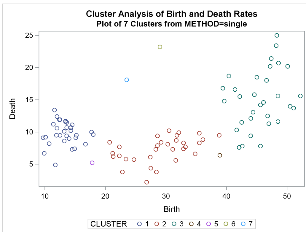
Output 34.2.10 Plot of Clusters for METHOD=SINGLE
