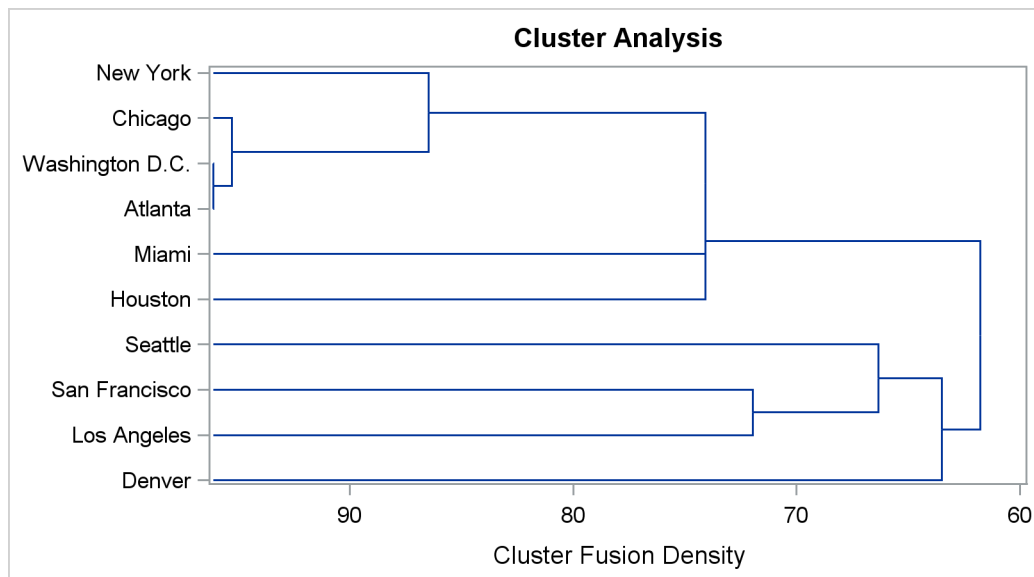
Output 34.1.7 Dendrogram Using METHOD=DENSITY K=3
