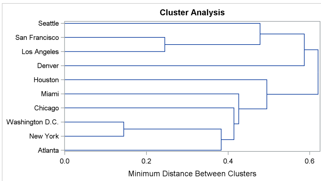
Output 34.1.9 Dendrogram Using METHOD=SINGLE
