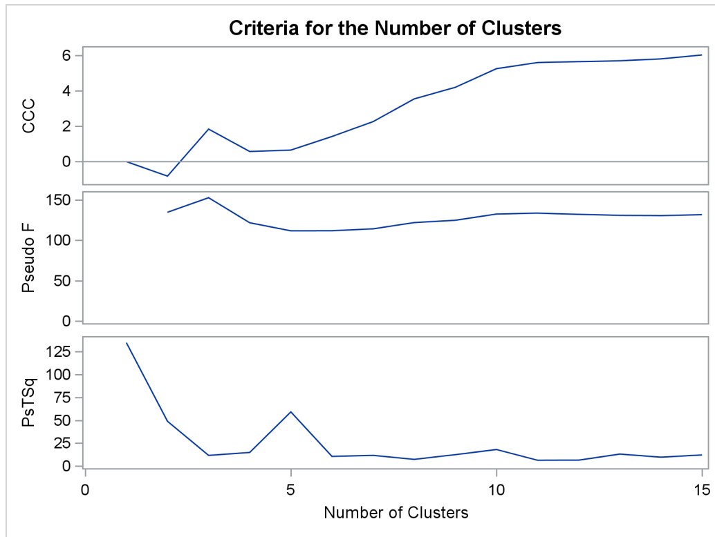
Figure 34.3 Plot of Statistics for Estimating the Number of Clusters
