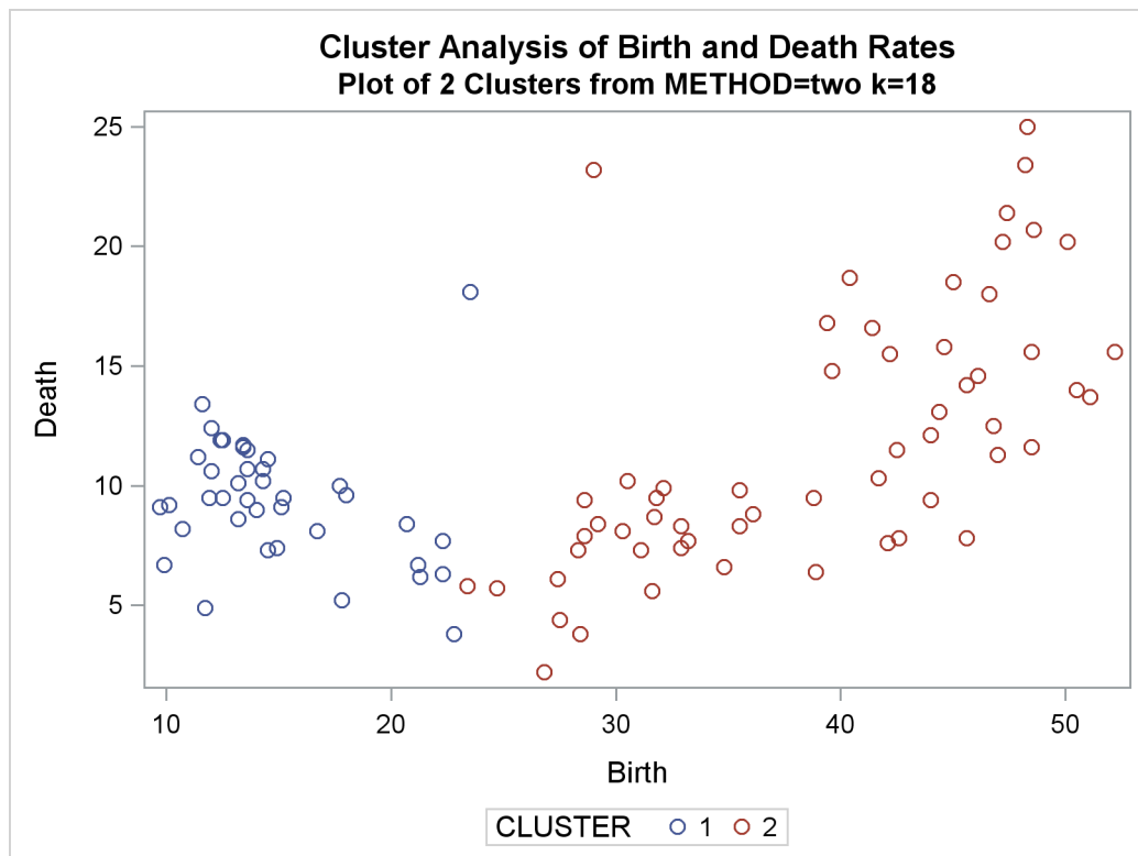
Output 34.2.14 Plot of Clusters for METHOD=TWOSTAGE K=18
