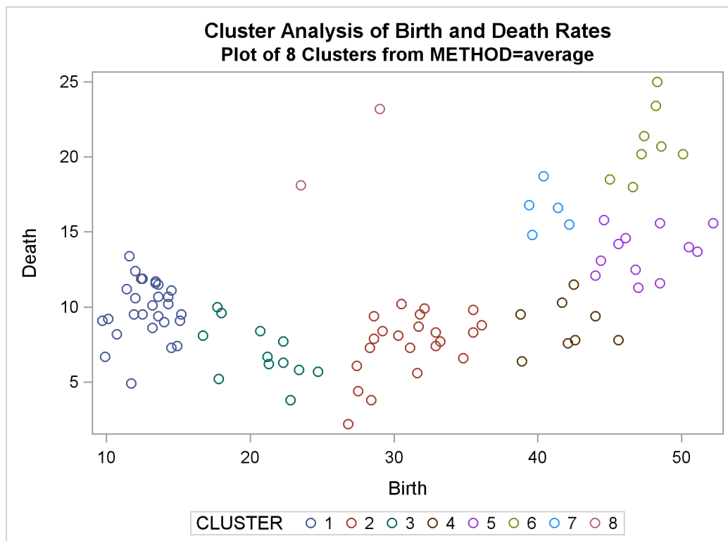
Output 34.2.4 Plot of Eight Clusters: METHOD=AVERAGE
