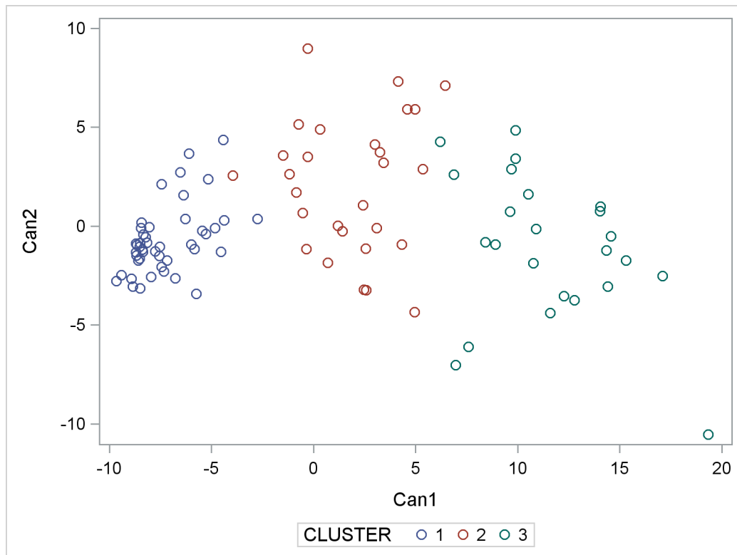
Figure 34.5 Plot of Canonical Variables and Cluster for Three Clusters
