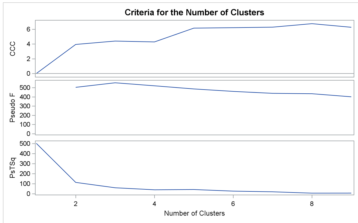
Output 34.3.12 Criteria for the Number of Clusters for Clustering Clusters from Ward's Method
