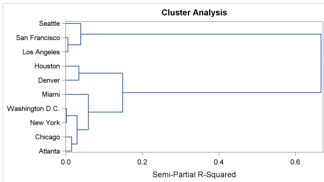
Output 34.1.13 Dendrogram Using METHOD=WARD
