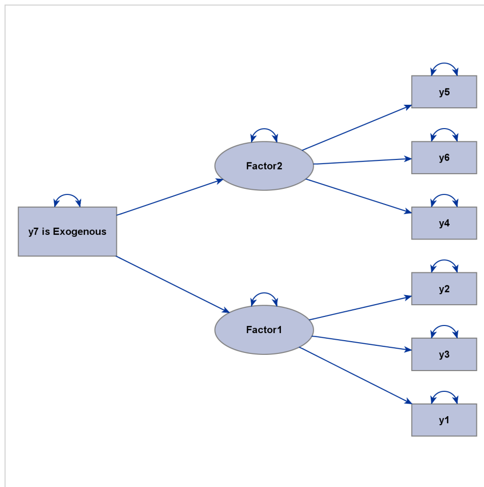
Figure 29.20 Including an Observed Variable as a Structural Variable: Full Model
