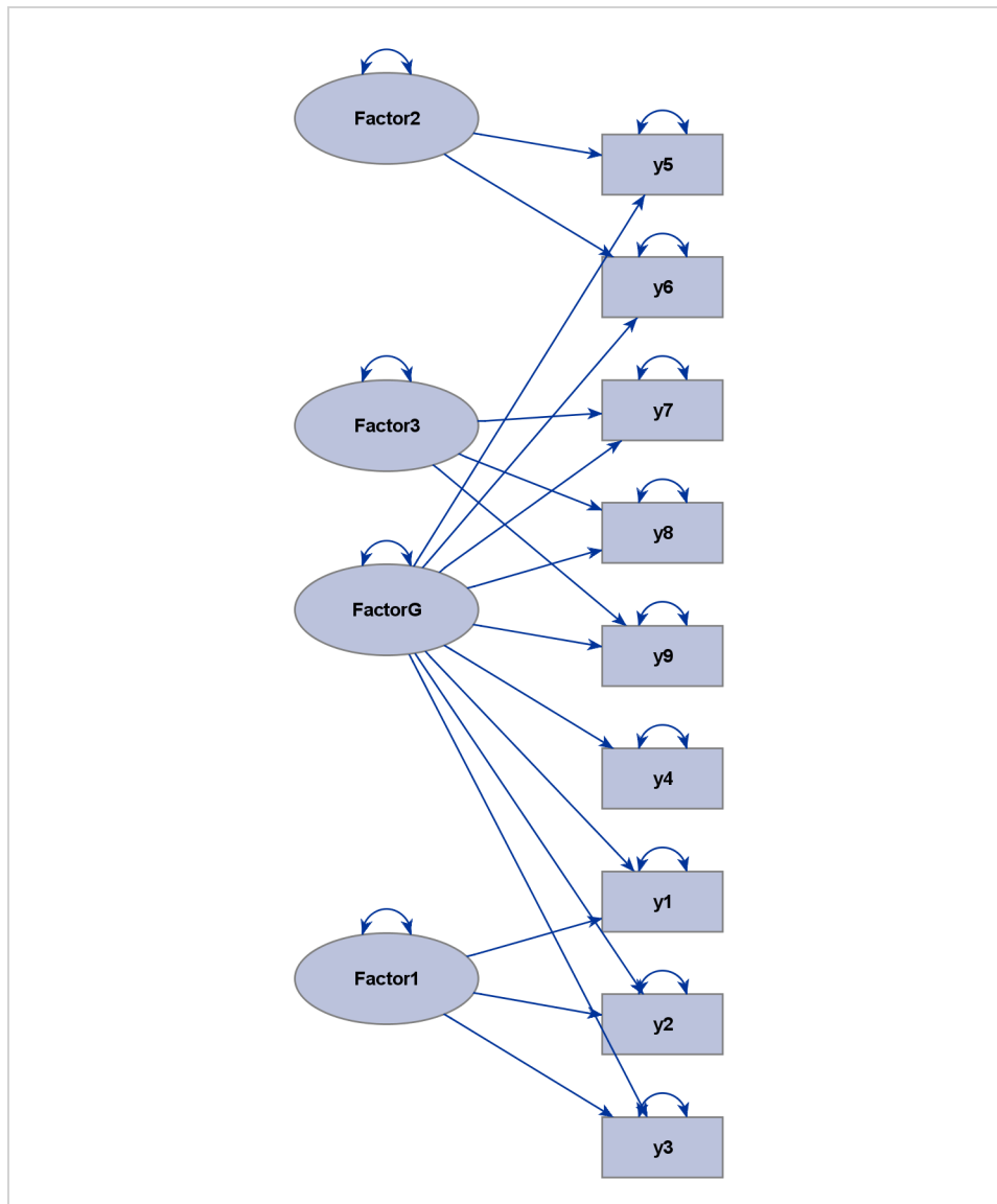
Figure 29.7 Hierarchical Factor Model That Exhibits an Ideal Process-Flow Pattern
