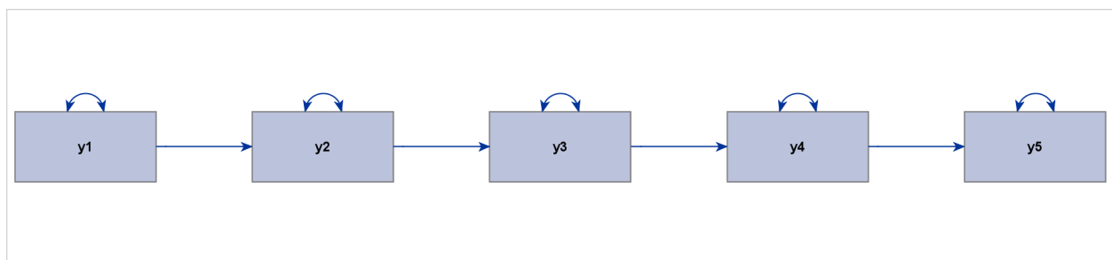
Figure 29.3 Linear Ordering of Observed Variables
