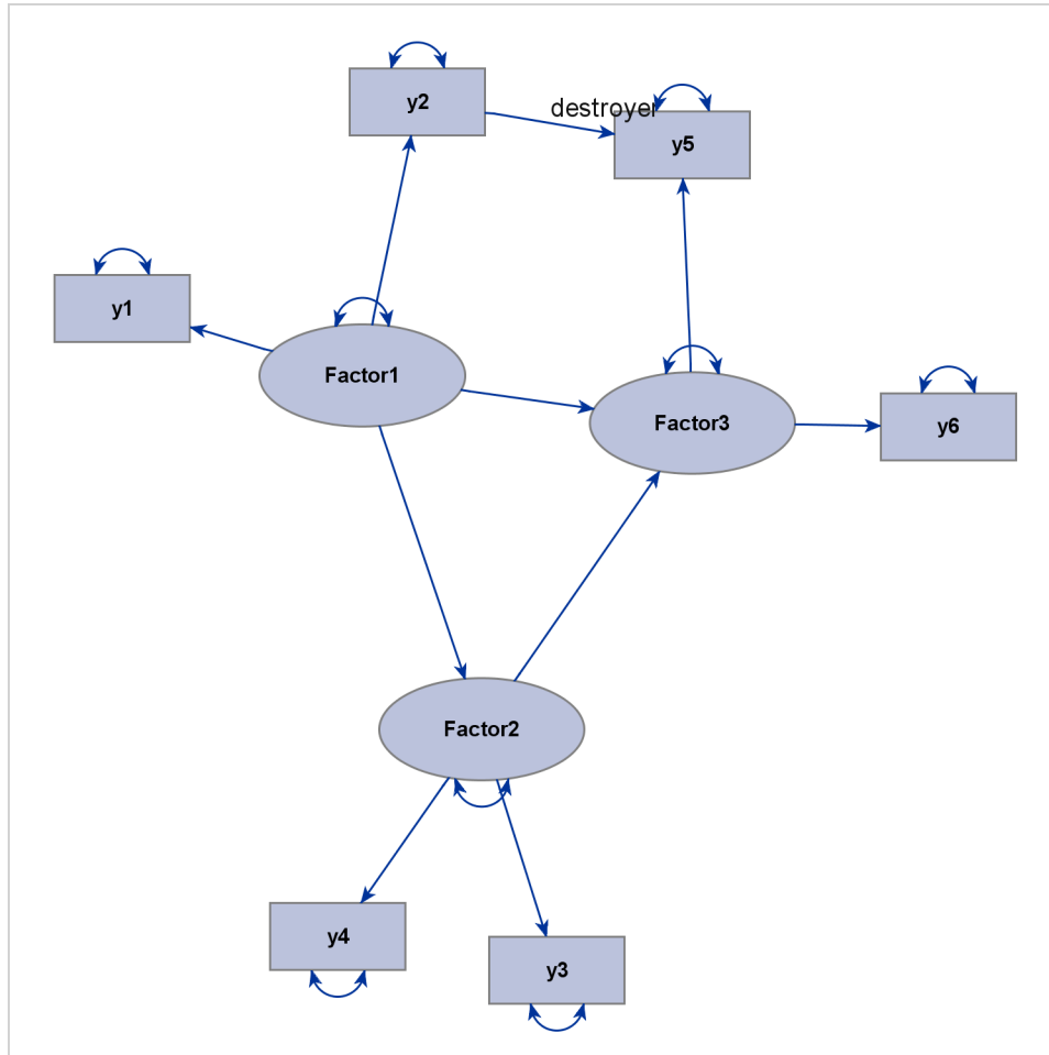
Figure 29.14 Path Diagram Whose Destroyer Path Is Not Handled by the GRIP Algorithm
