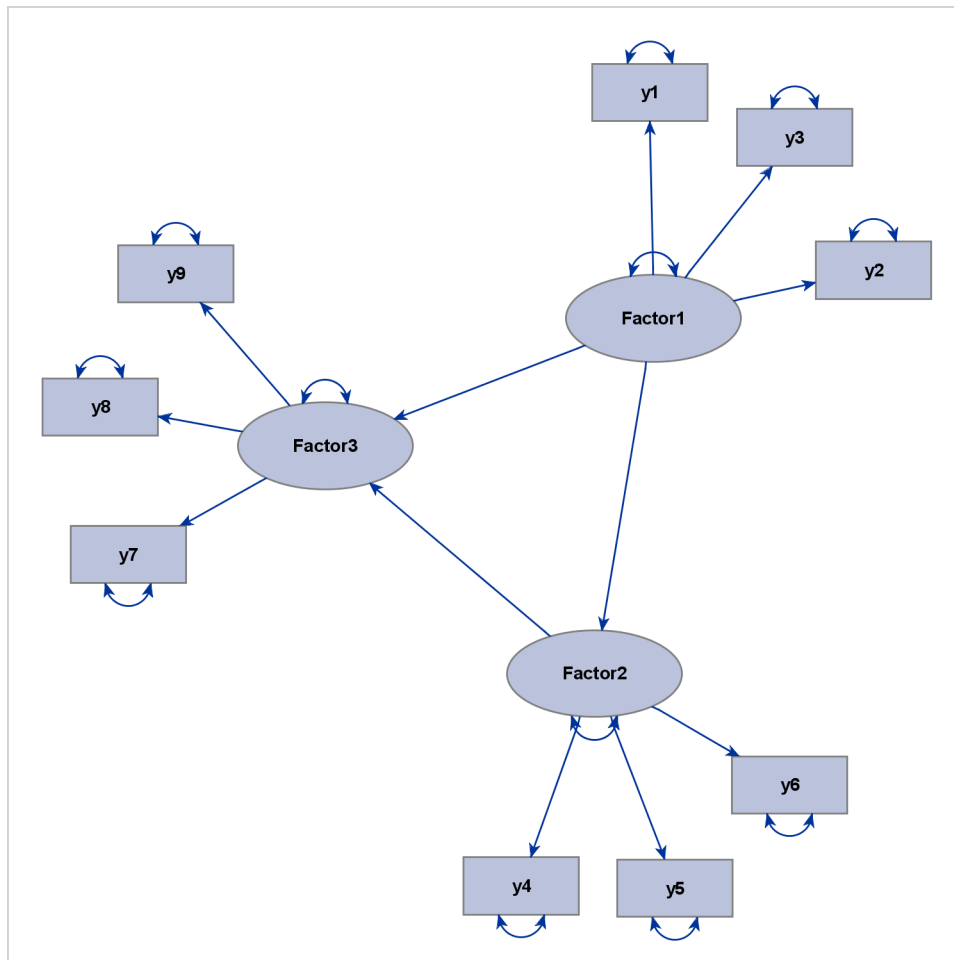
Figure 29.11 Path Diagram That Uses the GRIP Layout Algorithm
