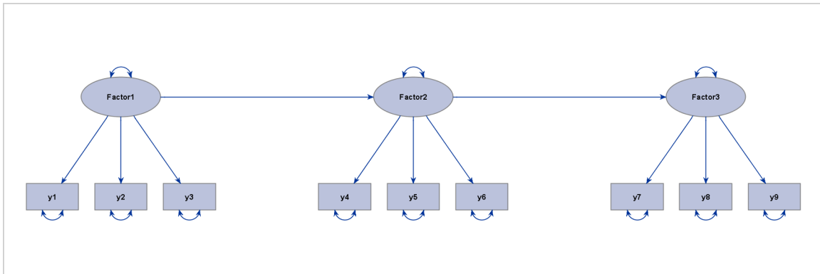
Figure 29.8 Linearly Ordered Factors with an Ideal Grouped-Flow Pattern
