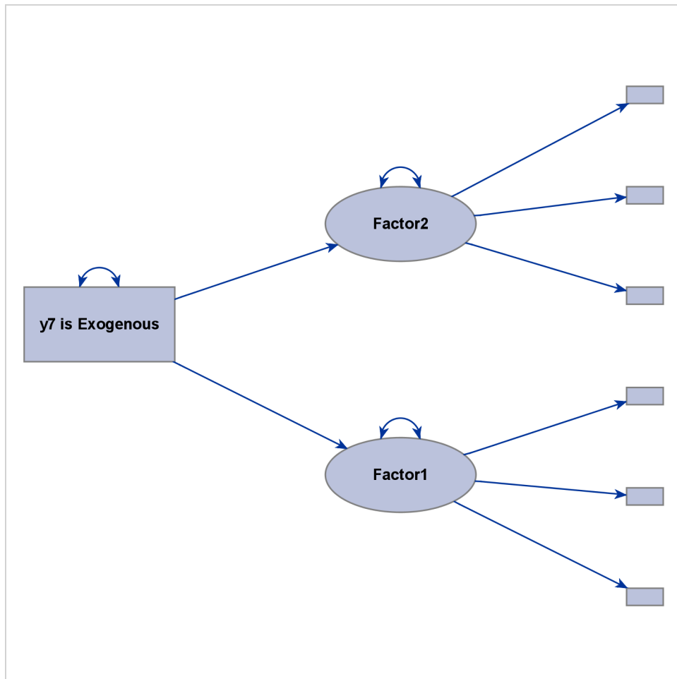
Figure 29.22 Including an Observed Variable as a Structural Variable: Structural Component
