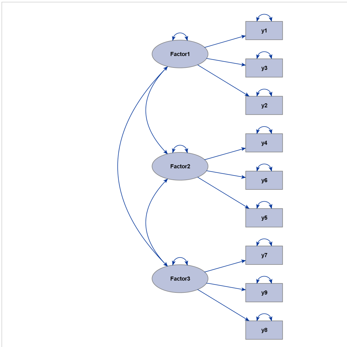
Figure 29.5 Confirmatory Factor Model That Exhibits an Ideal Process-Flow Pattern
