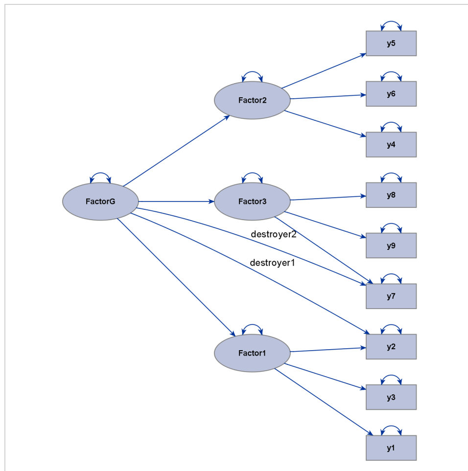
Figure 29.13 Higher-Order Factor Model with Two Destroyer Paths Identified
