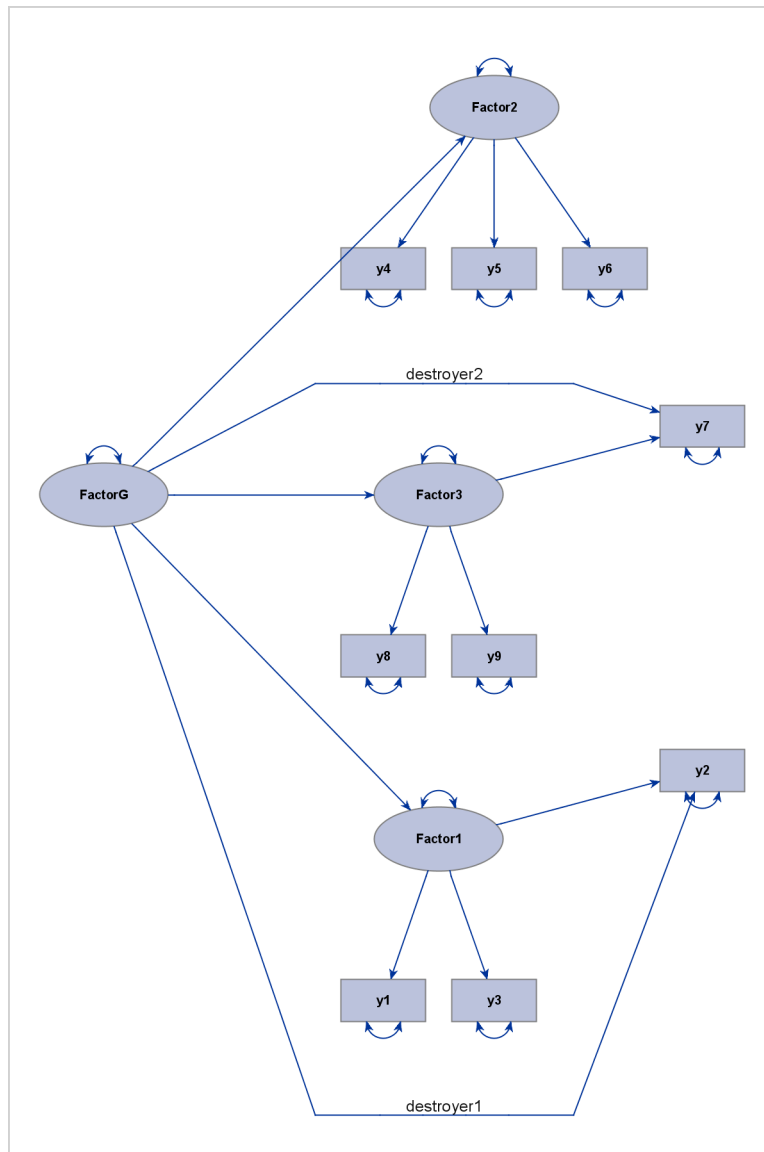
Figure 29.12 A Higher-Order Factor Model With Two Destroyer Paths
