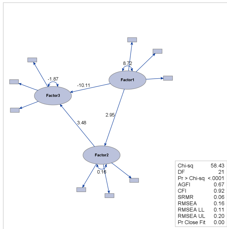
Figure 29.19 Emphasizing the Structural Component in the Path Diagram for the Unstandardized Solution
