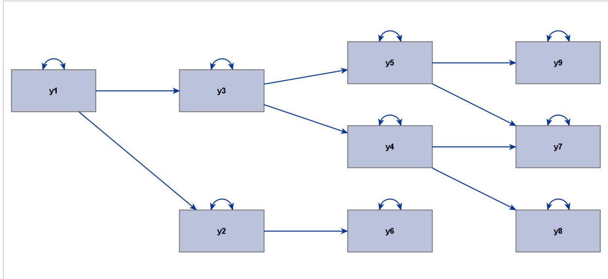
Figure 29.4 Hierarchical Ordering of Observed Variables
