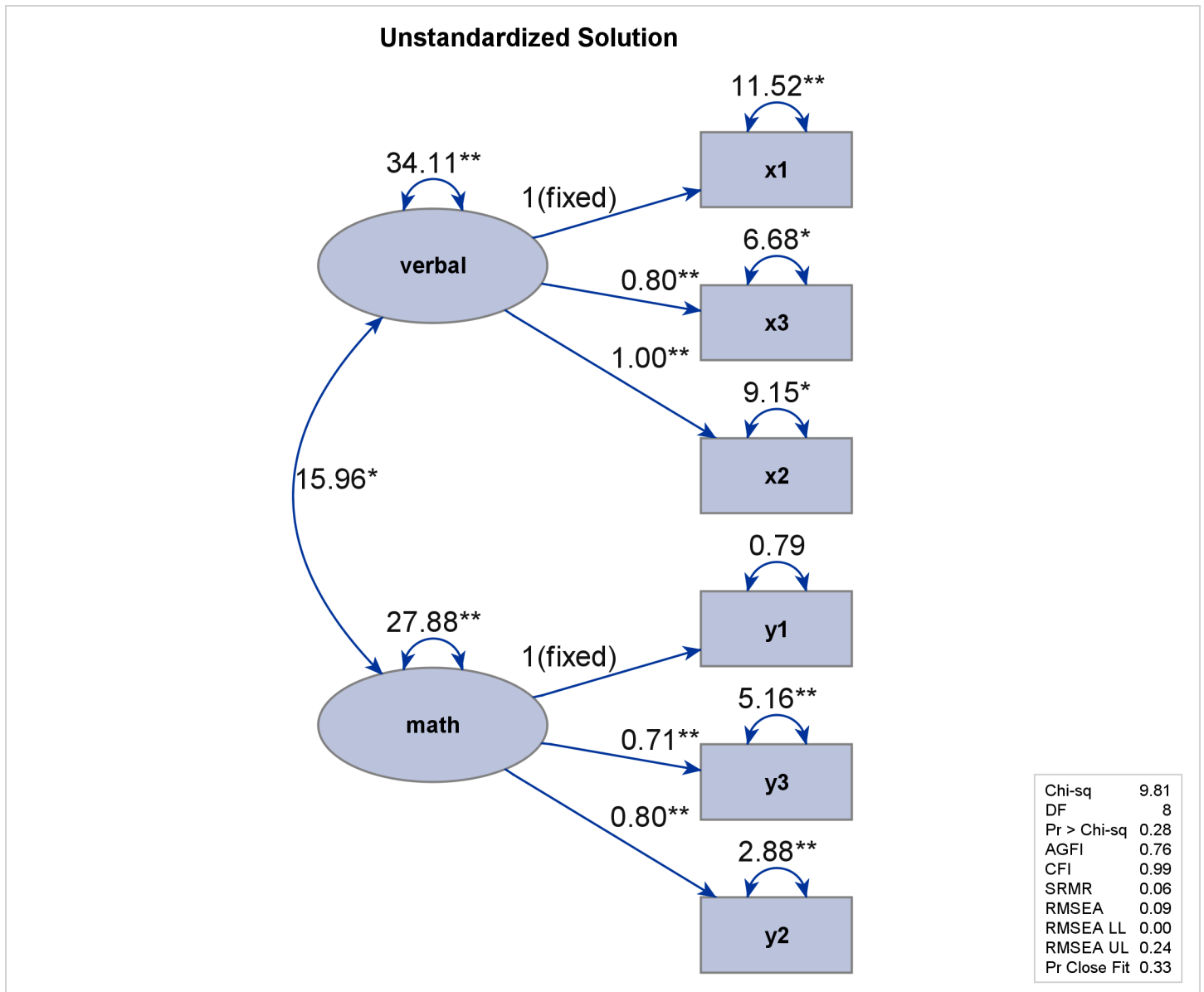
Output 29.12.8 Path Diagram and Fit Summary: Scores Data
