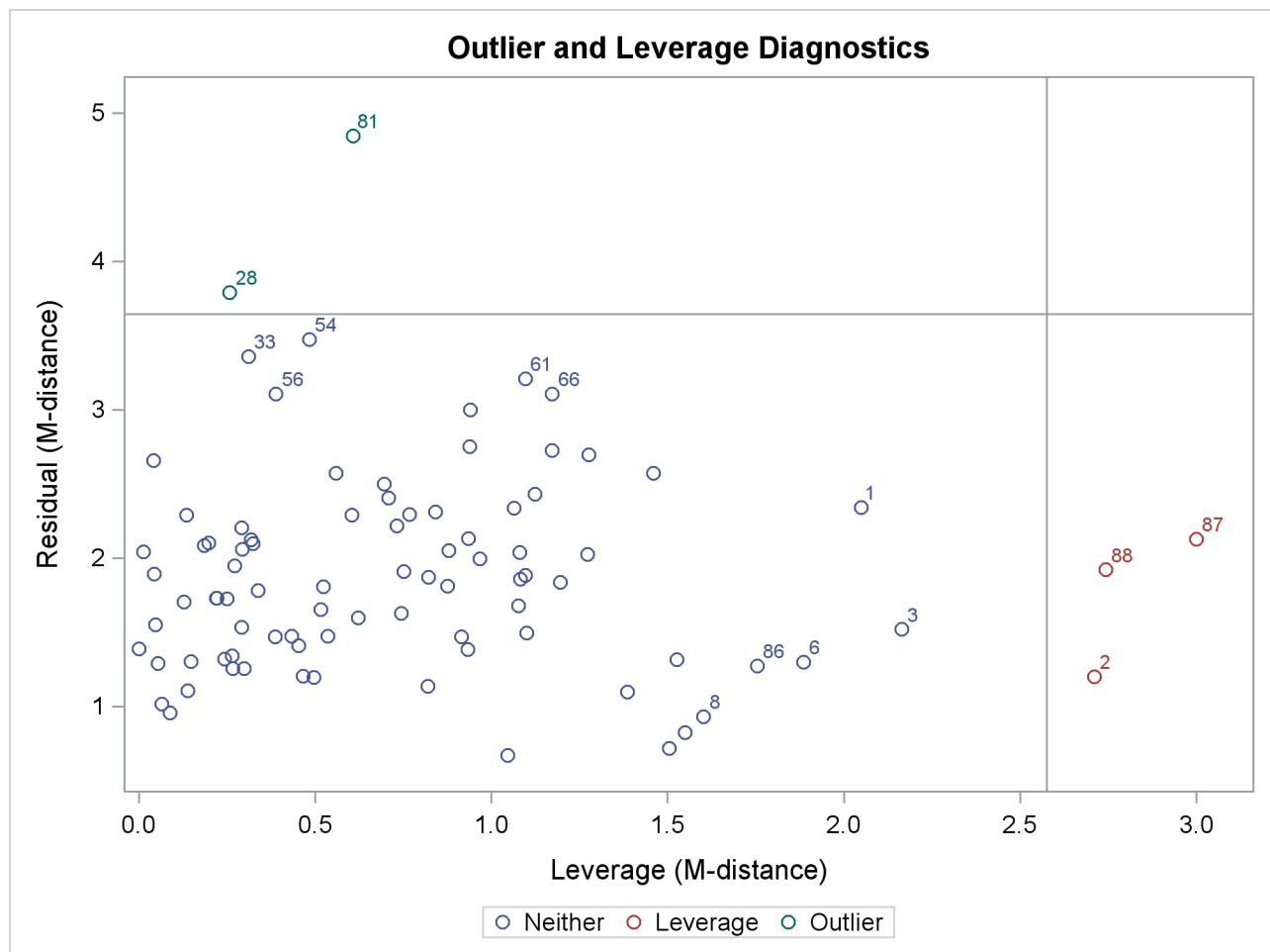
Output 29.14.13 Outliers and Leverage Observations with Direct Robust Estimation
