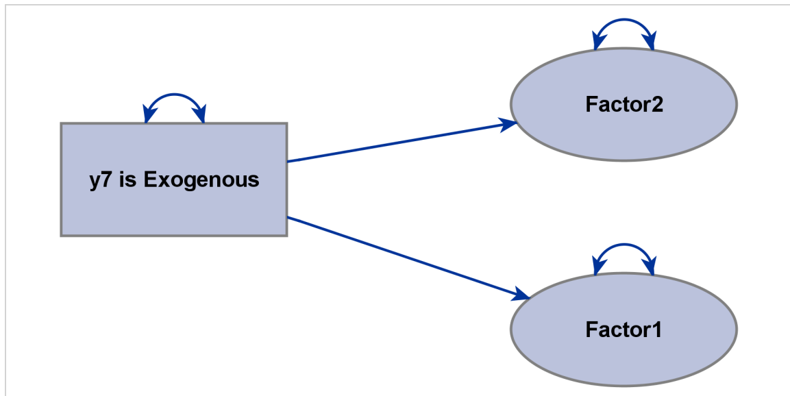
Figure 29.21 Including an Observed Variable as a Structural Variable: Emphasizing the Structural Component
