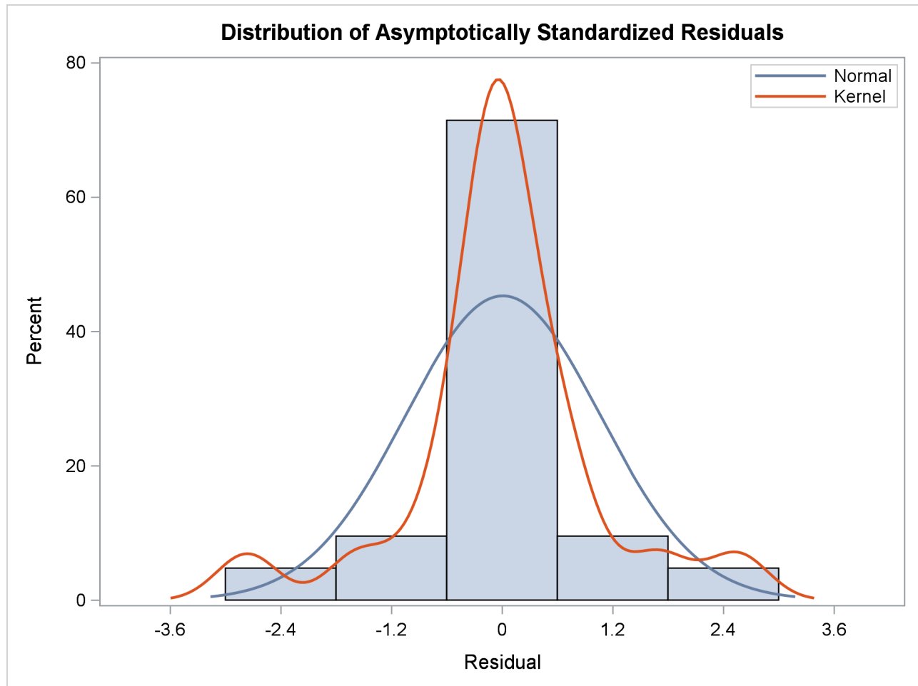
Output 29.17.10 Distribution of Asymptotically Standardized Residuals
