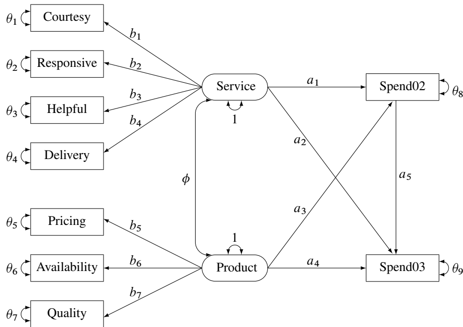
Figure 29.27 Path Diagram of Purchasing Behavior
