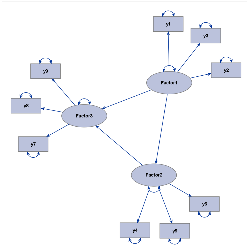
Figure 29.16 Path Diagram for the Complete Model
