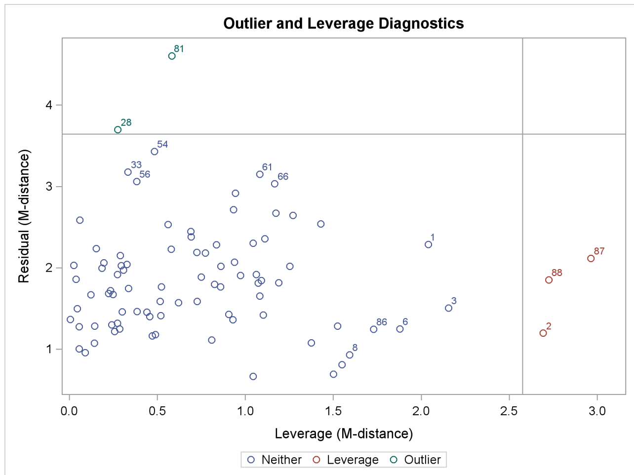
Output 29.14.3 Outliers and Leverage Observations
