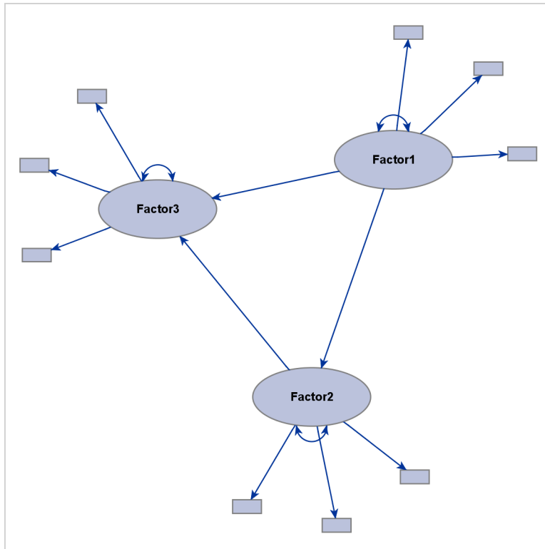
Figure 29.18 Emphasizing the Structural Component in the Path Diagram
