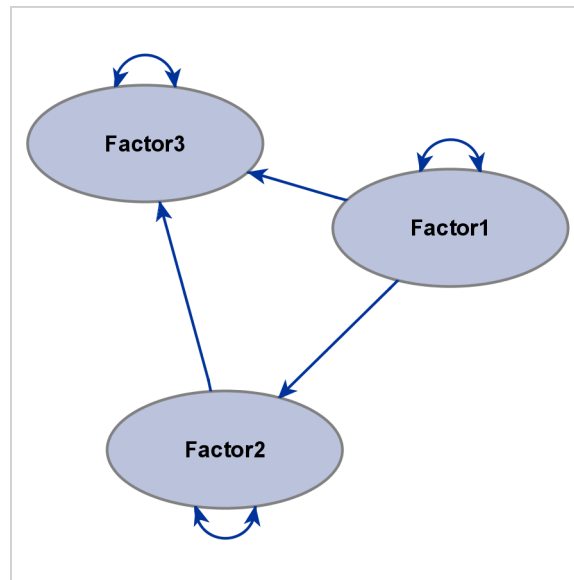
Figure 29.17 Path Diagram for the Structural Component
