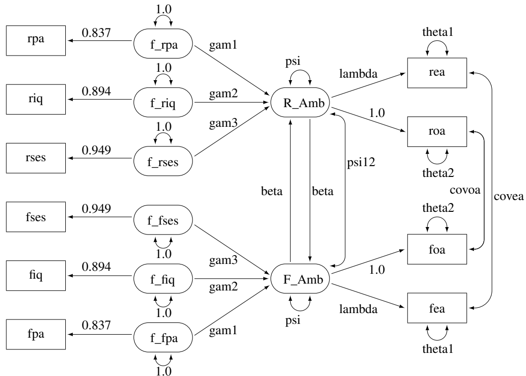
Figure 29.26 Path Diagram for Career Aspiration: Model 3
