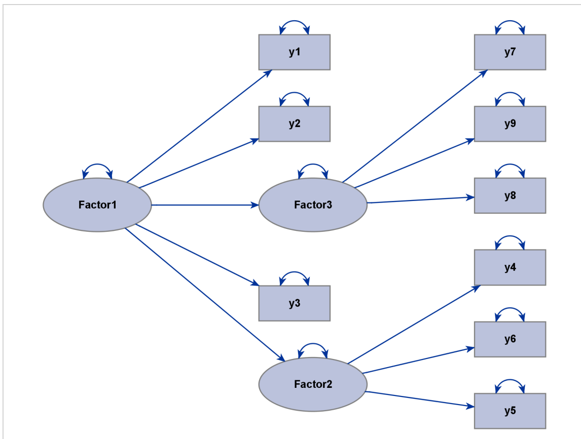
Figure 29.10 Applying the Process-Flow Algorithm to an Ideal Grouped-Flow Pattern
