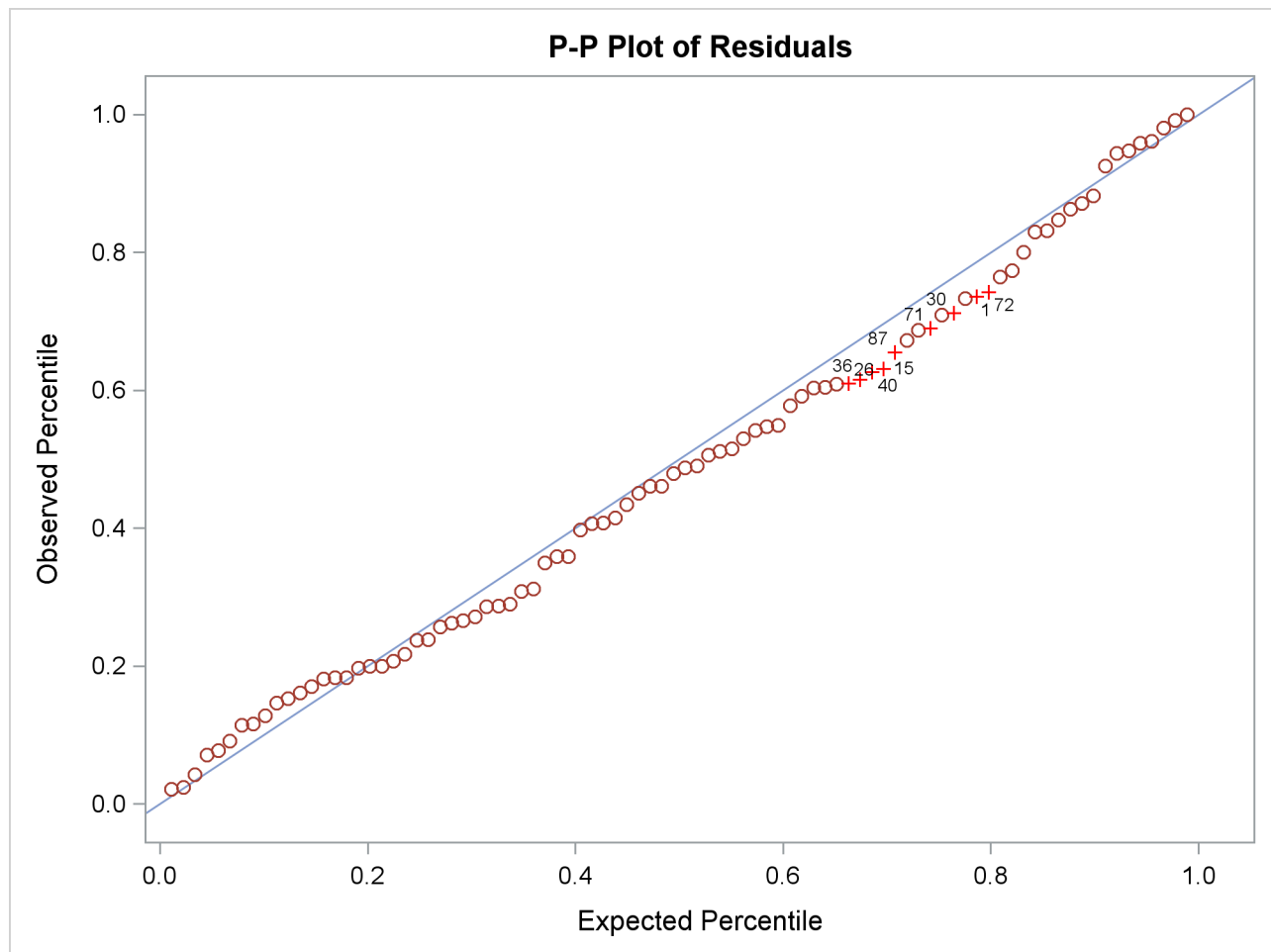
Output 29.14.8 P-P Plot of Residual M-Distances
