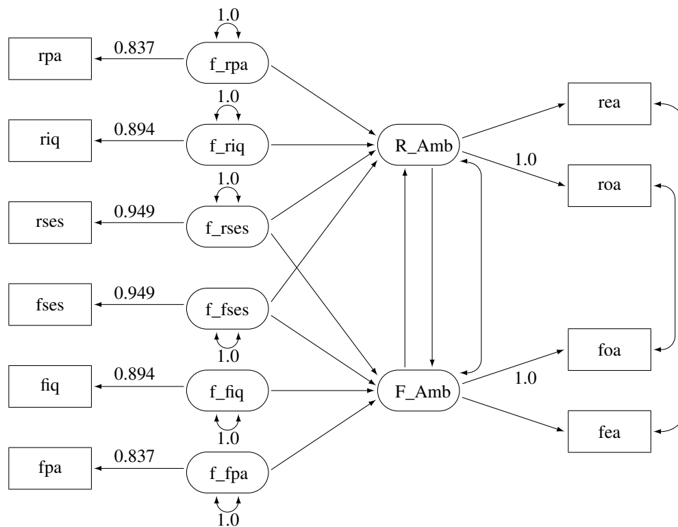
Figure 29.24 Path Diagram for Career Aspiration: Model 1
