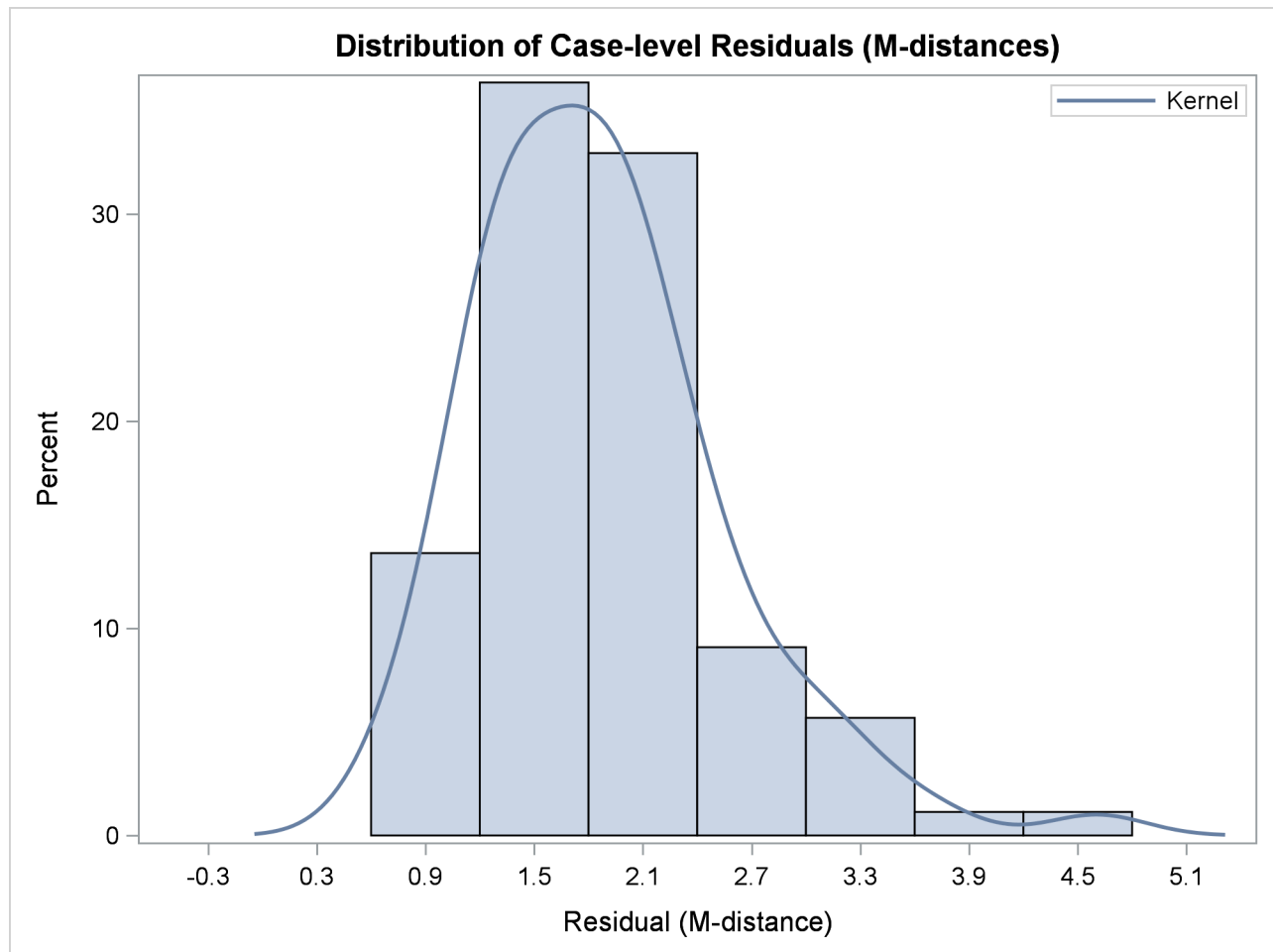
Output 29.14.6 Distribution of Case-Level Residuals
