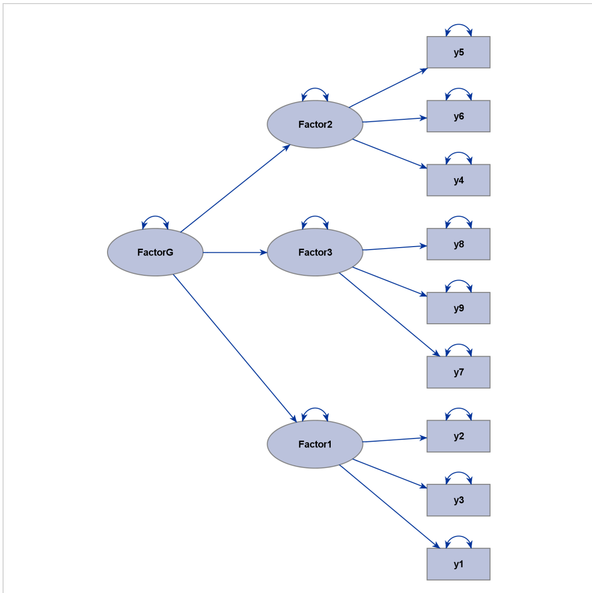
Figure 29.6 Linearly Ordered Factors with an Ideal Process-Flow Pattern
