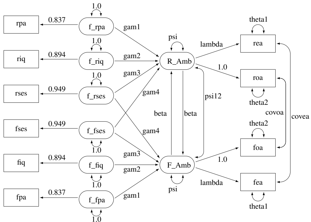
Figure 29.25 Path Diagram for Career Aspiration: Model 2
