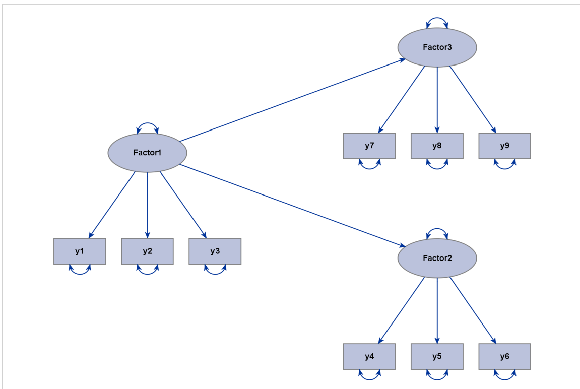
Figure 29.9 Hierarchically Ordered Factors with an Ideal Grouped-Flow Pattern
