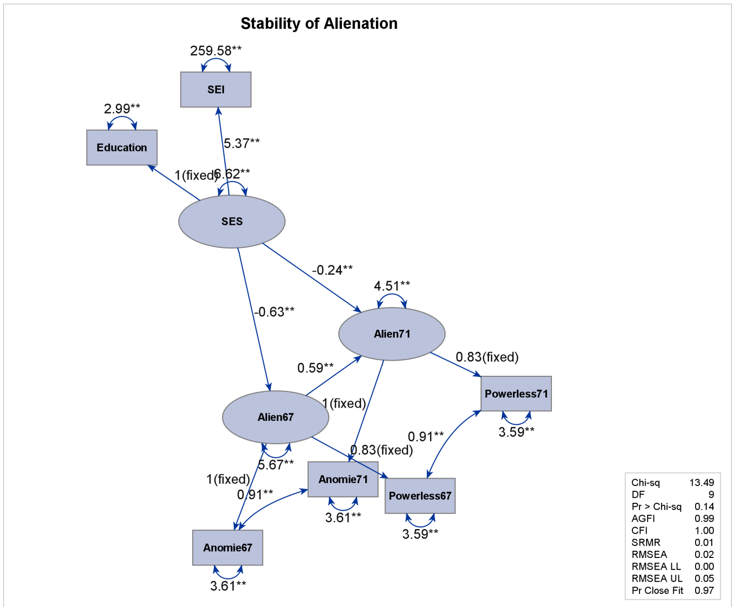
Output 29.17.7 Path Diagram and Fit Summary
