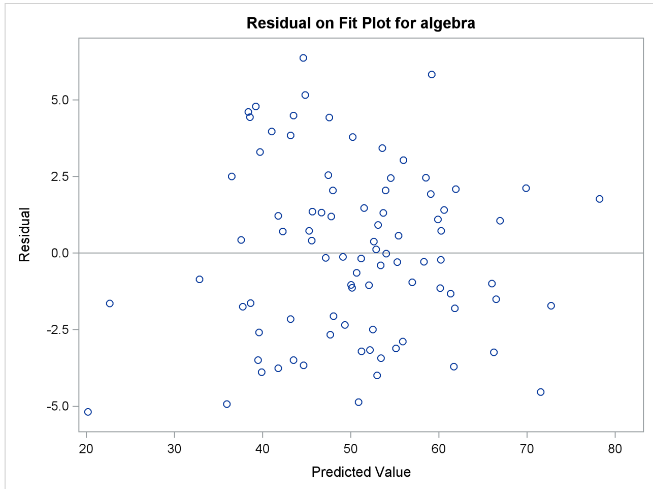
Output 29.14.10 Residual on Fit Plot for the Variable Algebra
