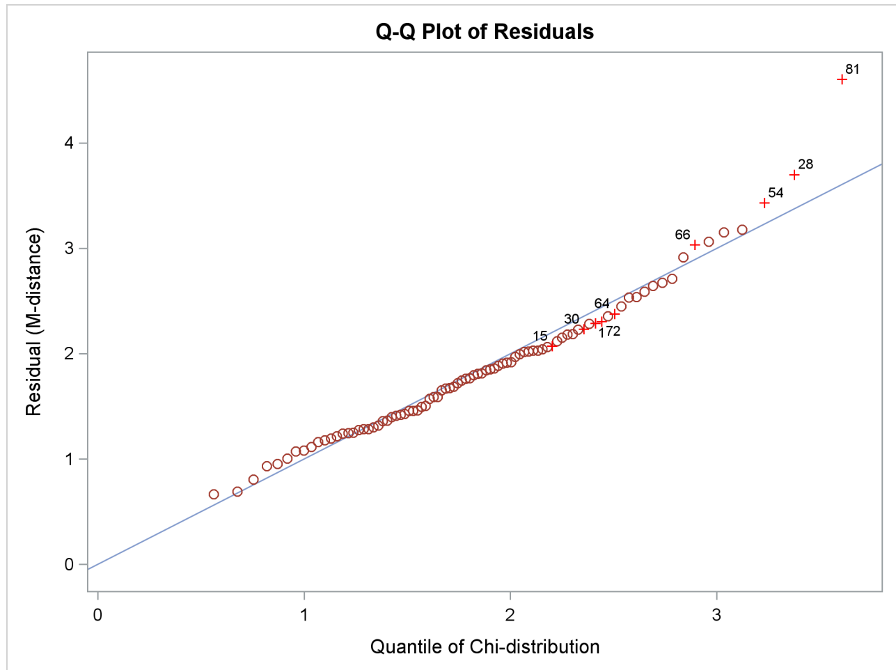
Output 29.14.7 Q-Q Plot of Residual M-Distances
