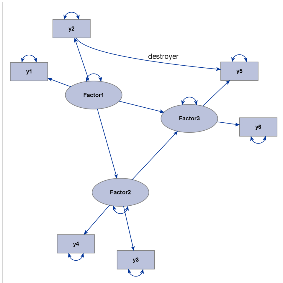
Figure 29.15 Path Diagram Whose Destroyer Path Is Handled by the GRIP Algorithm
