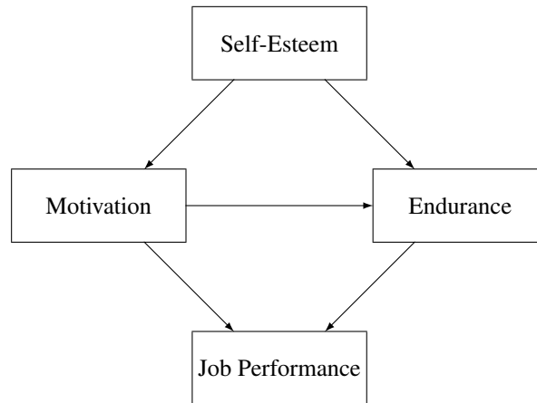
Figure 29.23 Direct and Indirect Effects of Self-Esteem on Job Performance
