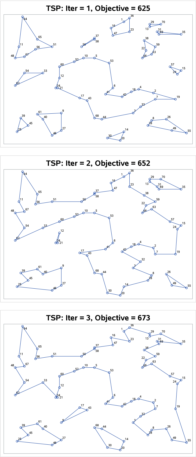
Output 9.6.1 Iterative Solution of Traveling Salesman Problem
