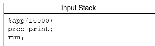
Figure 4.4 The Macro Call in the Input Stack
