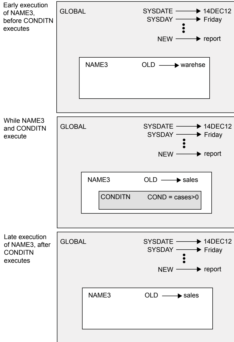
Figure 5.7 Symbol Tables Showing Two Levels of Nesting
