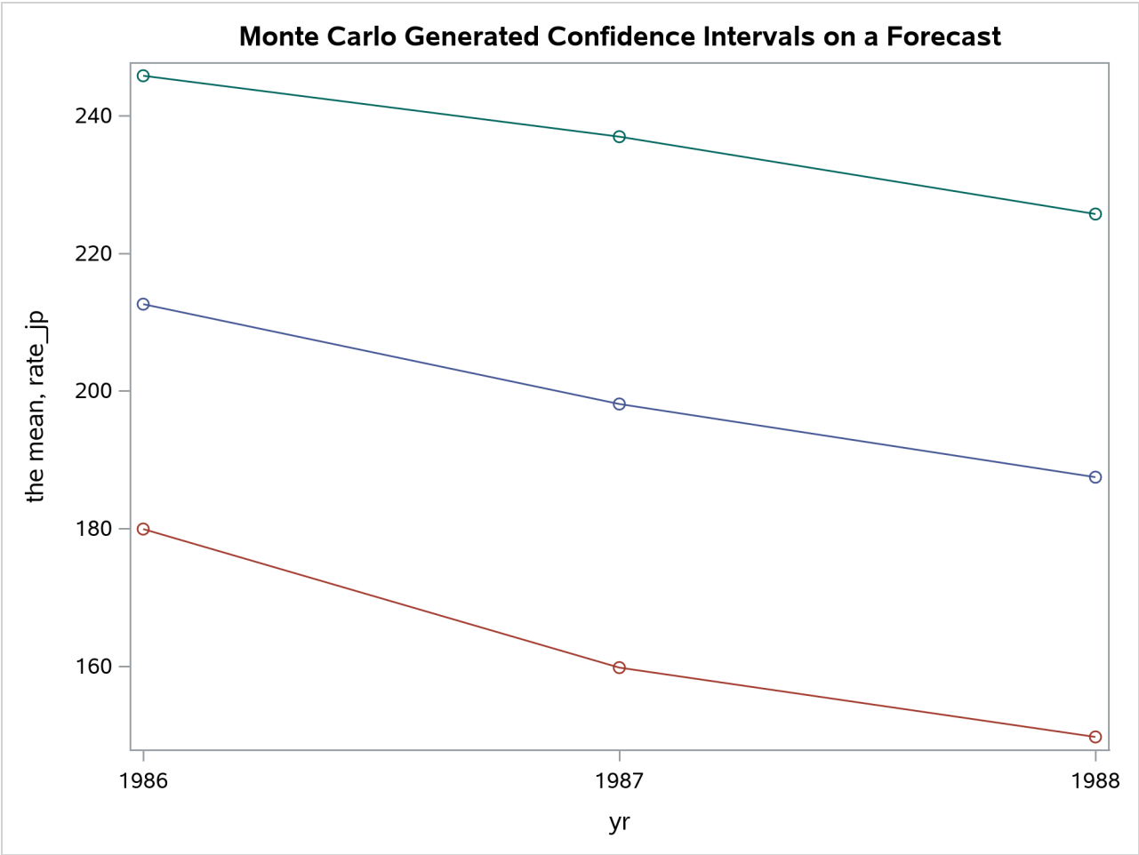
Figure 24.12 Monte Carlo Confidence Interval Plot
