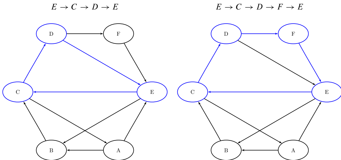
Figure 15.38 Cycles
