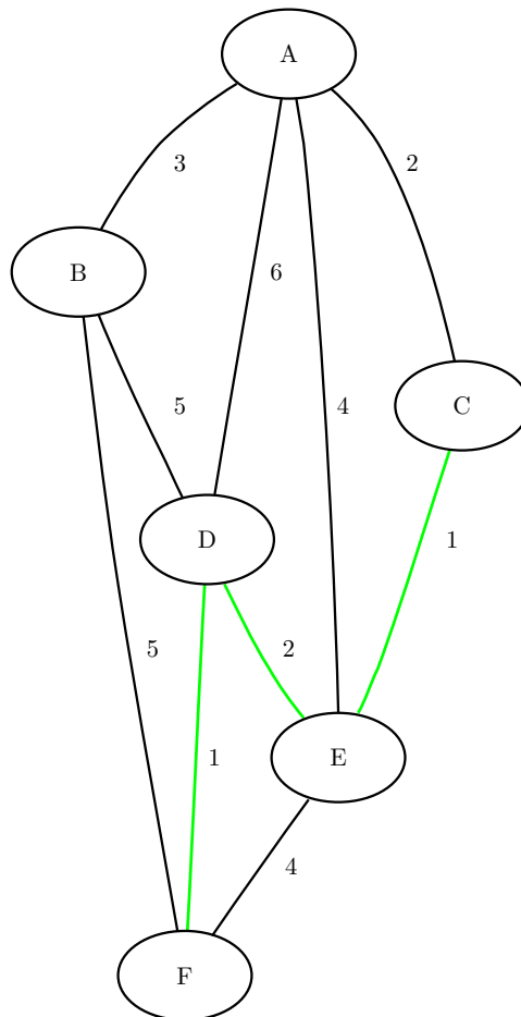
Figure 15.77 Shortest Path between Nodes C and F
