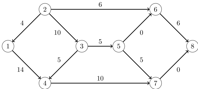
Figure 15.49 Minimum-Cost Network Flow Problem: Optimal Solution
