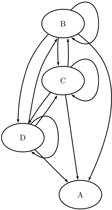
Figure 15.95 Transitive Closure of G
