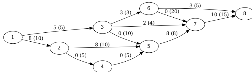
Figure 15.42 Maximum Network Flow Problem: Optimal Flows
