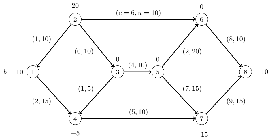
Figure 15.43 Minimum-Cost Network Flow Problem: Data
