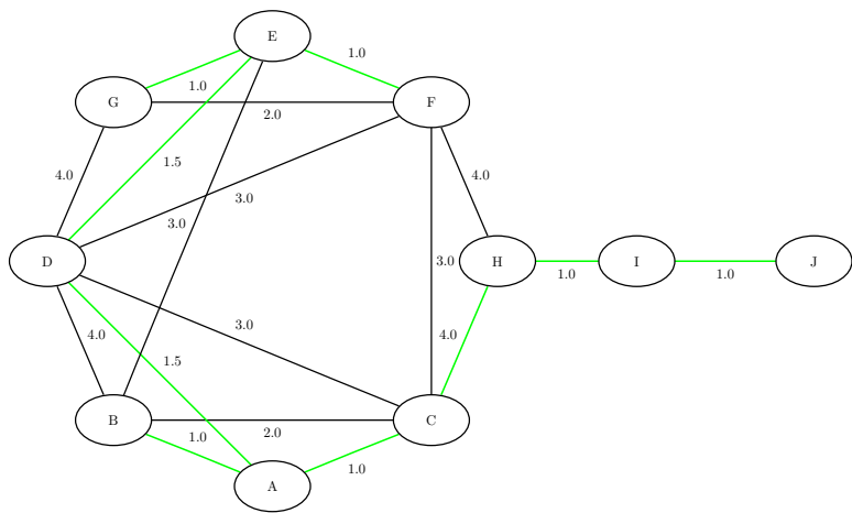
Figure 15.120 Minimum Spanning Tree for Office Computer Network
