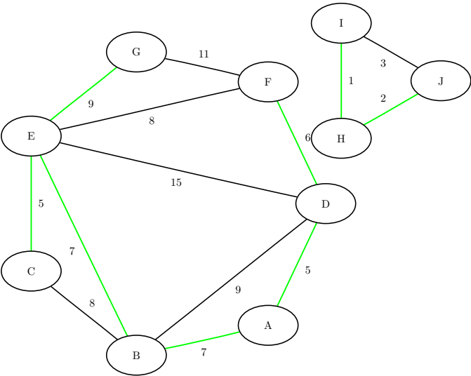
Figure 15.60 Minimum Spanning Forest
