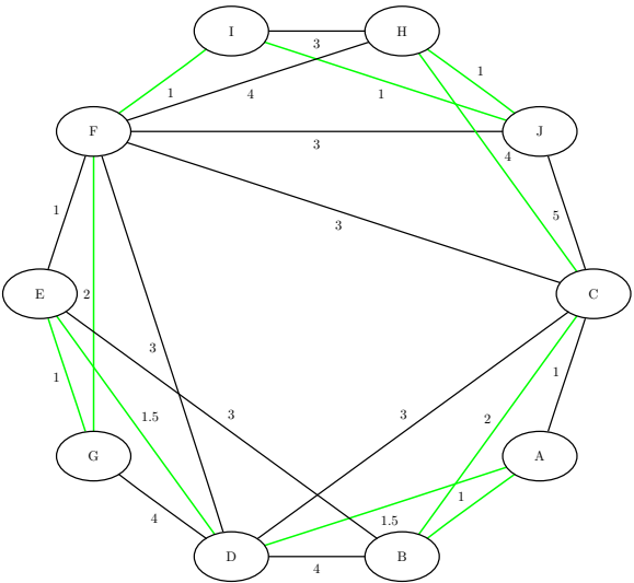
Figure 15.100 Optimal Traveling Salesman Tour
