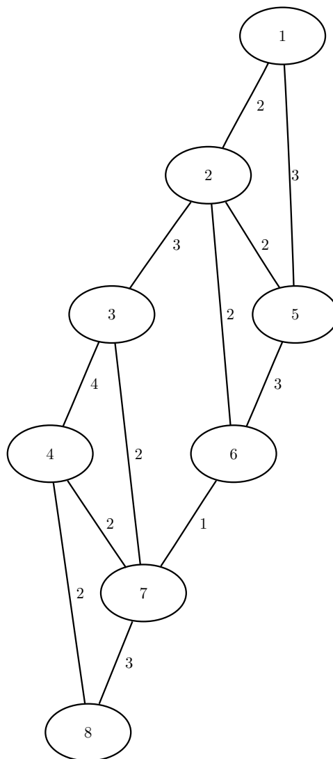
Figure 15.50 A Simple Undirected Graph
