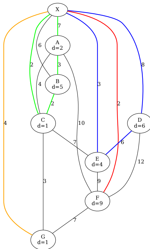
Figure 15.113 Optimal Routes
