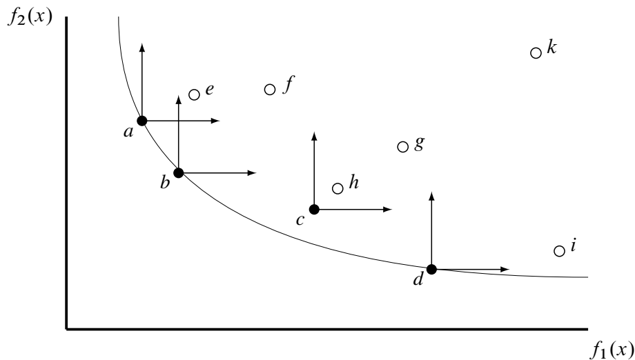
Figure 10.2 Pareto-Optimal Set
