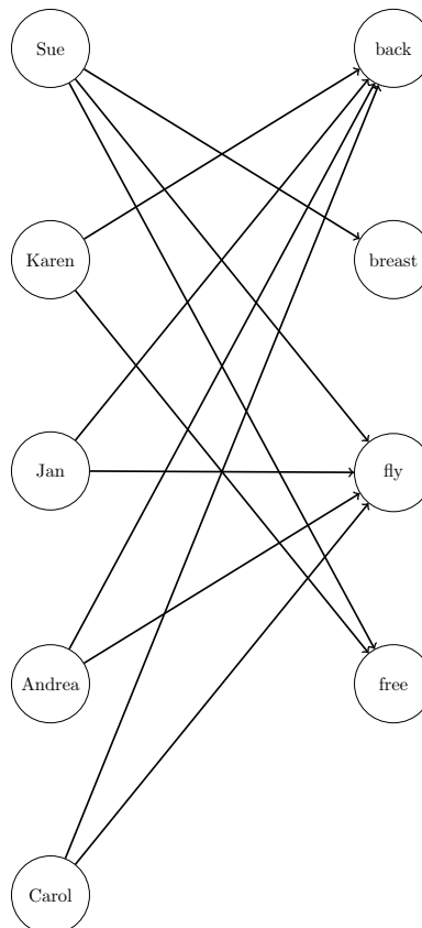
Figure 15.117 Bipartite Graph for Linear Assignment Problem
