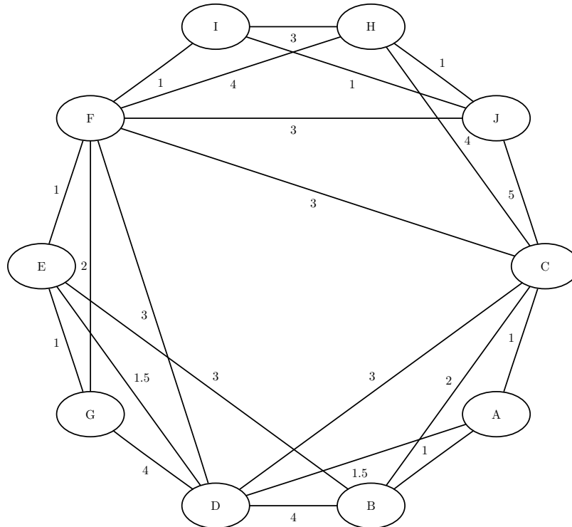
Figure 15.96 A Simple Undirected Graph
