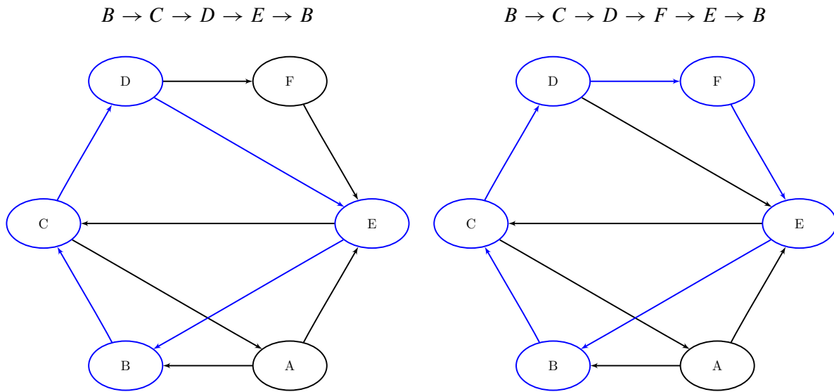
Figure 15.38 Cycles
