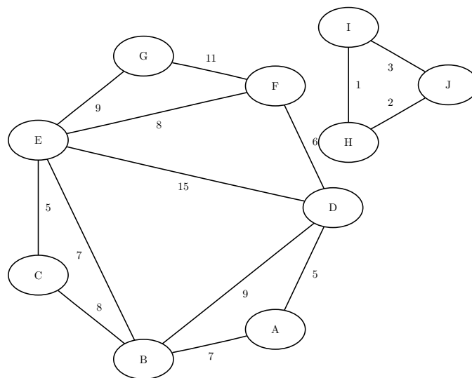
Figure 15.58 A Simple Undirected Graph
