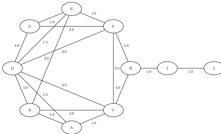
Figure 15.119 Potential Office Computer Network
