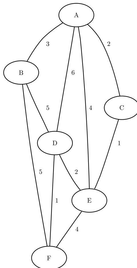
Figure 15.70 A Simple Undirected Graph G
