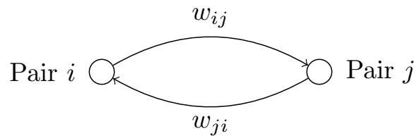
Figure 15.116 Kidney Donor Exchange Network
