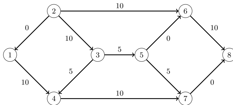
Figure 15.46 Minimum-Cost Network Flow Problem: Optimal Solution
