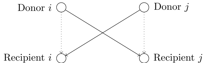
Figure 15.115 Kidney Donor Exchange Two-Way Swap
