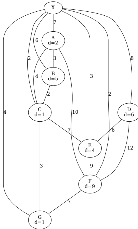
Figure 15.106 Undirected Graph
