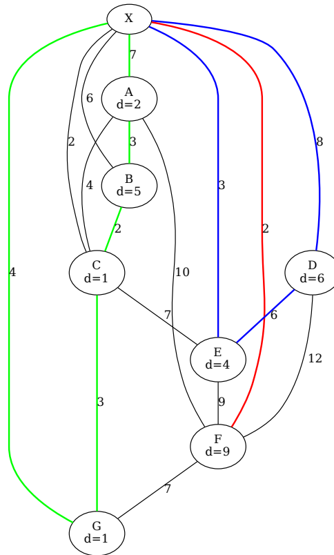
Figure 15.110 Optimal Routes
