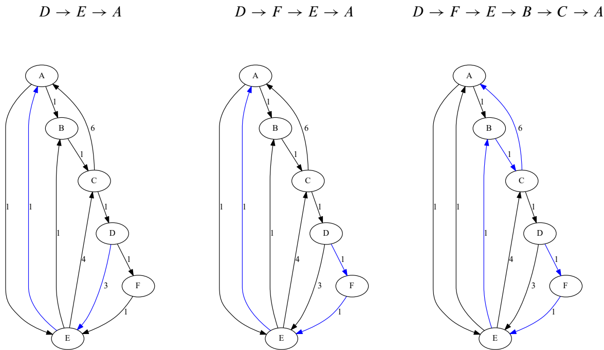
Figure 15.69 Paths
