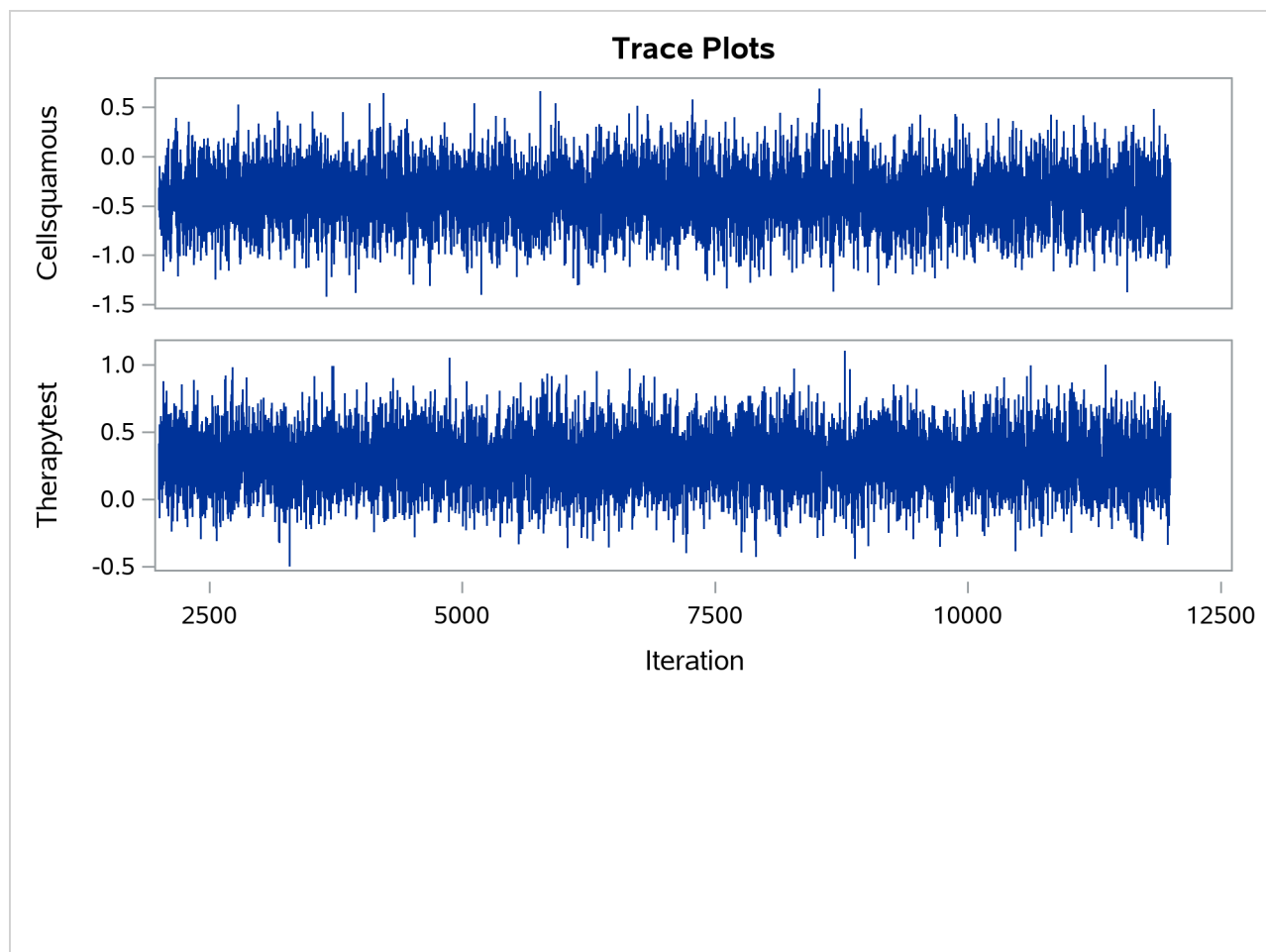
Output 92.13.10 continued
