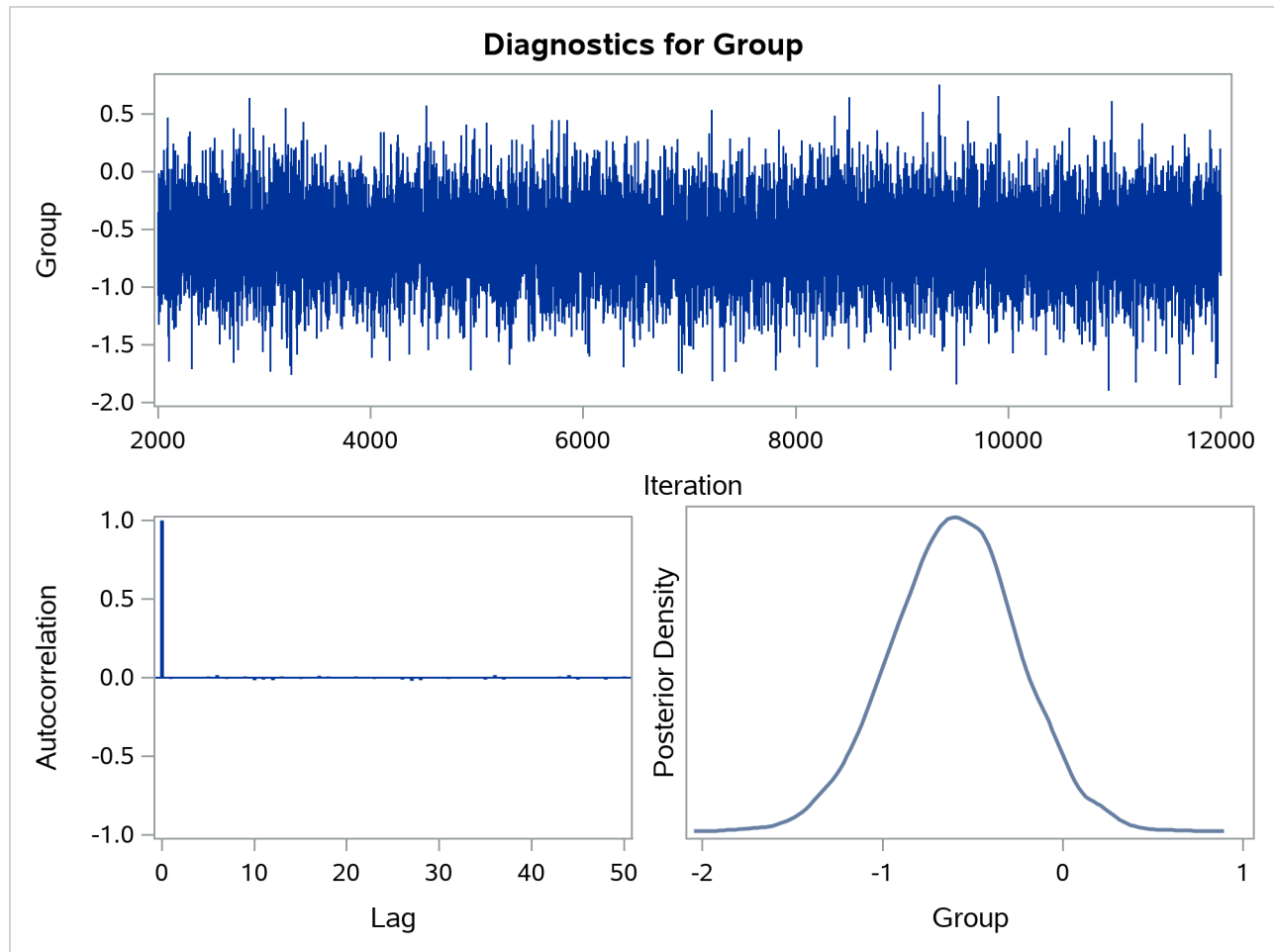
Figure 92.10 Diagnostic Plots
