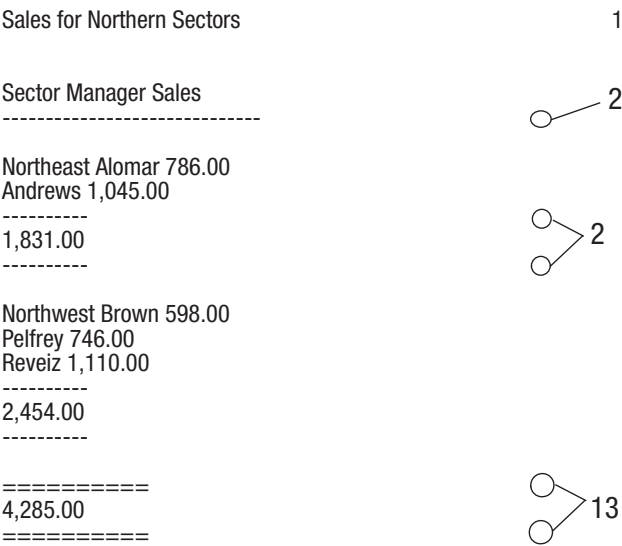
Figure 59.8 Formatting Characters in PROC REPORT Output
