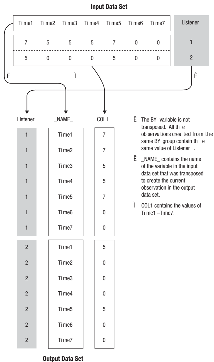
Figure 71.10 Transposing Two Observations
