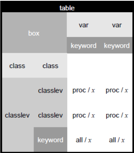
Figure 71.7 PROC TABULATE Areas and Corresponding Statements
