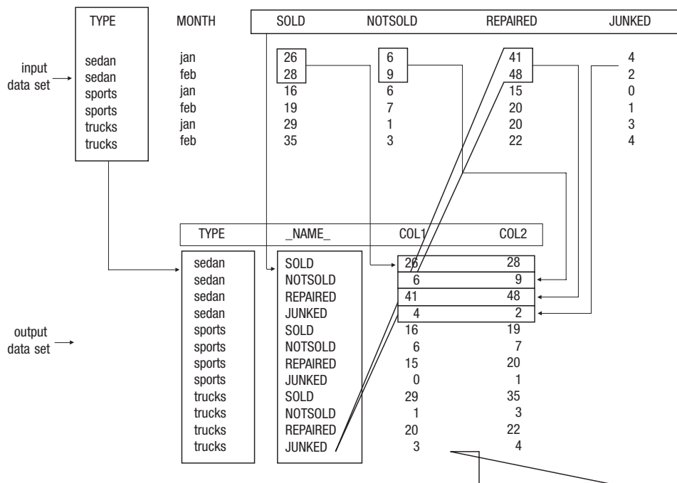
Figure 73.1 Transposition with BY Groups
