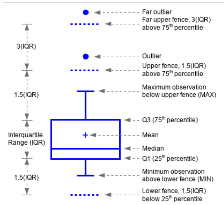
Figure 10.3 Parts of a Box Plot
