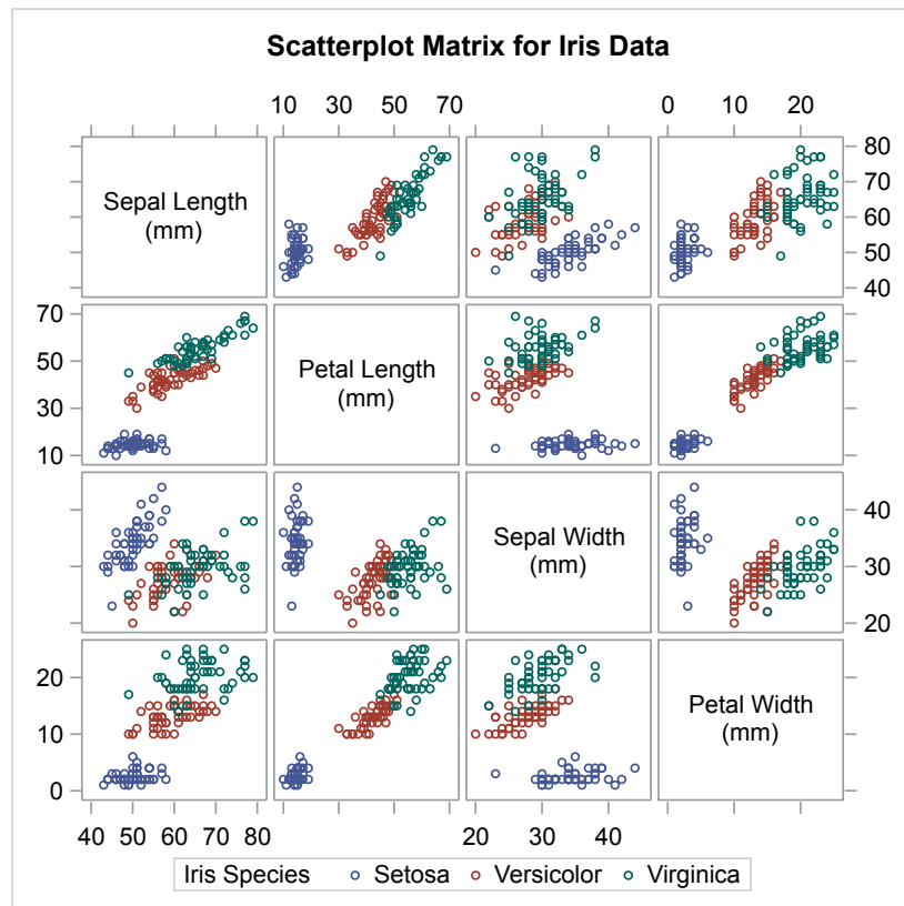
Figure 12.3 Example Graph from the MATRIX Statement
