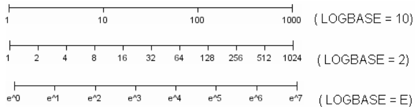
Figure 8.12 Graph Axes with LOGEXPAND
