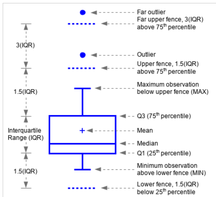
Figure 8.11 Parts of a Box Plot
