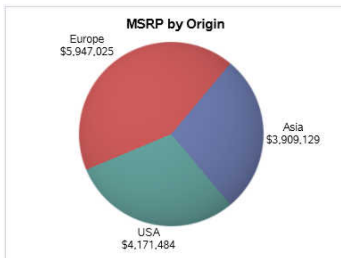
Figure 3.1 Pie Chart
