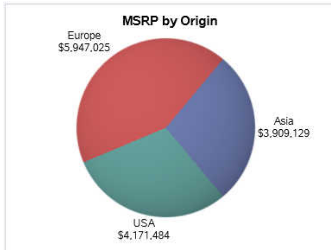
Figure 9.1 Pie Chart
