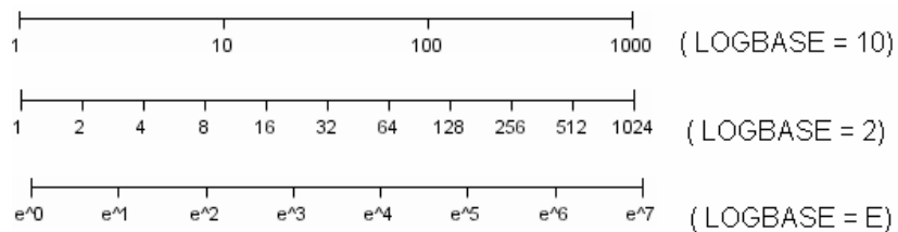
Figure 10.10 Graph Axes with LOGEXPAND
