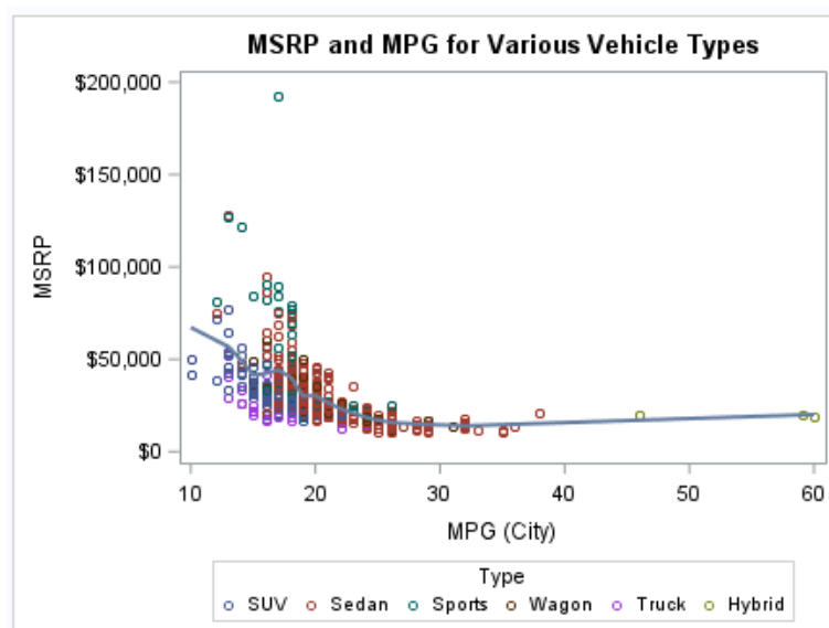
Figure 10.6 Graph without the LEGENDITEM or KEYLEGEND Statements
