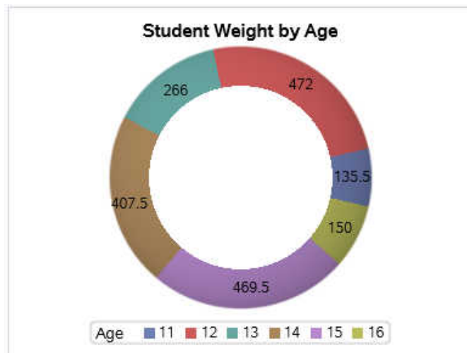
Figure 9.2 Donut Chart
