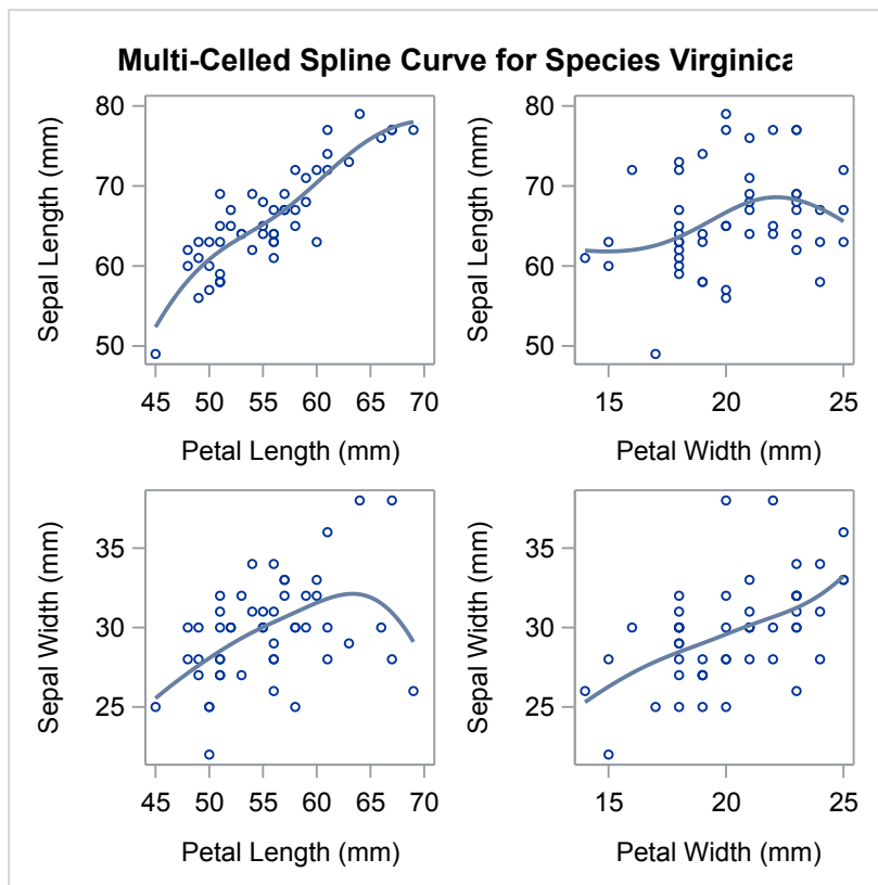
Figure 12.1 Example Graph from the PLOT Statement
